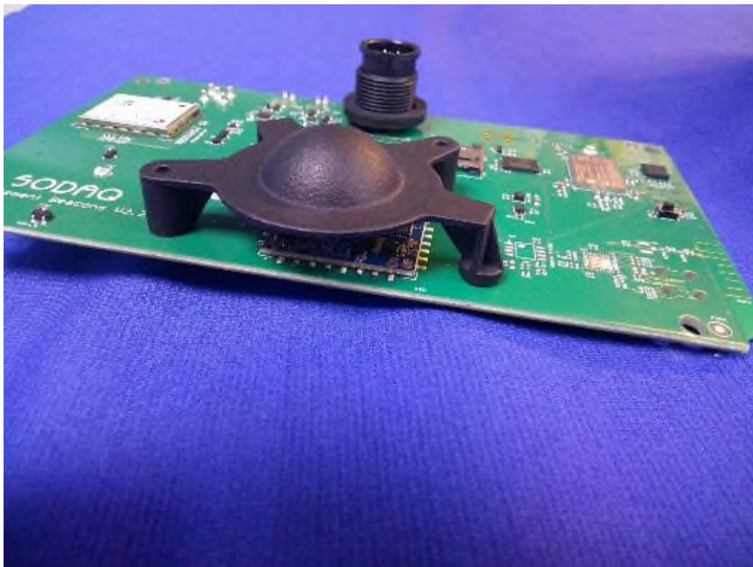
Photograph shows the EUTs 60GHz RADAR antenna with lens fitted
