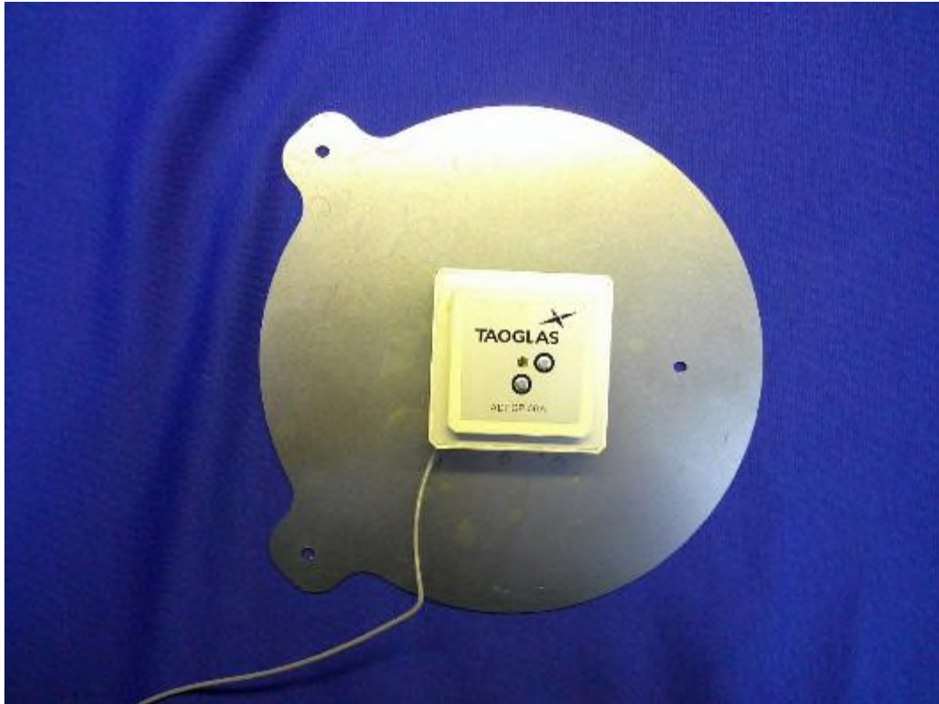
Photograph shows the EUT GPS antenna
