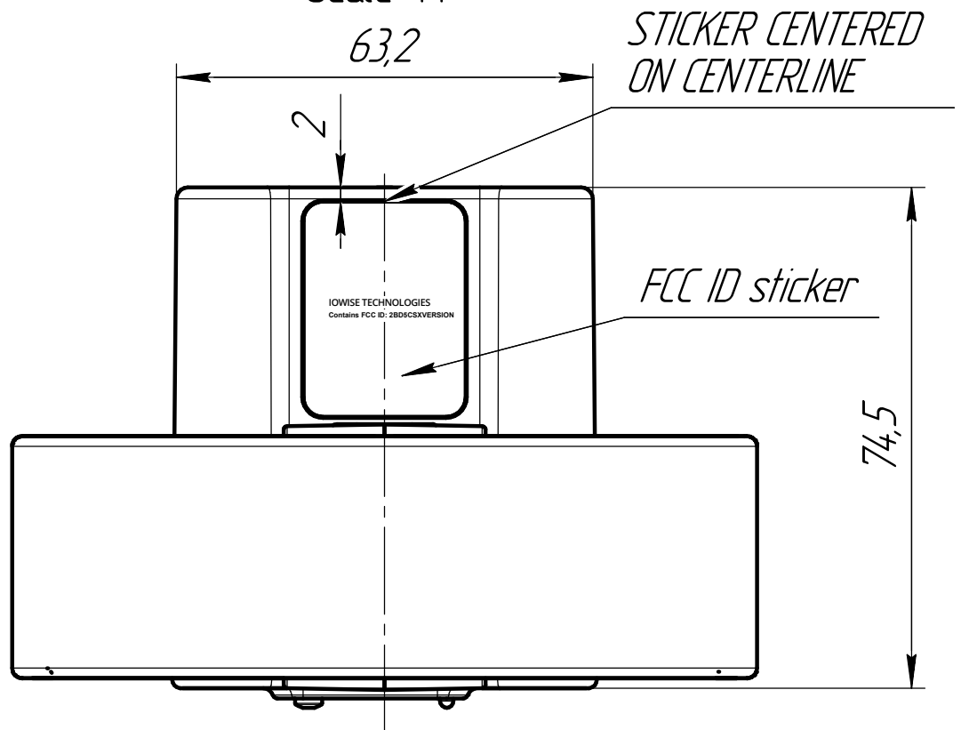
Back view of device Scale: 1:1
