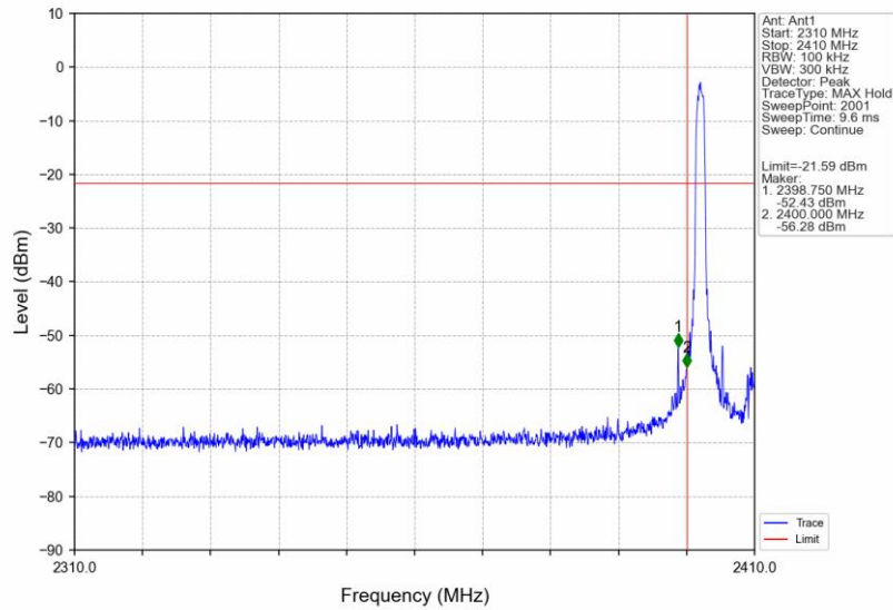
8DPSK_3DH5_LCH_2402MHz_Ant1_NTNV
