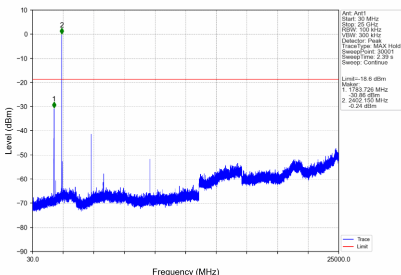
GFSK_DH5_LCH_2402MHz_Ant1_NTNV
