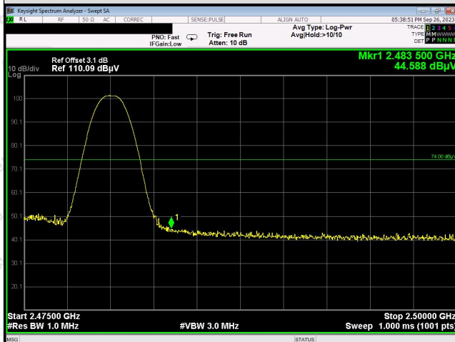
Peak Value(Vertical)
