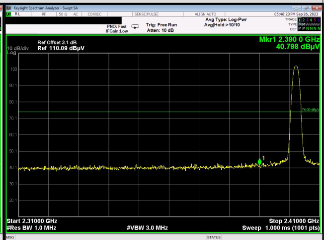
Peak Value(Horizontal)
