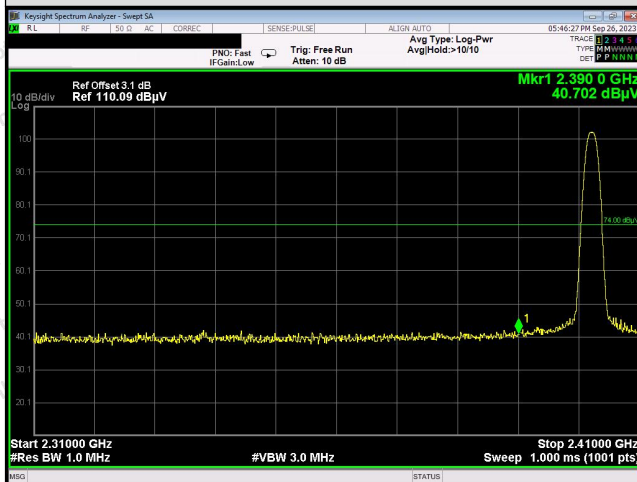
Peak Value(Vertical)
