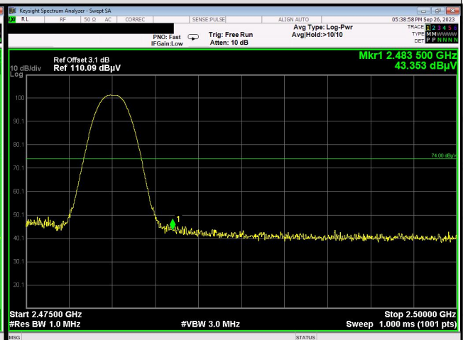
Peak Value(Horizontal)
