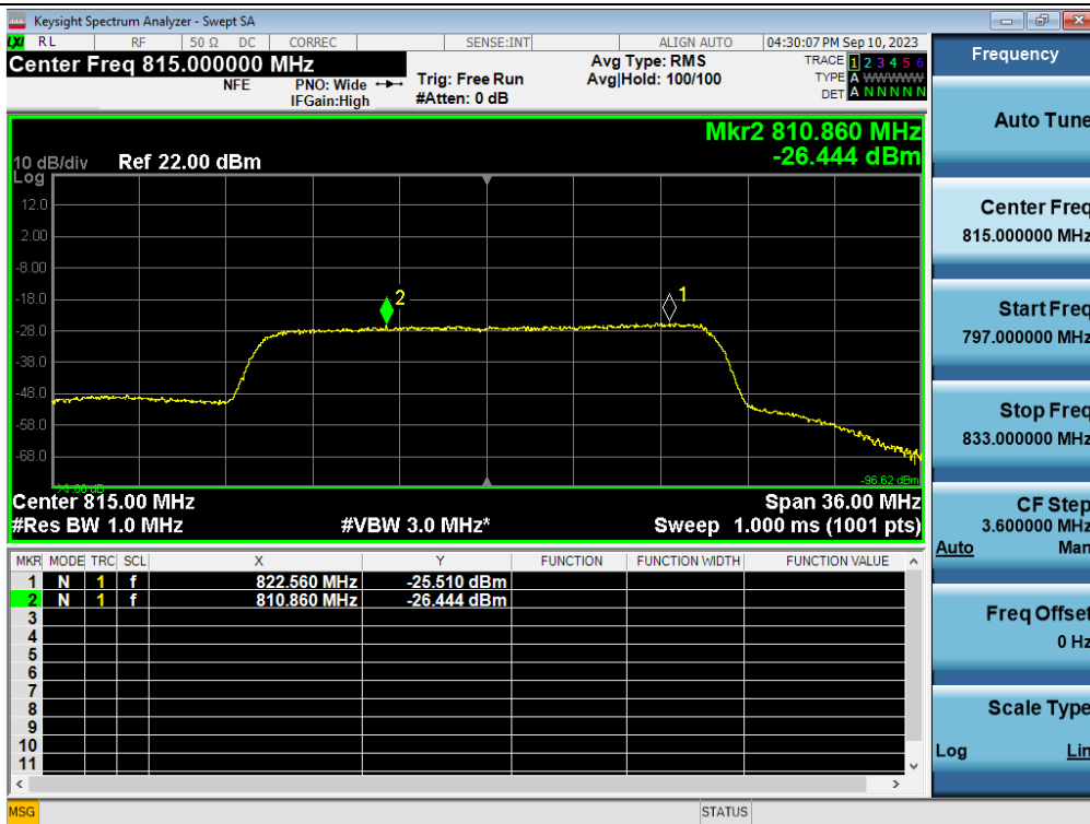
Noise Figure / 800 MHz / Uplink
