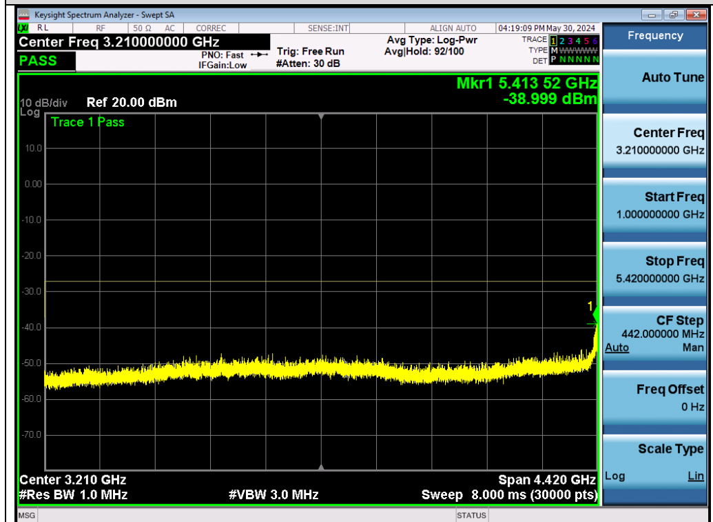
Test_Graph_802.11ac80_ANT1_5530_MCS9_Frequency Band 2
