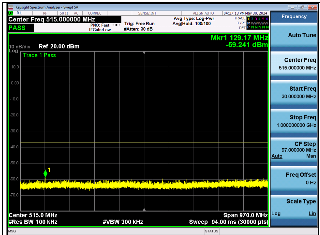
Test_Graph_802.11ac20_ANT1_5825_MCS9_Frequency Band1
