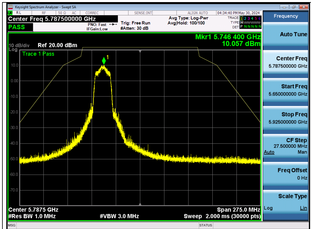
Test_Graph_802.11ac20_ANT1_5745_MCS0_Frequency Band3
