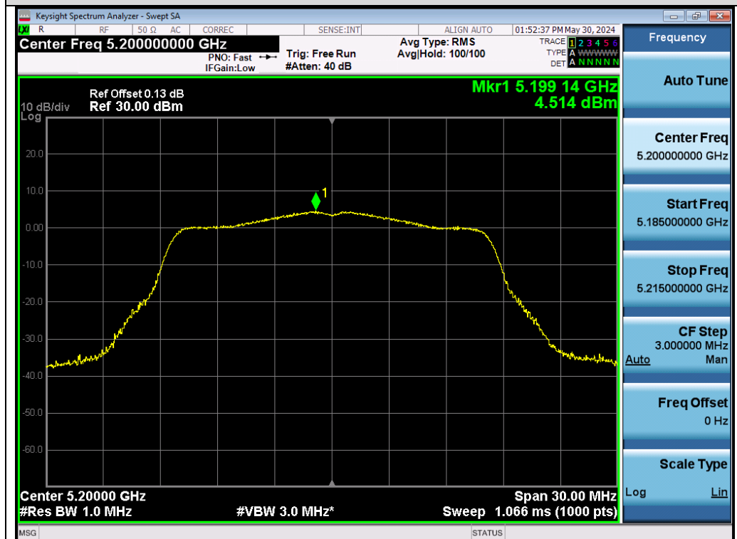
Test_Graph_802.11a_ANT1_5200_6Mbps_PSD
