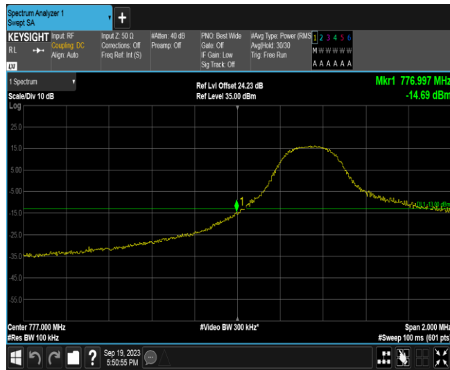
Band13-5MHz-QPSK-23205-1RB#24
