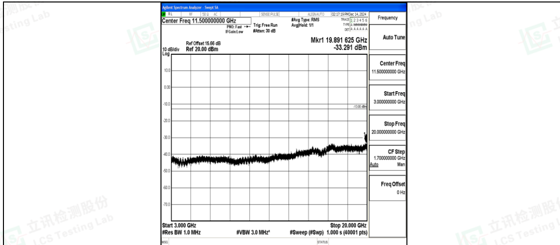
Band2_5MHz_16QAM_18900_1RB#0_3000~20000_3000~20000
