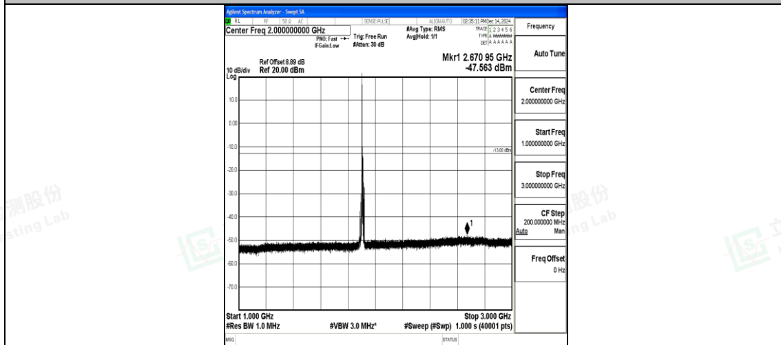
Band2_10MHz_QPSK_19150_1RB#0_1000~3000_1000~3000
