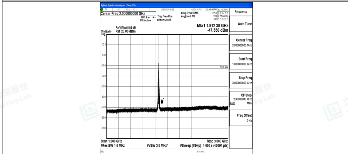
Band2_15MHz_16QAM_18675_1RB#0_1000~3000_1000~3000
