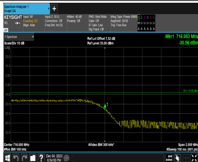
Band12-5MHz-16QAM-23155-1RB#0
