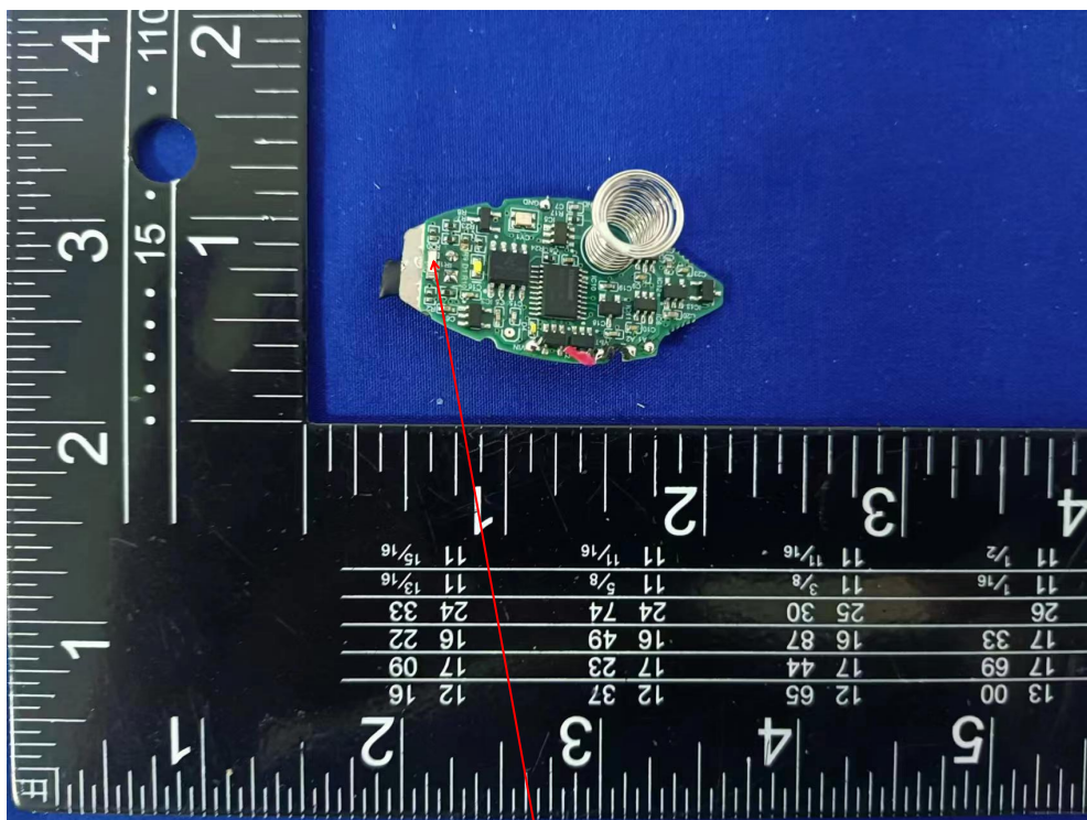
Chip antenna
