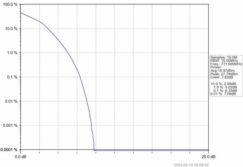
Band12_10MHz_16QAM_HCH_711MHz_RB_50_0_NTNV
