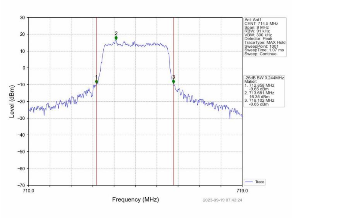
Band12_3MHz_16QAM_HCH_714.5MHz_RB_15_0_NTNV
