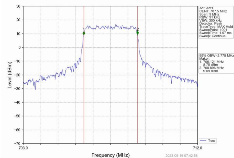
Band12_3MHz_QPSK_MCH_707.5MHz_RB_15_0_NTNV
