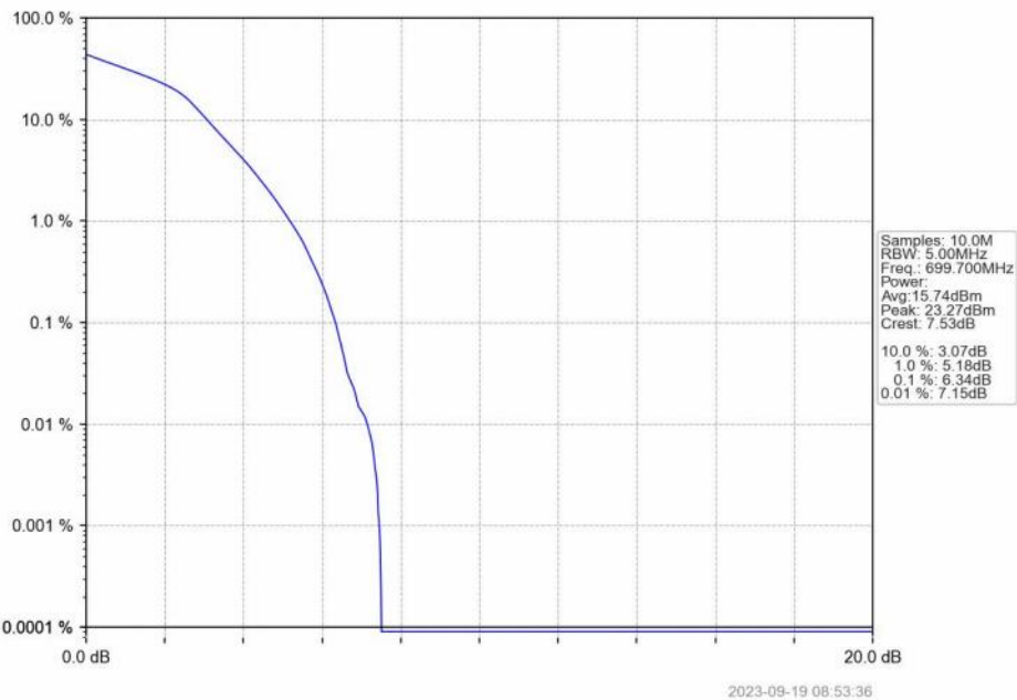
Band12_1.4MHz_16QAM_LCH_699.7MHz_RB_6_0_NTNV
