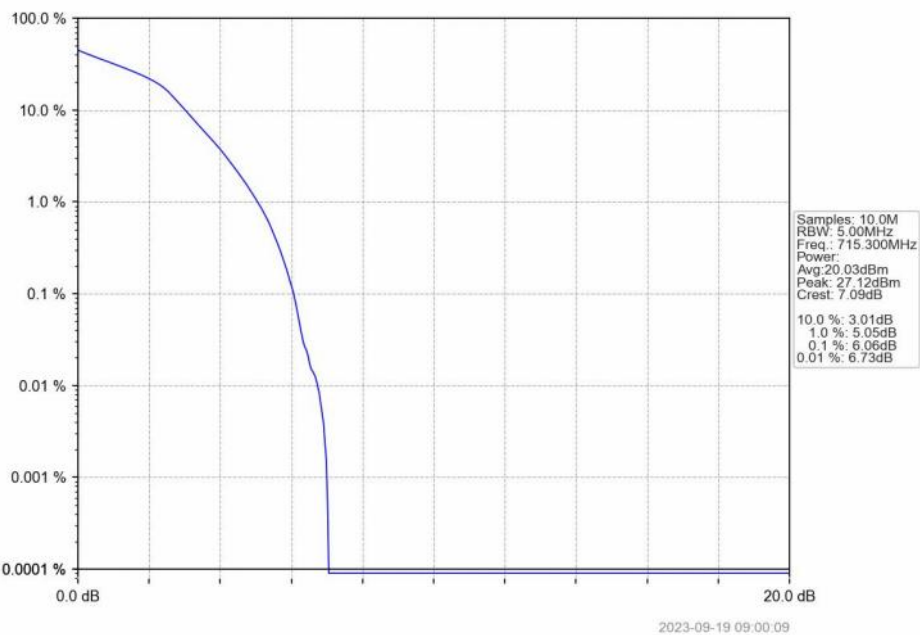
Band12_1.4MHz_16QAM_HCH_715.3MHz_RB_6_0_NTNV
