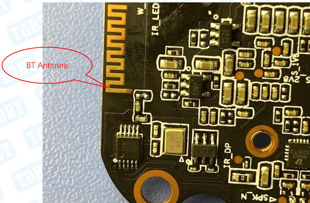
Photo 24 Appearance of PCB
