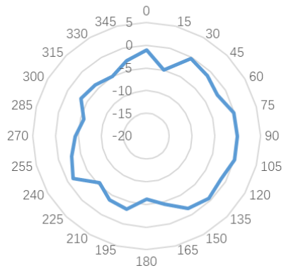
5250MHz_Theta=90°
