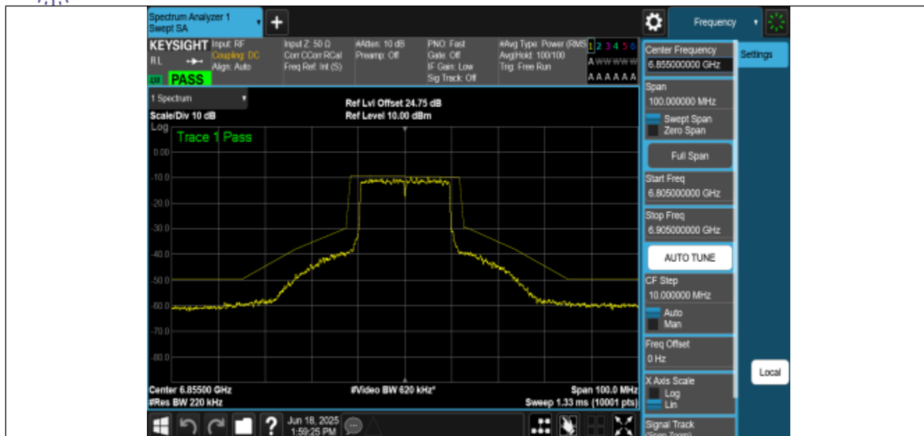
NTNV-11AX20MIMO-Ant2-6855-PASS
