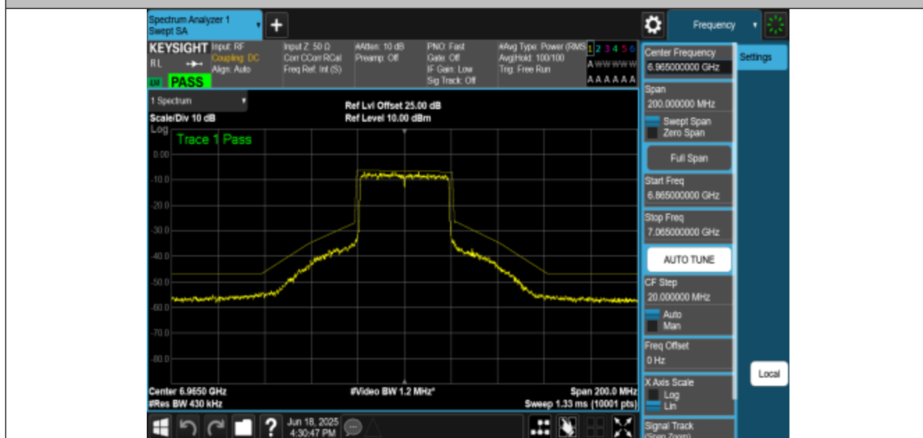
NTNV-11AX40MIMO-Ant3-6965-PASS
