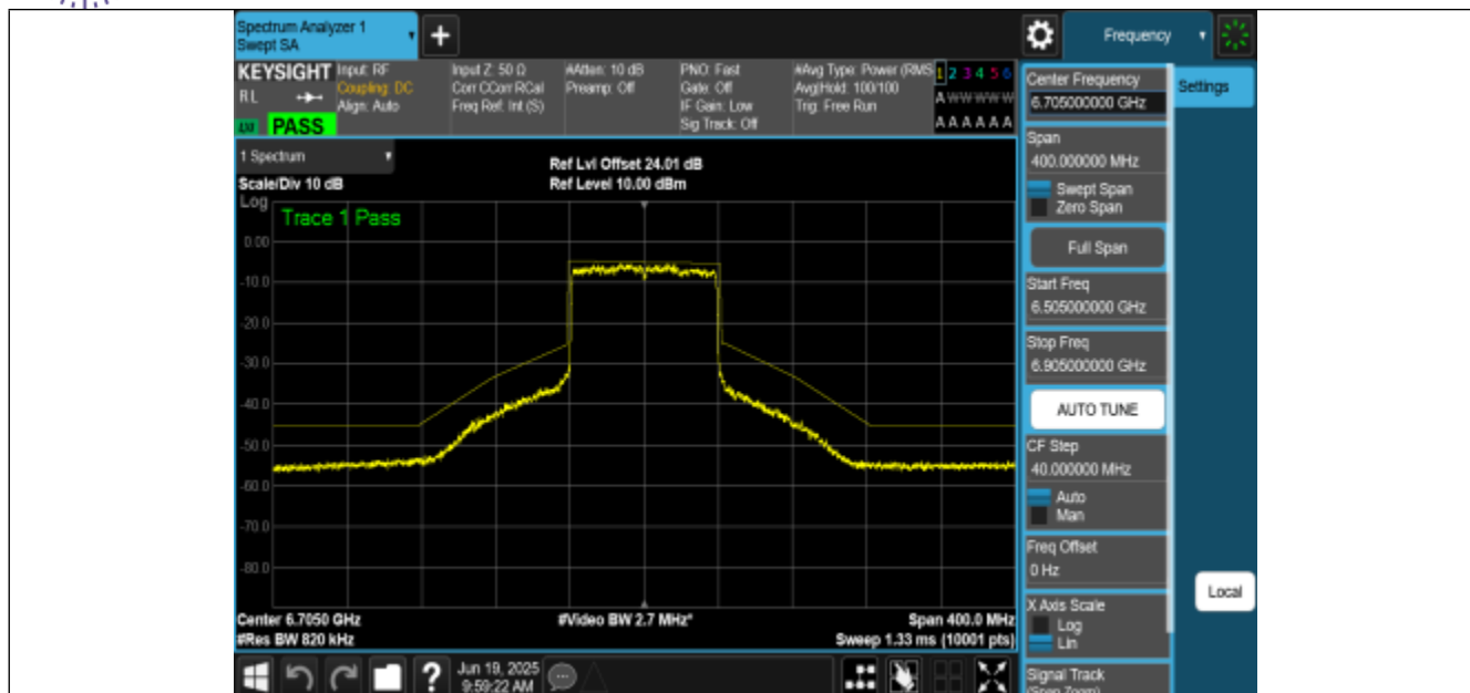
NTNV-11AX80MIMO-Ant0-6705-PASS
