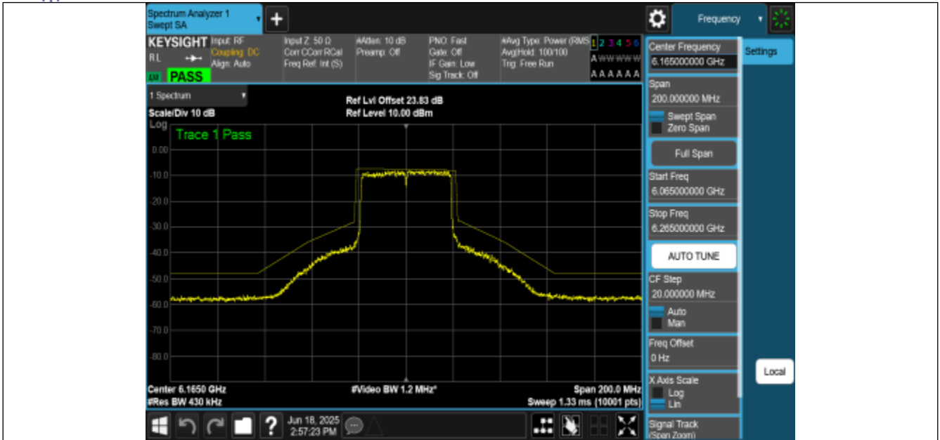
NTNV-11AX40MIMO-Ant0-6165-PASS
