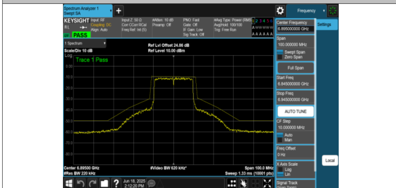
NTNV-11AX20MIMO-Ant3-6895-PASS
