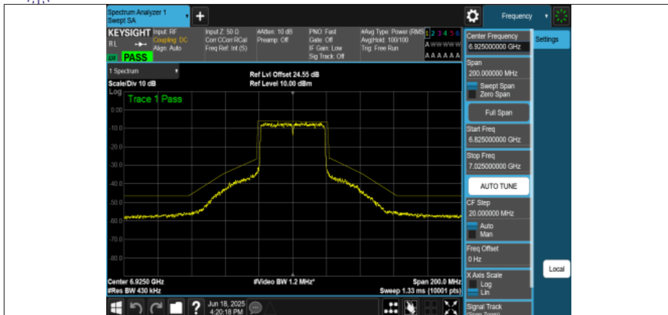
NTNV-11AX40MIMO-Ant2-6925-PASS
