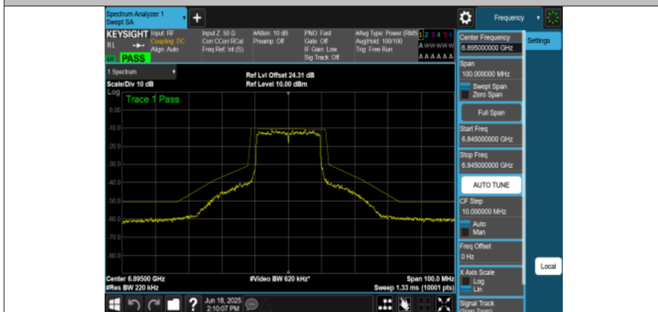
NTNV-11AX20MIMO-Ant1-6895-PASS
