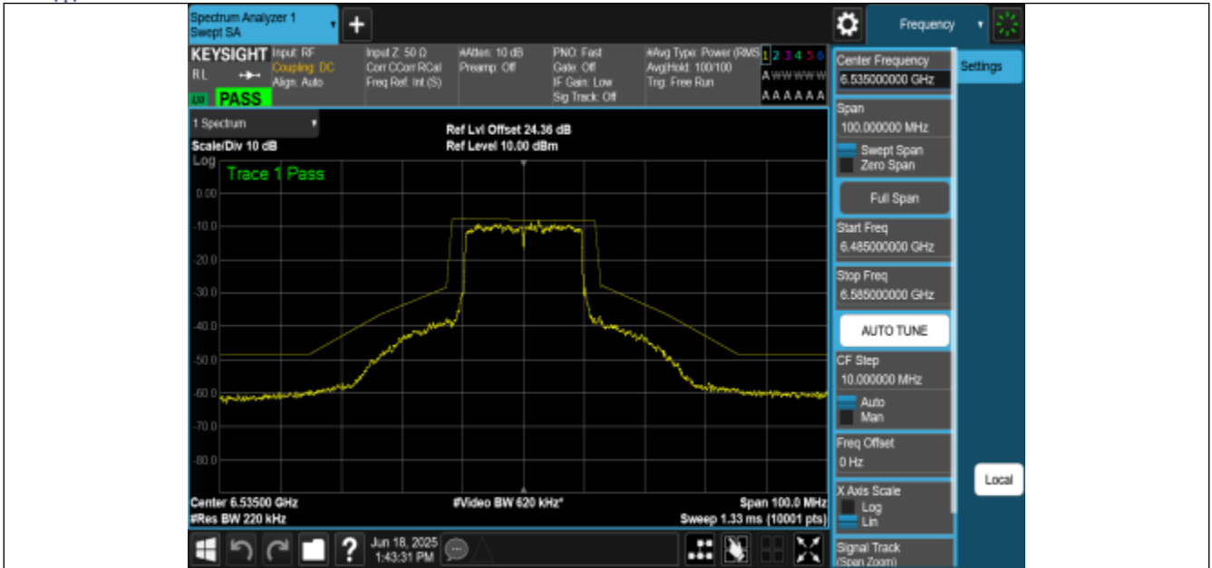
NTNV-11AX20MIMO-Ant0-6535-PASS
