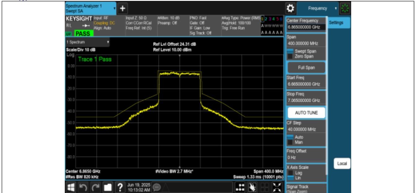
NTN-11AX80MIMO-Ant0-6865-PASS
