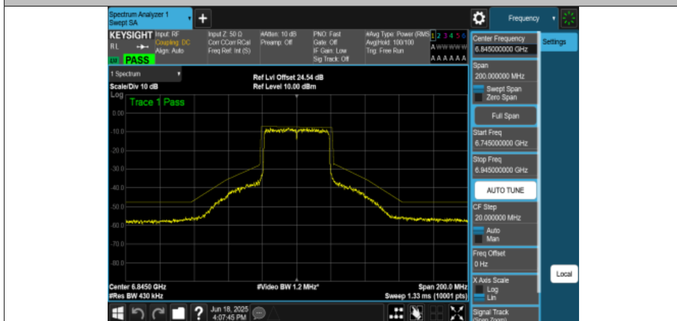
NTNV-11AX40MIMO-Ant1-6845-PASS
