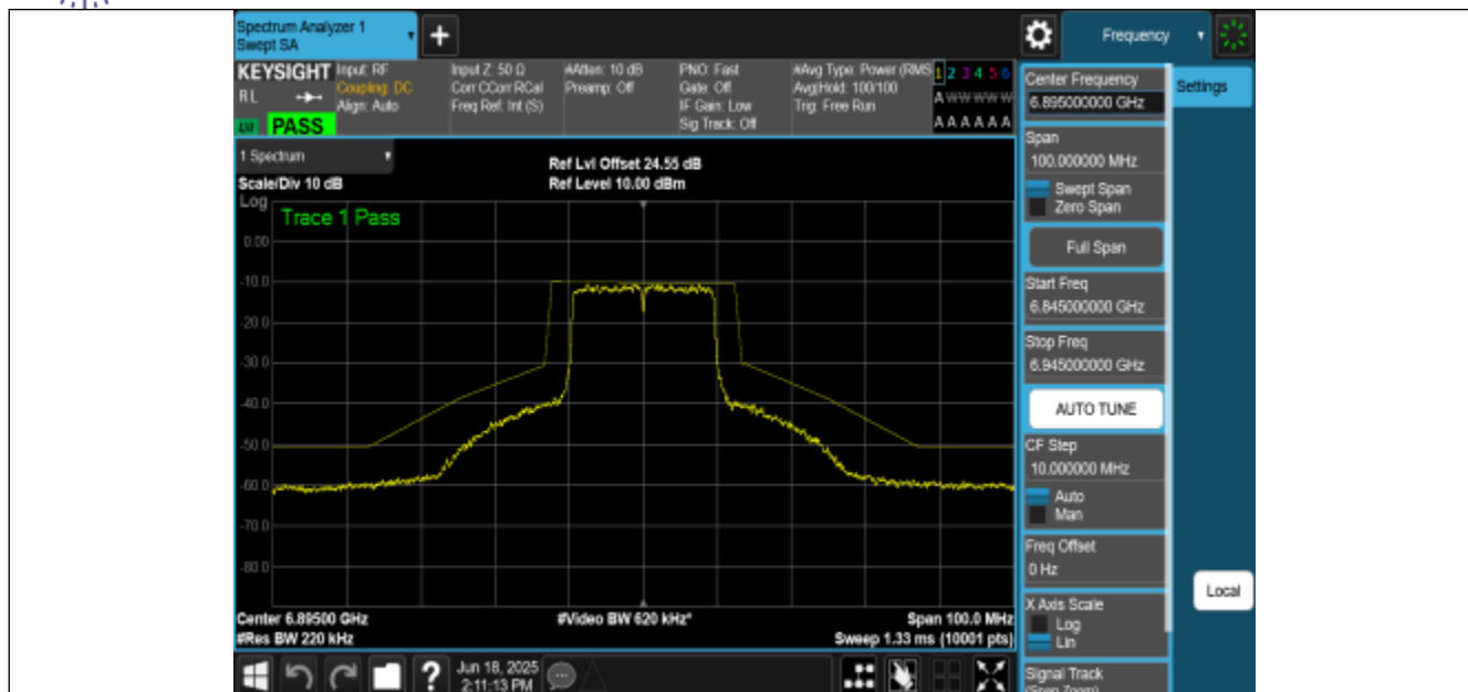
NTNV-11AX20MIMO-Ant2-6895-PASS
