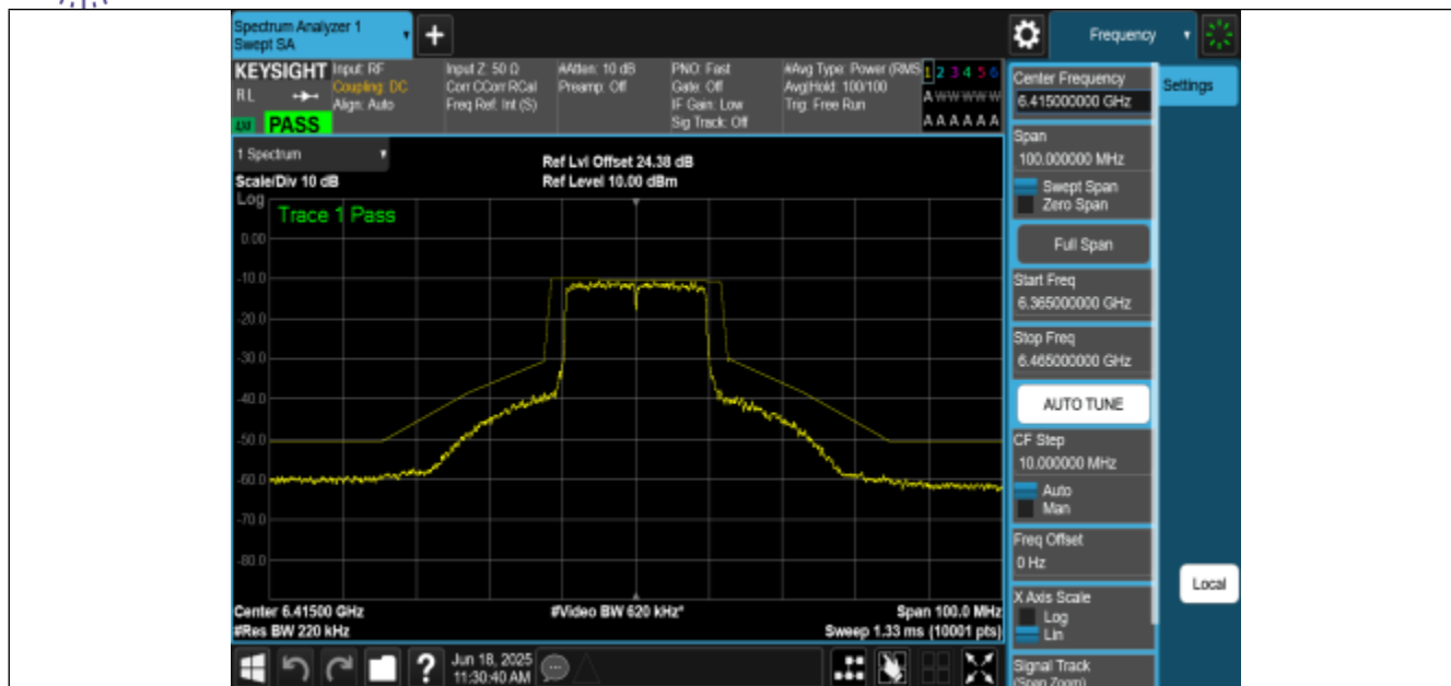
NTNV-11AX20MIMO-Ant2-6415-PASS
