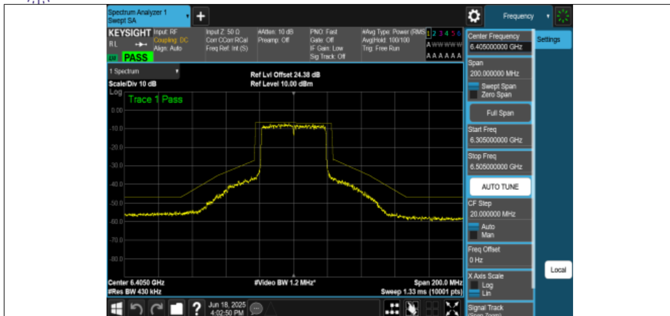
NTNV-11AX40MIMO-Ant2-6405-PASS
