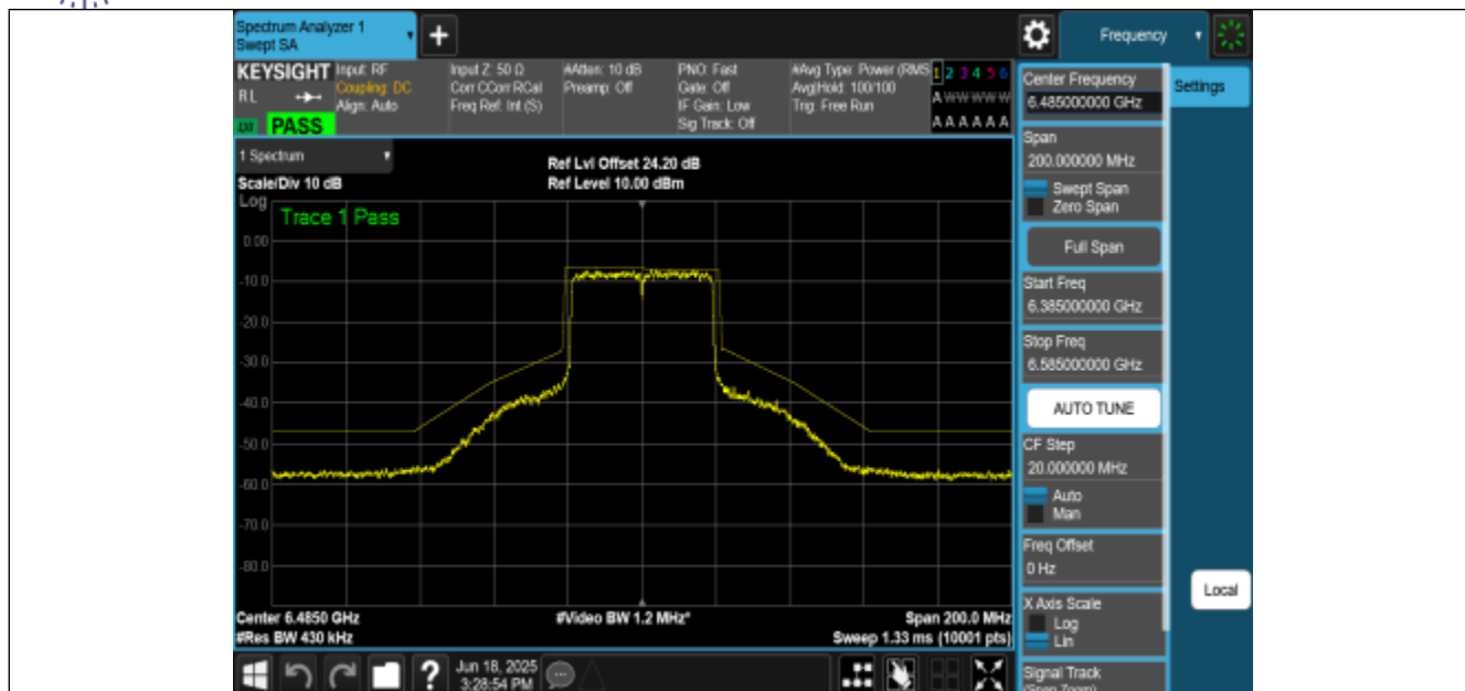
NTNV-11AX40MIMO-Ant2-6485-PASS
