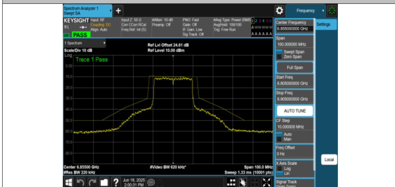
NTNV-11AX20MIMO-Ant3-6855-PASS
