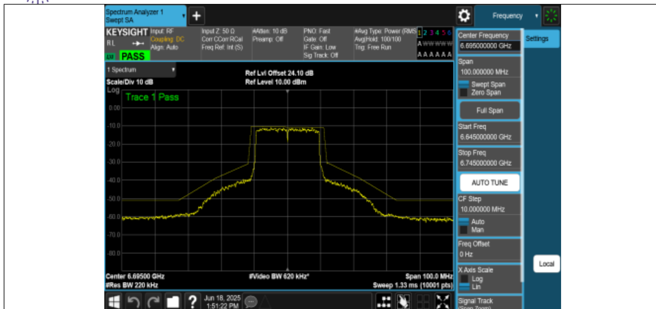
NTNV-11AX20MIMO-Ant0-6695-PASS
