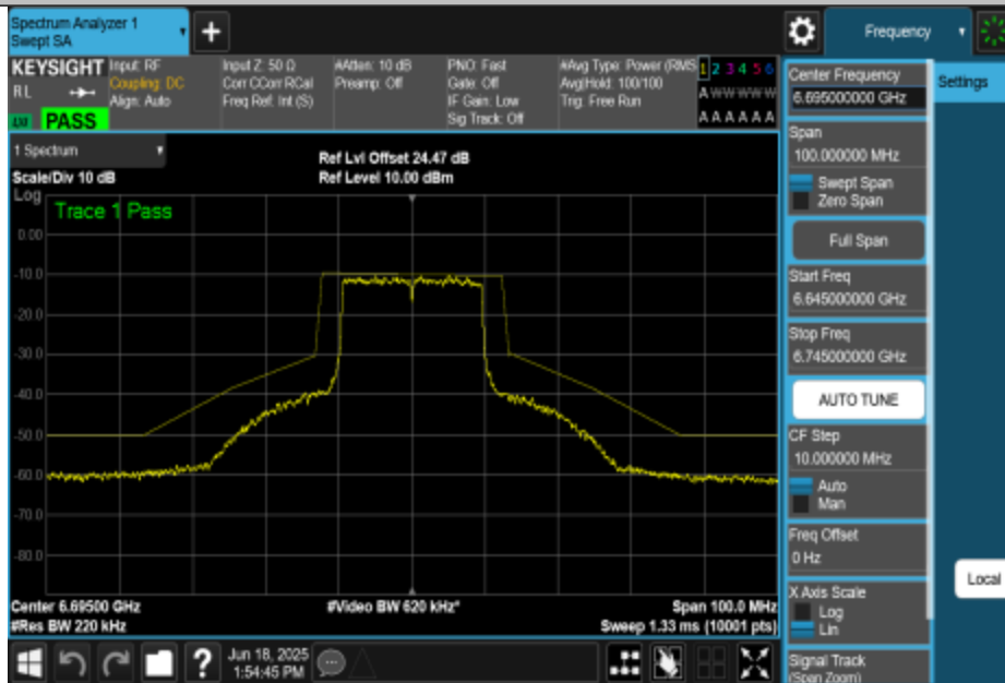
NTNV-11AX20MIMO-Ant3-6695-PASS
