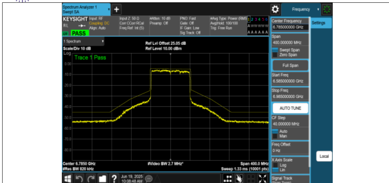
NTNV-11AX80MIMO-Ant2-6785-PASS
