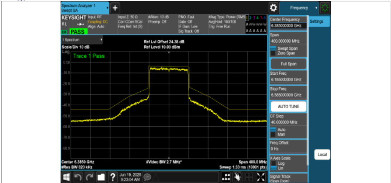
NTNV-11AX80MIMO-Ant2-6385-PASS
