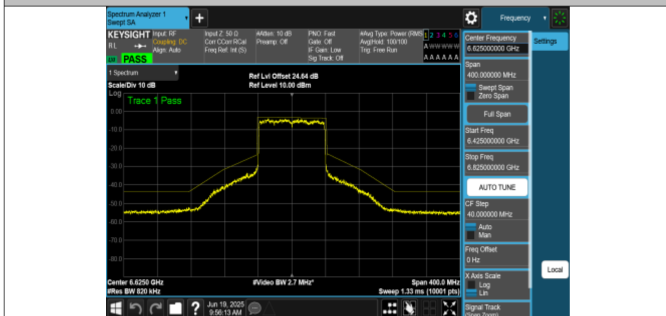
NTNV-11AX80MIMO-Ant3-6625-PASS
