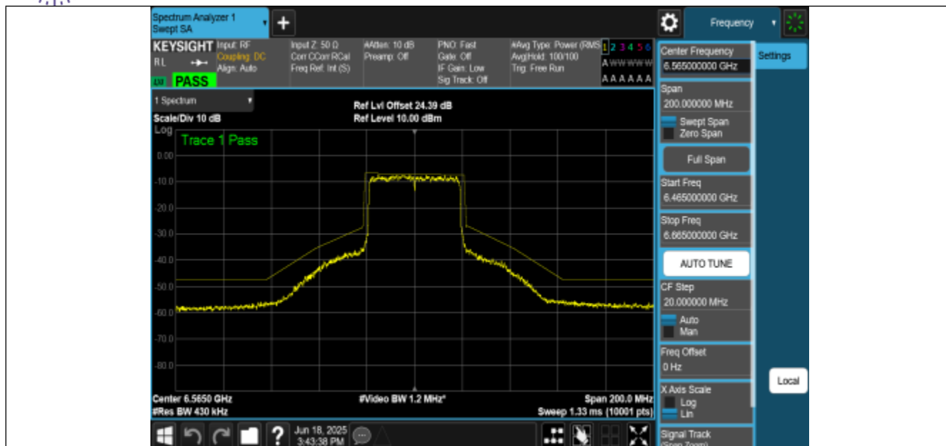
NTNV-11AX40MIMO-Ant0-6565-PASS
