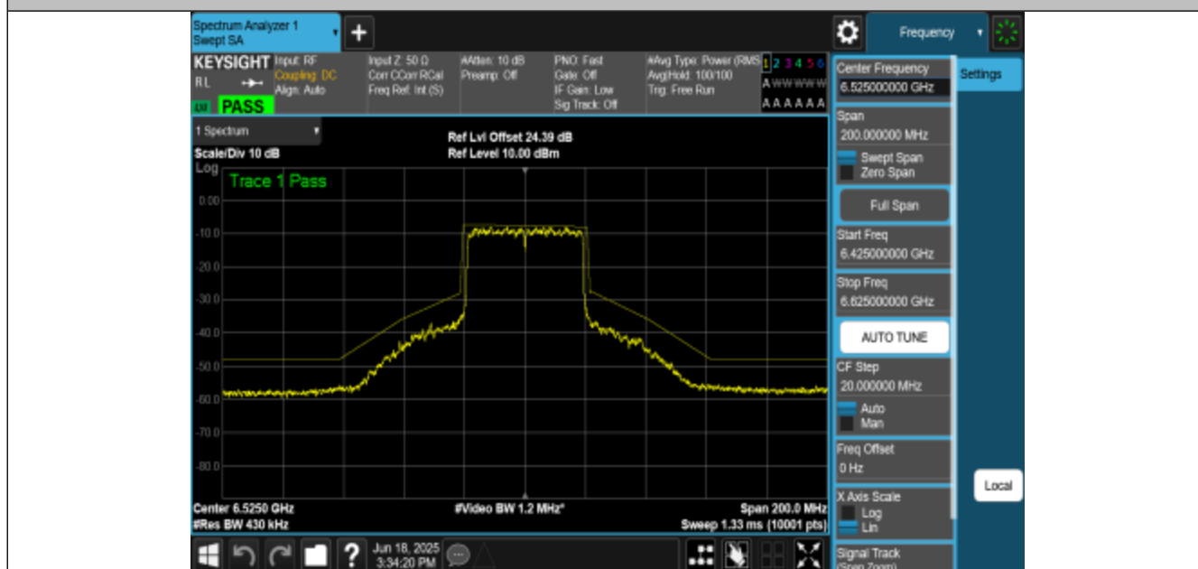
NTNV-11AX40MIMO-Ant1-6525-PASS
