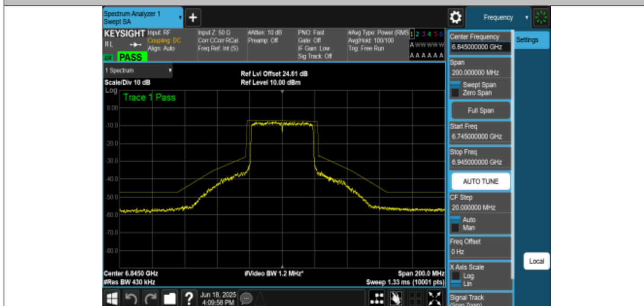
NTNV-11AX40MIMO-Ant3-6845-PASS
