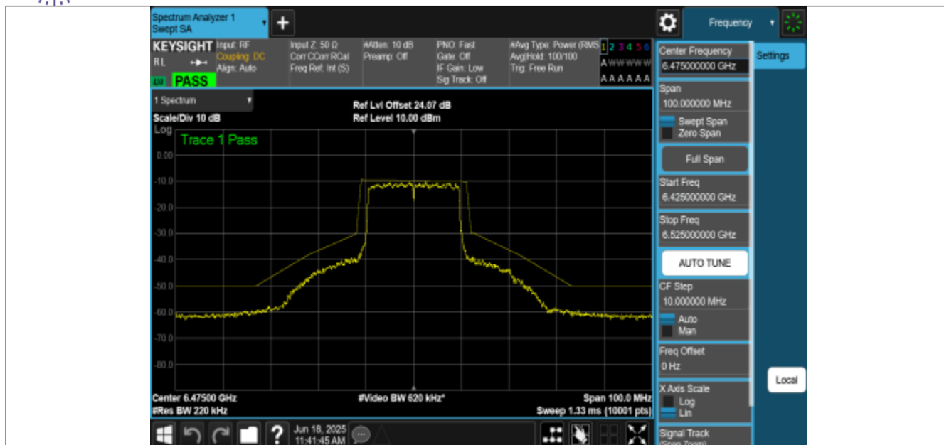
NTNV-11AX20MIMO-Ant0-6475-PASS
