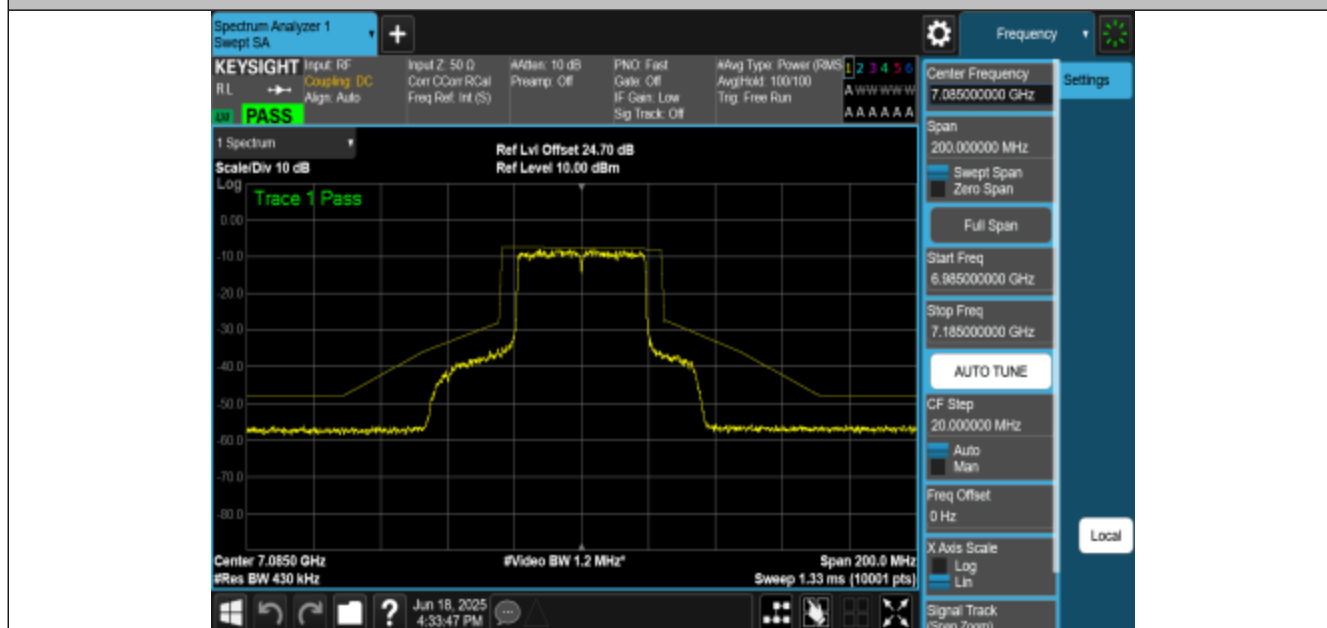
NTVN-11AX40MIMO-Ant1-7085-PASS
