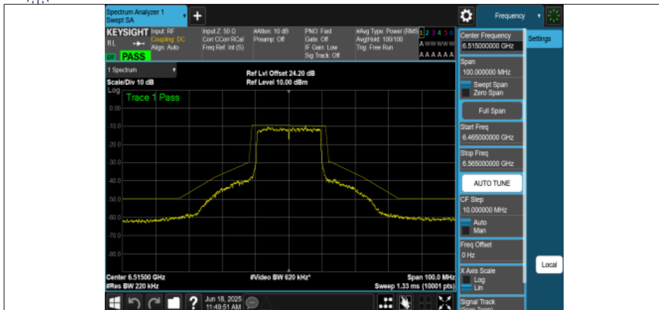
NTNV-11AX20MIMO-Ant2-6515-PASS
