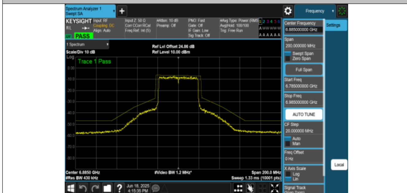
NTNV-11AX40MIMO-Ant3-6885-PASS
