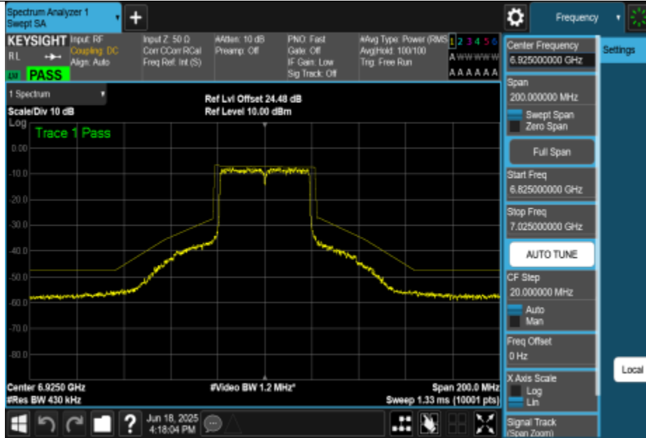
NTNV-11AX40MIMO-Ant0-6925-PASS
