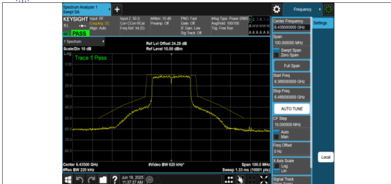
NTNV-11AX20MIMO-Ant2-6435-PASS
