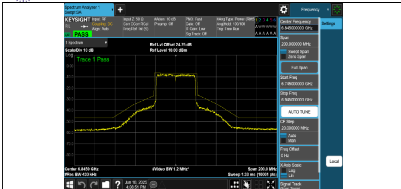
NTNV-11AX40MIMO-Ant2-6845-PASS
