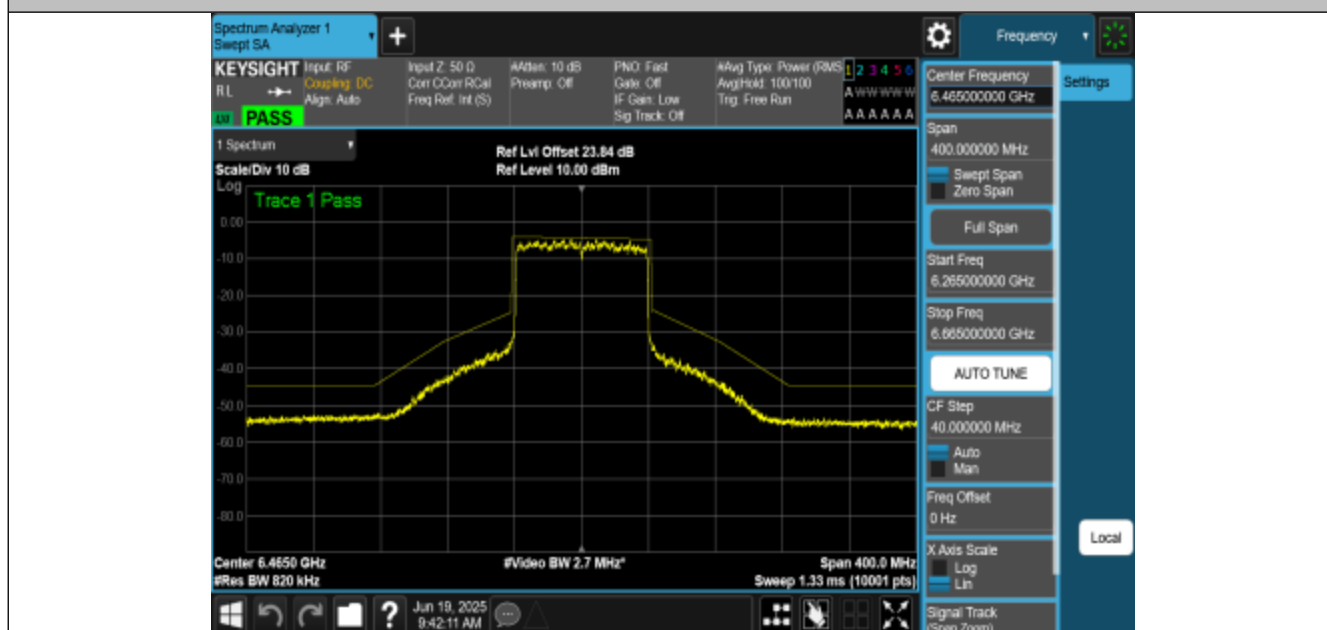
NTNV-11AX80MIMO-Ant1-6465-PASS
