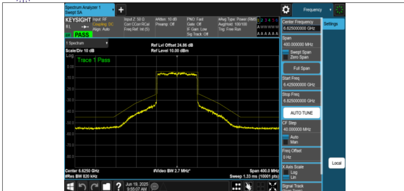
NTNV-11AX80MIMO-Ant2-6625-PASS
