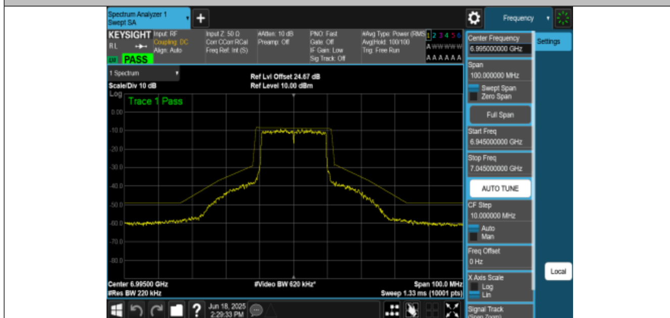
NTNV-11AX20MIMO-Ant3-6995-PASS
