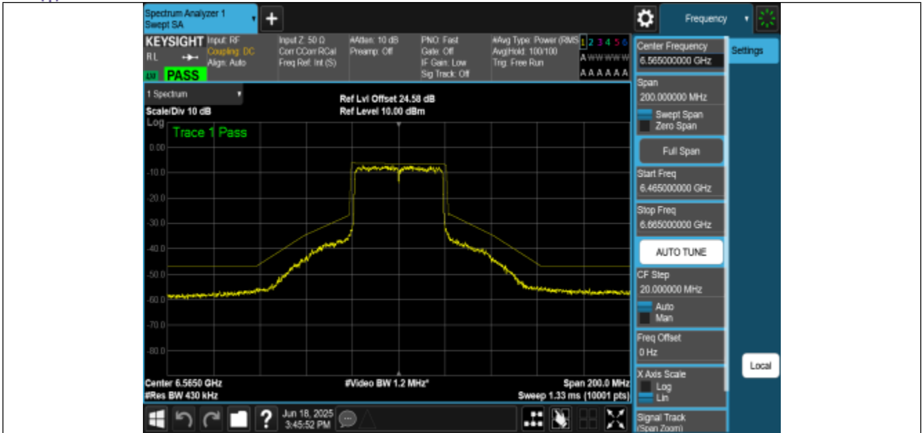
NTNV-11AX40MIMO-Ant2-6565-PASS
