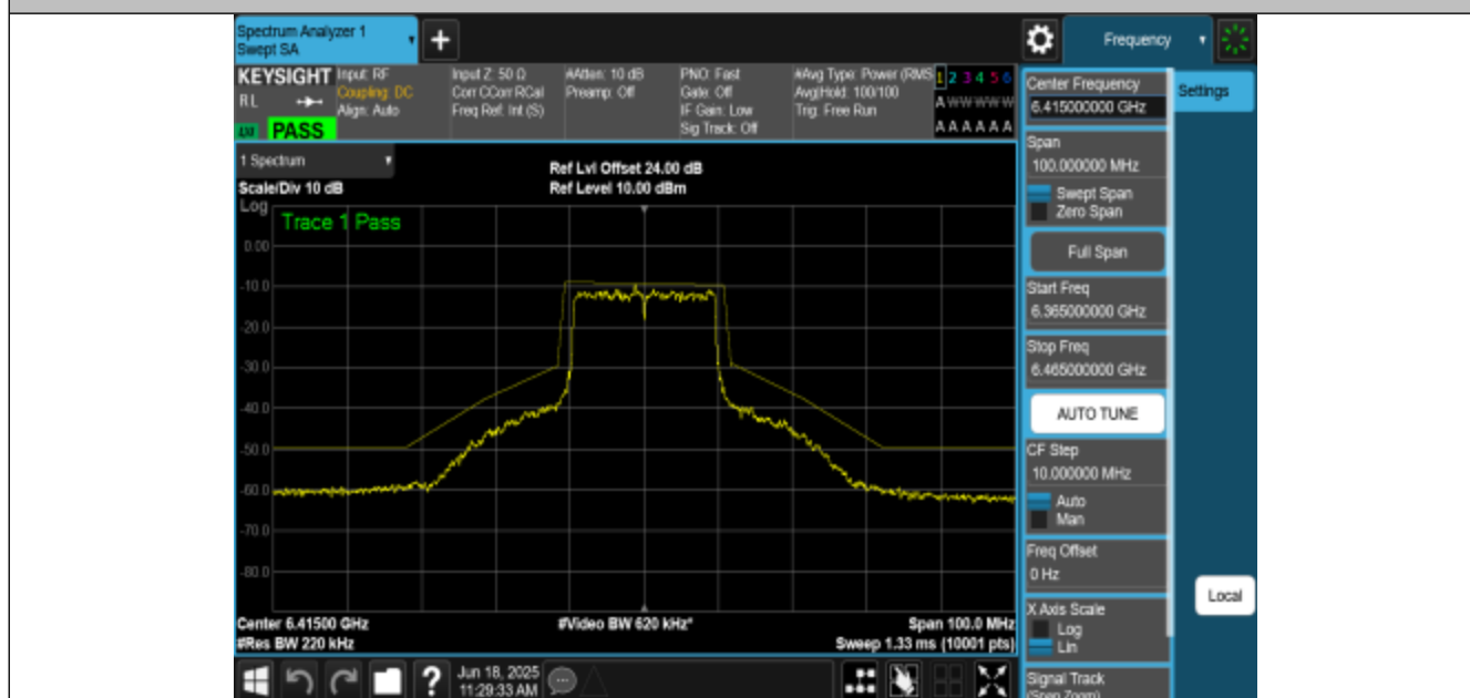
NTNV-11AX20MIMO-Ant1-6415-PASS
