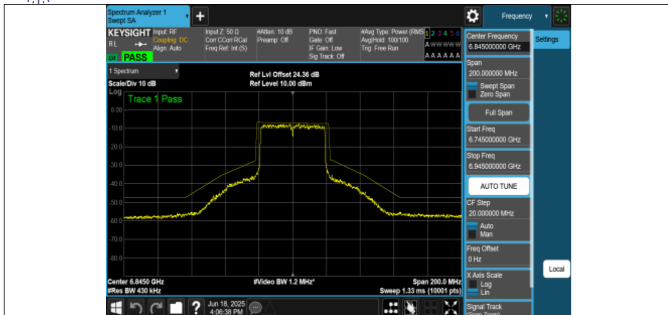
NTNV-11AX40MIMO-Ant0-6845-PASS
