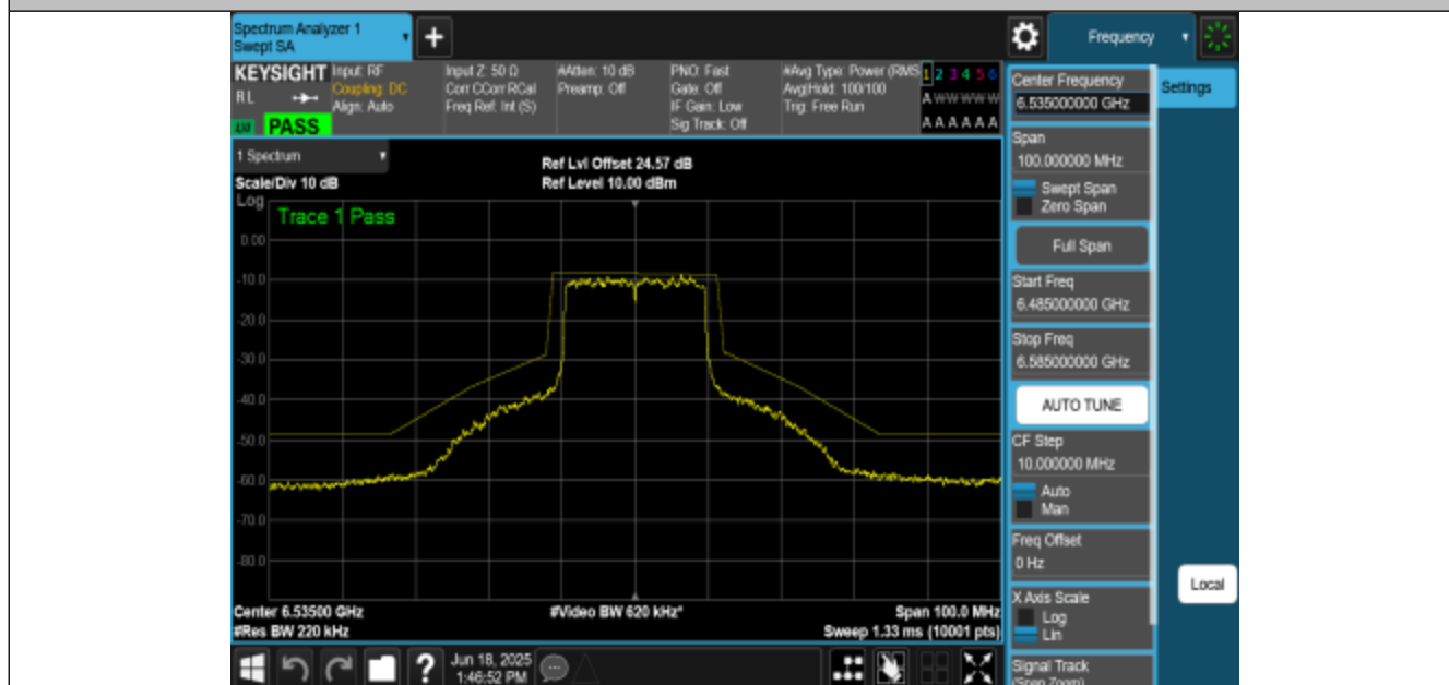
NTNV-11AX20MIMO-Ant3-6535-PASS
