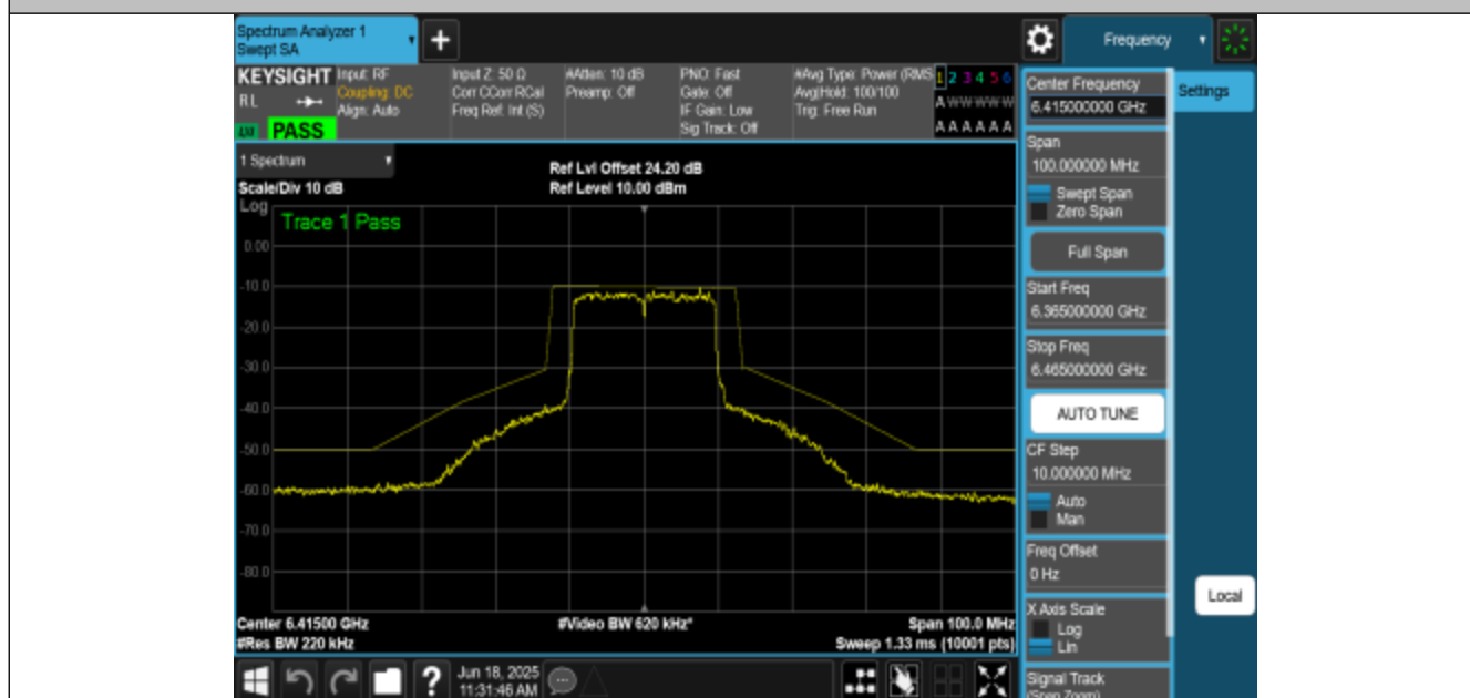
NTNV-11AX20MIMO-Ant3-6415-PASS
