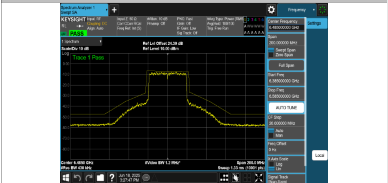
NTNV-11AX40MIMO-Ant1-6485-PASS
