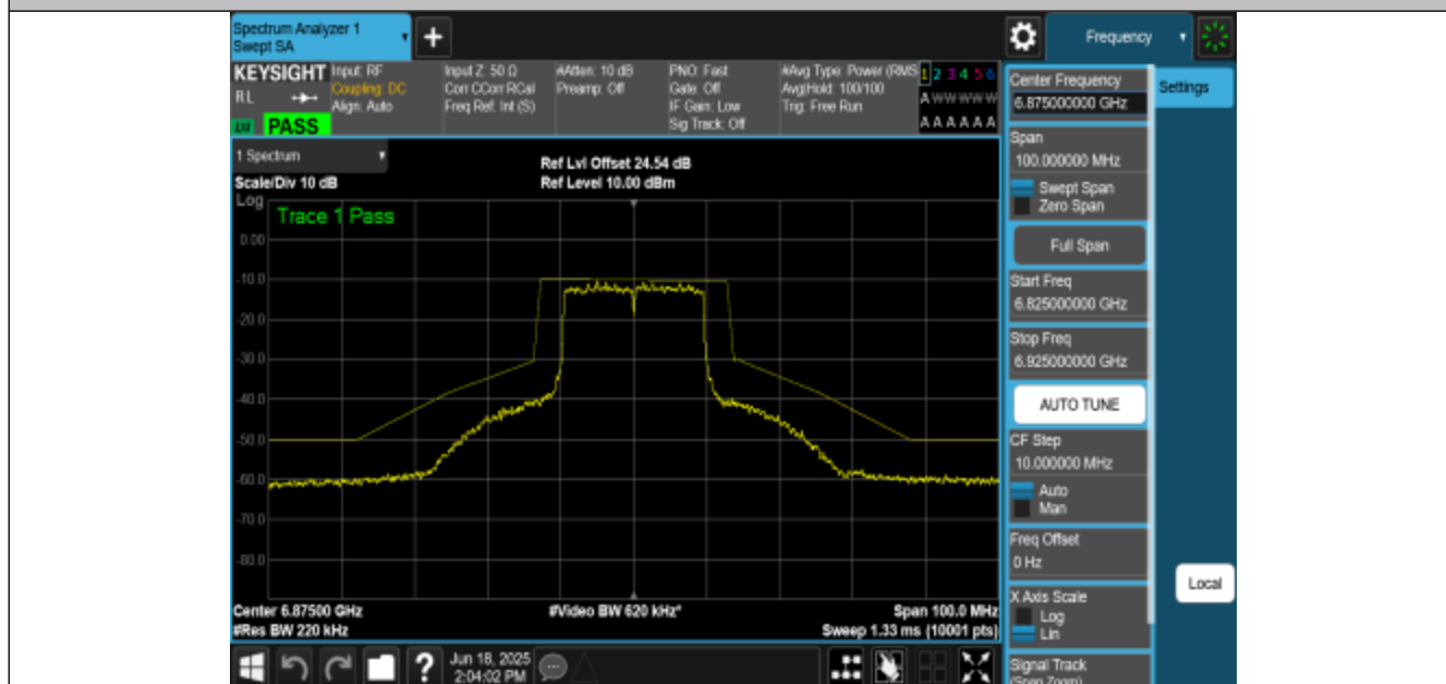
NTNV-11AX20MIMO-Ant1-6875-PASS
