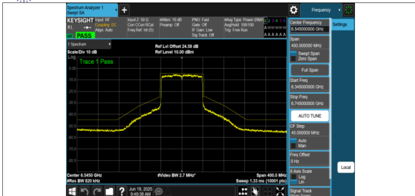
NTNV-11AX80MIMO-Ant2-6545-PASS
