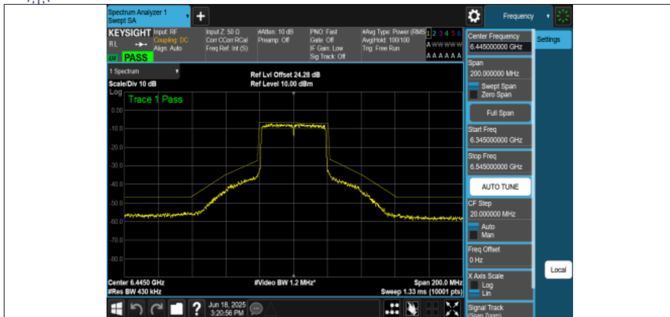
NTNV-11AX40MIMO-Ant2-6445-PASS
