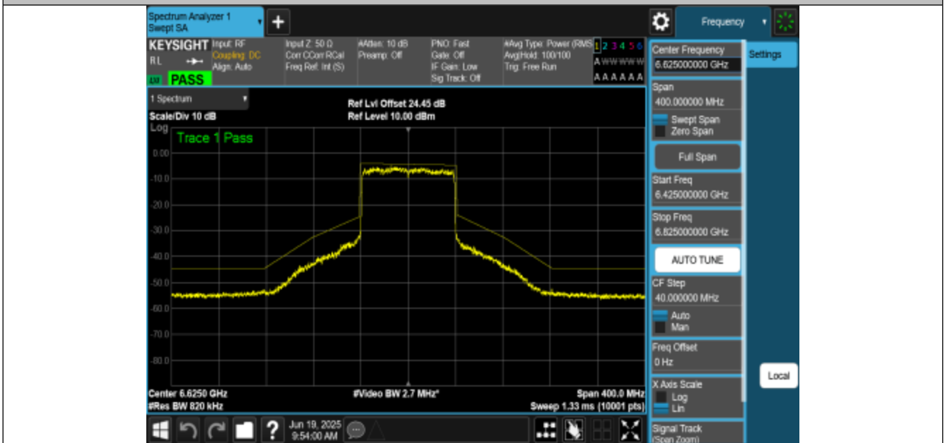
NTNV-11AX80MIMO-Ant1-6625-PASS
