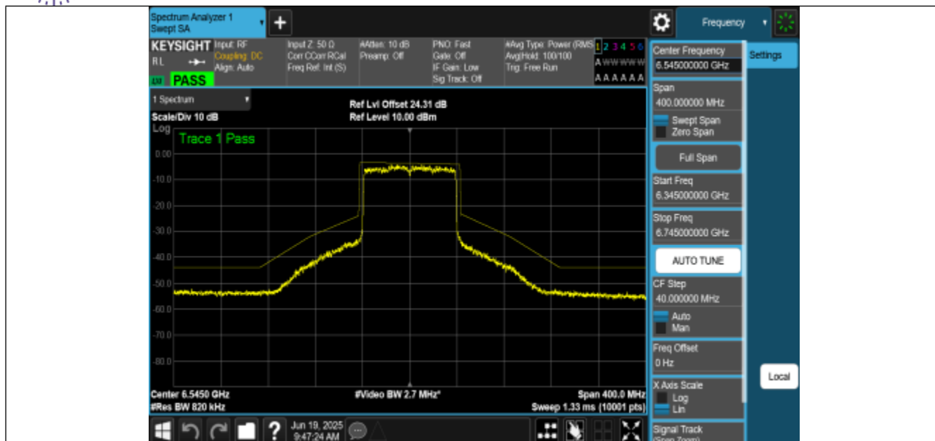
NTNV-11AX80MIMO-Ant0-6545-PASS
