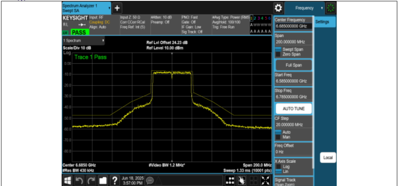
NTNV-11AX40MIMO-Ant2-6685-PASS
