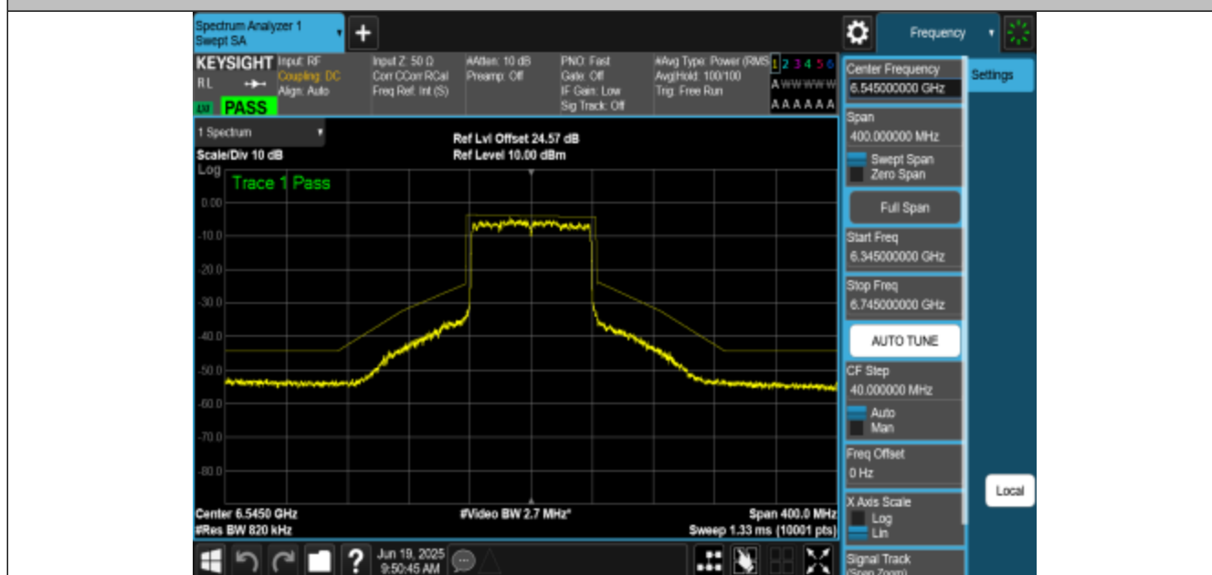
NTNV-11AX80MIMO-Ant3-6545-PASS
