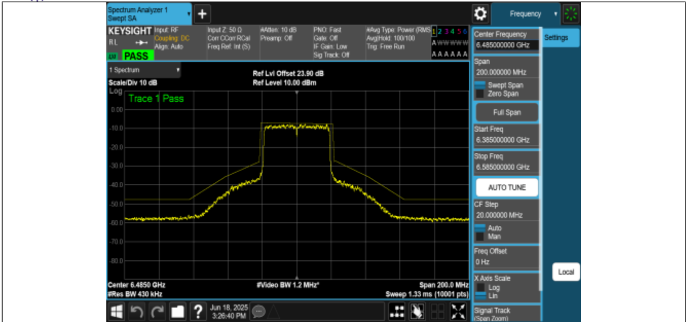
NTNV-11AX40MIMO-Ant0-6485-PASS
