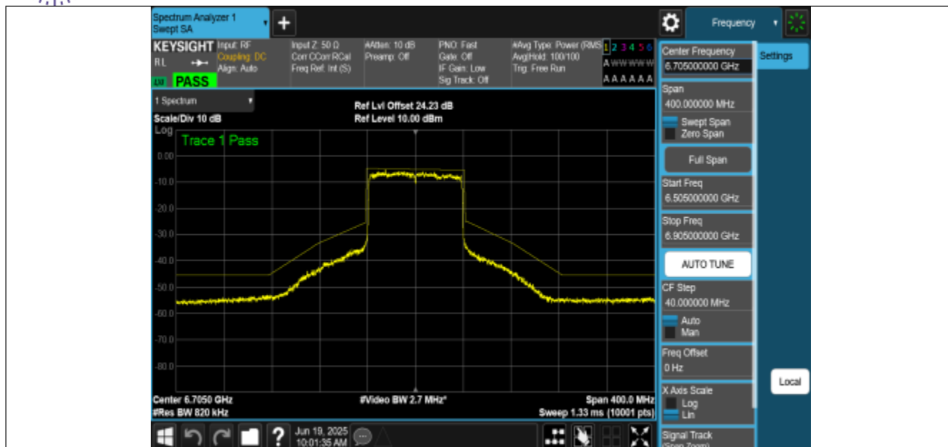
NTNV-11AX80MIMO-Ant2-6705-PASS
