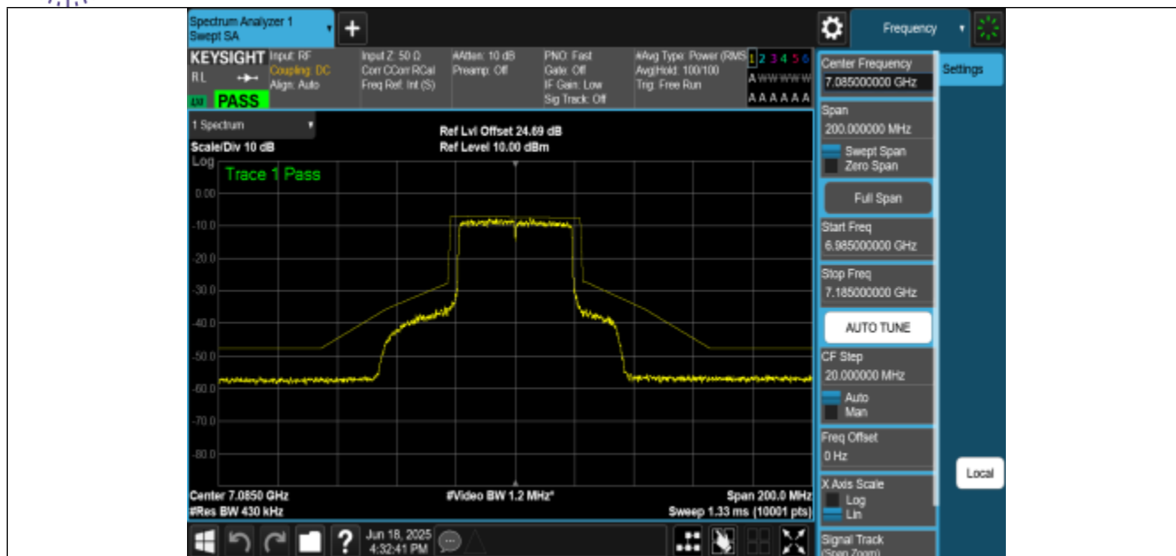
NTVN-11AX40MIMO-Ant0-7085-PASS
