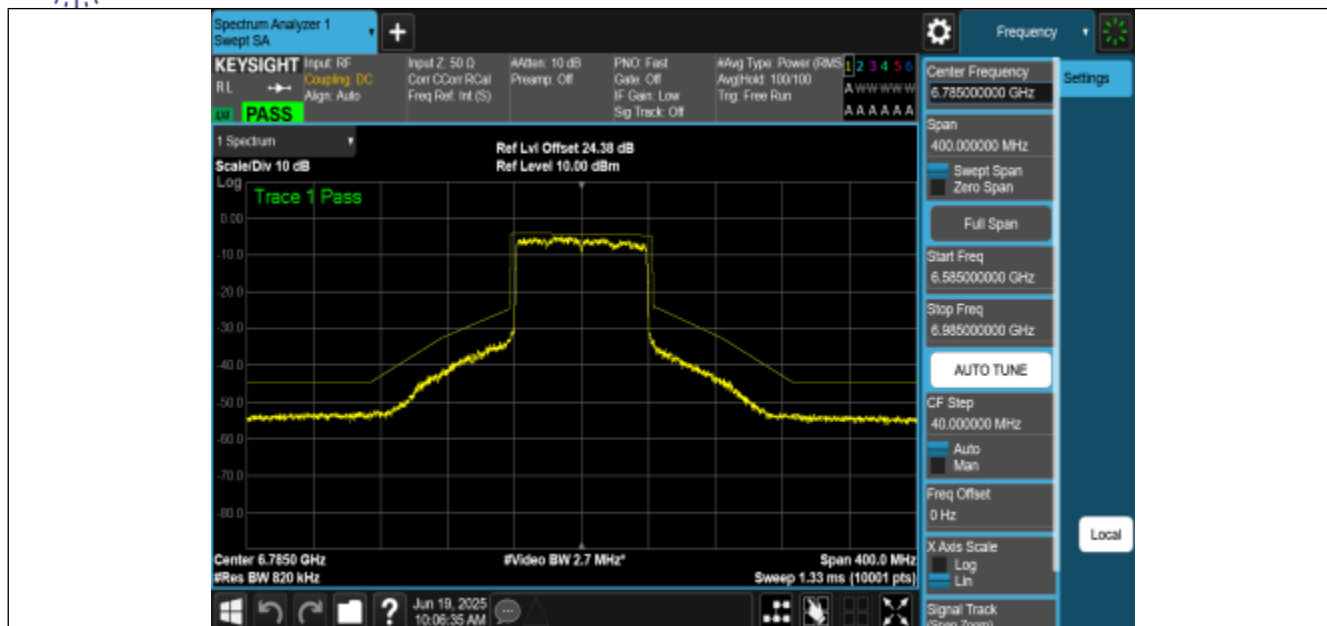
NTNV-11AX80MIMO-Ant0-6785-PASS
