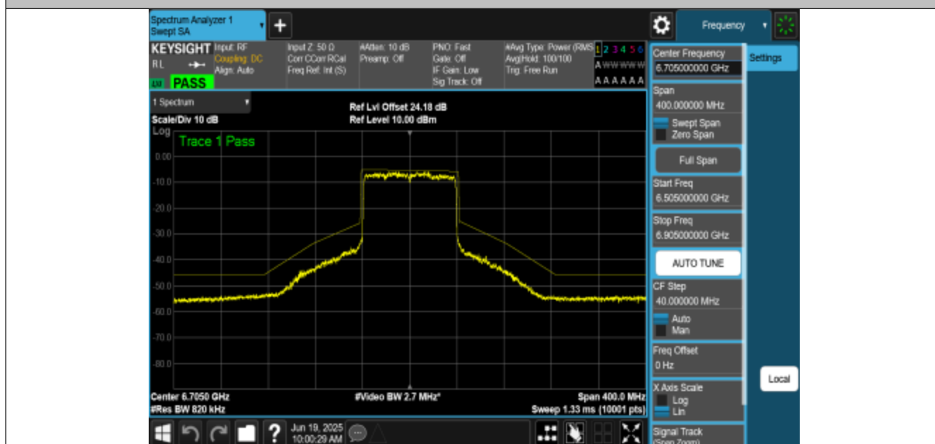
NTNV-11AX80MIMO-Ant1-6705-PASS
