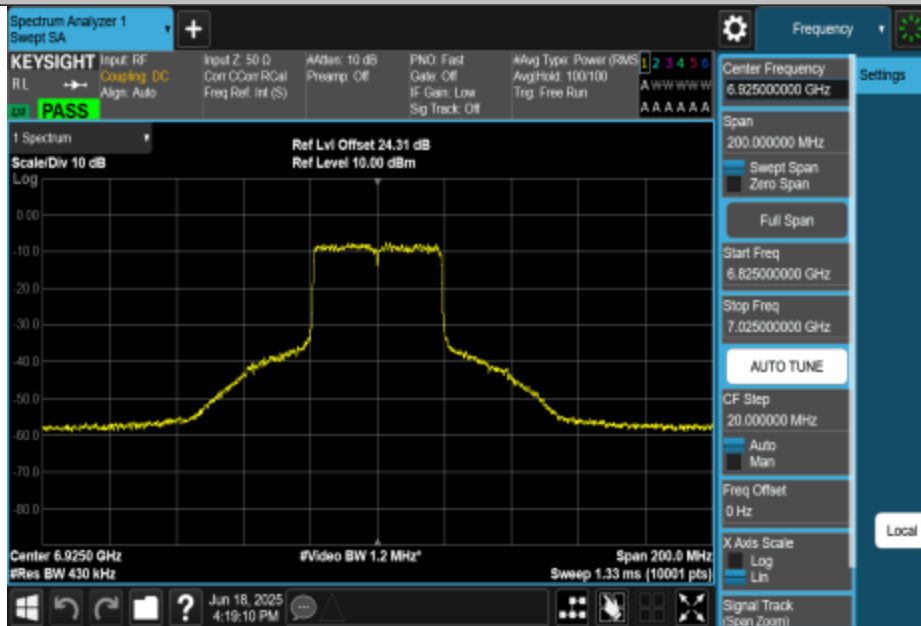
NTNV-11AX40MIMO-Ant1-6925-PASS
