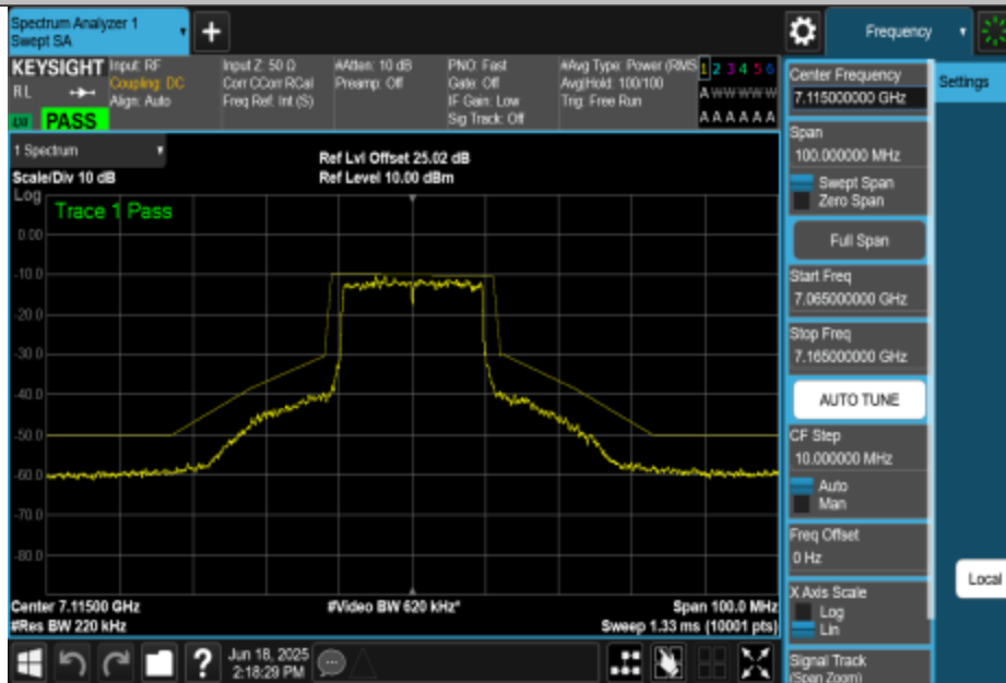
NTNV-11AX20MIMO-Ant3-7115-PASS
