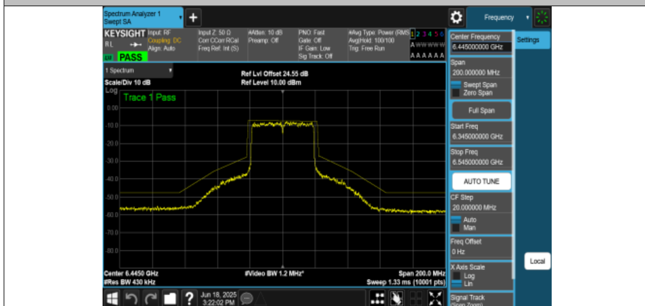
NTNV-11AX40MIMO-Ant3-6445-PASS
