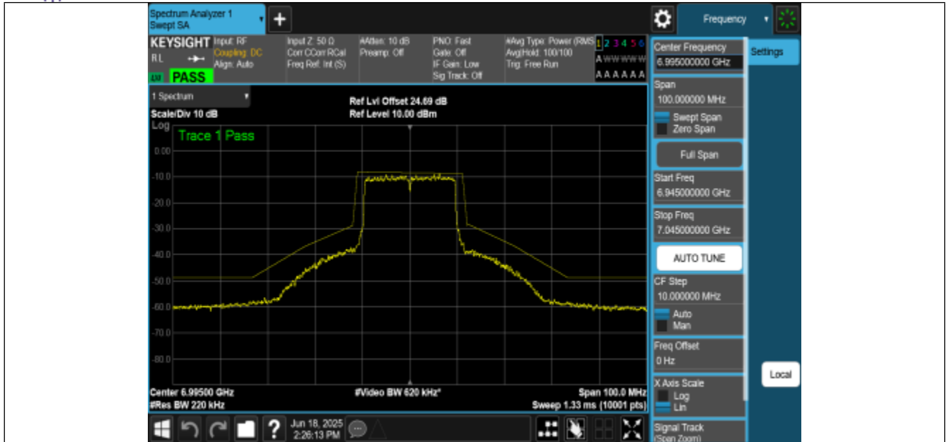
NTNV-11AX20MIMO-Ant0-6995-PASS
