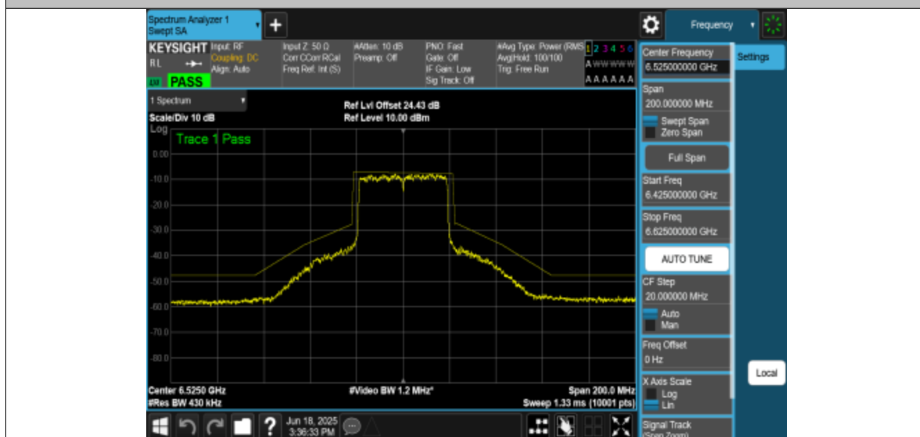
NTNV-11AX40MIMO-Ant3-6525-PASS
