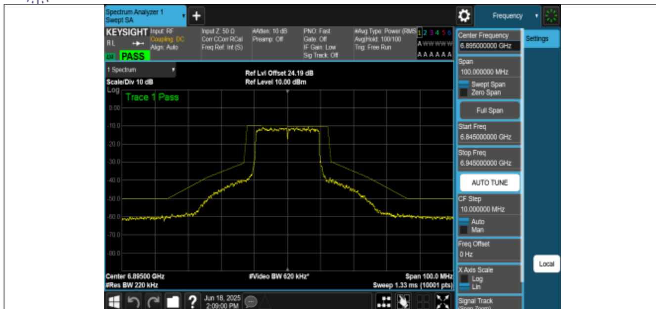
NTNV-11AX20MIMO-Ant0-6895-PASS
