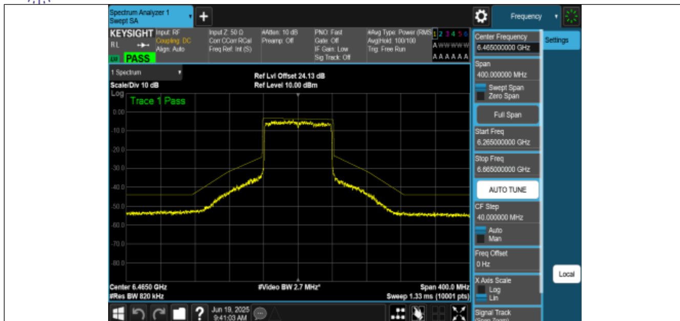
NTNV-11AX80MIMO-Ant0-6465-PASS
