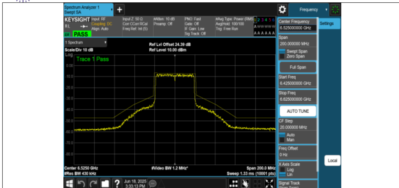
NTNV-11AX40MIMO-Ant0-6525-PASS
