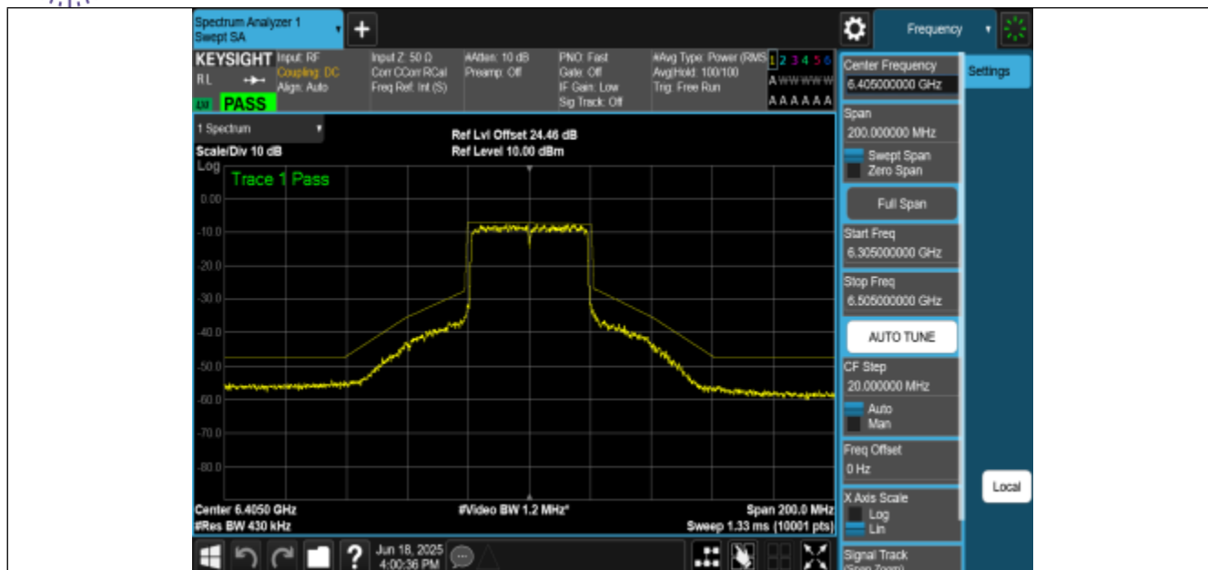
NTNV-11AX40MIMO-Ant0-6405-PASS
