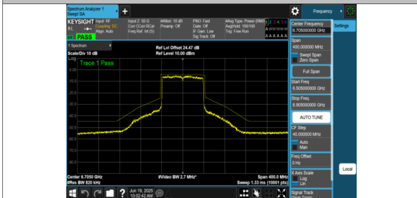
NTNV-11AX80MIMO-Ant3-6705-PASS
