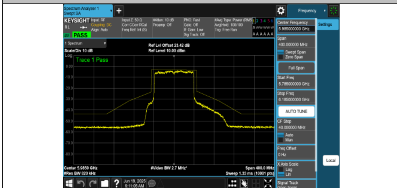
NTNV-11AX80MIMO-Ant0-5985-PASS
