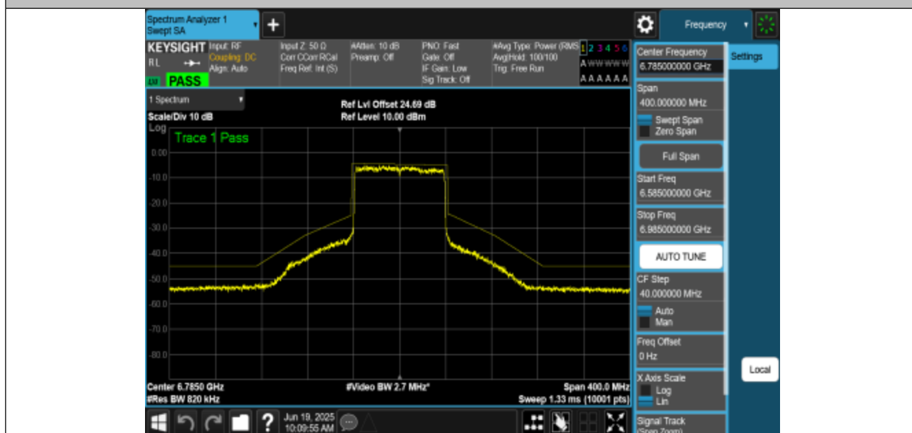
NTNV-11AX80MIMO-Ant3-6785-PASS
