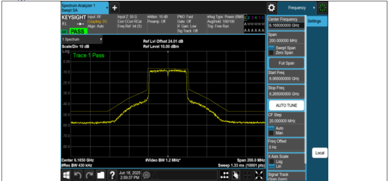
NTNV-11AX40MIMO-Ant2-6165-PASS
