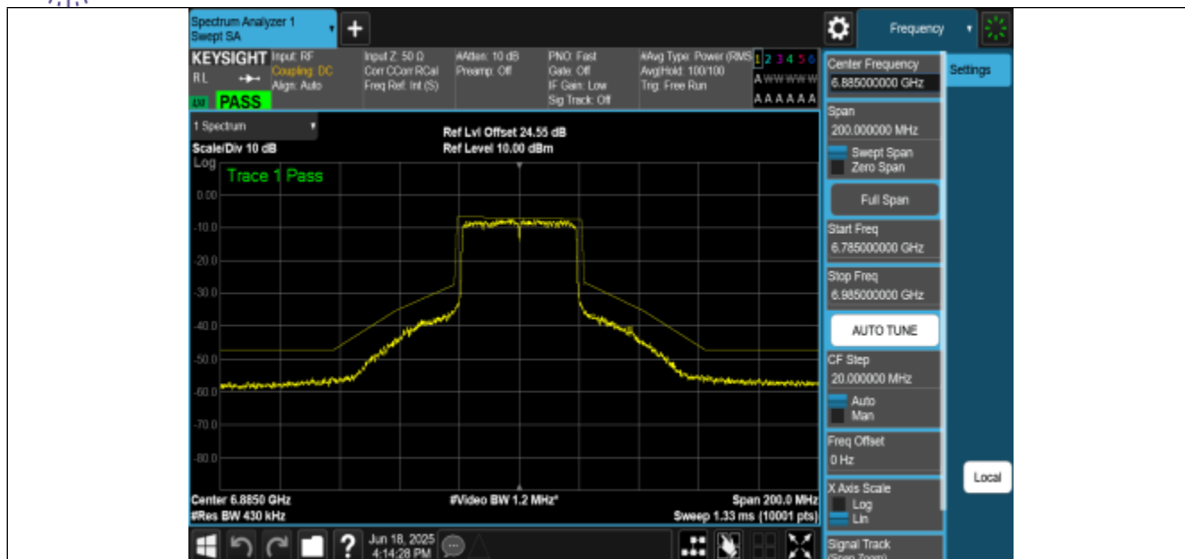
NTNV-11AX40MIMO-Ant2-6885-PASS
