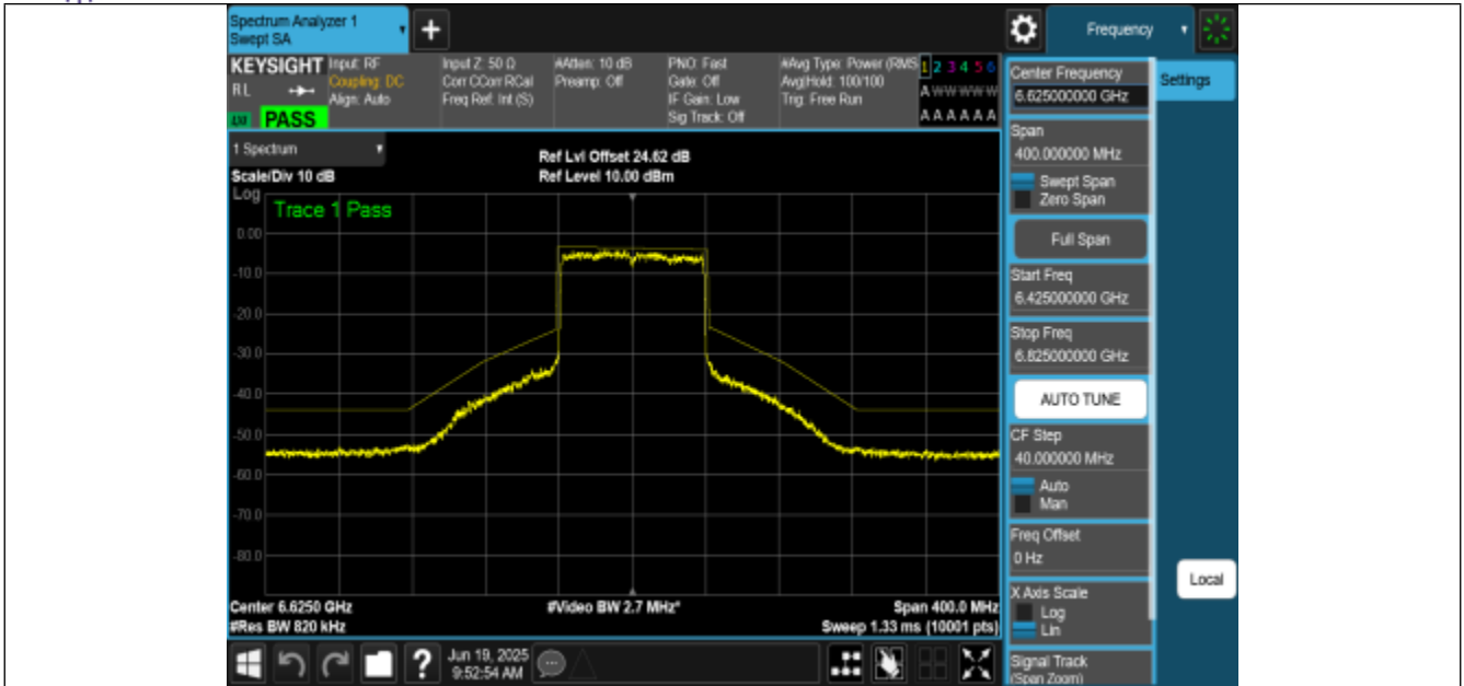
NTNV-11AX80MIMO-Ant0-6625-PASS
