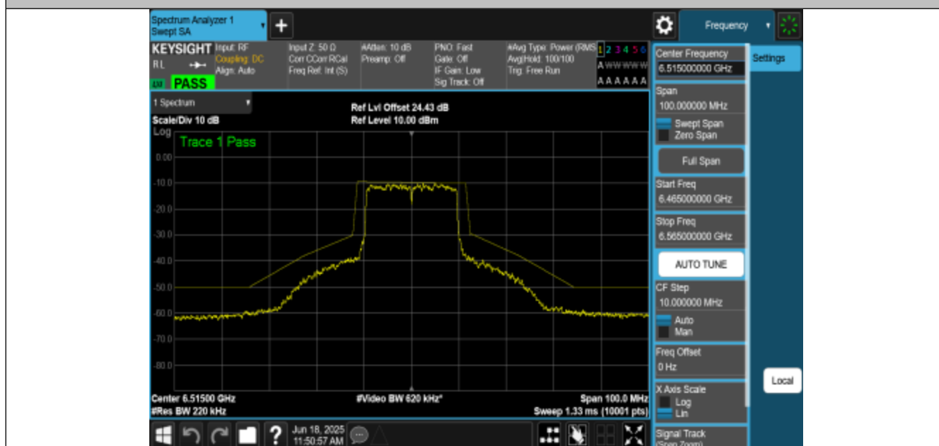
NTNV-11AX20MIMO-Ant3-6515-PASS
