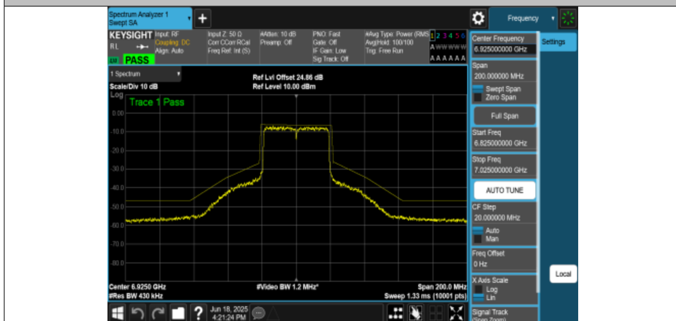
NTNV-11AX40MIMO-Ant3-6925-PASS
