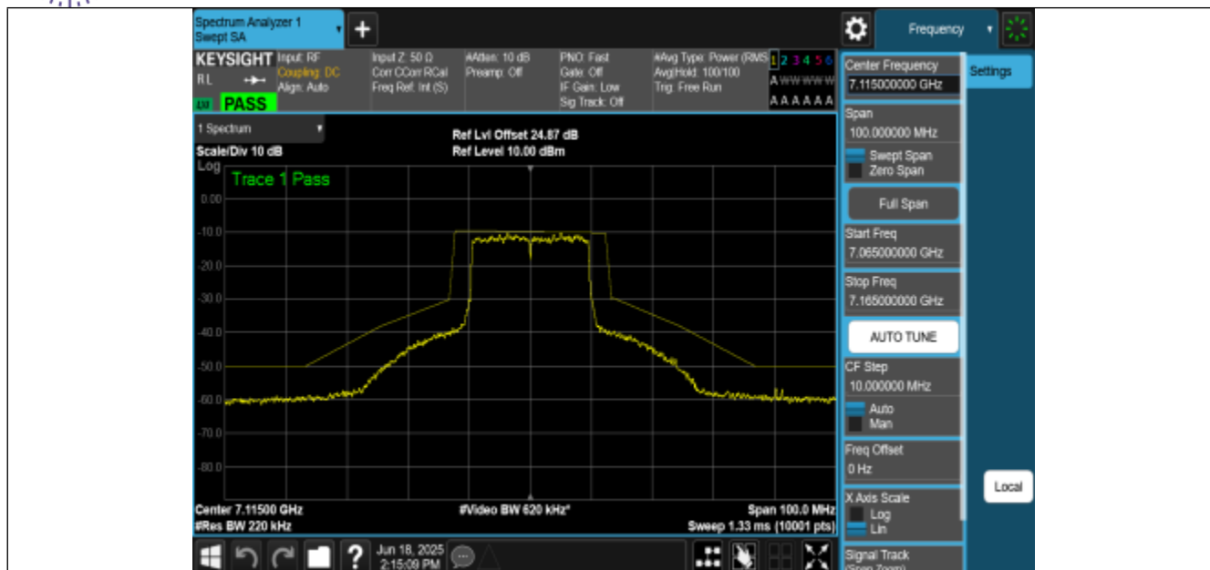
NTNV-11AX20MIMO-Ant0-7115-PASS
