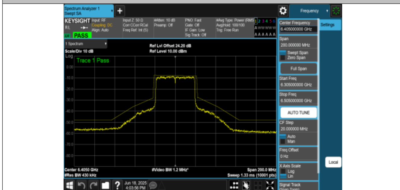
NTNV-11AX40MIMO-Ant3-6405-PASS
