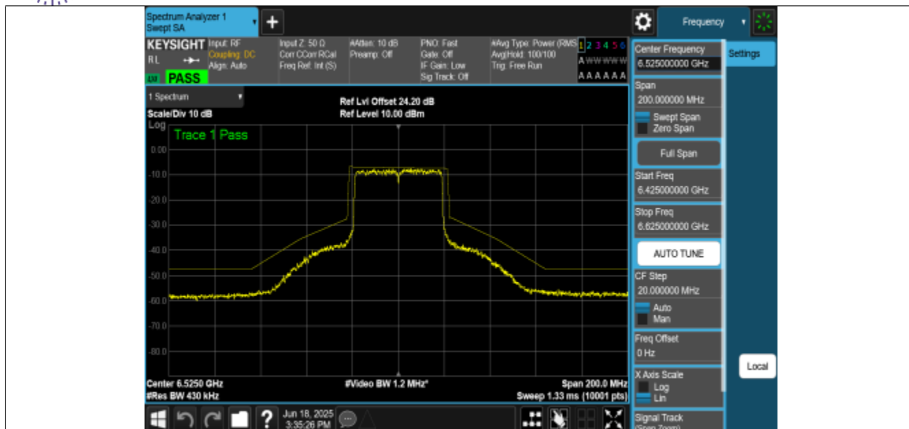
NTNV-11AX40MIMO-Ant2-6525-PASS
