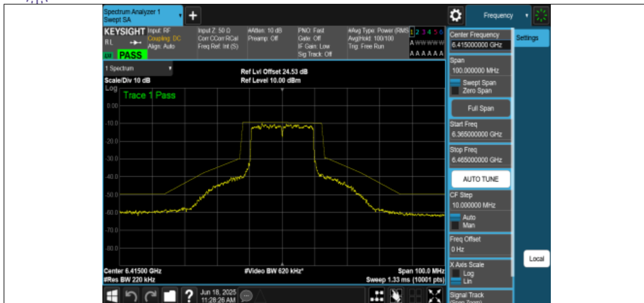
NTNV-11AX20MIMO-Ant0-6415-PASS
