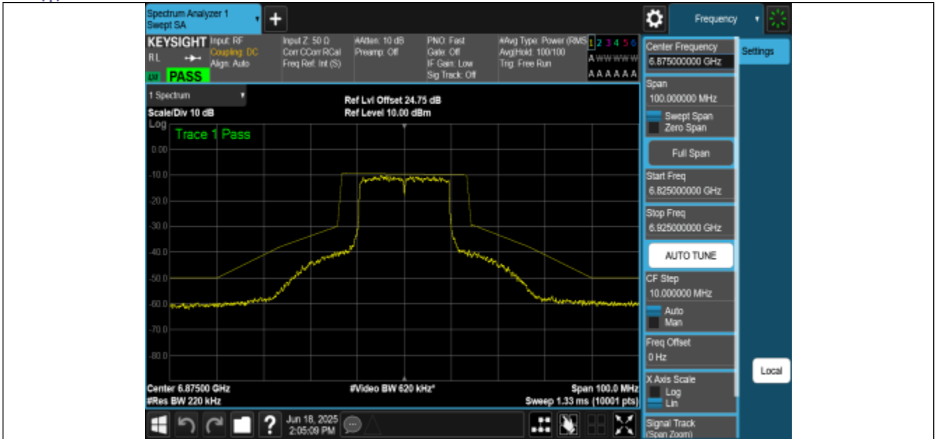
NTNV-11AX20MIMO-Ant2-6875-PASS
