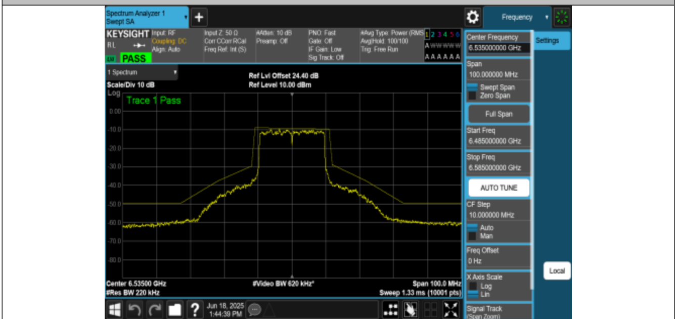
NTNV-11AX20MIMO-Ant1-6535-PASS
