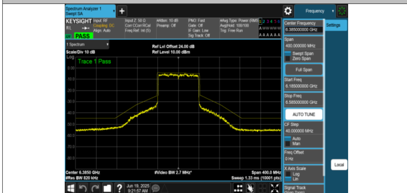
NTNV-11AX80MIMO-Ant1-6385-PASS
