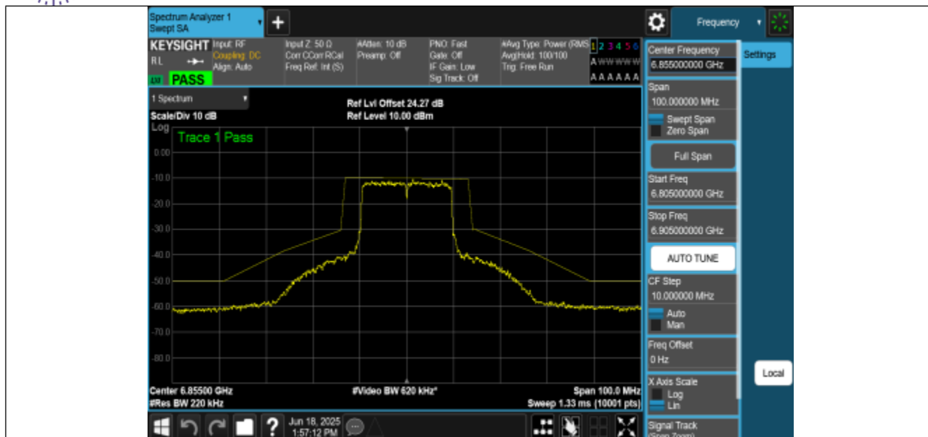
NTNV-11AX20MIMO-Ant0-6855-PASS
