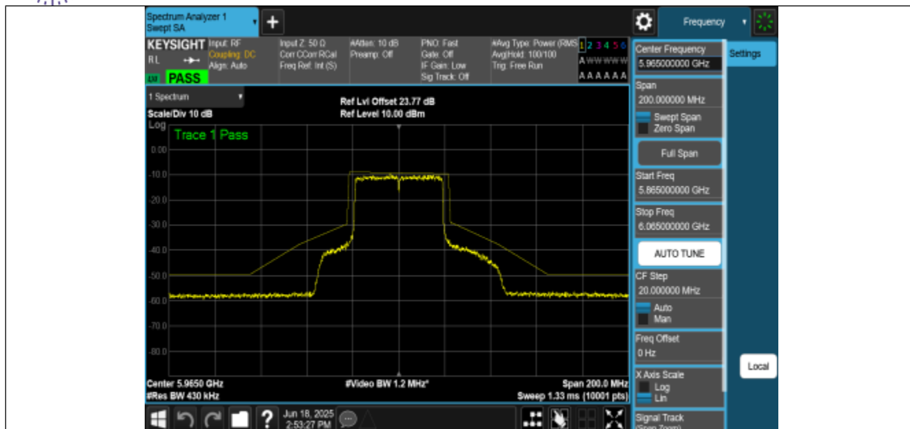
NTNV-11AX40MIMO-Ant2-5965-PASS
