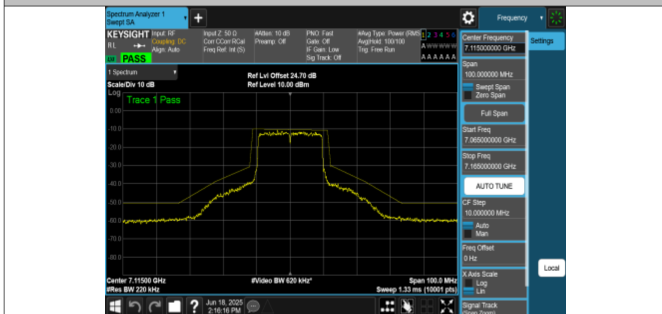
NTNV-11AX20MIMO-Ant1-7115-PASS
