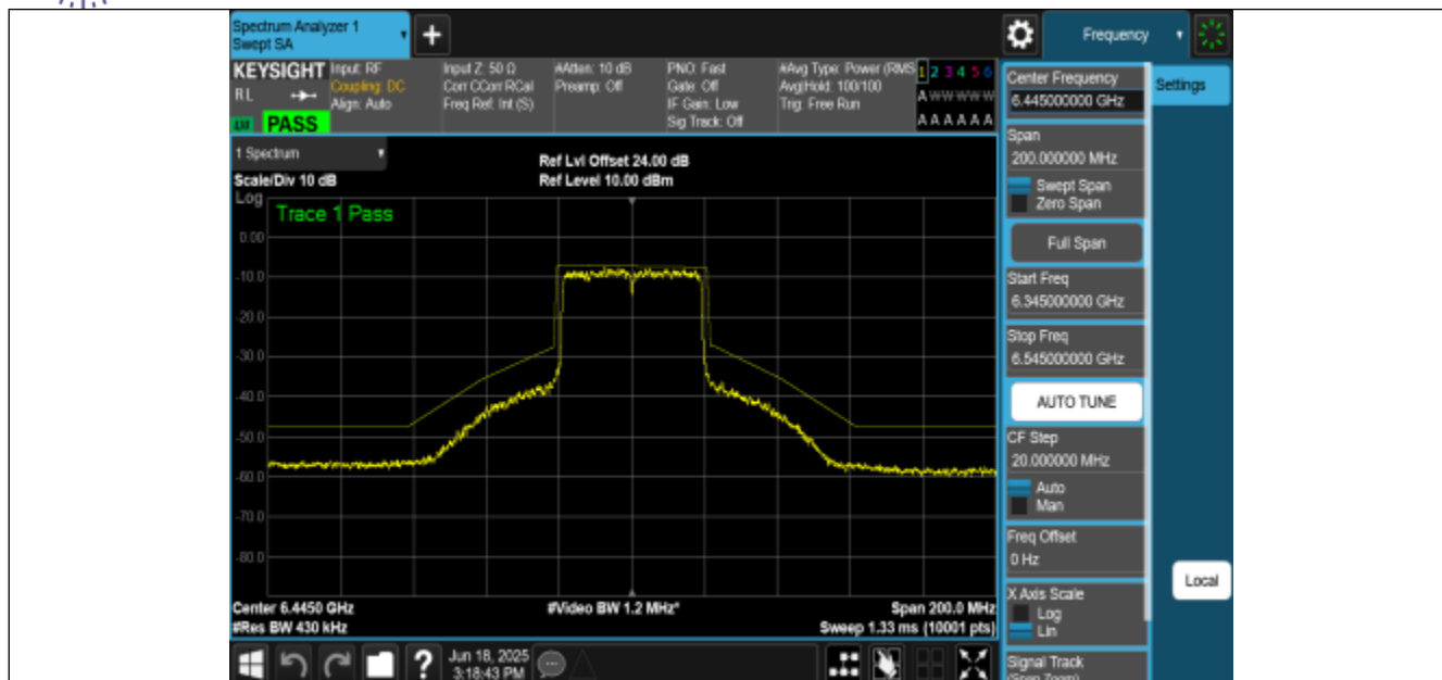
NTNV-11AX40MIMO-Ant0-6445-PASS
