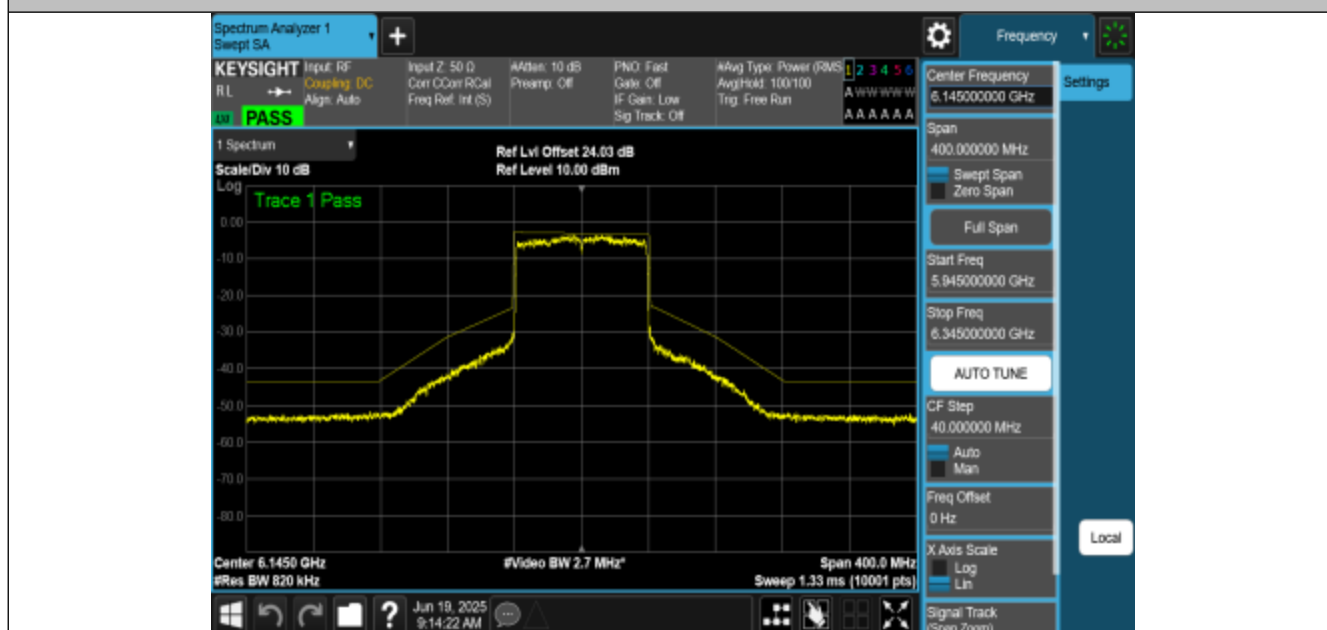
NTNV-11AX80MIMO-Ant1-6145-PASS
