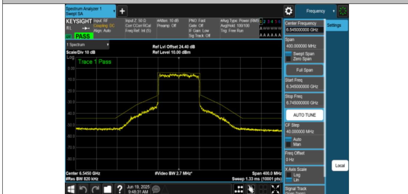
NTNV-11AX80MIMO-Ant1-6545-PASS
