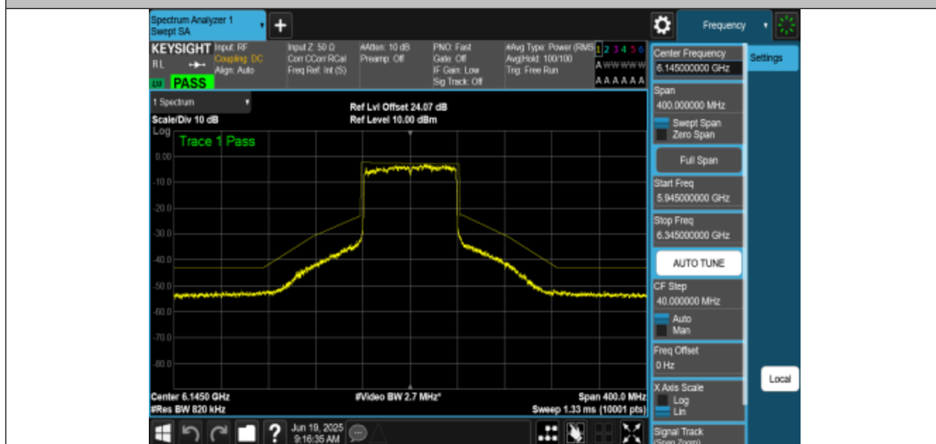
NTNV-11AX80MIMO-Ant3-6145-PASS
