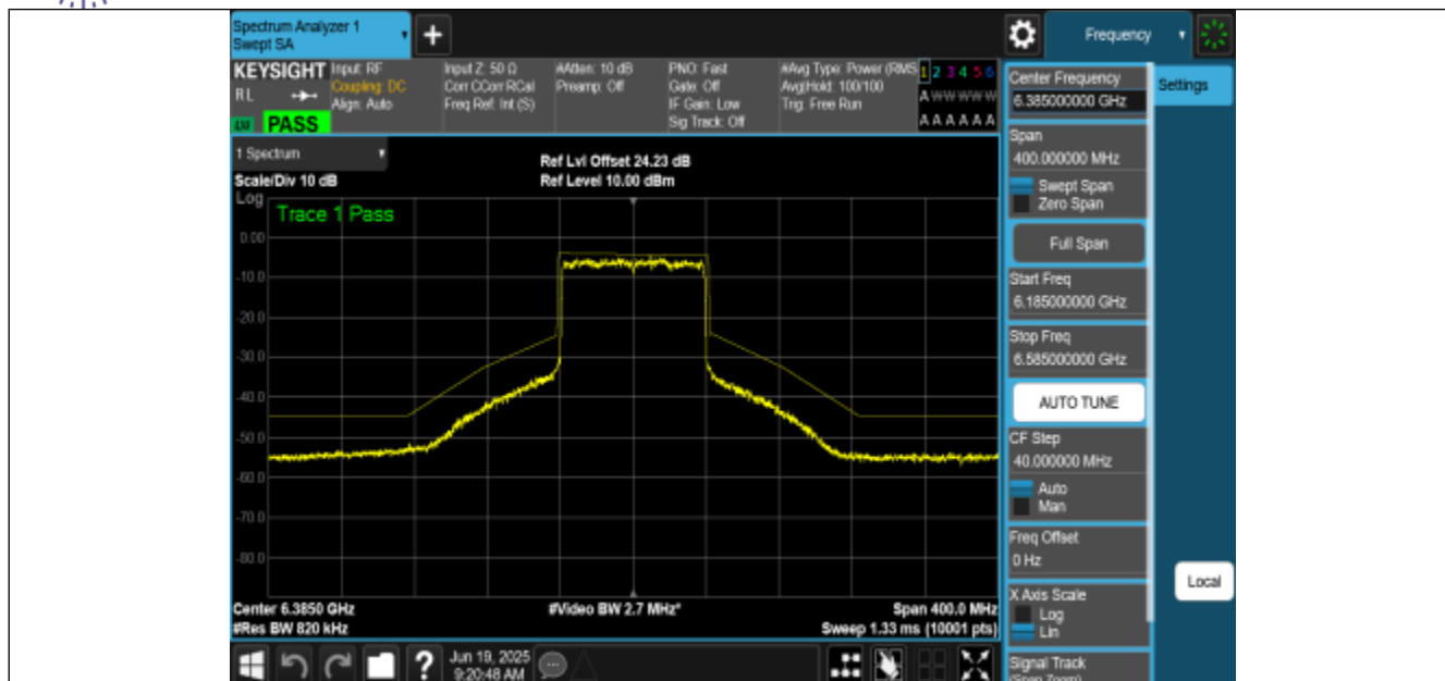
NTNV-11AX80MIMO-Ant0-6385-PASS
