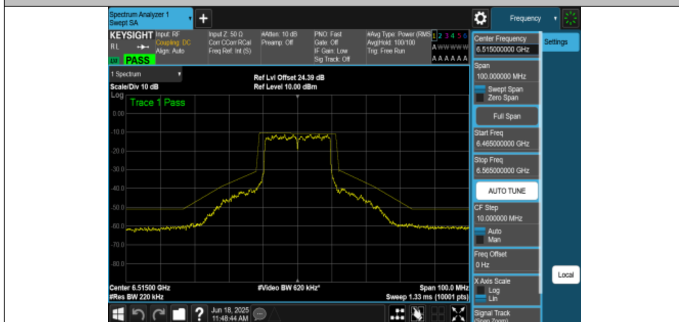
NTNV-11AX20MIMO-Ant1-6515-PASS
