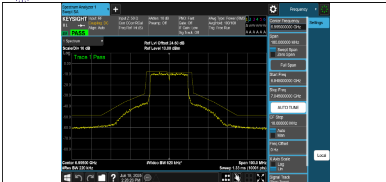
NTNV-11AX20MIMO-Ant2-6995-PASS
