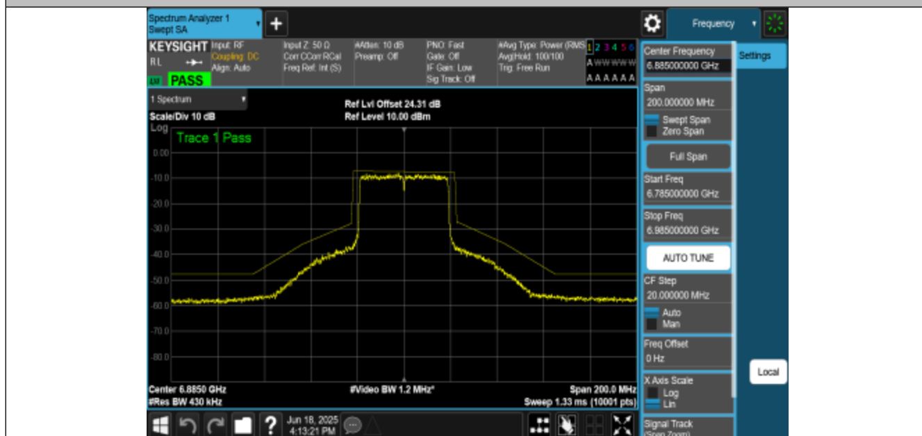
NTNV-11AX40MIMO-Ant1-6885-PASS
