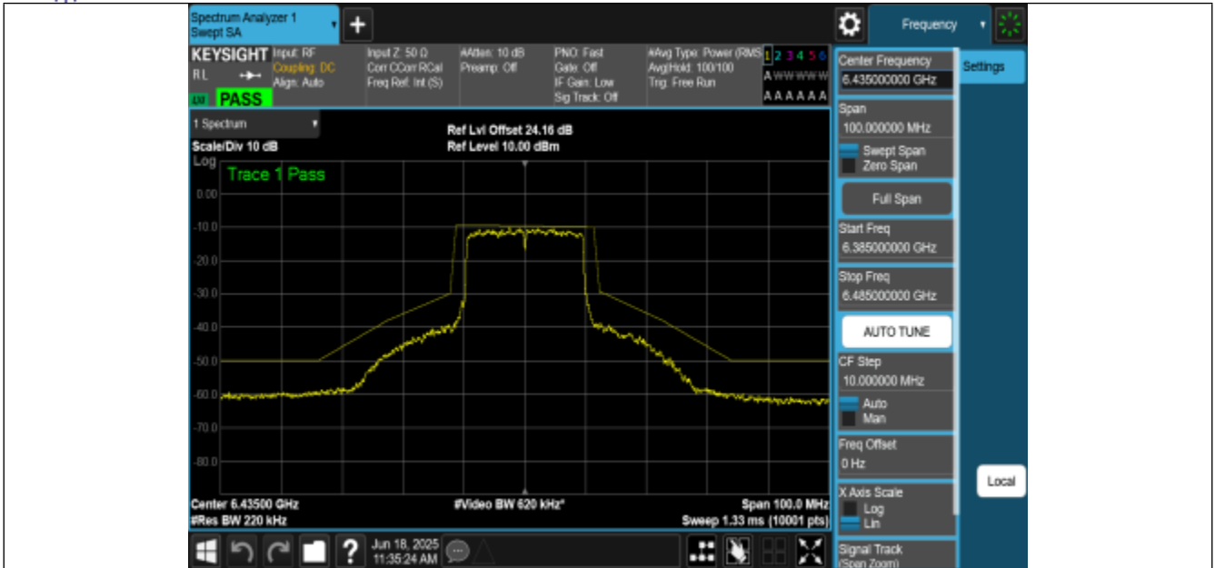
NTN-11AX20MIMO-Ant0-6435-PASS
