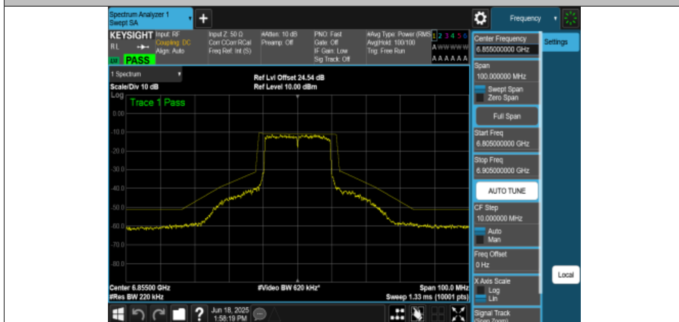
NTNV-11AX20MIMO-Ant1-6855-PASS
