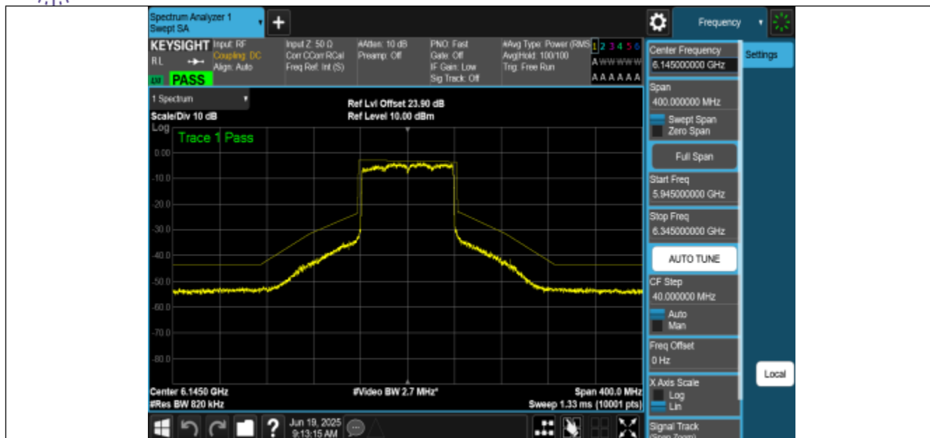
NTNV-11AX80MIMO-Ant0-6145-PASS
