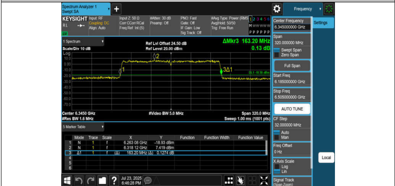
11BE160MIMO-Ant2-6345
