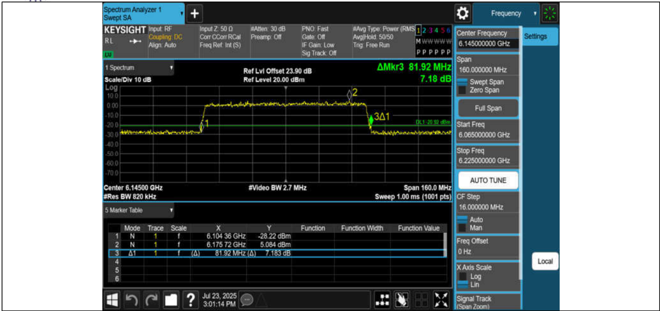
11BE80MIMO-Ant1-6145
