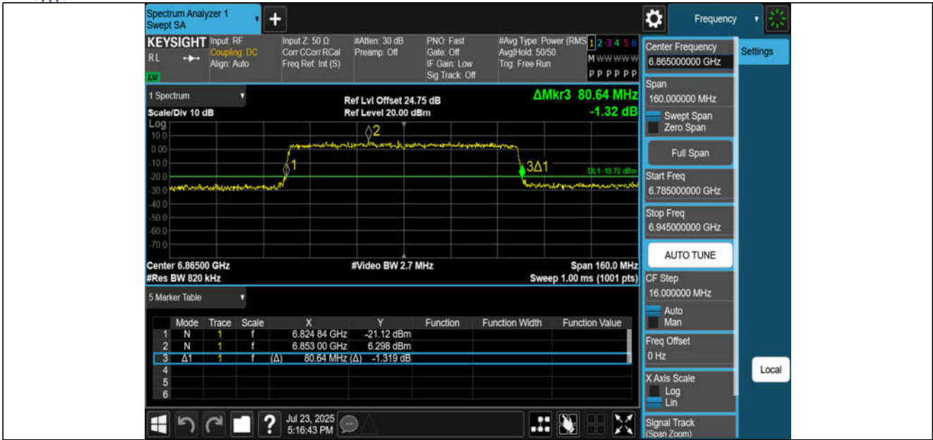
11BE80MIMO-Ant3-6865
