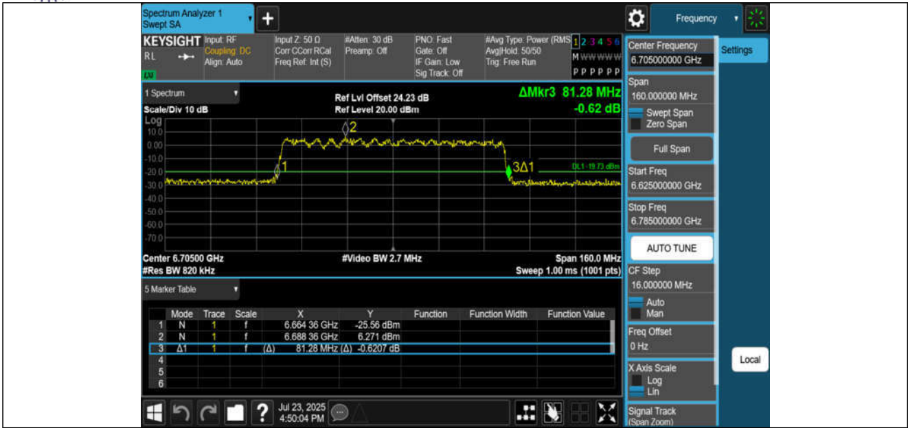
11BE80MIMO-Ant3-6705
