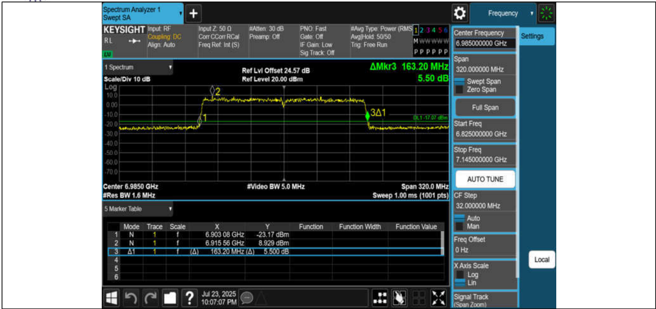
11BE160MIMO-Ant1-6985
