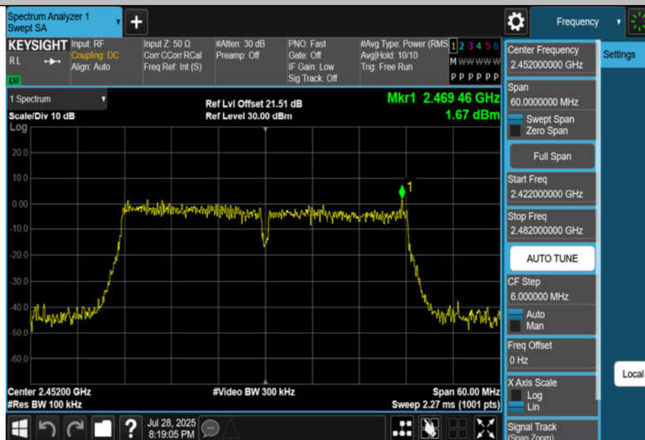
11N40MIMO-Ant2-2452-0-Reference-PASS
