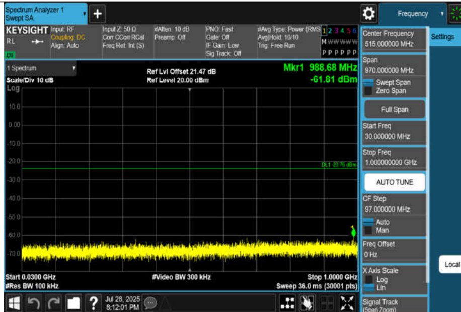
11N20MIMO-Ant1-2462-30~1000-PASS
