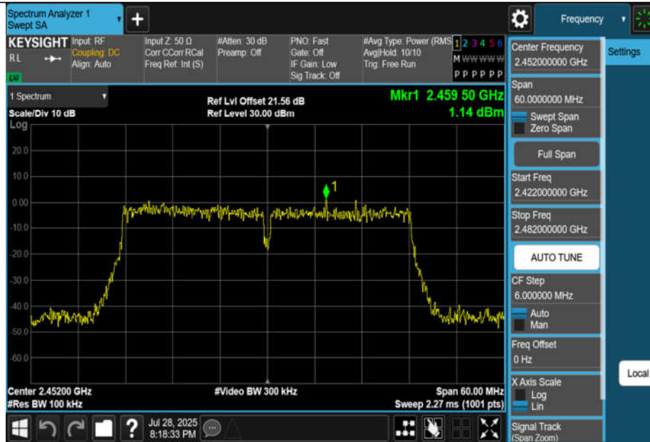
11N40MIMO-Ant1-2452-0-Reference-PASS
