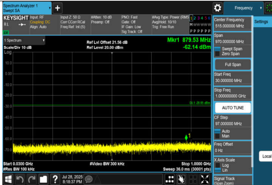
11N40MIMO-Ant1-2452-30~1000-PASS
