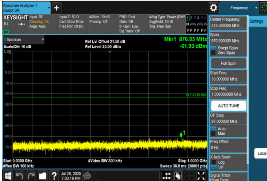
11AX20MIMO-Ant1-2412-30~1000-PASS
