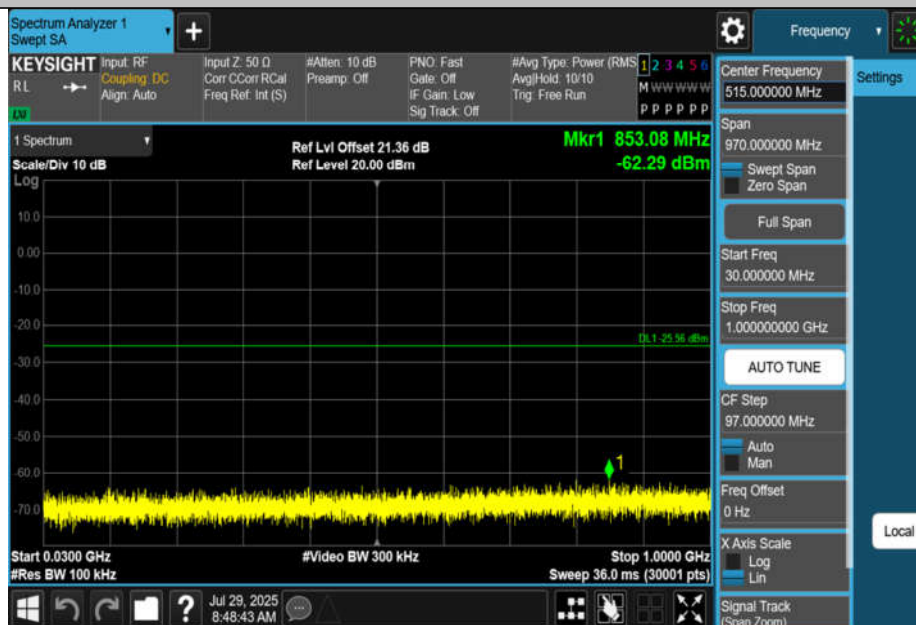
11BE20MIMO-Ant2-2412-30~1000-PASS
