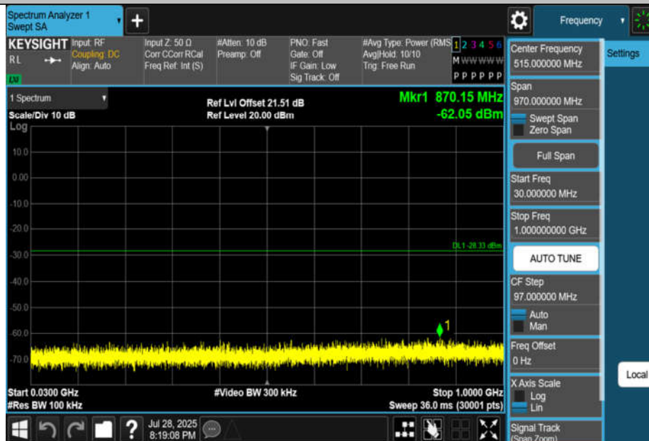
11N40MIMO-Ant2-2452-30~1000-PASS
