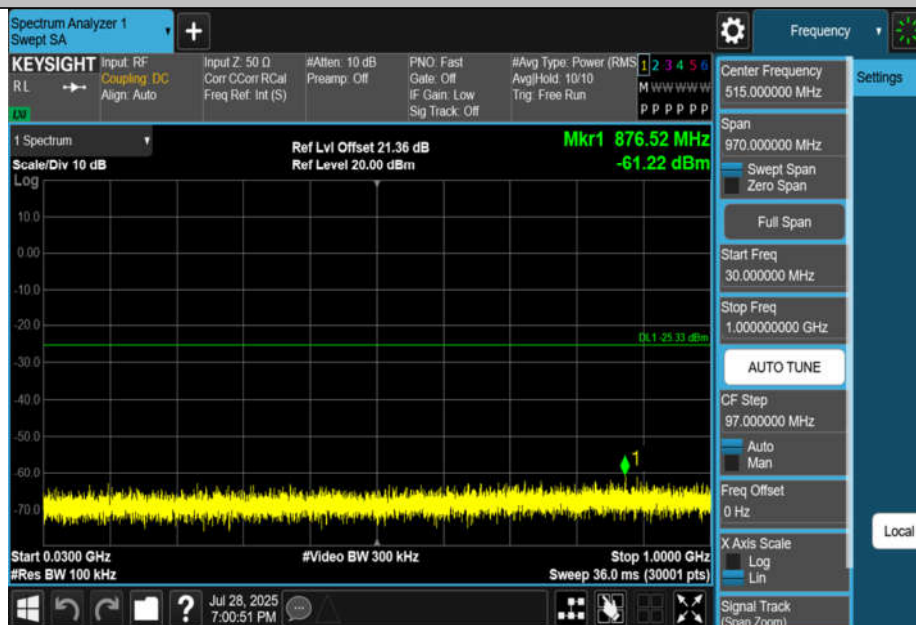
11AX20MIMO-Ant2-2412-30~1000-PASS
