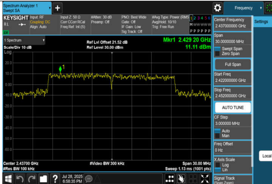
11AX20MIMO-Ant1-2437-0~Reference-PASS
