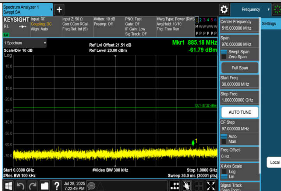
11AX40MIMO-Ant2-2452-30~1000-PASS
