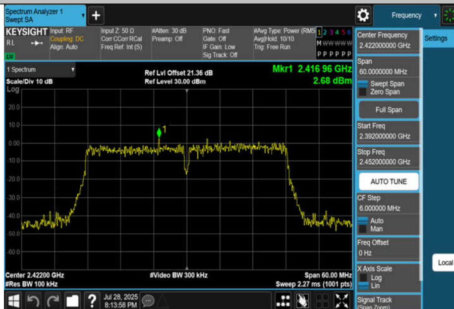
11N40MIMO-Ant2-2422-0~Reference-PASS
