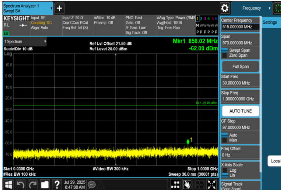
11BE20MIMO-Ant1-2412-30~1000-PASS
