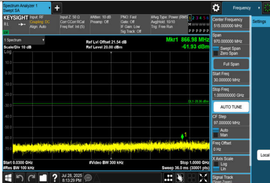
11N40MIMO-Ant1-2422-30~1000-PASS
