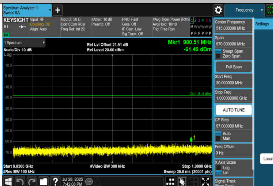
11AX40MIMO-Ant2-2437-30~1000-PASS
