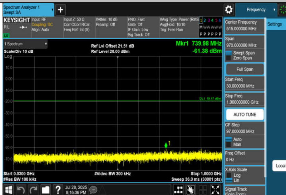
11N40MIMO-Ant2-2437-30~1000-PASS
