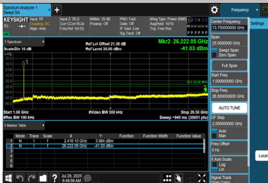
11BE20MIMO-Ant2-2412-1000~26500-PASS
