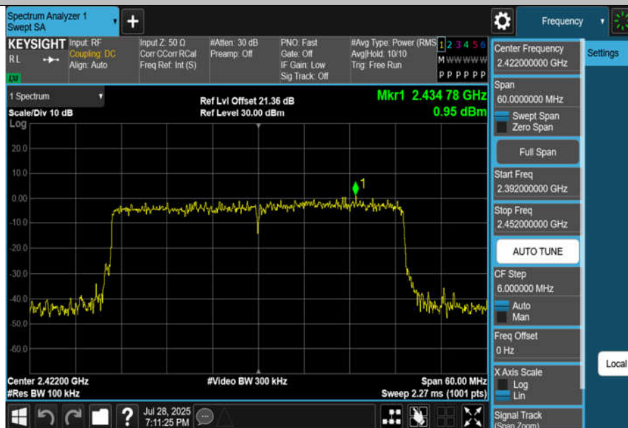
11AX40MIMO-Ant2-2422-0~Reference-PASS
