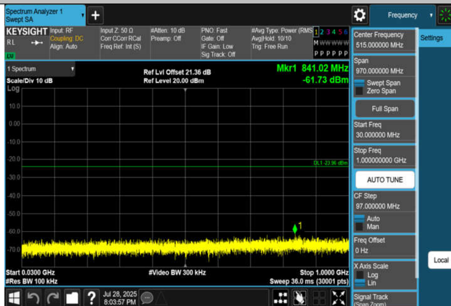
11N20MIMO-Ant2-2412-30~1000-PASS
