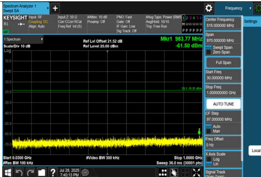
11AX40MIMO-Ant1-2437-30~1000-PASS
