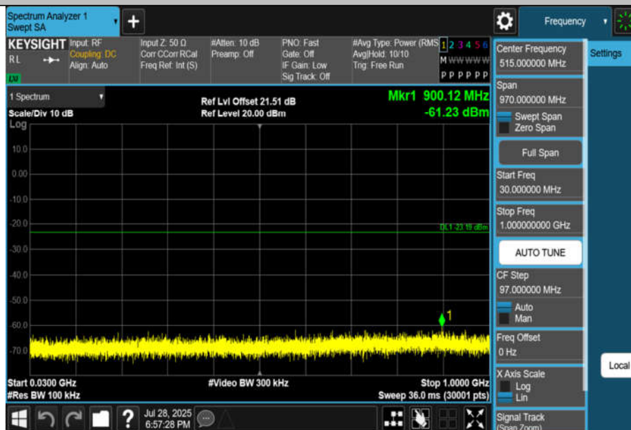
11AX20MIMO-Ant2-2462-30~1000-PASS
