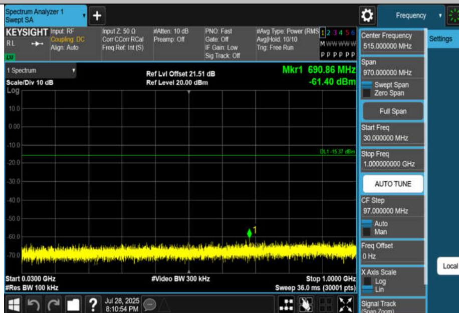
11N20MIMO-Ant2-2437-30~1000-PASS
