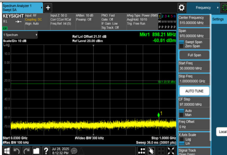
11N20MIMO-Ant2-2462-30~1000-PASS
