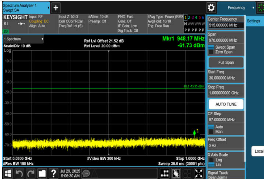
11BE20MIMO-Ant1-2437-30~1000-PASS
