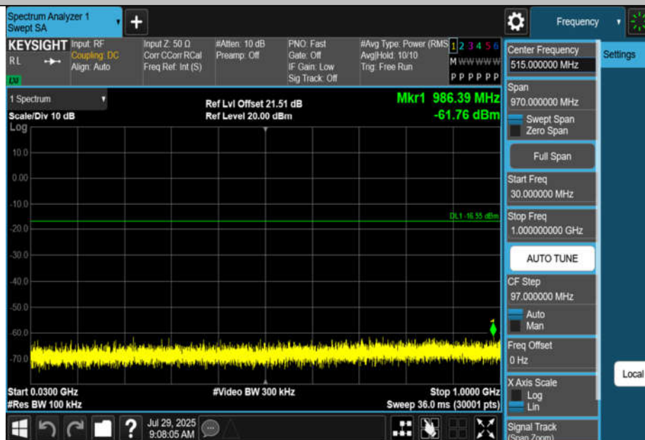
11BE20MIMO-Ant2-2437-30~1000-PASS
