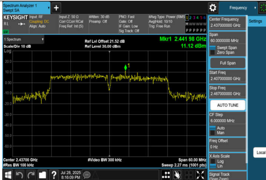
11N40MIMO-Ant1-2437-0~Reference-PASS
