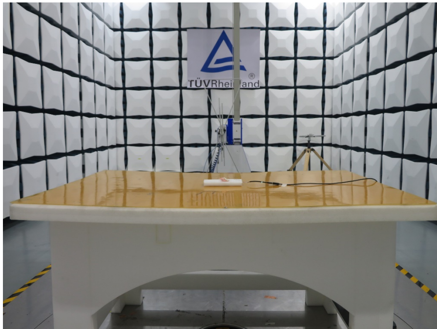
Photograph 2: Set-up photo for Radiated Spurious Emission, below 1GHz (Right earbud)
