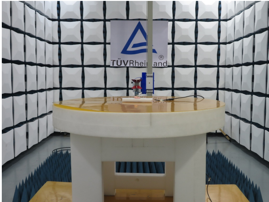
Photograph 4: Set-up photo for Radiated Spurious Emission, above 1GHz (Right earbud)
