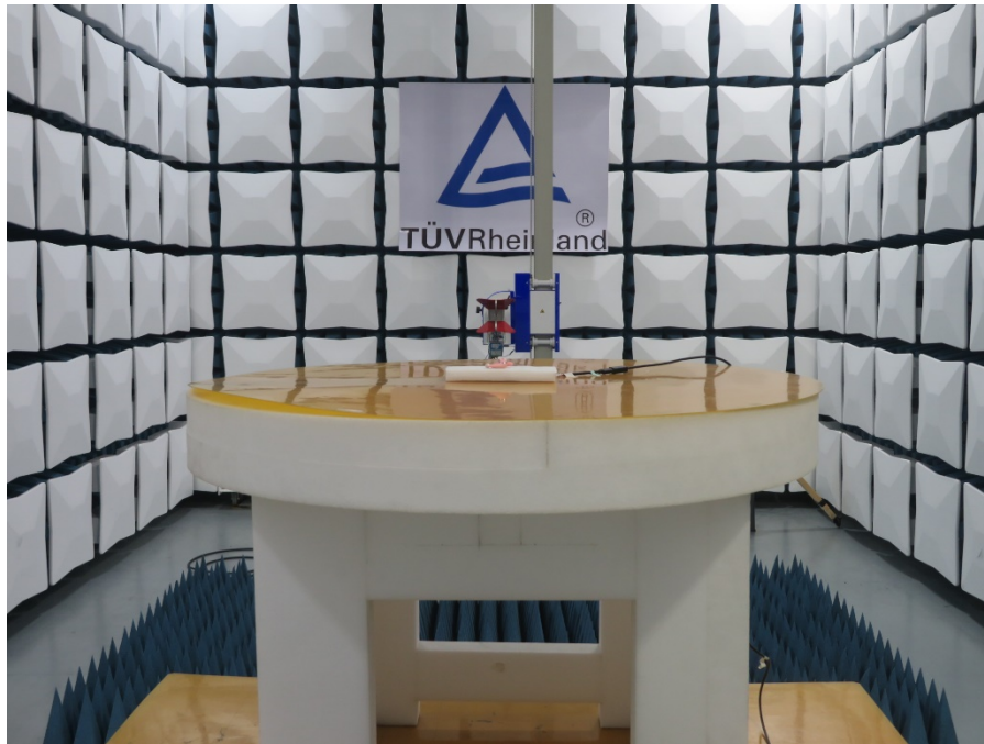
Photograph 3: Set-up photo for Radiated Spurious Emission, above 1GHz (Left earbud)
