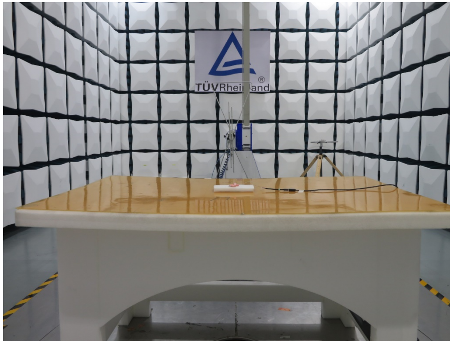
Photograph 1: Set-up photo for Radiated Spurious Emission, below 1GHz (Left earbud)
