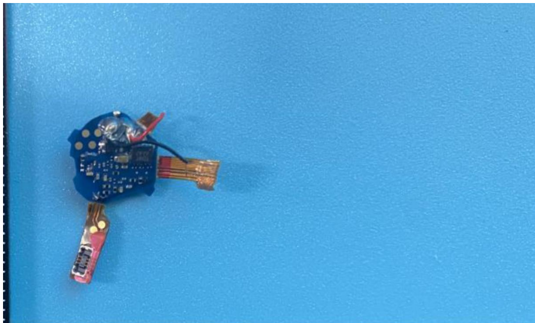
Fig. 6 PCB view of earbuds
