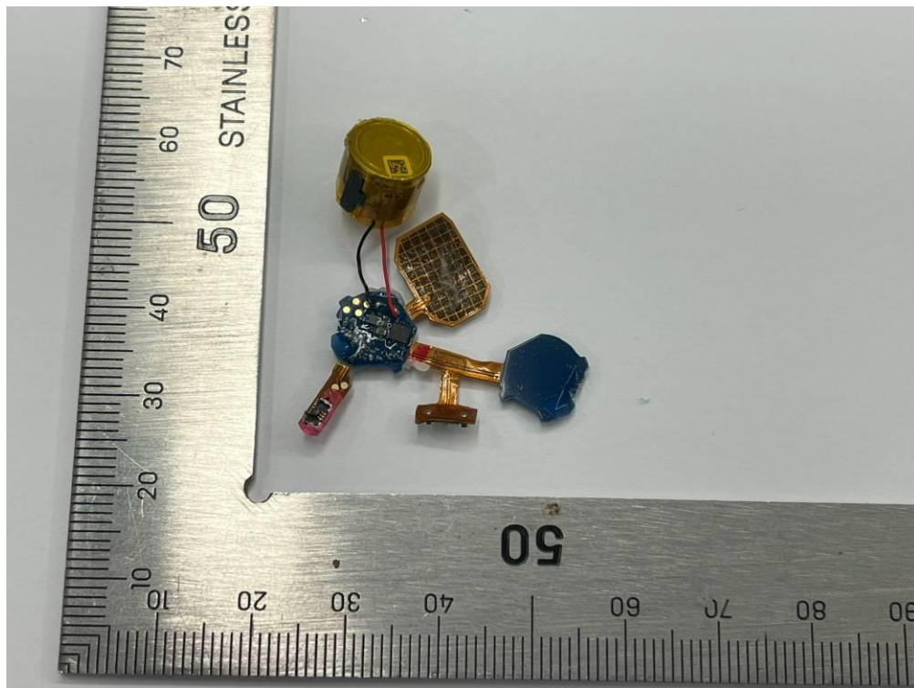
Fig. 3 Internal view 3 of earbuds
