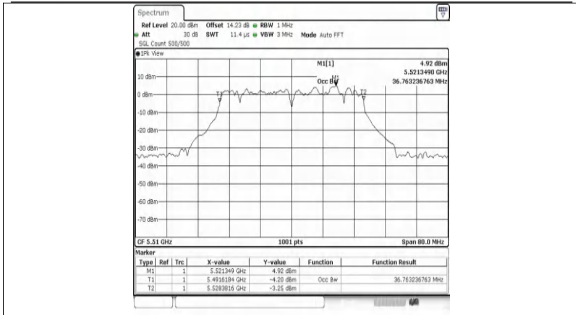
11AX40SISO-Ant1-5510
