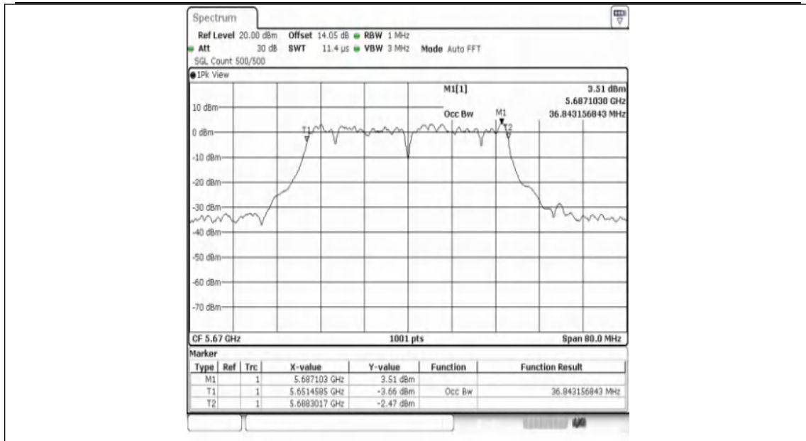
11N40SISO-Ant1-5670
