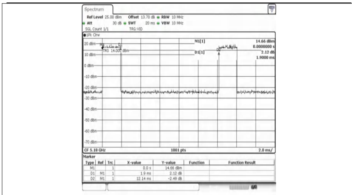
NTNV-11AX20SISO-Ant1-5180
