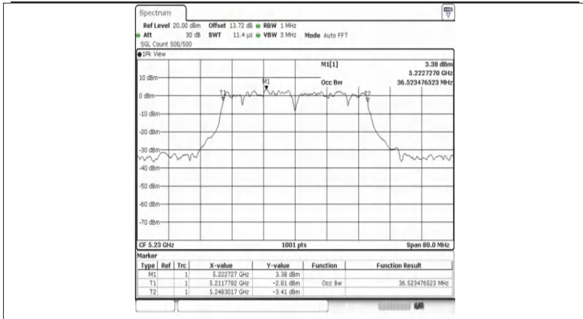
11AC40SISO-Ant1-5230
