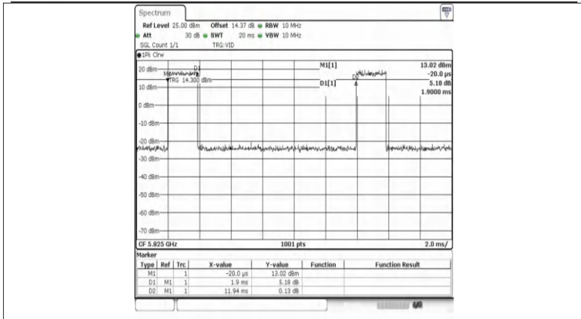
NTNV-11AC20SISO-Ant1-5825
