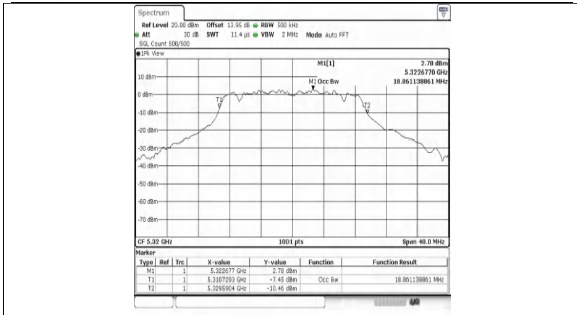
11AC20SISO-Ant1-5320
