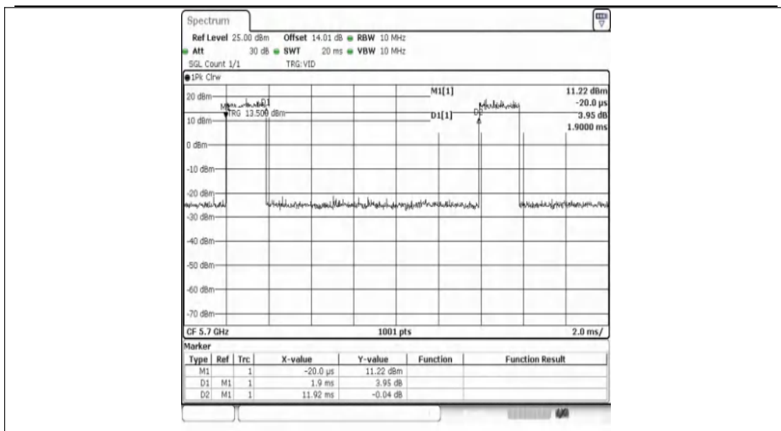
NTNV-11N20SISO-Ant1-5700
