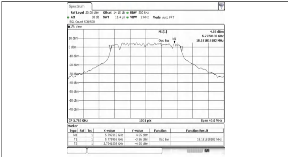
11N20SISO-Ant1-5785
