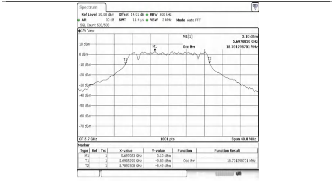
11AX20SISO-Ant1-5700
