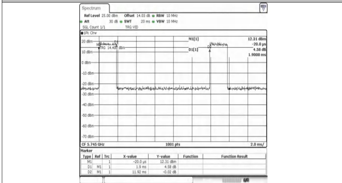
NTNV-11N20SISO-Ant1-5745
