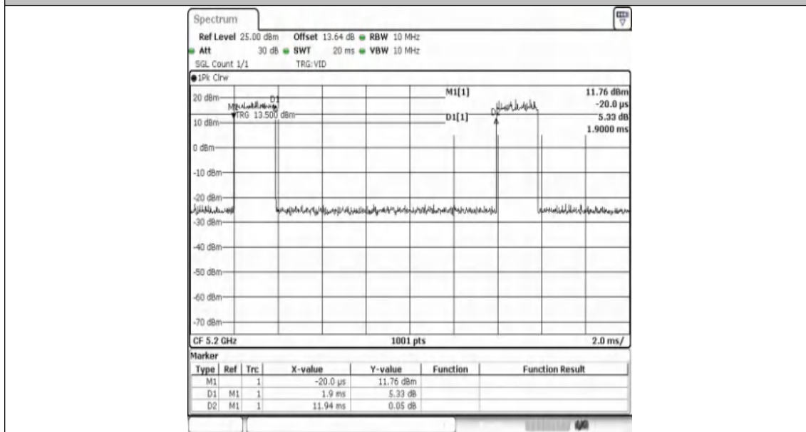
NTNV-11AX20SISO-Ant1-5200
