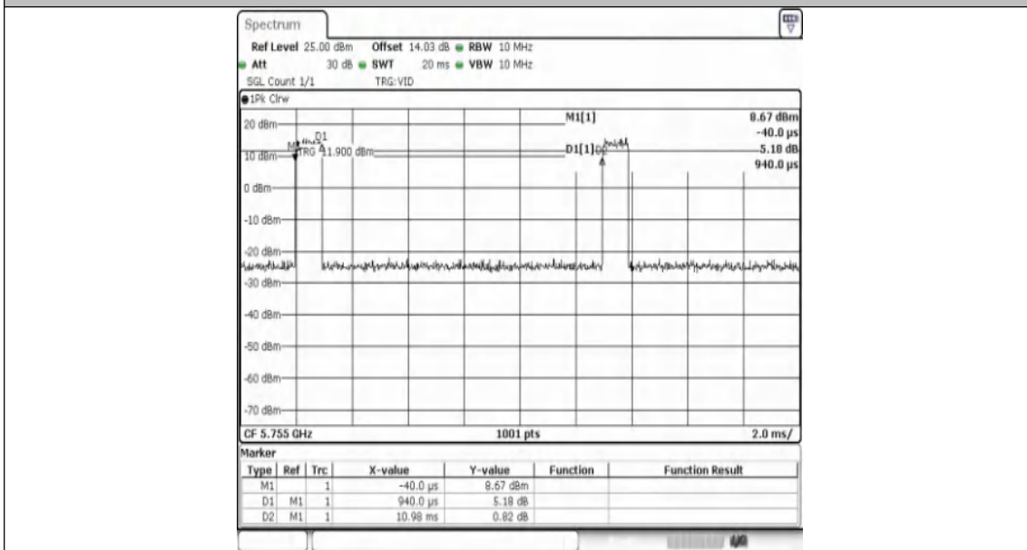
NTNV-11AX40SISO-Ant1-5755
