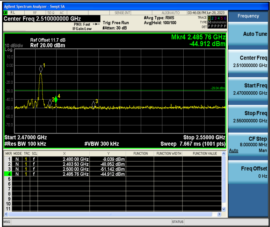
BLE_1M-Ant1-2480
