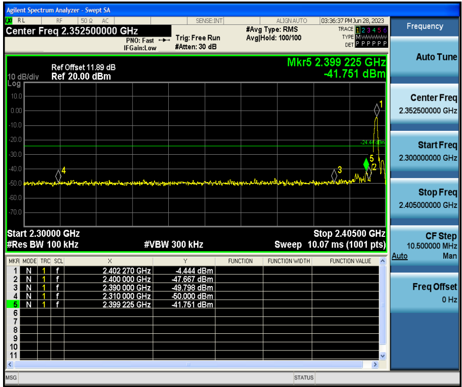
BLE_1M-Ant1-2402
