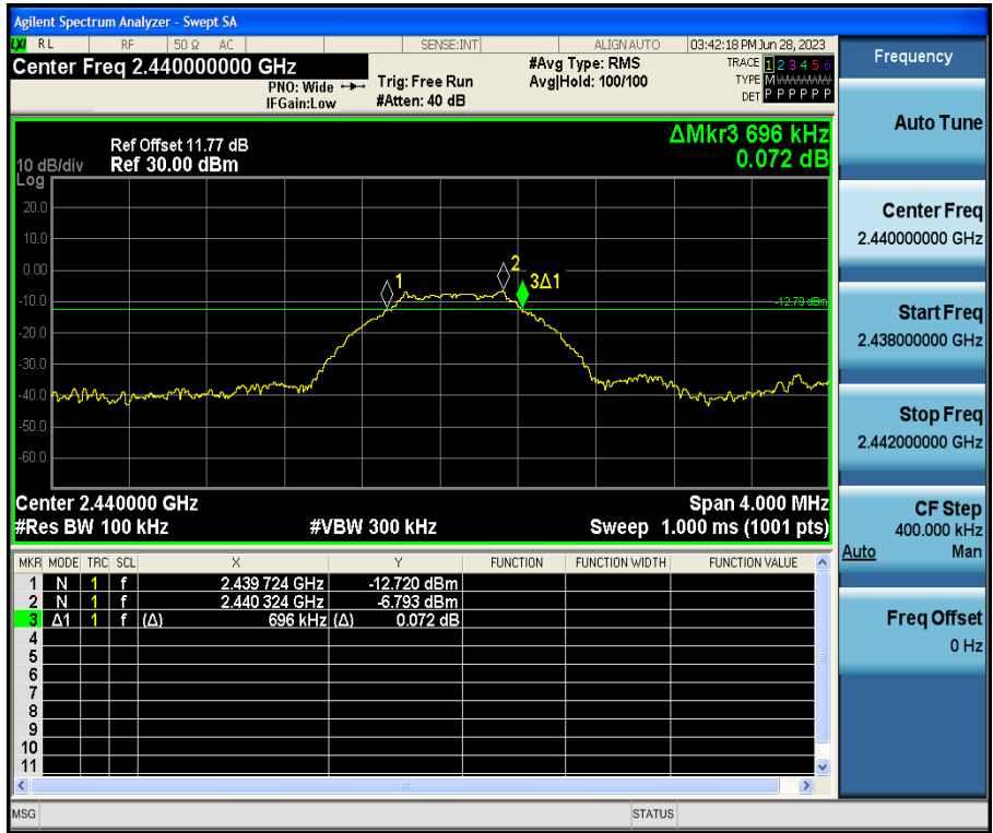
BLE_1M-Ant1-2440
