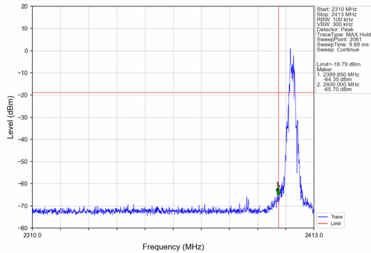
1_LCH_2405MHz_Ant1_NTNV
