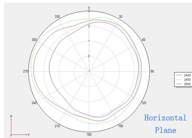
Theta 90 2D
