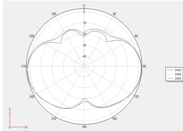
Phi 0 2D
