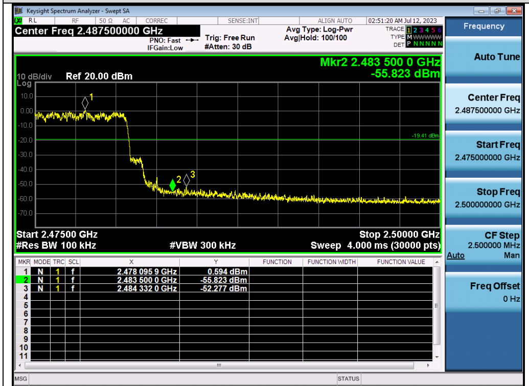
Test_Graph_BR_HOP_ANT1_NA_2Mbps_Higher Band Edge Emissions
