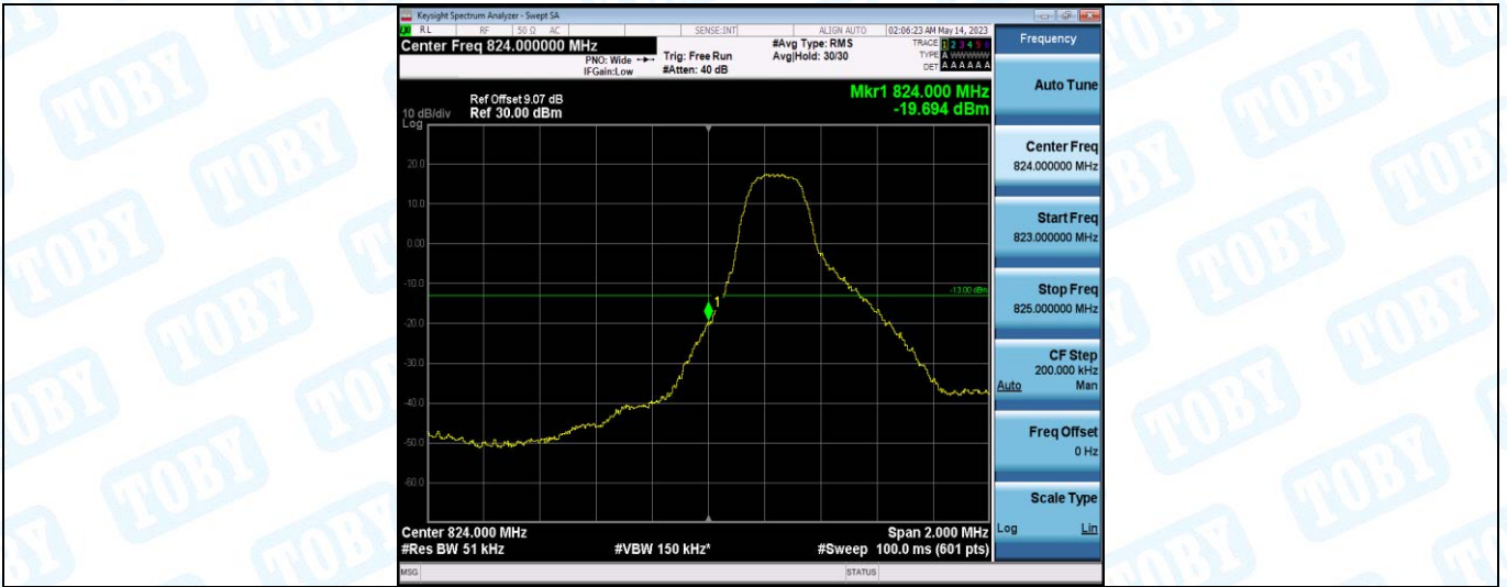
Band5-3MHz-QPSK-20415-1RB#14
