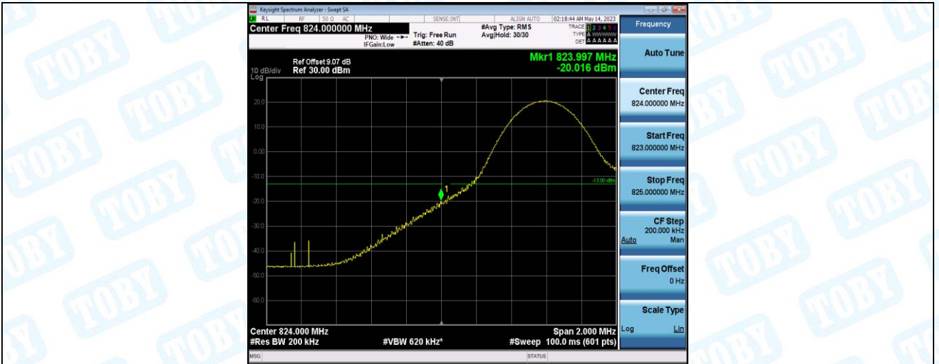
Band5-10MHz-16QAM-20450-1RB#49
