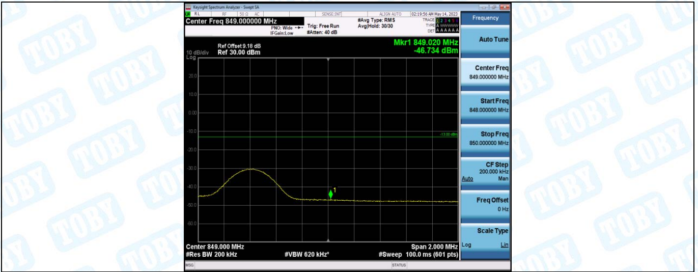
Band5-10MHz-16QAM-20600-1RB#49
