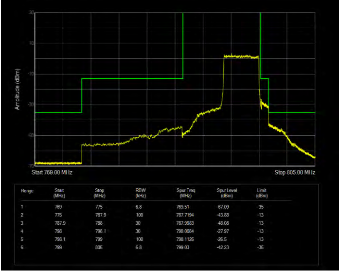
Band14 QPSK BW=5MHz Channel=23355 RB Size=25 Position=#0 Normal
