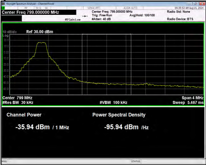
Band14 QPSK BW=5MHz Channel=23355 RB Size=1 Position=#Max Extended
