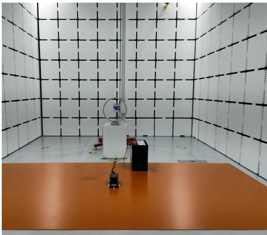
Radiated emissions- Below 30MHz
