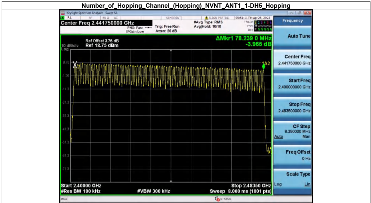
Number_of_Hopping_Channel_(Hopping)_NVNT_ANT1_1-DH5_Hopping
