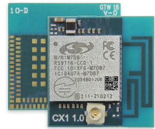
LGA Module (15 x 15.7 x 2.2) mm
