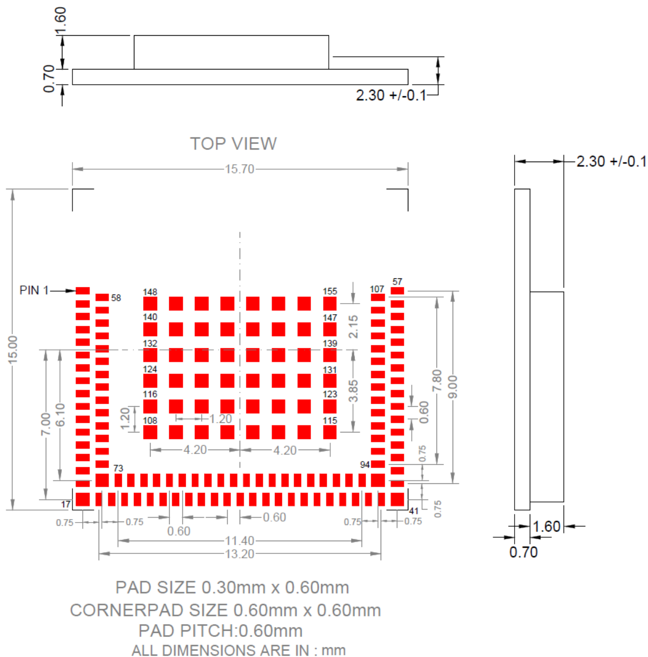
Figure 45. Package Outline
