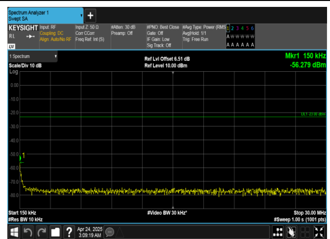
Band26(814-824)-10MHz-16QAM-26740-1RB#49-0.15-30-PASS
