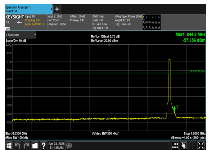
Band26(814-824)-10MHz-16QAM-26740-50RB#0-30~1000-PASS
