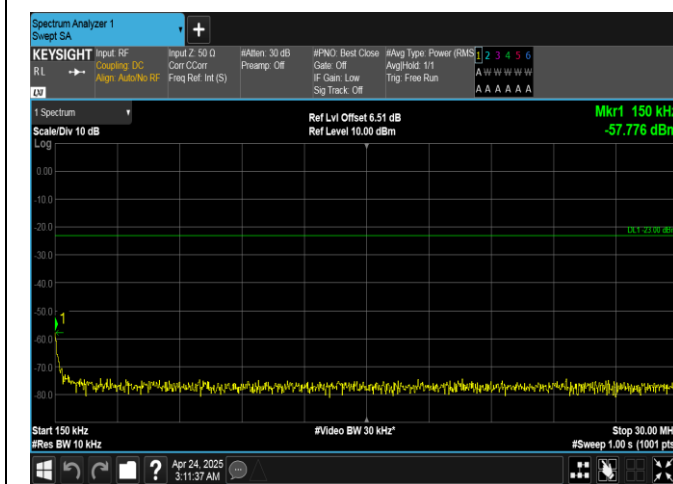
Band26(814-824)-10MHz-16QAM-26740-50RB#0-0.15~30-PASS
