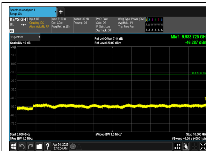
Band26(814-824)-10MHz-16QAM-26740-1RB#49-3000~10000-PASS
