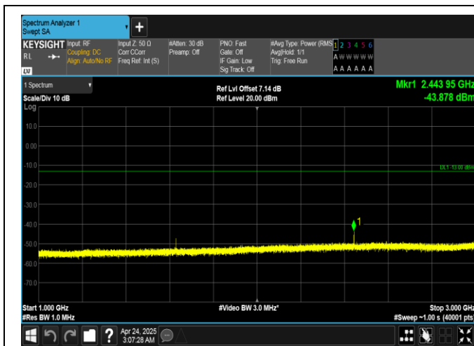
Band26(814-824)-10MHz-16QAM-26740-1RB#0-1000-3000-PASS
