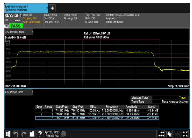
Band17-5MHz-QPSK-23825-25RB#0-PASS
