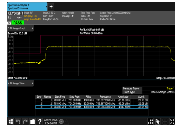
Band17-5MHz-QPSK-23755-25RB#0-PASS
