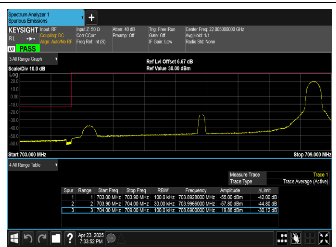
Band17-5MHz-QPSK-23755-1RB#24-PASS
