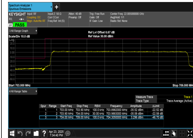
Band17-5MHz-16QAM-23755-25RB#0-PASS
