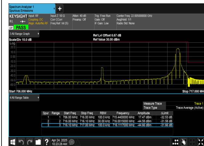
Band17-10MHz-16QAM-23800-1RB#49-PASS
