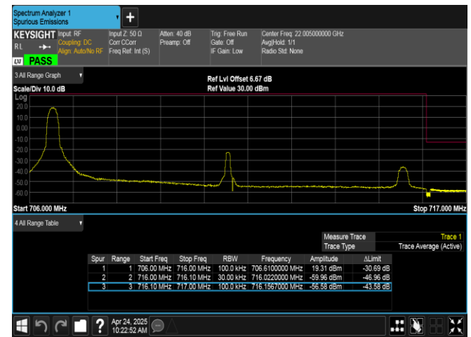
Band17-10MHz-16QAM-23800-1RB#0-PASS
