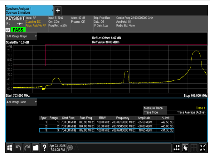
Band17-5MHz-16QAM-23755-1RB#24-PASS
