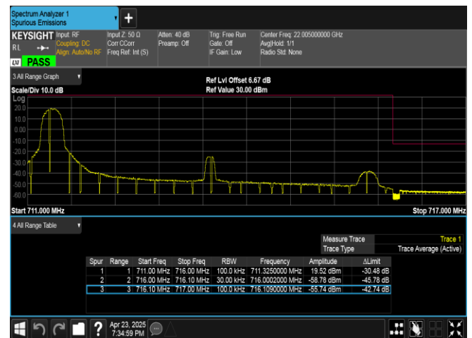
Band17-5MHz-QPSK-23825-1RB#0-PASS
