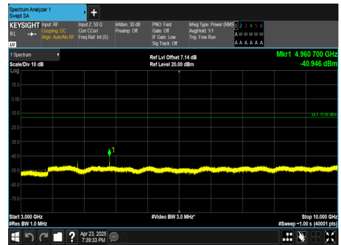
Band17-5MHz-QPSK-23755-1RB#24-3000~10000-PASS
