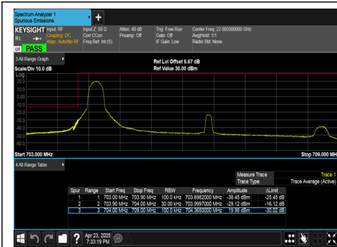
Band17-5MHz-QPSK-23755-1RB#0-PASS
