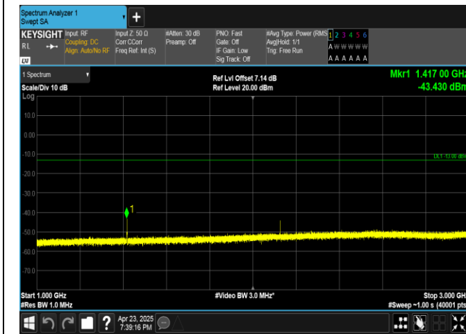
Band17-5MHz-QPSK-23755-1RB#24-1000~3000-PASS
