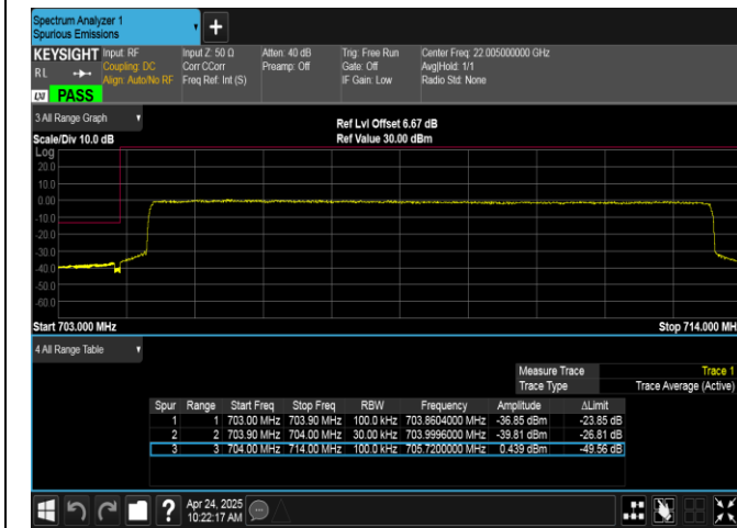
Band17-10MHz-16QAM-23780-50RB#0-PASS
