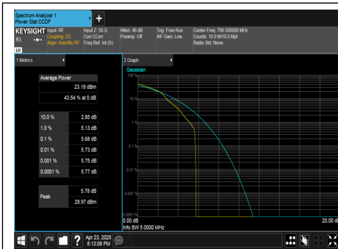
Band17-5MHz-16QAM-23755-1RB#0-PASS
