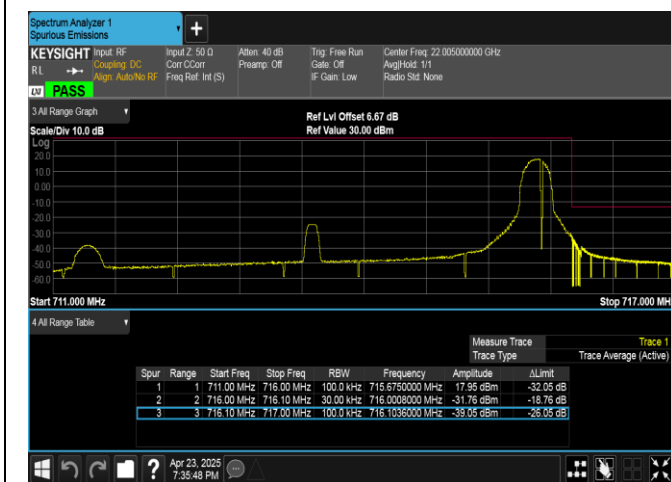
Band17-5MHz-16QAM-23825-1RB#24-PASS
