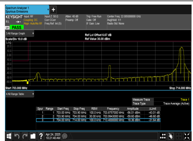
Band17-10MHz-16QAM-23780-1RB#49-PASS
