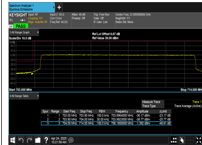
Band17-10MHz-QPSK-23780-50RB#0-PASS
