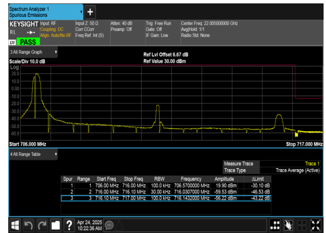
Band17-10MHz-QPSK-23800-1RB#0-PASS
