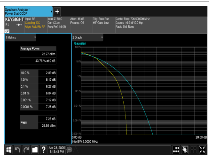
Band17-5MHz-16QAM-23755-25RB#0-PASS
