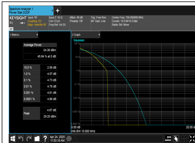
Band17-10MHz-QPSK-23780-1RB#0-PASS
