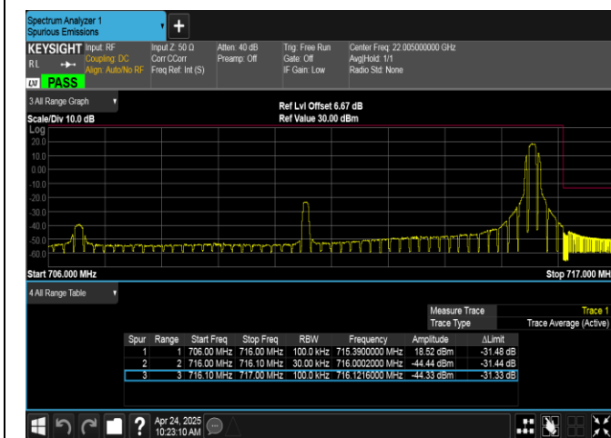
Band17-10MHz-QPSK-23800-1RB#49-PASS
