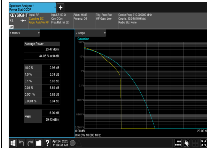
Band17-10MHz-16QAM-23790-1RB#0-PASS
