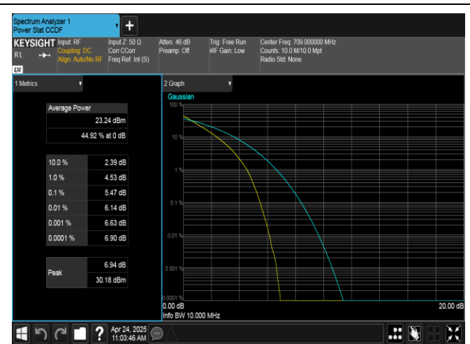
Band17-10MHz-QPSK-23780-50RB#0-PASS
