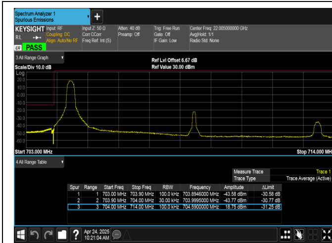
Band17-10MHz-16QAM-23780-1RB#0-PASS
