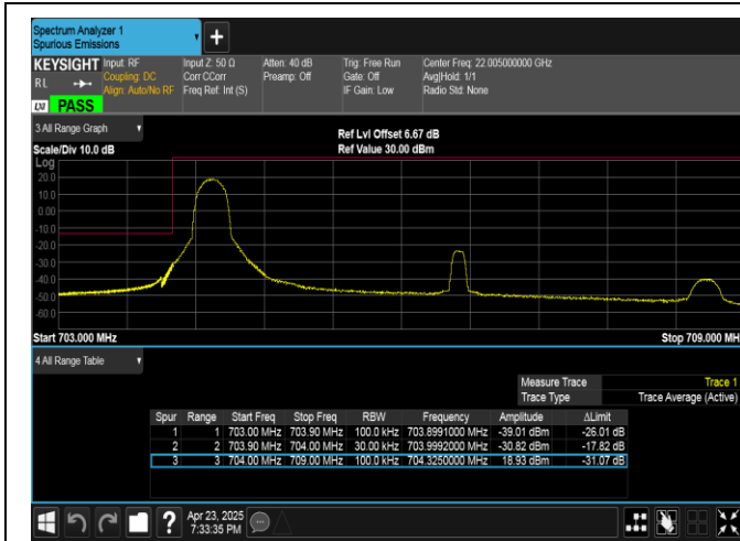
Band17-5MHz-16QAM-23755-1RB#0-PASS
