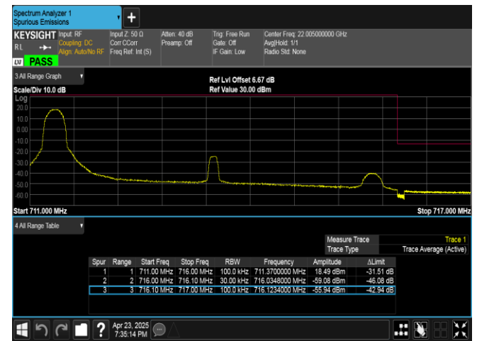
Band17-5MHz-16QAM-23825-1RB#0-PASS
