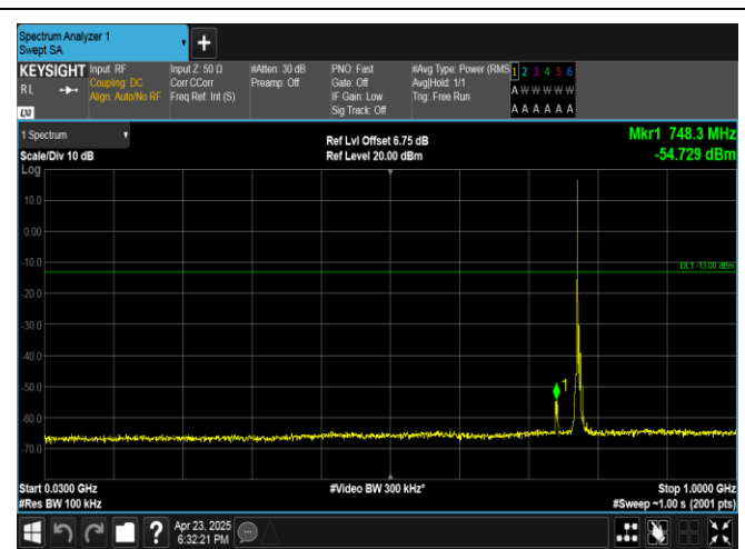
Band13-5MHz-16QAM-23205-1RB#0-30~1000-PASS
