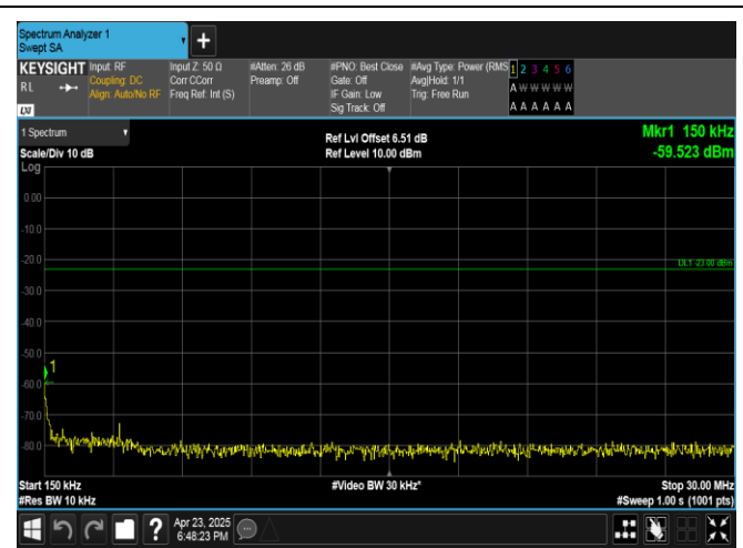
Band13-5MHz-QPSK-23255-25RB#0-0.15~30-PASS
