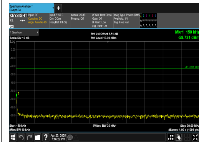
Band13-10MHz-QPSK-23230-1RB#49-0.15~30-PASS
