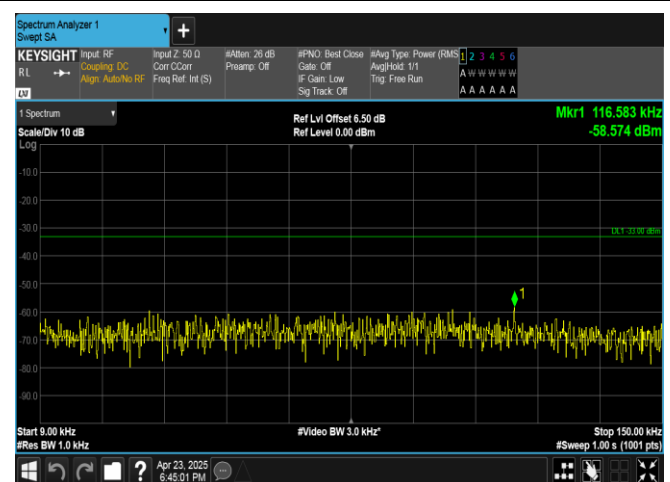
Band13-5MHz-16QAM-23255-1RB#0-0.009~0.15-PASS
