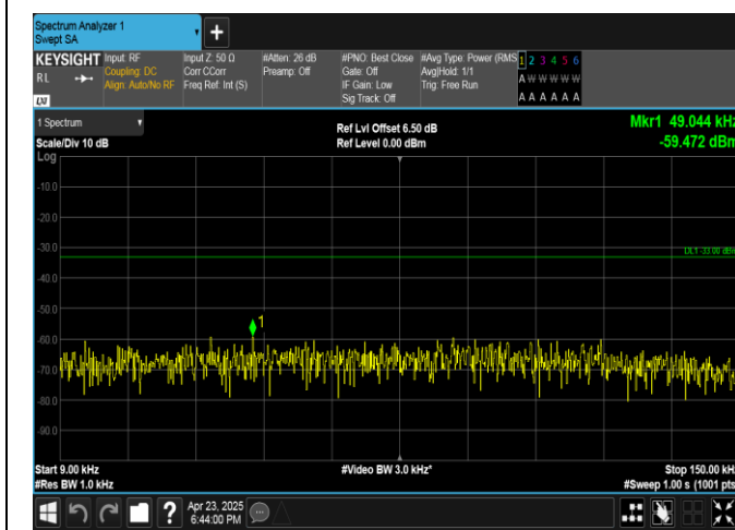
Band13-5MHz-QPSK-23255-1RB#0-0.009~0.15-PASS
