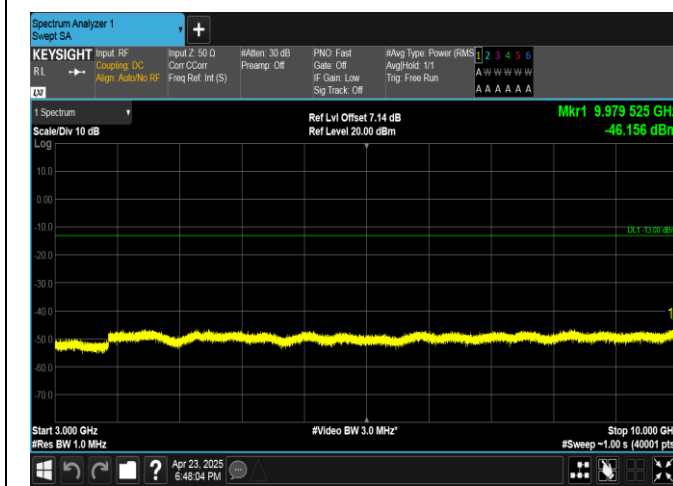
Band13-5MHz-16QAM-23255-1RB#24-3000~10000-PASS
