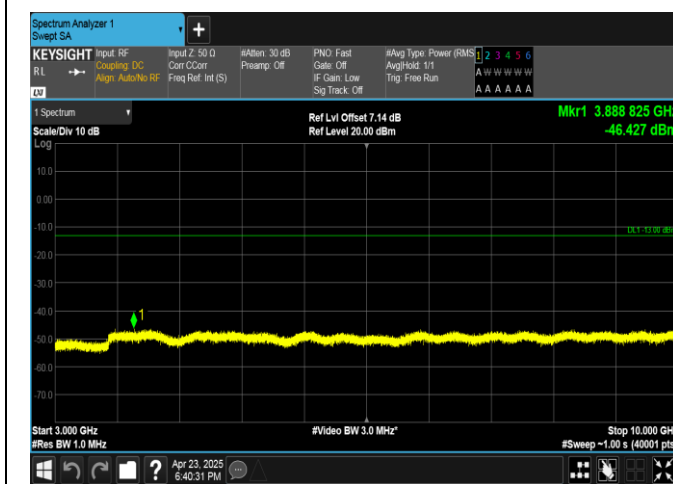
Band13-5MHz-QPSK-23230-1RB#24-3000~10000-PASS
