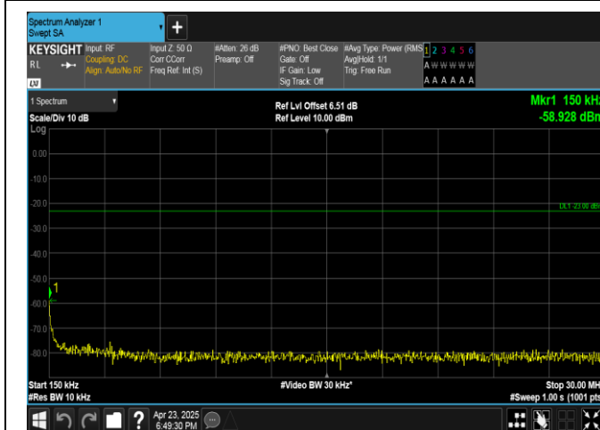
Band13-5MHz-16QAM-23255-25RB#0-0.15~30-PASS
