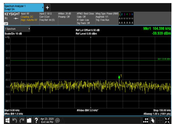
Band13-5MHz-QPSK-23230-25RB#0-0.009~0.15-PASS
