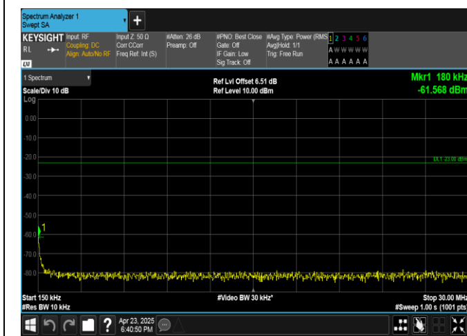
Band13-5MHz-16QAM-23230-1RB#24-0.15~30-PASS
