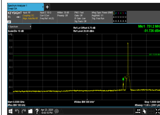
Band13-5MHz-16QAM-23230-25RB#0-30~1000-PASS
