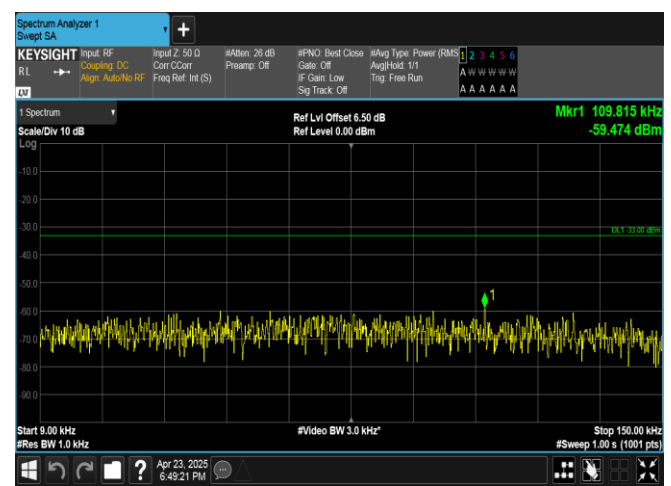
Band13-5MHz-16QAM-23255-25RB#0-0.009~0.15-PASS
