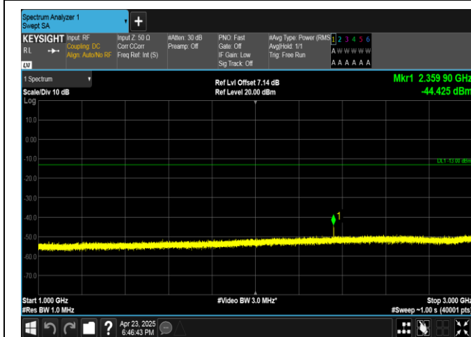
Band13-5MHz-QPSK-23255-1RB#24-1000~3000-PASS
