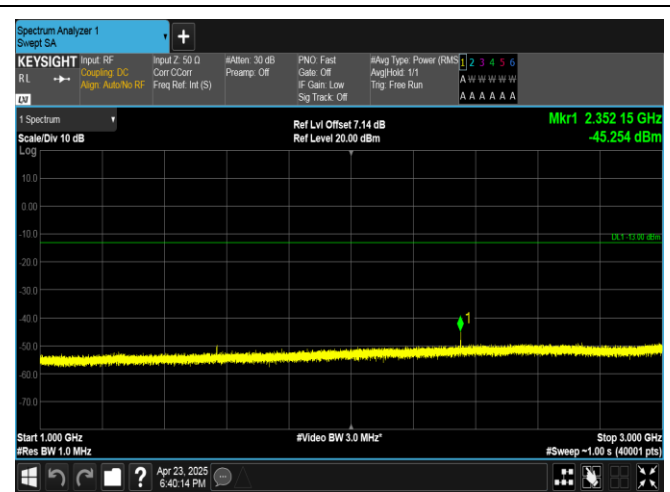
Band13-5MHz-QPSK-23230-1RB#24-1000~3000-PASS
