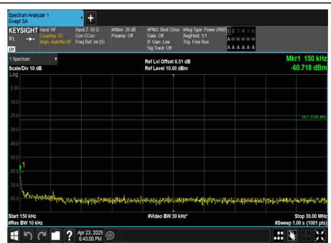
Band13-5MHz-16QAM-23230-25RB#0-0.15~30-PASS
