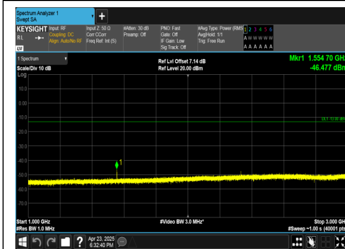
Band13-5MHz-16QAM-23205-1RB#0-1000~3000-PASS
