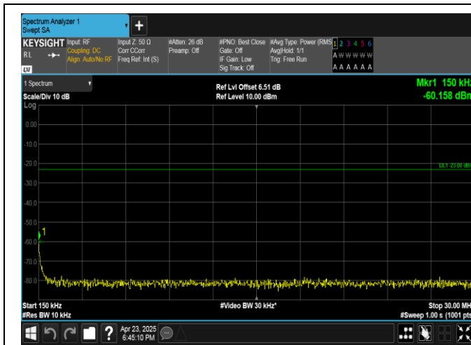
Band13-5MHz-16QAM-23255-1RB#0-0.15~30-PASS
