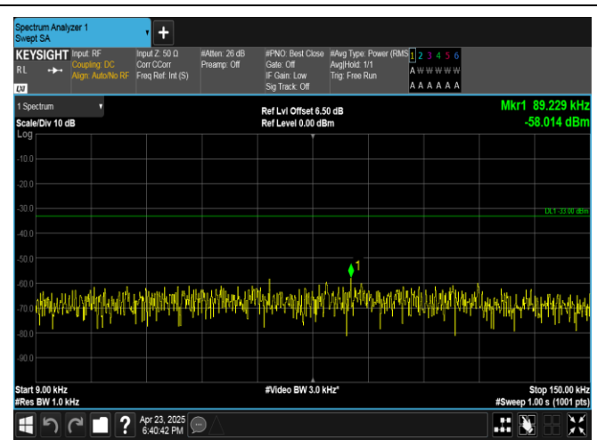
Band13-5MHz-16QAM-23230-1RB#24-0.009~0.15-PASS
