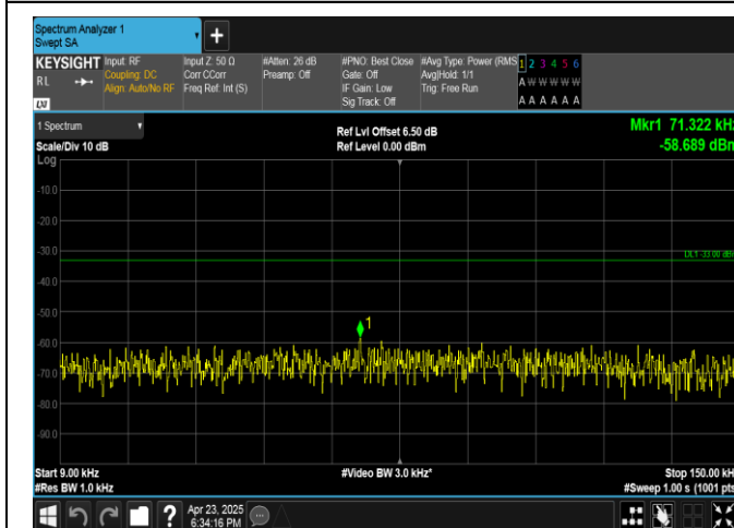
Band13-5MHz-16QAM-23205-1RB#24-0.009~0.15-PASS
