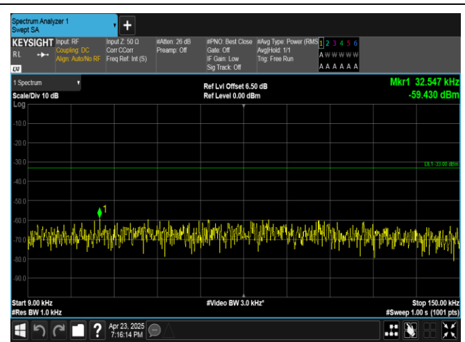
Band13-10MHz-QPSK-23230-1RB#49-0.009~0.15-PASS
