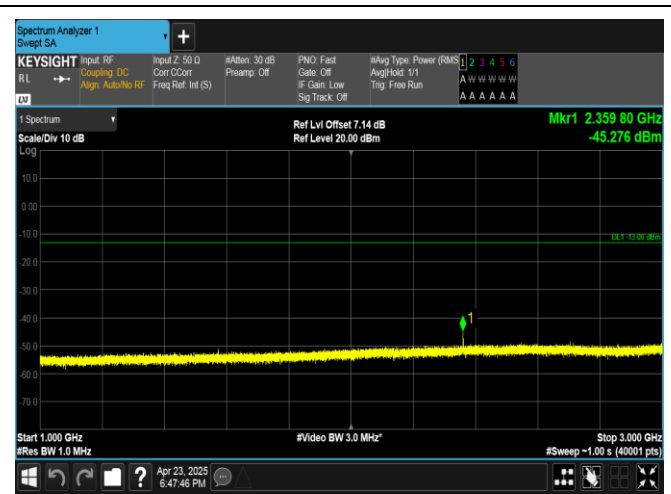
Band13-5MHz-16QAM-23255-1RB#24-1000~3000-PASS
