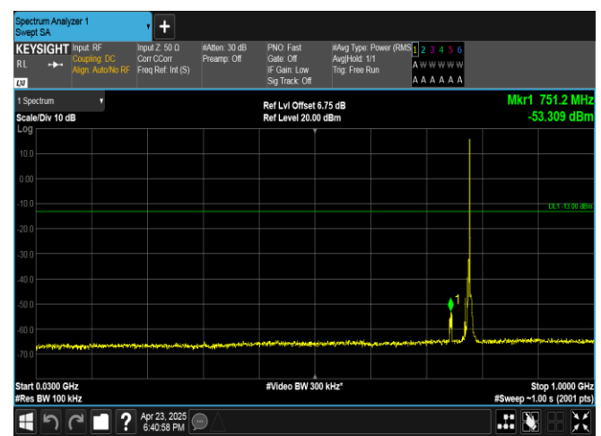
Band13-5MHz-16QAM-23230-1RB#24-30~1000-PASS
