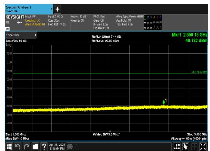
Band13-5MHz-QPSK-23255-25RB#0-1000~3000-PASS
