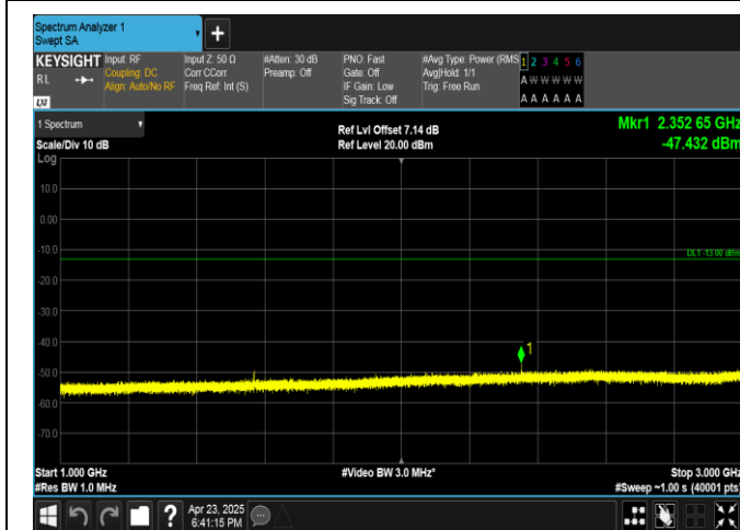
Band13-5MHz-16QAM-23230-1RB#24-1000~3000-PASS
