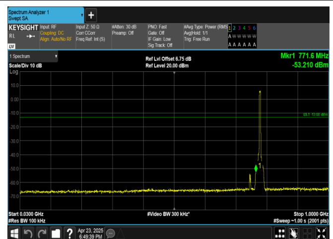
Band13-5MHz-16QAM-23255-25RB#0-30~1000-PASS
