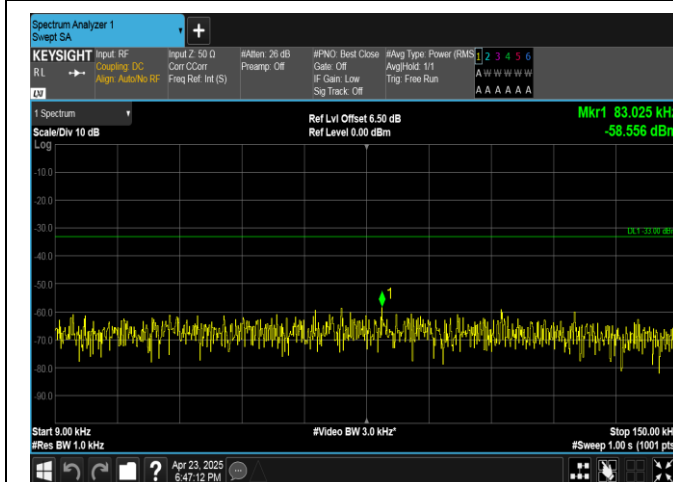
Band13-5MHz-16QAM-23255-1RB#24-0.009~0.15-PASS
