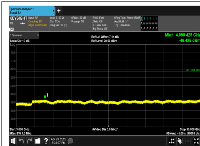
Band13-5MHz-16QAM-23230-1RB#0-3000~10000-PASS
