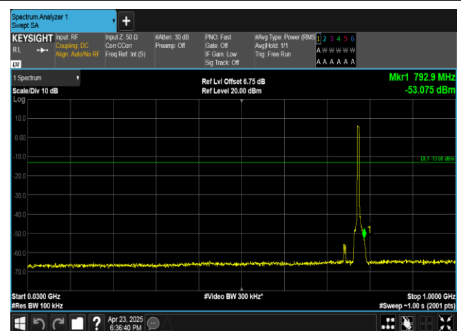
Band13-5MHz-16QAM-23205-25RB#0-30~1000-PASS
