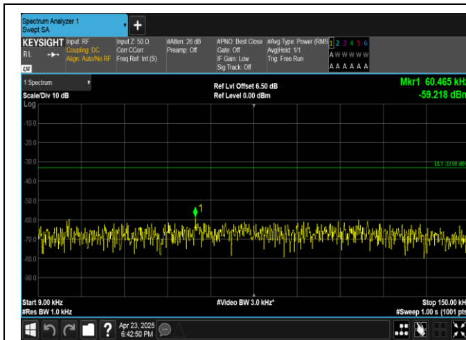
Band13-5MHz-16QAM-23230-25RB#0-0.009~0.15-PASS
