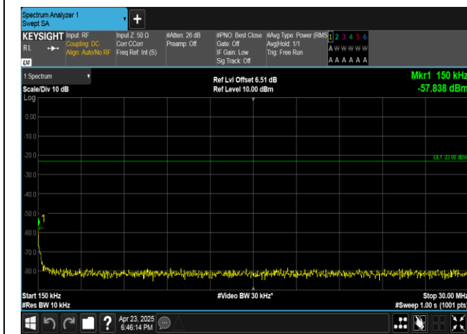
Band13-5MHz-QPSK-23255-1RB#24-0.15~30-PASS
