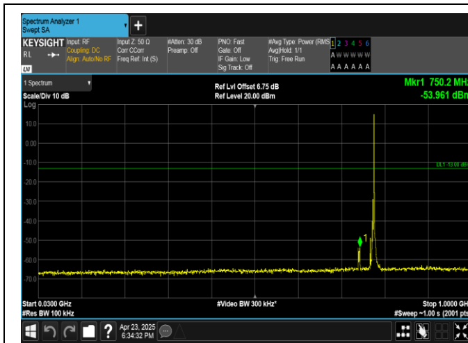
Band13-5MHz-16QAM-23205-1RB#24-30~1000-PASS
