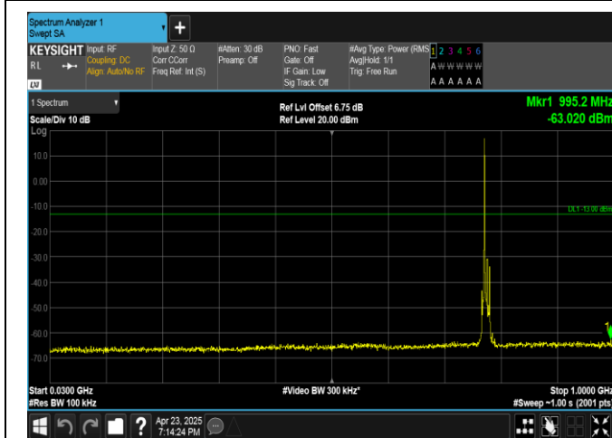
Band13-10MHz-QPSK-23230-1RB#0-30~1000-PASS
