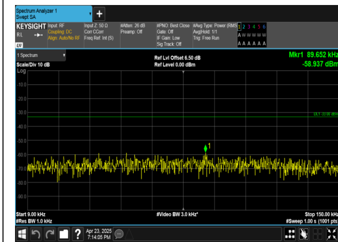
Band13-10MHz-QPSK-23230-1RB#0-0.009~0.15-PASS
