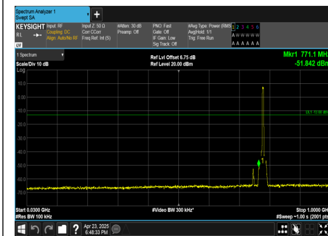
Band13-5MHz-QPSK-23255-25RB#0-30~1000-PASS
