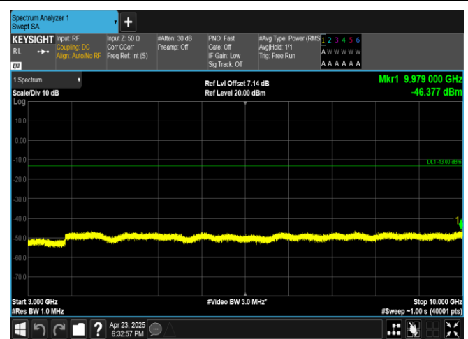
Band13-5MHz-16QAM-23205-1RB#0-3000~10000-PASS
