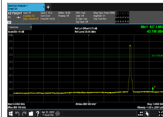
Band13-10MHz-QPSK-23230-50RB#0-30~1000-PASS
