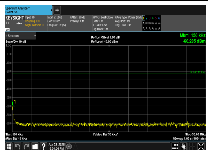
Band13-5MHz-16QAM-23205-1RB#24-0.15~30-PASS
