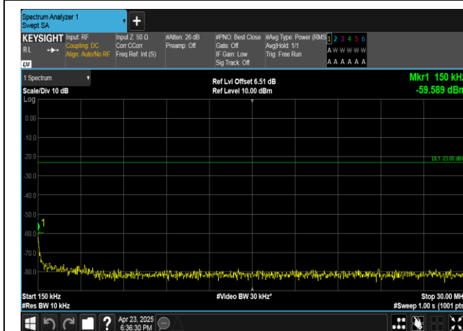
Band13-5MHz-16QAM-23205-25RB#0-0.15~30-PASS
