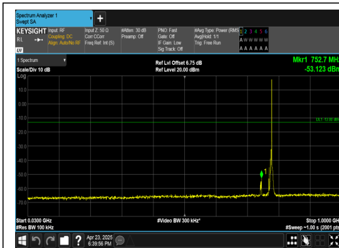
Band13-5MHz-QPSK-23230-1RB#24-30~1000-PASS
