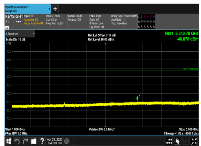
Band13-5MHz-16QAM-23230-25RB#0-1000~3000-PASS
