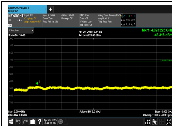
Band13-5MHz-QPSK-23255-1RB#0-3000~10000-PASS
