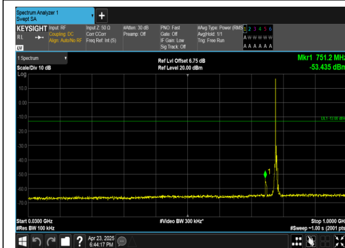
Band13-5MHz-QPSK-23255-1RB#0-30~1000-PASS
