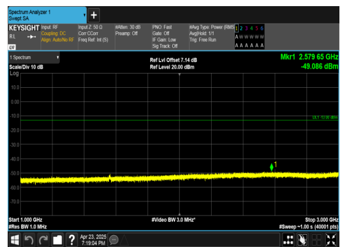
Band13-10MHz-QPSK-23230-50RB#0-1000~3000-PASS
