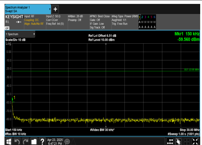
Band13-5MHz-16QAM-23255-1RB#24-0.15~30-PASS
