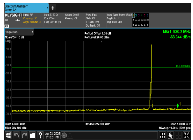
Band13-10MHz-QPSK-23230-1RB#49-30~1000-PASS
