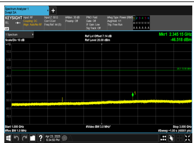
Band13-5MHz-16QAM-23205-1RB#24-1000~3000-PASS
