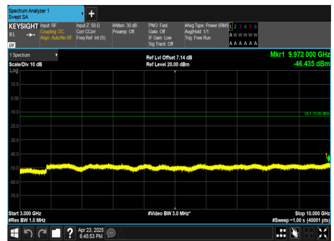
Band13-5MHz-16QAM-23255-1RB#0-3000~10000-PASS
