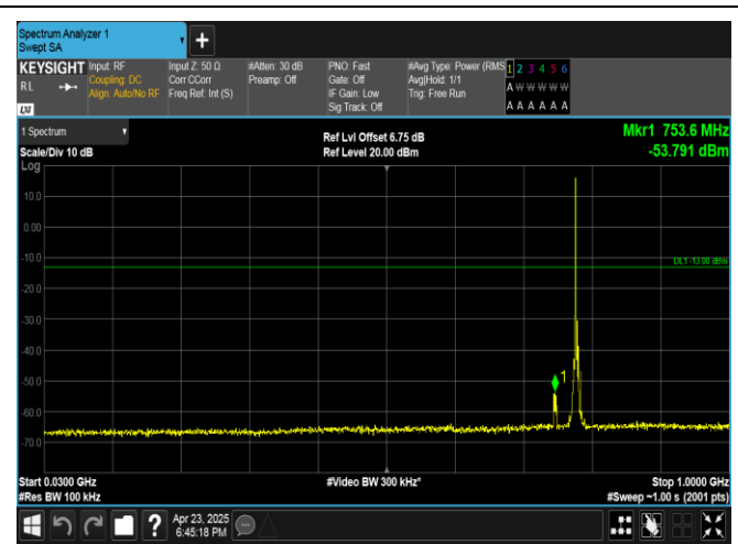
Band13-5MHz-16QAM-23255-1RB#0-30~1000-PASS
