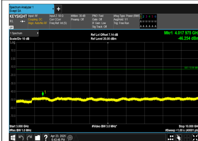
Band13-5MHz-16QAM-23230-25RB#0-3000~10000-PASS
