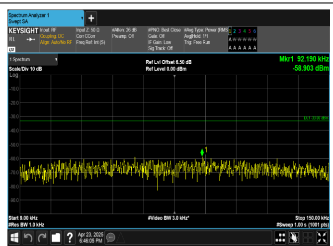
Band13-5MHz-QPSK-23255-1RB#24-0.009~0.15-PASS
