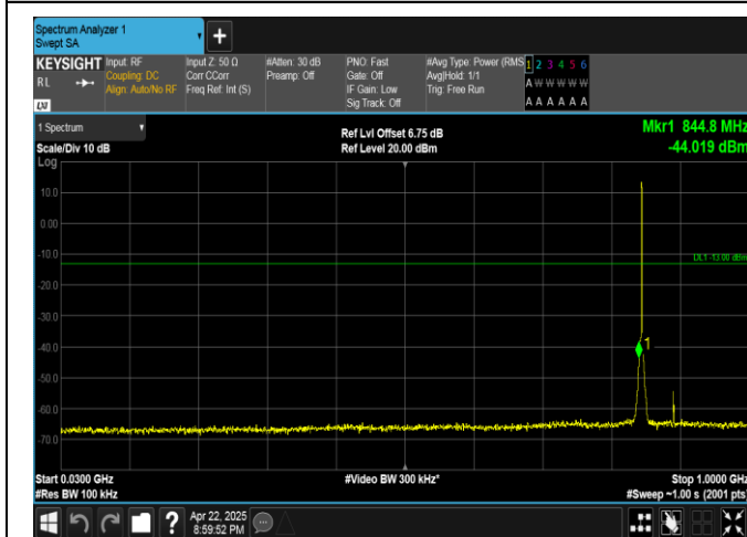
Band5-1.4MHz-QPSK-20643-6RB#0-30~1000-PASS
