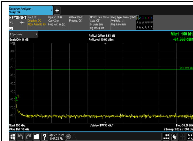
Band5-1.4MHz-16QAM-20407-6RB#0-0.15~30-PASS
