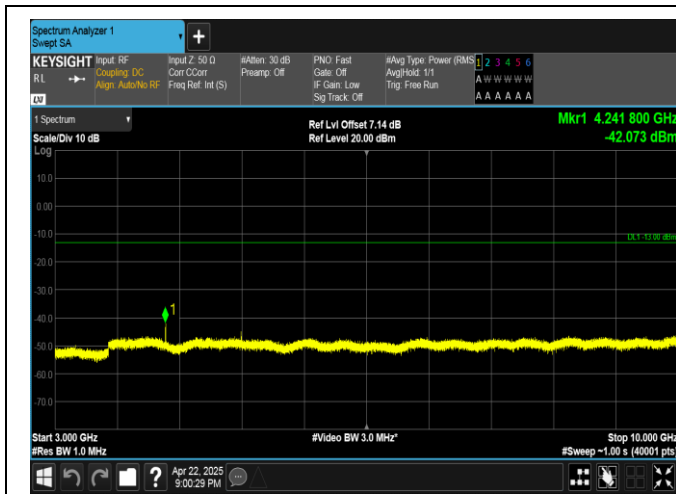
Band5-1.4MHz-QPSK-20643-6RB#0-3000~10000-PASS
