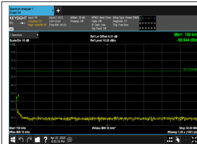
Band5-1.4MHz-QPSK-20525-6RB#0-0.15~30-PASS
