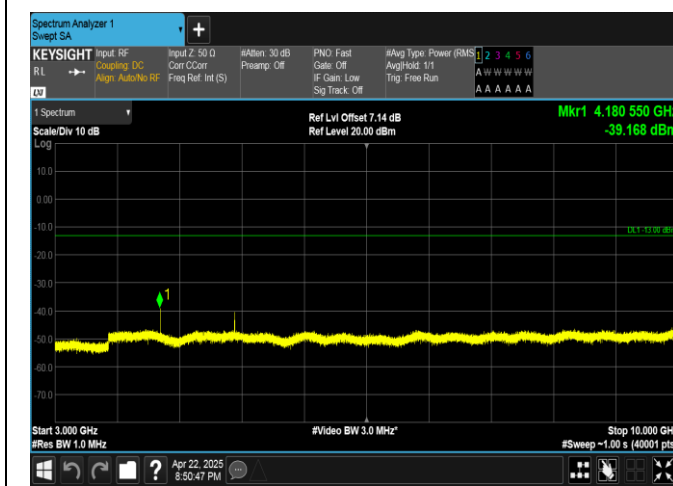
Band5-1.4MHz-16QAM-20525-1RB#0-3000~10000-PASS
