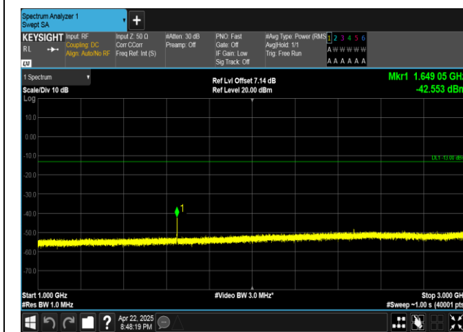
Band5-1.4MHz-16QAM-20407-6RB#0-1000~3000-PASS
