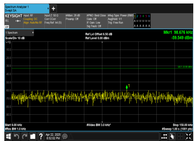
Band5-1.4MHz-16QAM-20525-1RB#5-0.009~0.15-PASS
