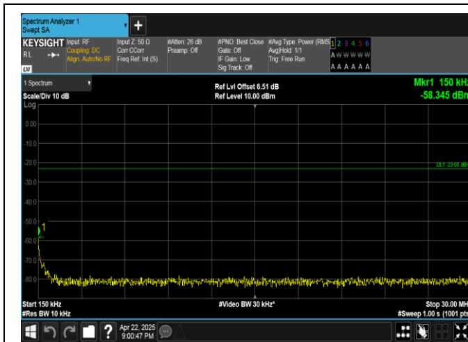
Band5-1.4MHz-16QAM-20643-6RB#0-0.15~30-PASS
