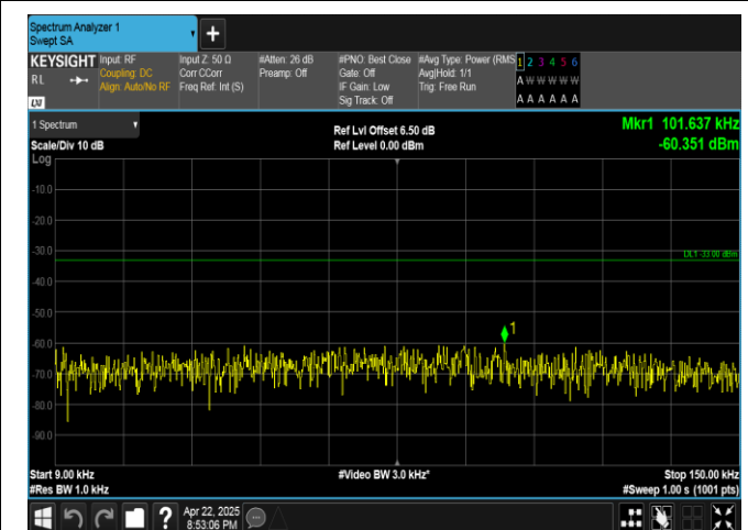
Band5-1.4MHz-QPSK-20525-6RB#0-0.009~0.15-PASS
