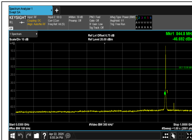
Band5-1.4MHz-QPSK-20643-1RB#0-30~1000-PASS
