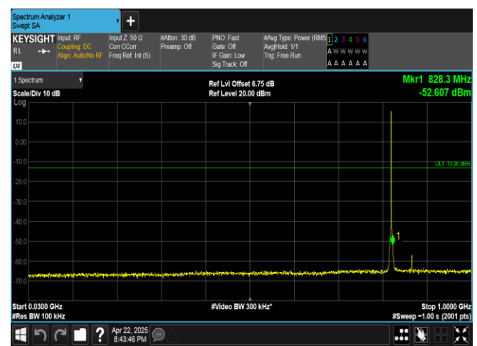
Band5-1.4MHz-16QAM-20407-1RB#0-30~1000-PASS
