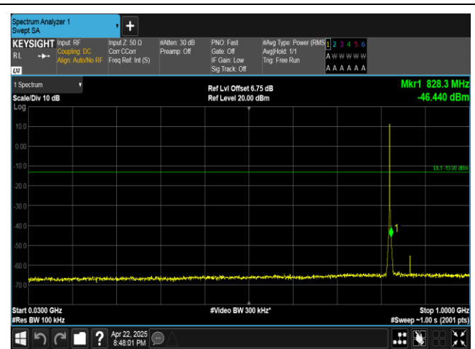
Band5-1.4MHz-16QAM-20407-6RB#0-30~1000-PASS
