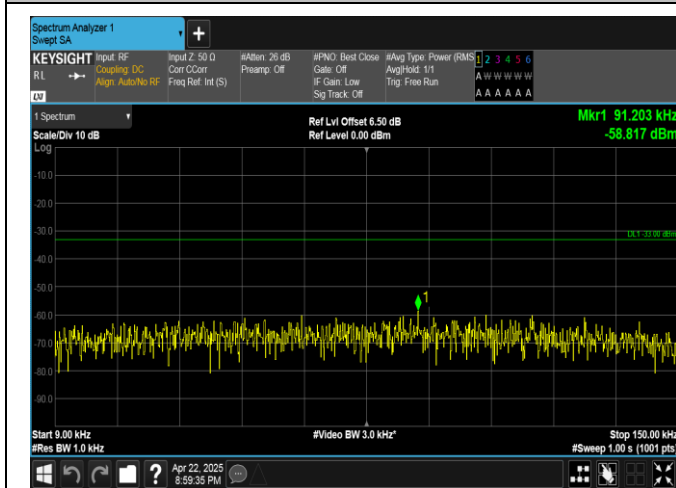
Band5-1.4MHz-QPSK-20643-6RB#0-0.009~0.15-PASS
