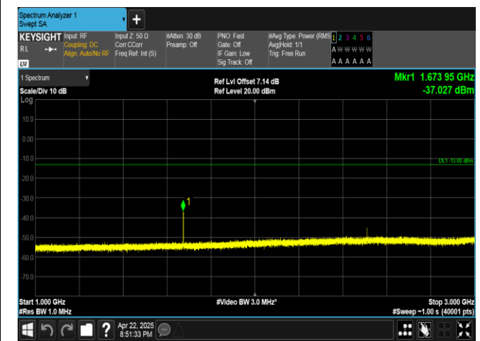
Band5-1.4MHz-QPSK-20525-1RB#5-1000~3000-PASS
