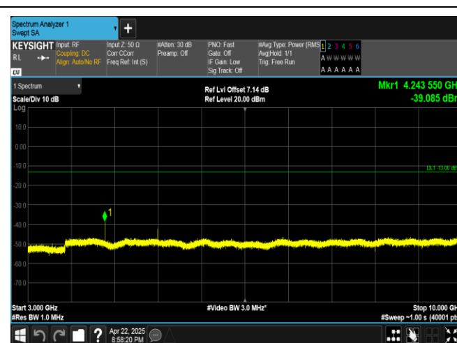
Band5-1.4MHz-QPSK-20643-1RB#5-3000~10000-PASS
