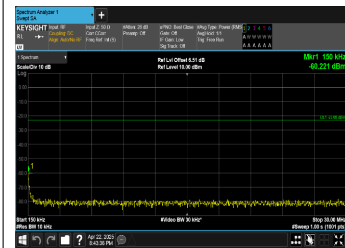
Band5-1.4MHz-16QAM-20407-1RB#0-0.15~30-PASS
