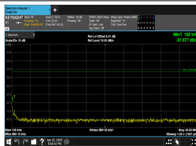
Band5-1.4MHz-QPSK-20643-6RB#0-0.15~30-PASS
