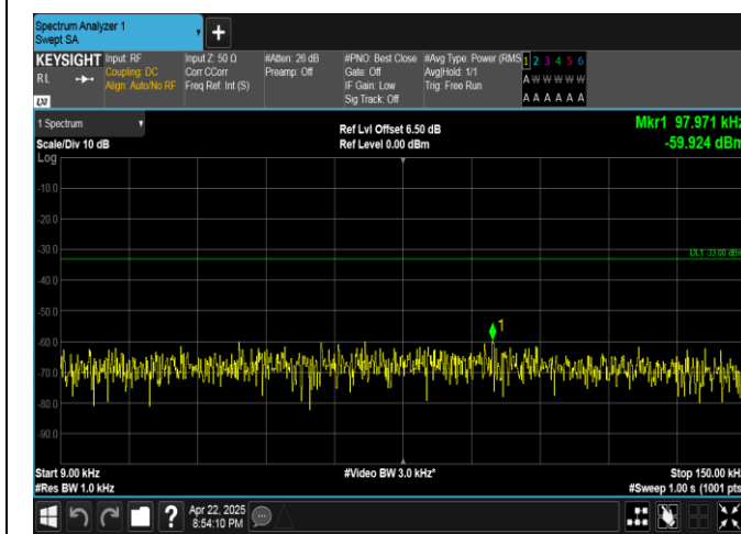
Band5-1.4MHz-16QAM-20525-6RB#0-0.009~0.15-PASS
