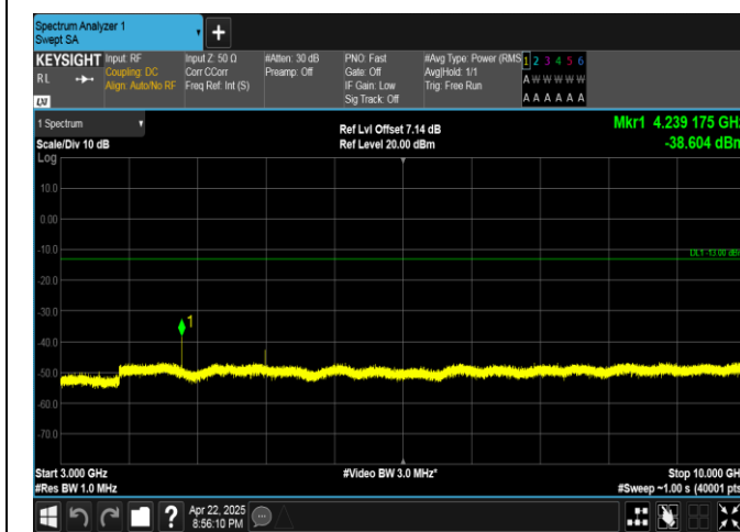
Band5-1.4MHz-QPSK-20643-1RB#0-3000~10000-PASS
