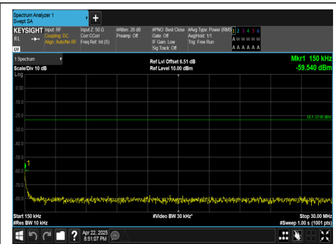
Band5-1.4MHz-QPSK-20525-1RB#5-0.15~30-PASS
