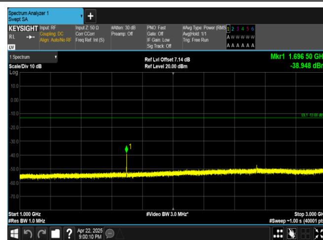
Band5-1.4MHz-QPSK-20643-6RB#0-1000~3000-PASS
