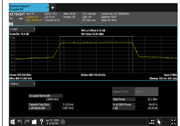
Band5-3MHz-16QAM-20415-15RB#0-PASS
