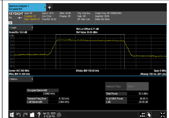
Band5-3MHz-16QAM-20635-15RB#0-PASS
