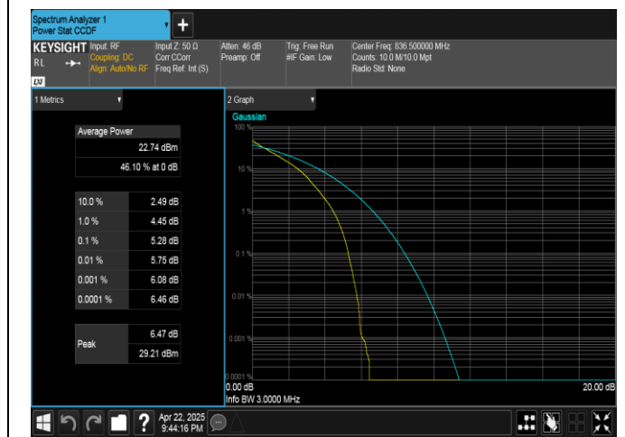
Band5-3MHz-QPSK-20525-15RB#0-PASS
