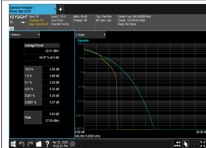
Band5-5MHz-16QAM-20625-1RB#0-PASS
