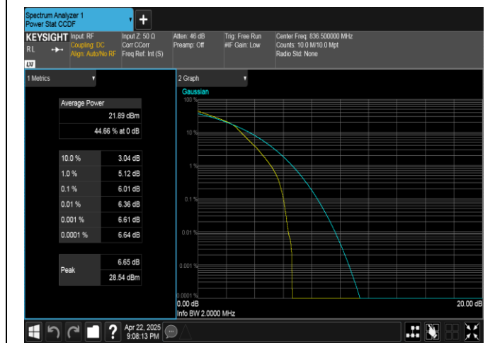
Band5-1.4MHz-16QAM-20525-6RB#0-PASS
