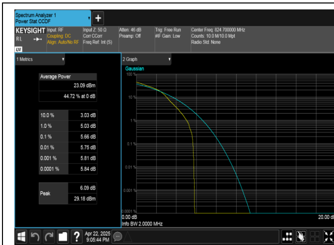
Band5-1.4MHz-16QAM-20407-1RB#0-PASS
