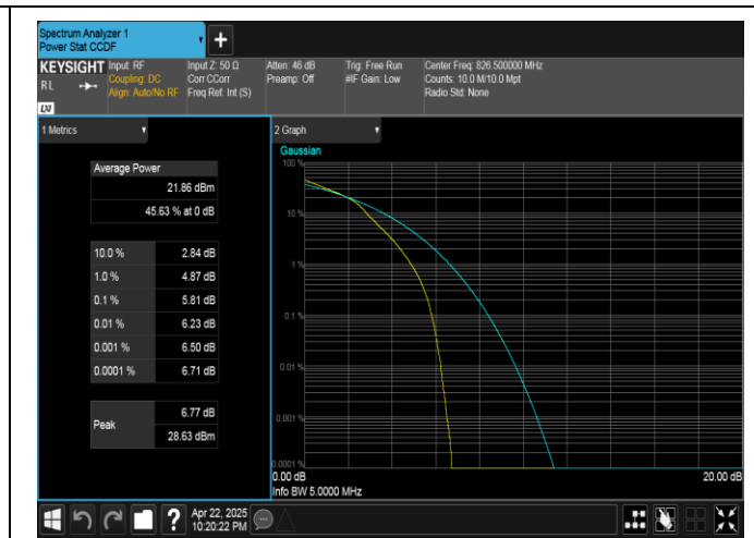
Band5-5MHz-16QAM-20425-25RB#0-PASS
