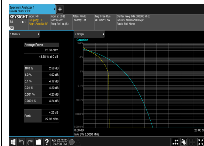
Band5-3MHz-QPSK-20635-1RB#0-PASS
