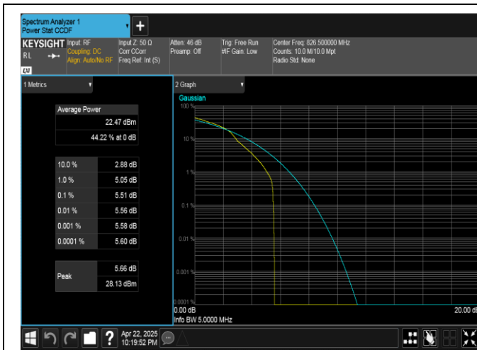
Band5-5MHz-16QAM-20425-1RB#0-PASS
