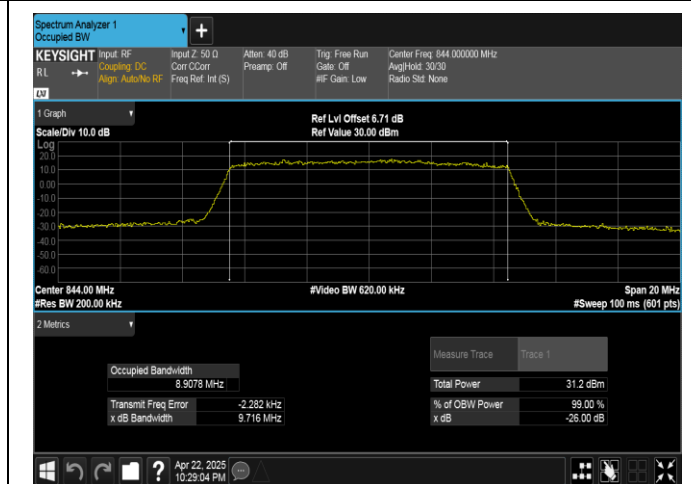
Band5-10MHz-16QAM-20600-50RB#0-PASS
