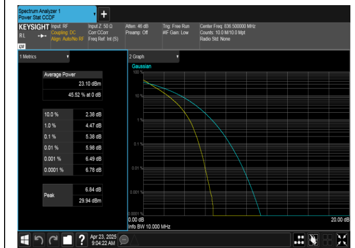
Band5-10MHz-QPSK-20525-50RB#0-PASS
