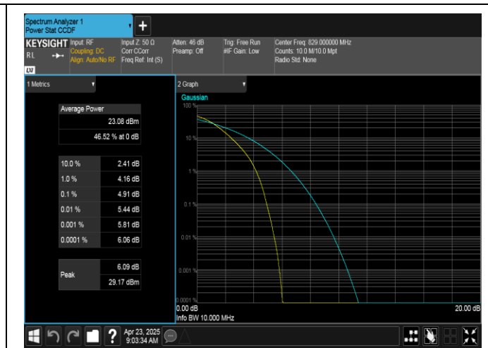
Band5-10MHz-QPSK-20450-50RB#0-PASS
