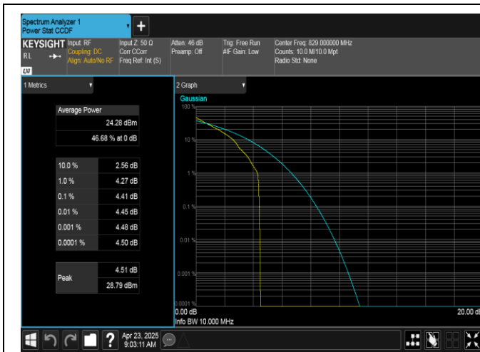
Band5-10MHz-QPSK-20450-1RB#0-PASS
