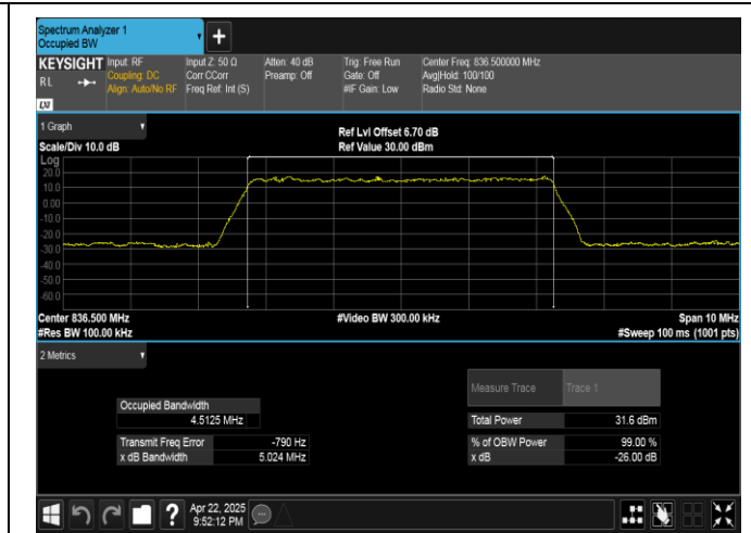
Band5-5MHz-QPSK-20525-25RB#0-PASS
