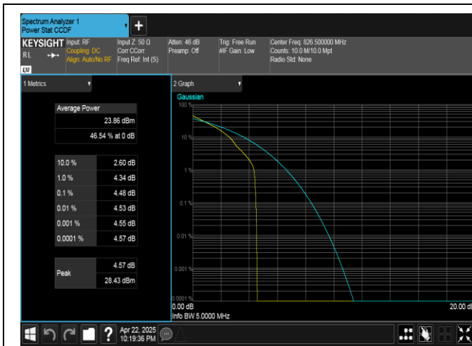
Band5-5MHz-QPSK-20425-1RB#0-PASS
