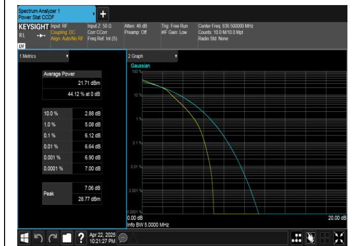
Band5-5MHz-16QAM-20525-25RB#0-PASS
