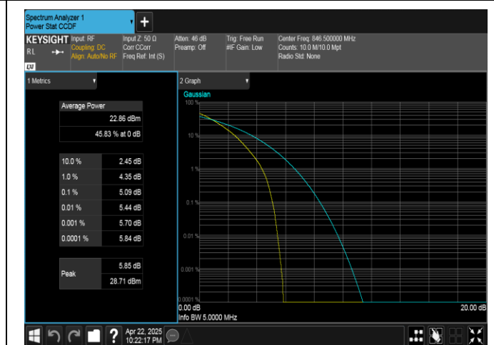
Band5-5MHz-QPSK-20625-25RB#0-PASS
