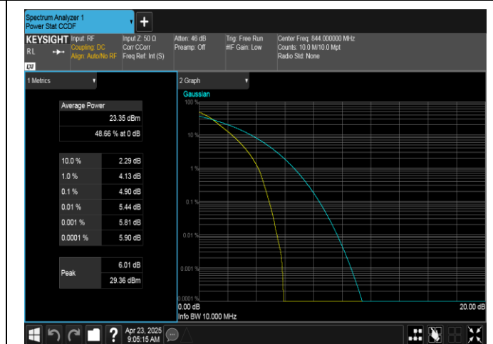
Band5-10MHz-QPSK-20600-50RB#0-PASS
