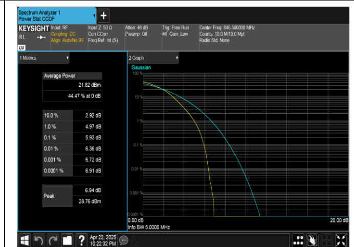
Band5-5MHz-16QAM-20625-25RB#0-PASS
