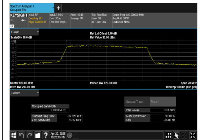
Band5-10MHz-16QAM-20450-50RB#0-PASS
