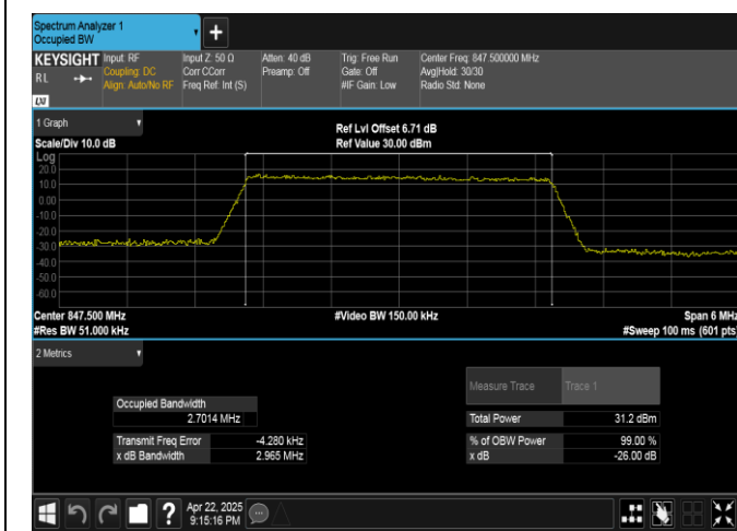
Band5-3MHz-QPSK-20635-15RB#0-PASS
