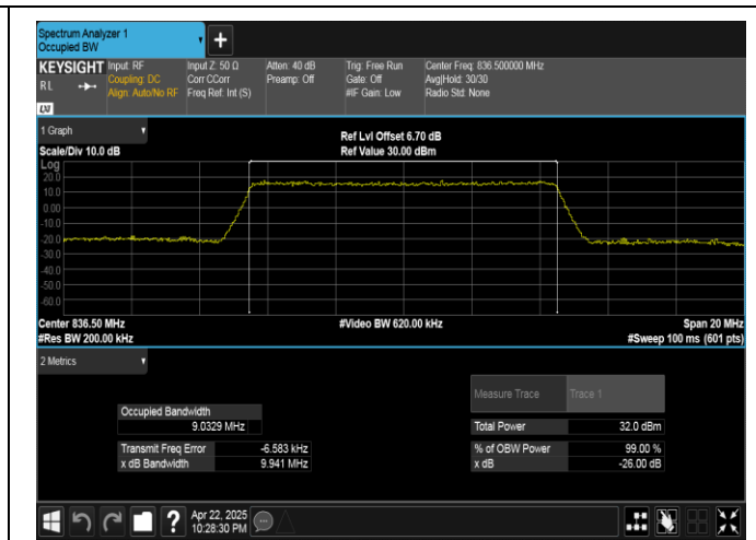
Band5-10MHz-QPSK-20525-50RB#0-PASS
