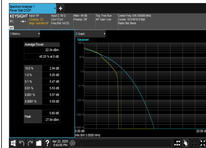
Band5-3MHz-16QAM-20525-1RB#0-PASS
