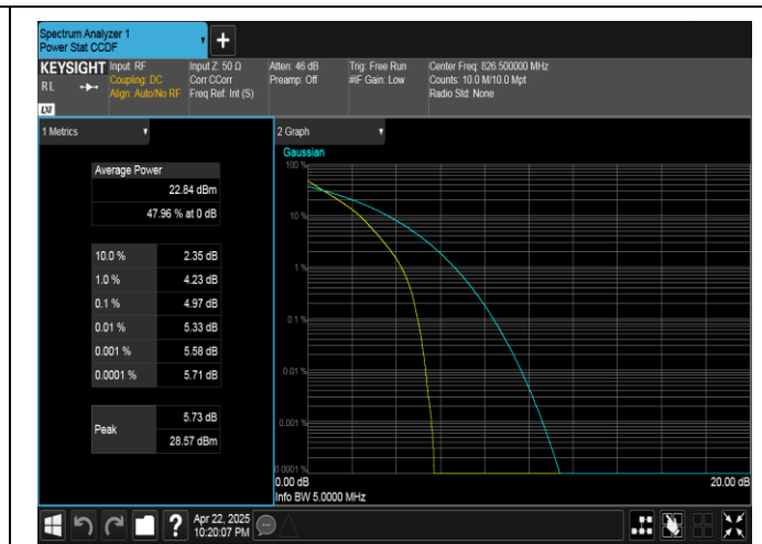
Band5-5MHz-QPSK-20425-25RB#0-PASS
