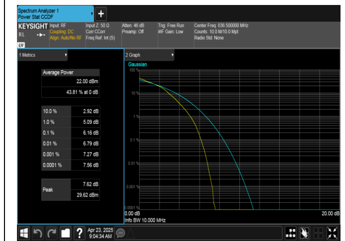
Band5-10MHz-16QAM-20525-50RB#0-PASS
