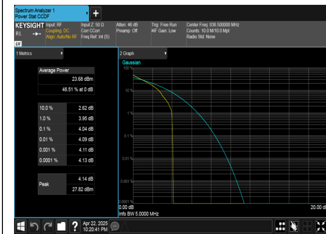
Band5-5MHz-QPSK-20525-1RB#0-PASS
