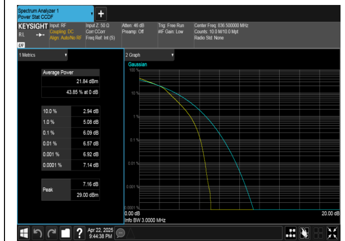
Band5-3MHz-16QAM-20525-15RB#0-PASS
