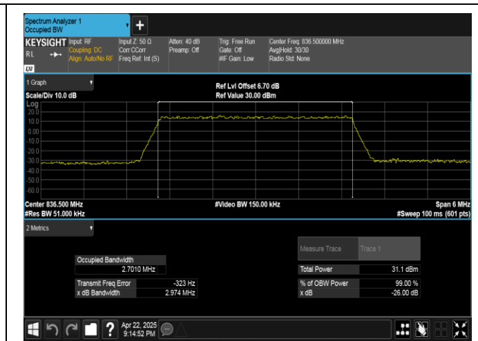
Band5-3MHz-QPSK-20525-15RB#0-PASS
