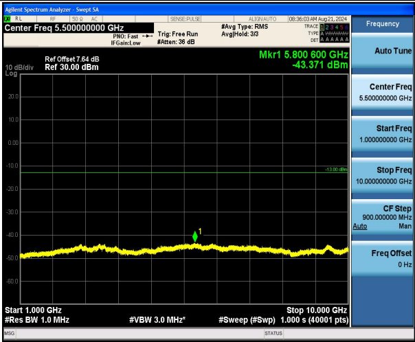
Band17_10MHz_16QAM_23790_1RB#0_1000~10000_1000~10000
