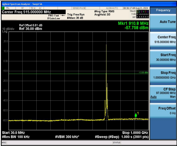
Band17_10MHz_QPSK_23800_1RB#0_30~1000_30~1000
