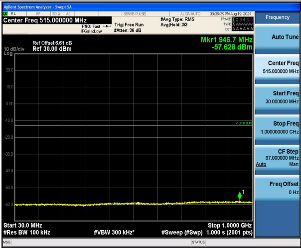
Band2_15MHz_16QAM_18900_1RB#0_30~1000_30~1000
