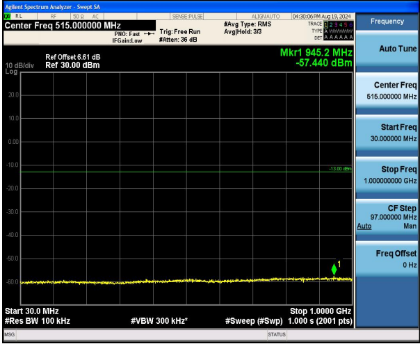
Band4_3MHz_16QAM_19965_1RB#0_30~1000_30~1000
