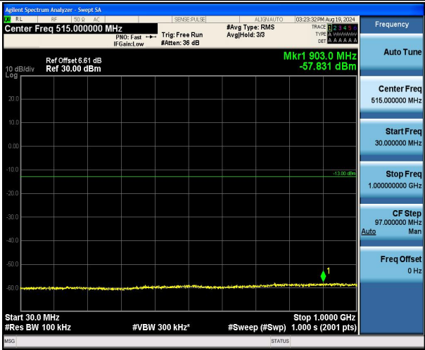
Band2_10MHz_16QAM_19150_1RB#0_30~1000_30~1000
