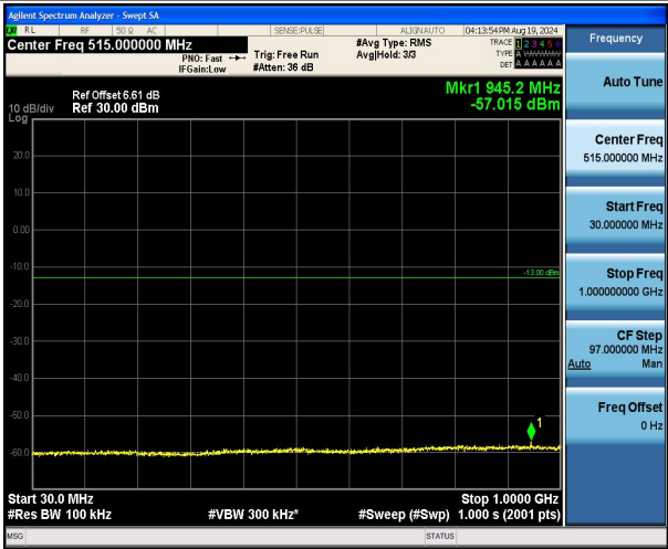
Band4_1.4MHz_QPSK_19957_1RB#0_30~1000_30~1000
