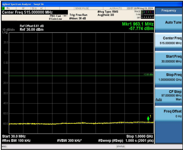
Band2_20MHz_16QAM_18900_1RB#0_30~1000_30~1000
