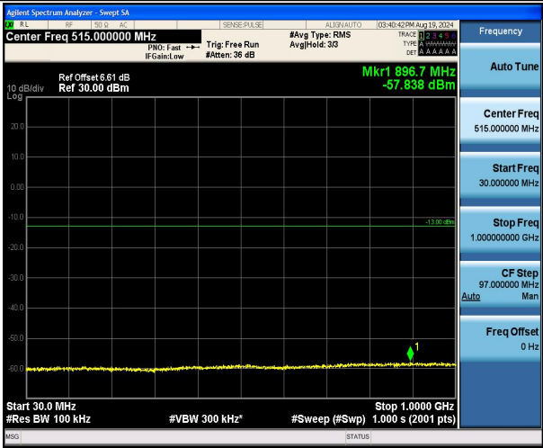
Band2_15MHz_16QAM_19125_1RB#0_30~1000_30~1000
