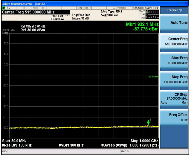
Band4_1.4MHz_QPSK_20393_1RB#0_30~1000_30~1000
