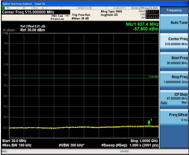
Band2_15MHz_QPSK_19125_1RB#0_30~1000_30~1000
