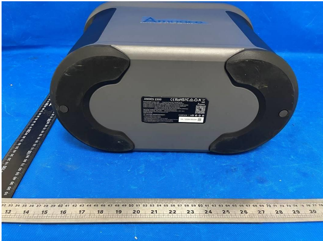
Figure 10 Bottom view
