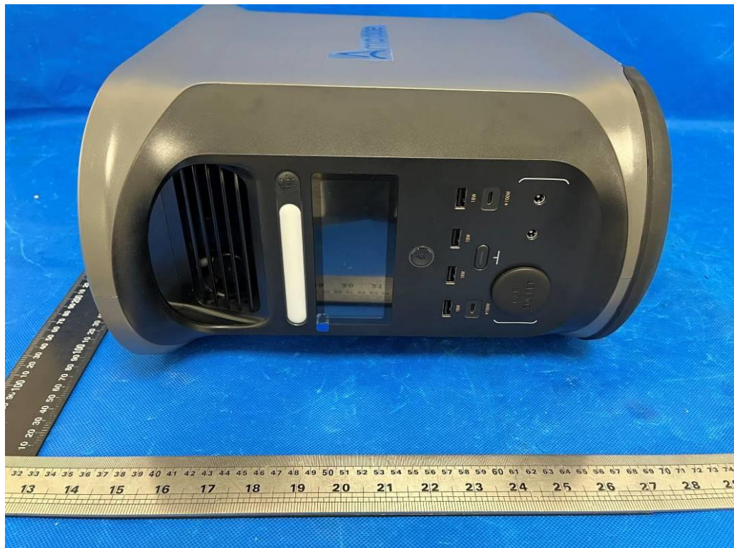
Figure 8 Side view (DC output side)
