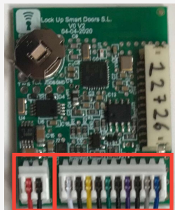
H2 PWR connector 2x1 (cable 2x1) H3 Data Connector 10x1 (cable 10x1)
