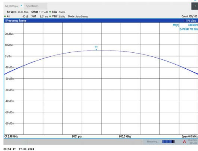
BLE_1M_Ant1_2480
