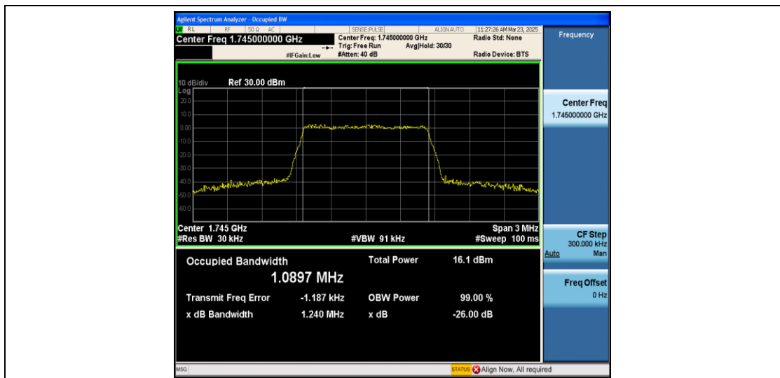
Band66-1.4MHz-16QAM-132322-6RB#0-PASS
