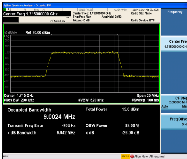
Band66-10MHz-16QAM-131022-50RB#0-PASS
