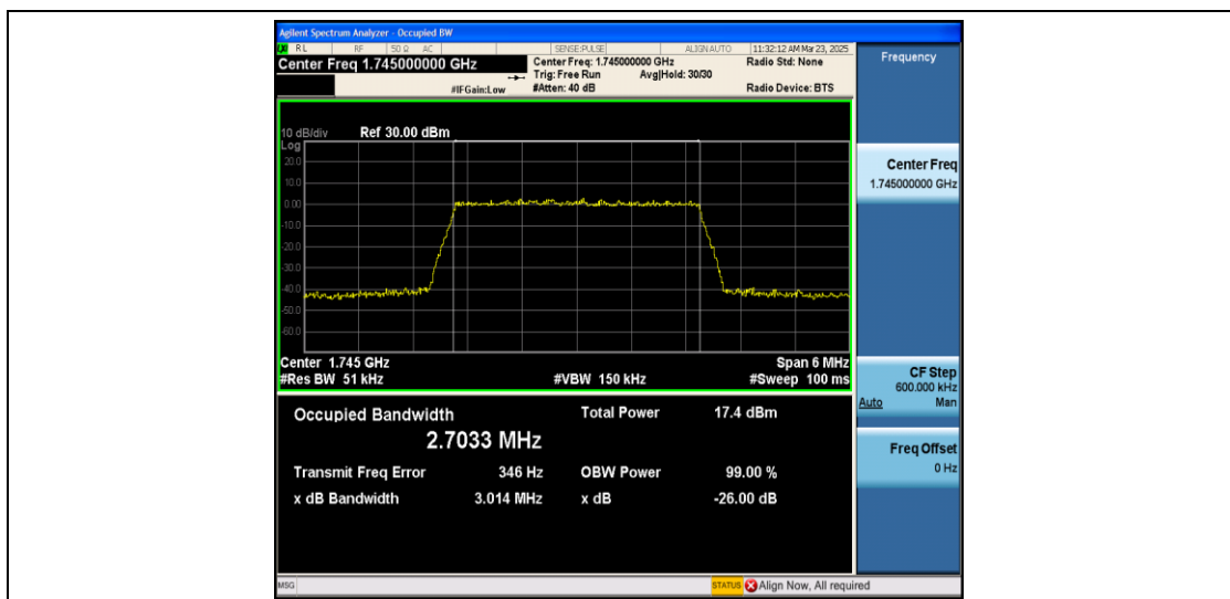
Band66-3MHz-QPSK-132322-15RB#0-PASS
