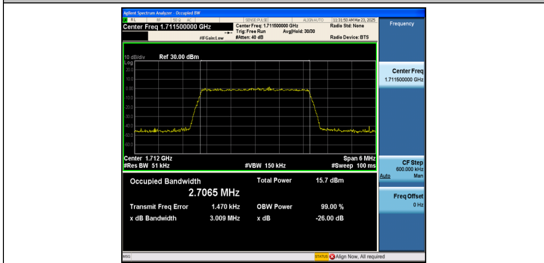
Band66-3MHz-QPSK-131987-15RB#0-PASS
