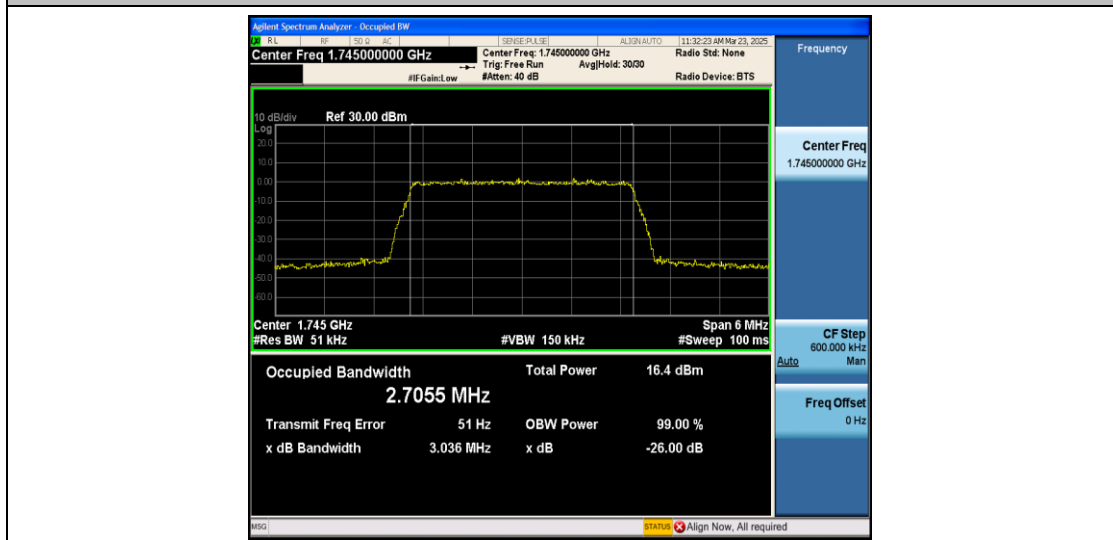
Band66-3MHz-16QAM-132322-15RB#0-PASS
