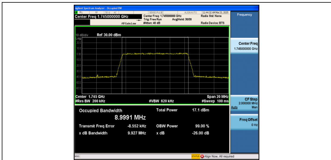
Band66-10MHz-16QAM-132322-50RB#0-PASS
