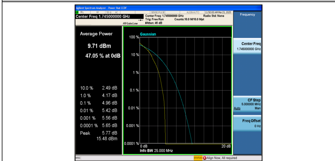
Band66-10MHz-QPSK-132322-1RB#0-PASS
