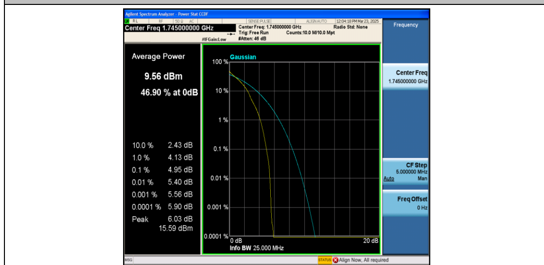
Band66-20MHz-QPSK-132322-1RB#0-PASS
