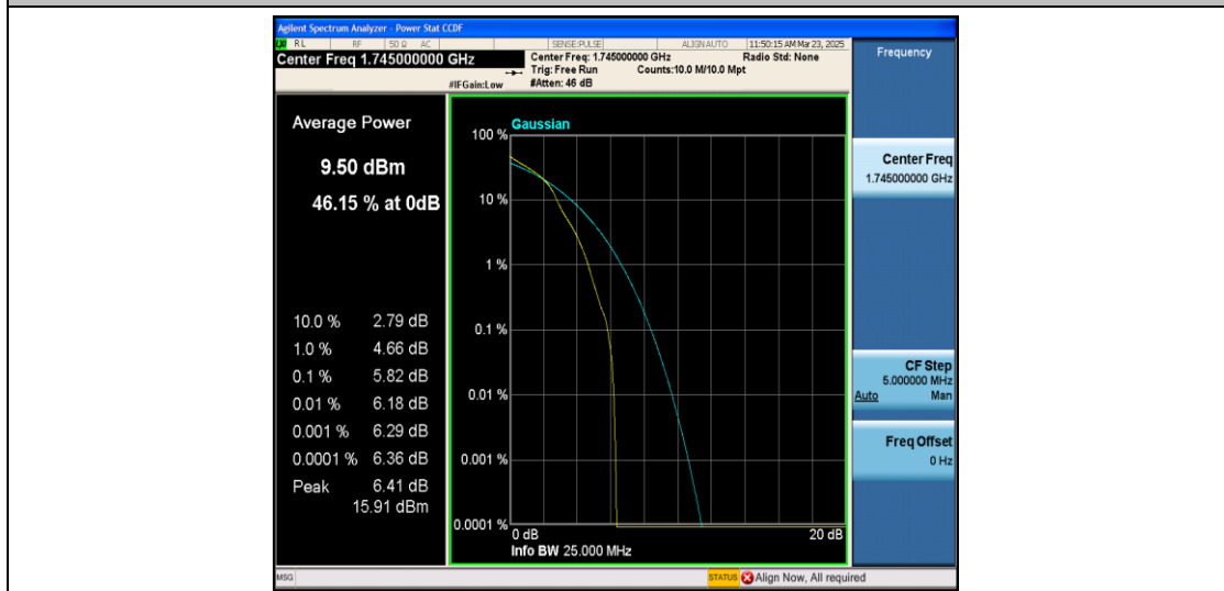
Band66-10MHz-16QAM-132322-1RB#0-PASS
