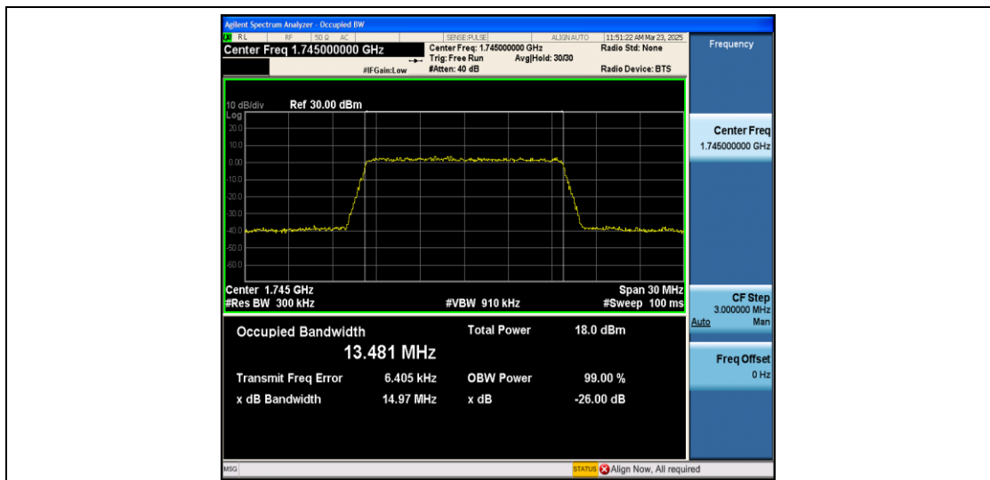
Band66-15MHz-QPSK-132322-75RB#0-PASS
