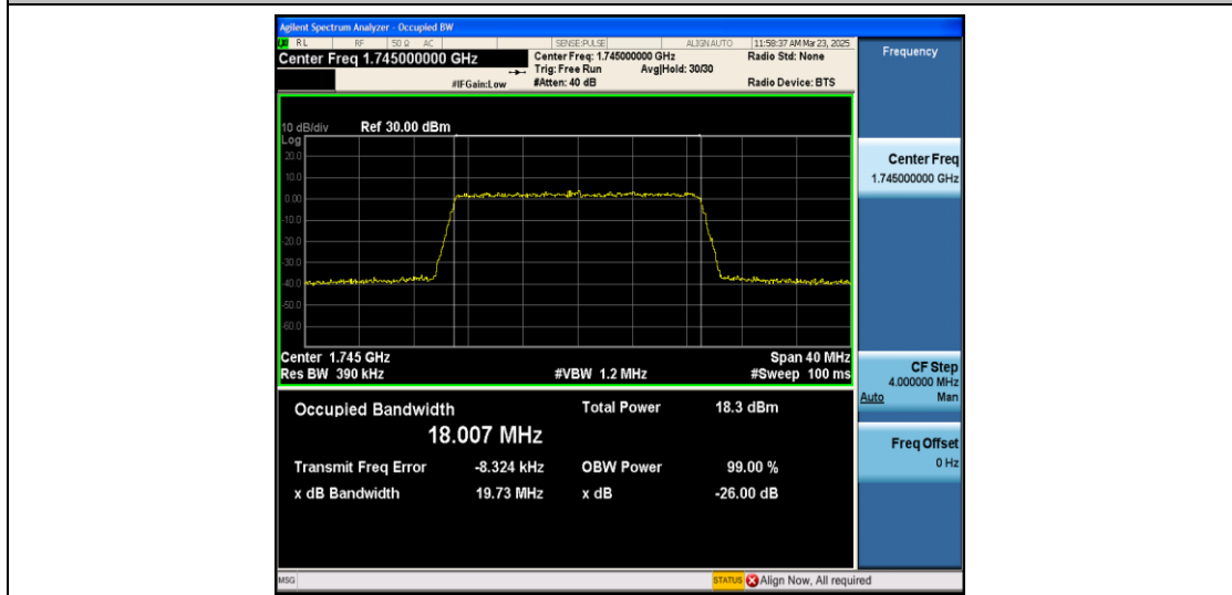
Band66-20MHz-QPSK-132322-100RB#0-PASS
