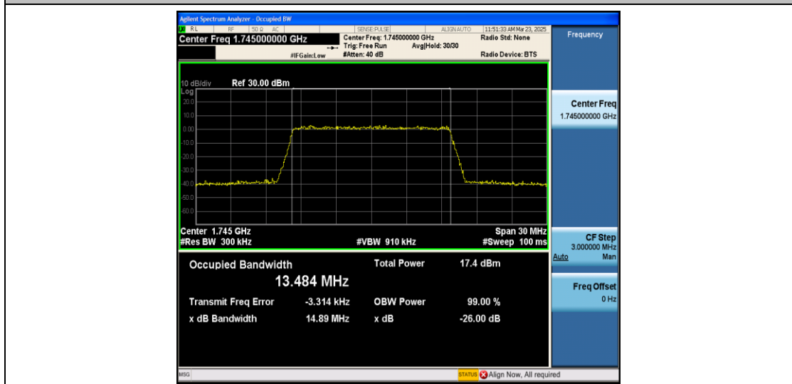
Band66-15MHz-16QAM-132322-75RB#0-PASS
