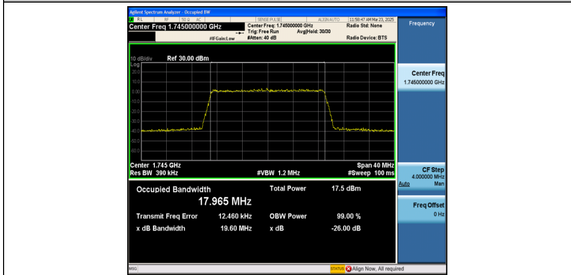
Band66-20MHz-16QAM-132322-100RB#0-PASS
