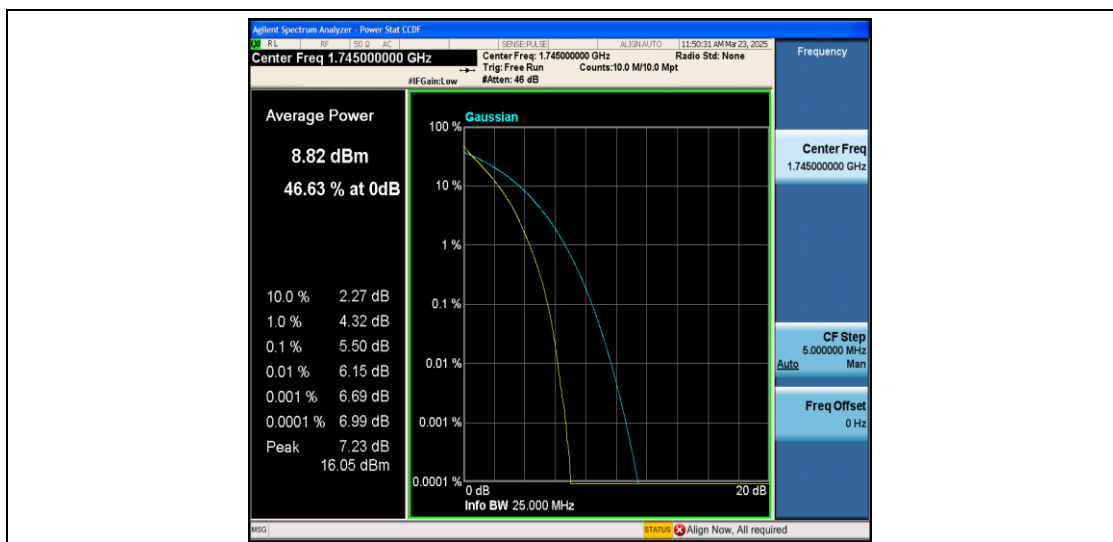
Band66-10MHz-QPSK-132322-50RB#0-PASS
