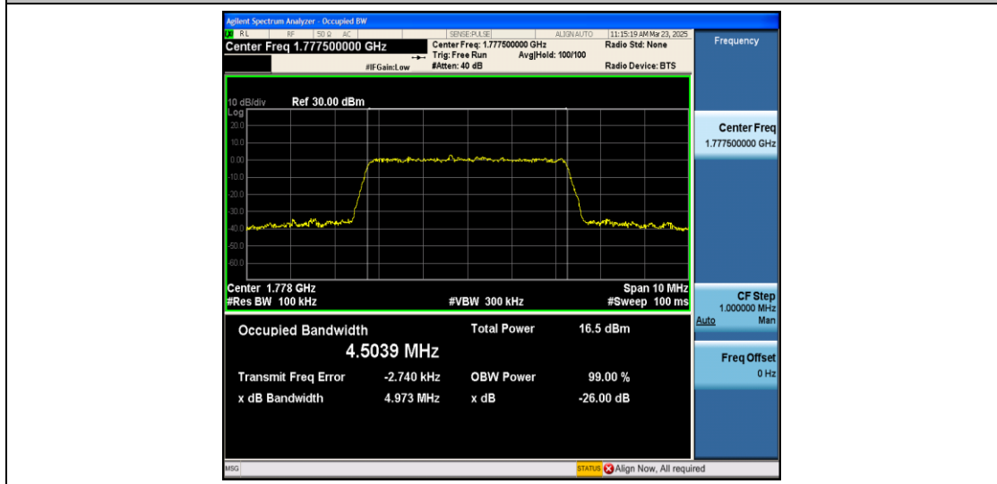
Band66-5MHz-16QAM-132647-25RB#0-PASS
