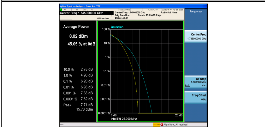
Band66-10MHz-16QAM-132322-50RB#0-PASS
