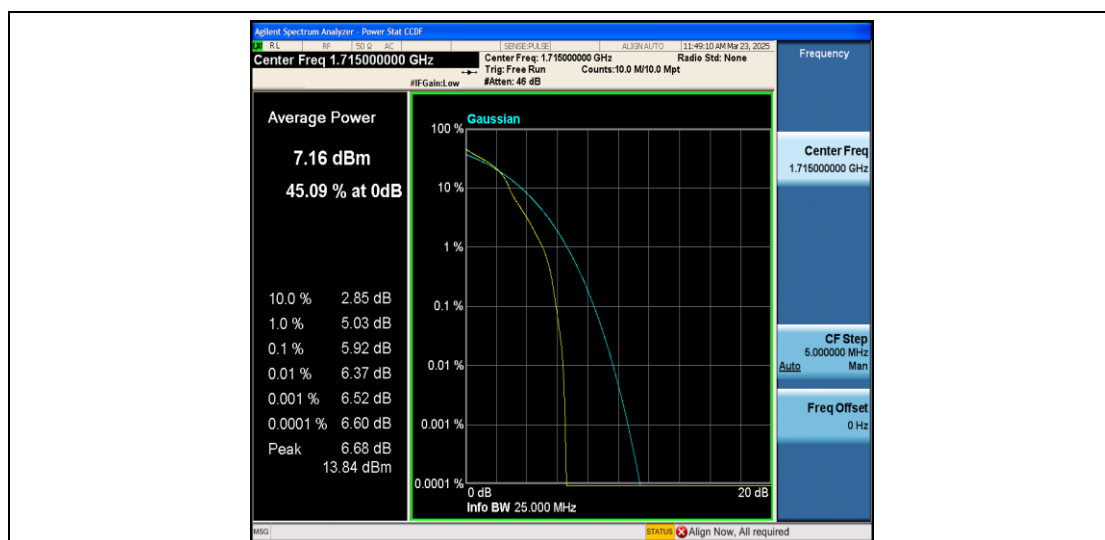
Band66-10MHz-16QAM-131022-1RB#0-PASS
