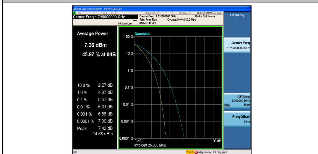
Band66-10MHz-QPSK-131022-50RB#0-PASS
