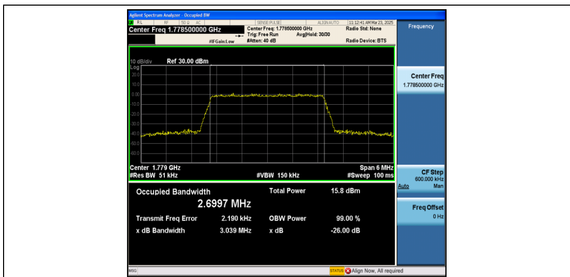
Band66-3MHz-16QAM-132657-15RB#0-PASS
