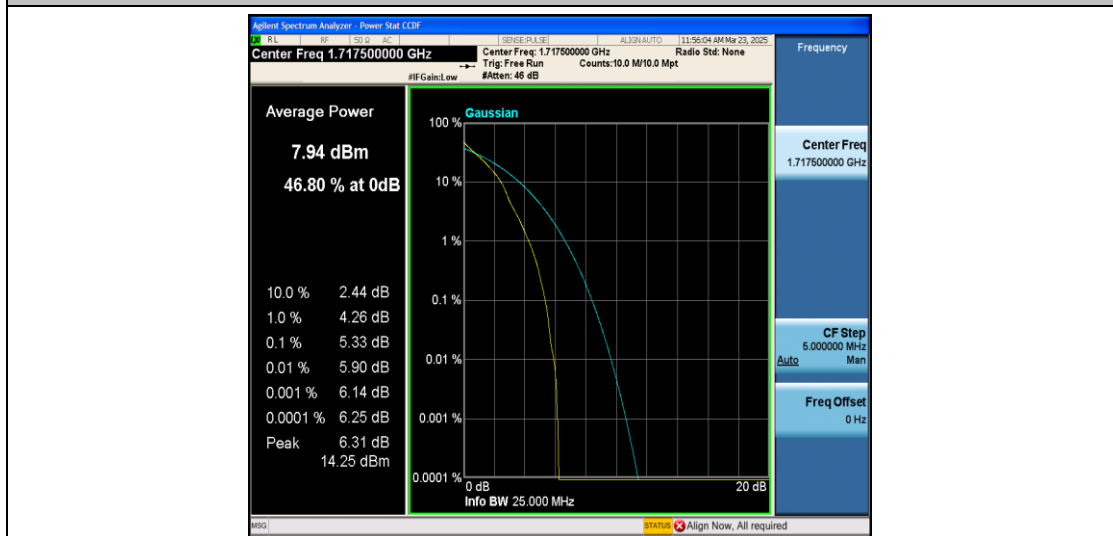
Band66-15MHz-QPSK-131047-1RB#0-PASS
