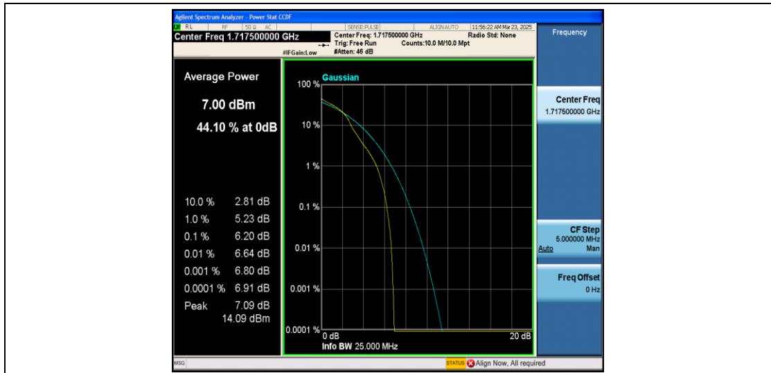
Band66-15MHz-16QAM-131047-1RB#0-PASS
