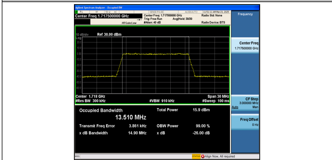
Band66-15MHz-16QAM-131047-75RB#0-PASS
