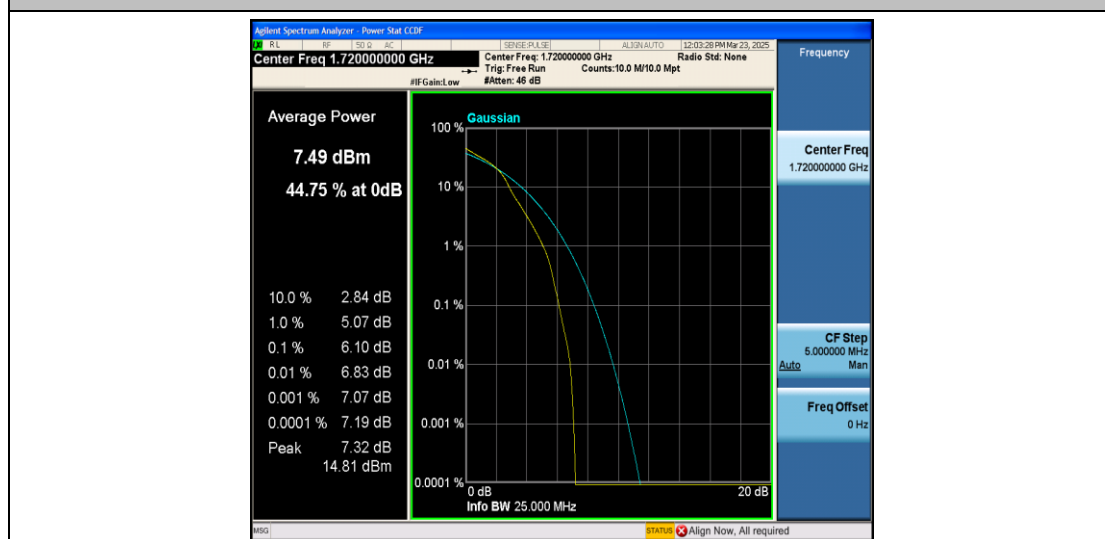
Band66-20MHz-16QAM-132072-1RB#0-PASS
