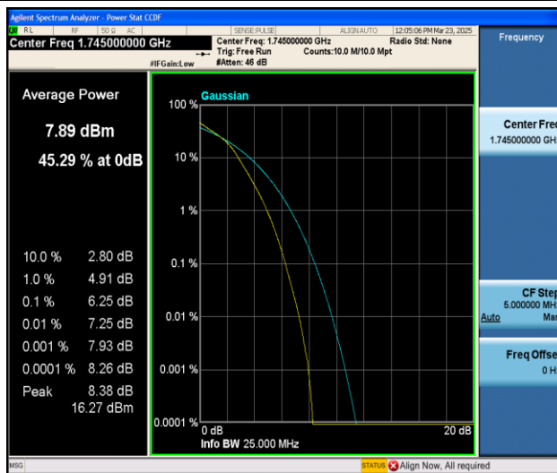
Band66-20MHz-16QAM-132322-100RB#0-PASS
