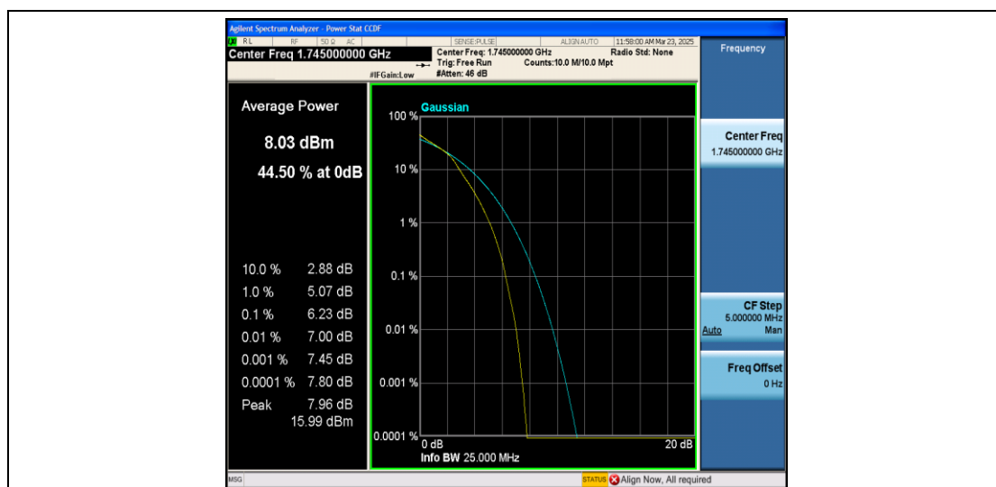
Band66-15MHz-16QAM-132322-75RB#0-PASS
