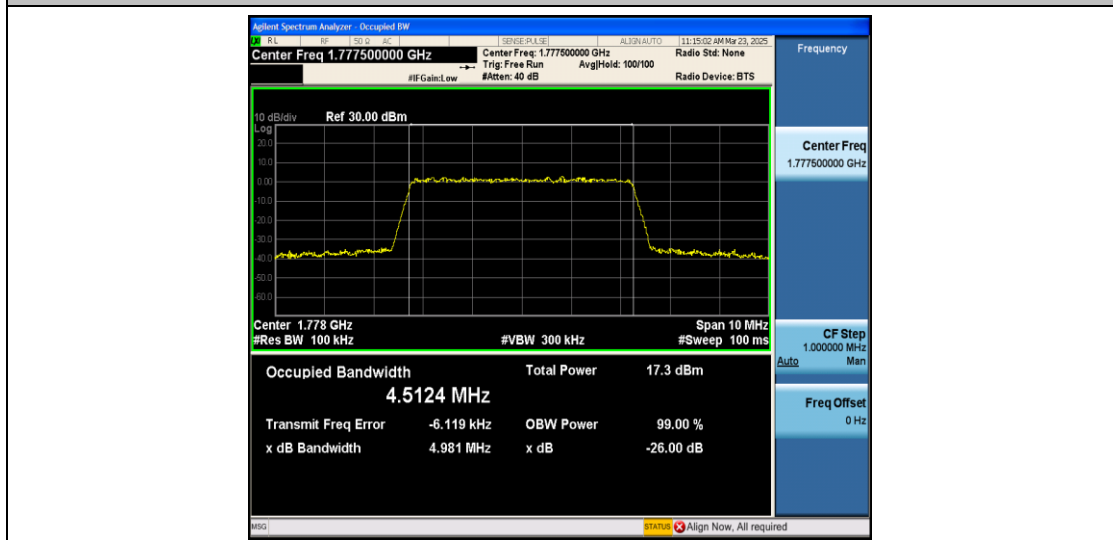
Band66-5MHz-QPSK-132647-25RB#0-PASS
