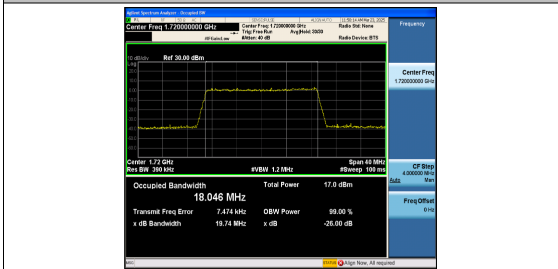
Band66-20MHz-QPSK-132072-100RB#0-PASS
