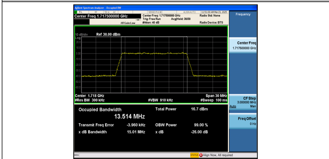
Band66-15MHz-QPSK-131047-75RB#0-PASS
