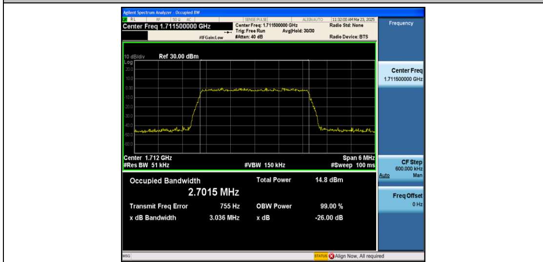
Band66-3MHz-16QAM-131987-15RB#0-PASS
