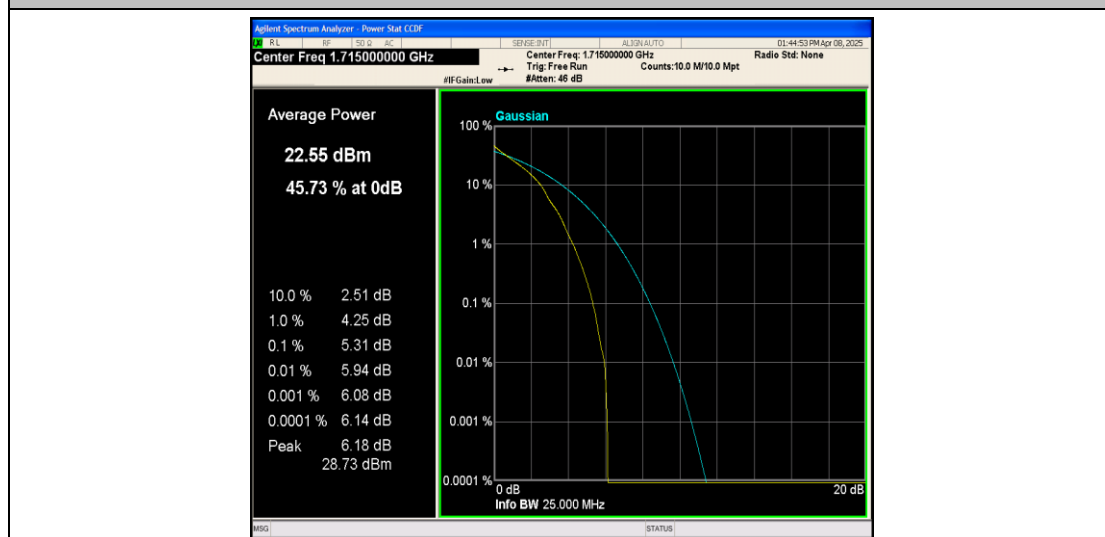
Band66-10MHz-QPSK-131022-1RB#0-PASS
