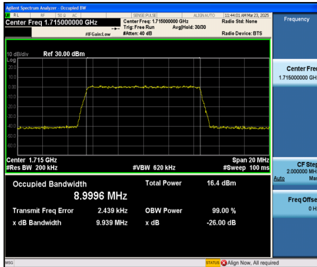
Band66-10MHz-QPSK-131022-50RB#0-PASS
