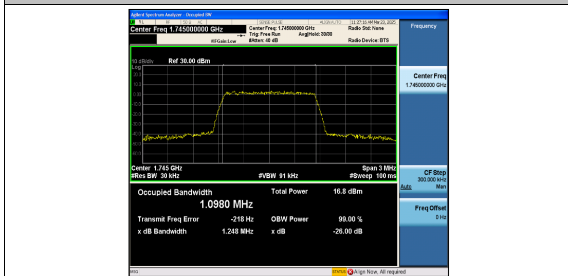
Band66-1.4MHz-QPSK-132322-6RB#0-PASS
