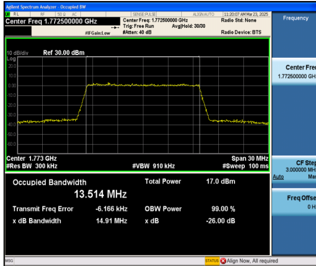
Band66-15MHz-16QAM-132597-75RB#0-PASS
