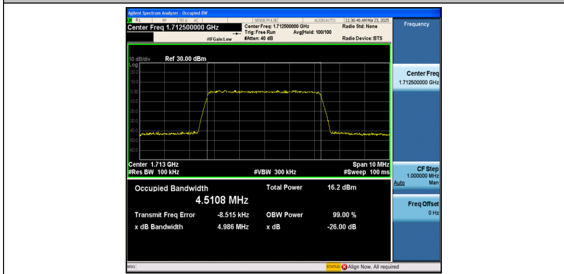
Band66-5MHz-QPSK-131997-25RB#0-PASS
