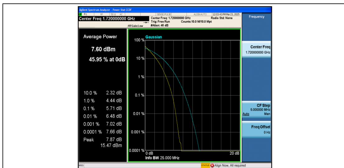
Band66-20MHz-QPSK-132072-100RB#0-PASS
