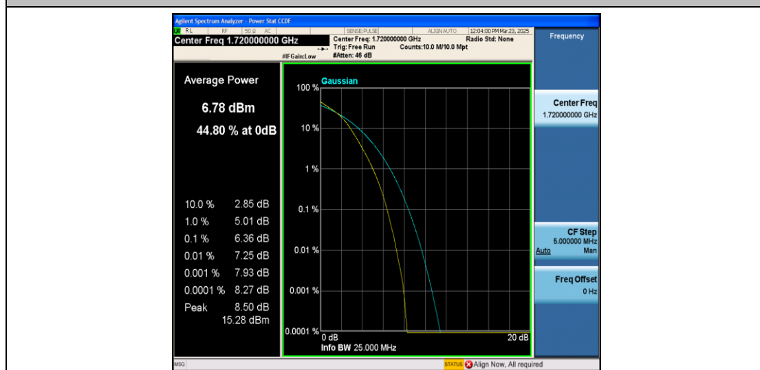
Band66-20MHz-16QAM-132072-100RB#0-PASS
