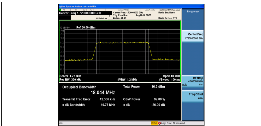
Band66-20MHz-16QAM-132072-100RB#0-PASS
