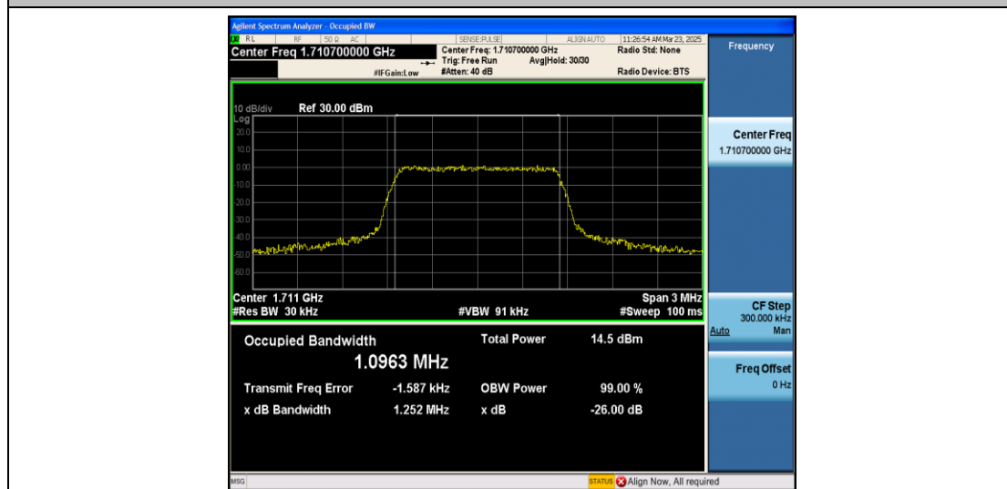
Band66-1.4MHz-16QAM-131979-6RB#0-PASS
