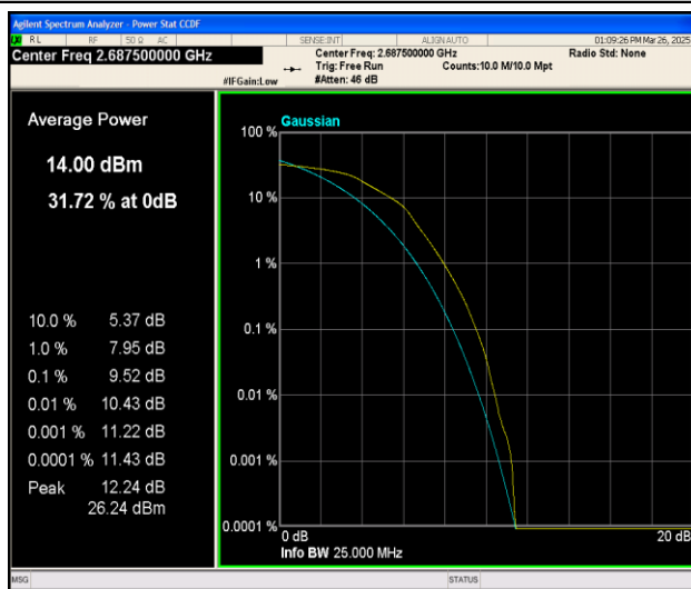
Band41-5MHz-16QAM-41565-25RB#0-PASS
