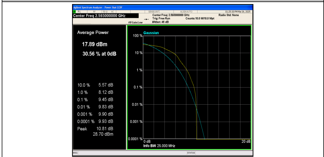
Band41-10MHz-16QAM-40620-1RB#0-PASS
