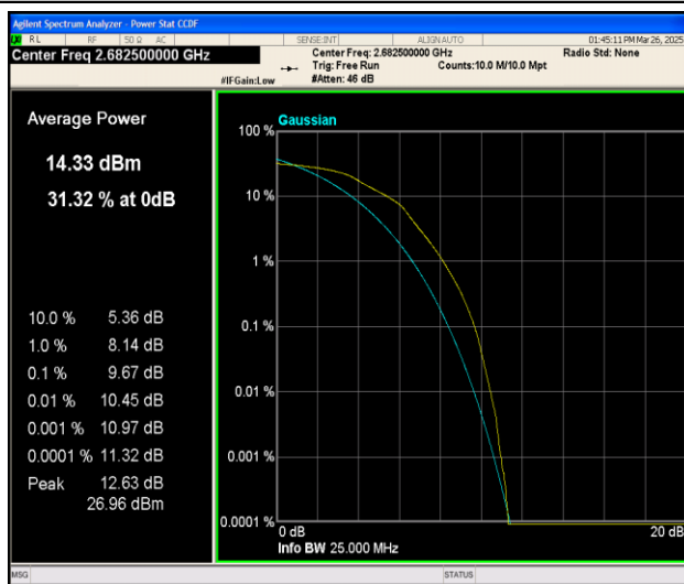
Band41-15MHz-16QAM-41515-75RB#0-PASS
