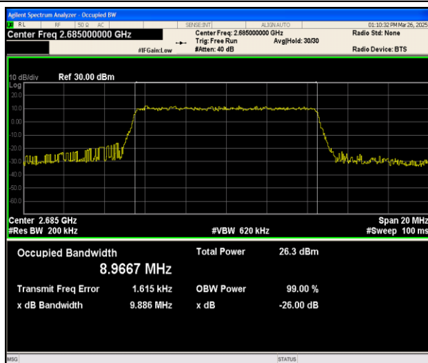
Band41-10MHz-16QAM-41540-50RB#0-PASS
