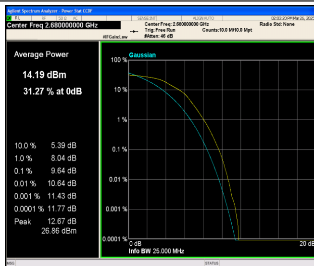
Band41-20MHz-16QAM-41490-100RB#0-PASS
