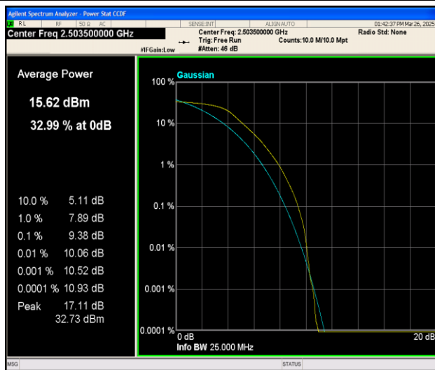
Band41-15MHz-QPSK-39725-75RB#0-PASS
