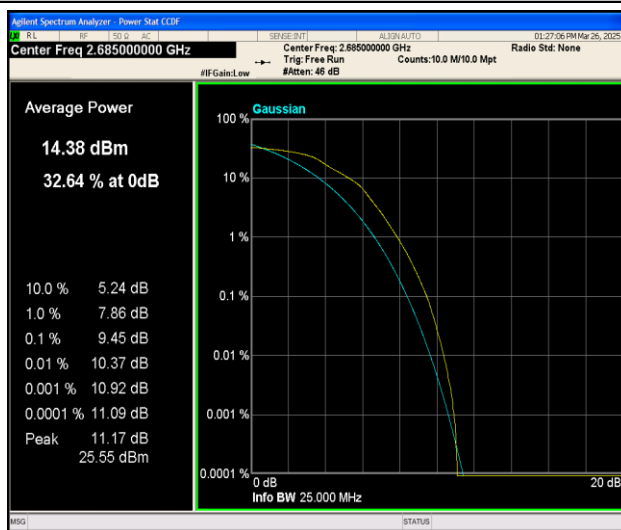
Band41-10MHz-16QAM-41540-50RB#0-PASS
