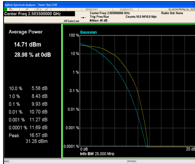
Band41-15MHz-16QAM-39725-75RB#0-PASS
