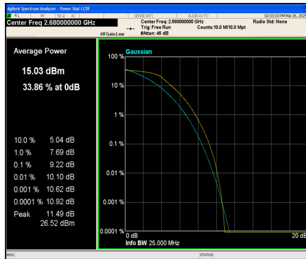
Band41-20MHz-QPSK-41490-100RB#0-PASS
