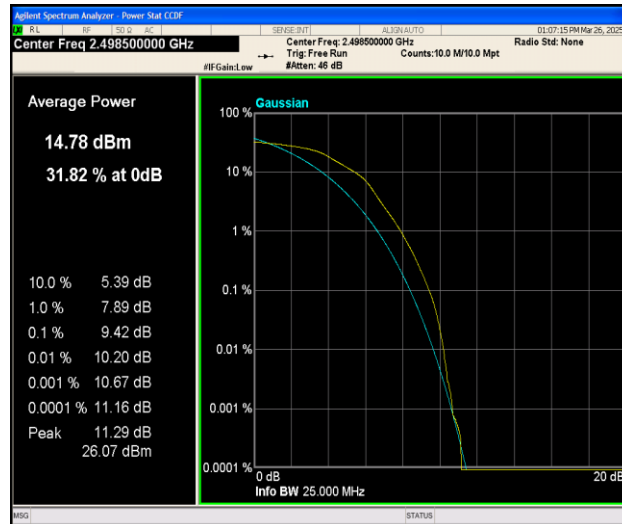
Band41-5MHz-16QAM-39675-25RB#0-PASS
