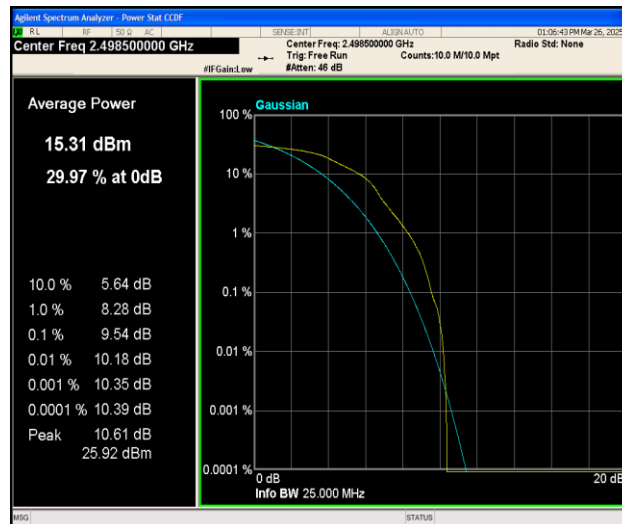
Band41-5MHz-16QAM-39675-1RB#0-PASS
