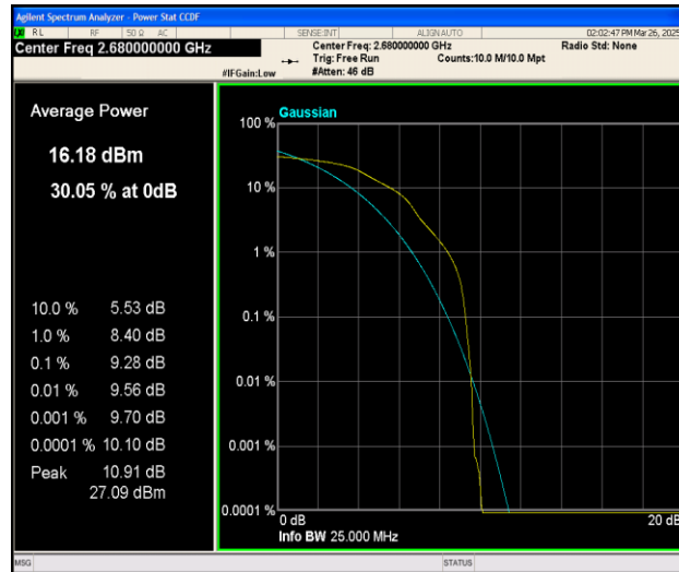
Band41-20MHz-16QAM-41490-1RB#0-PASS
