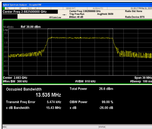
Band41-15MHz-16QAM-41515-75RB#0-PASS
