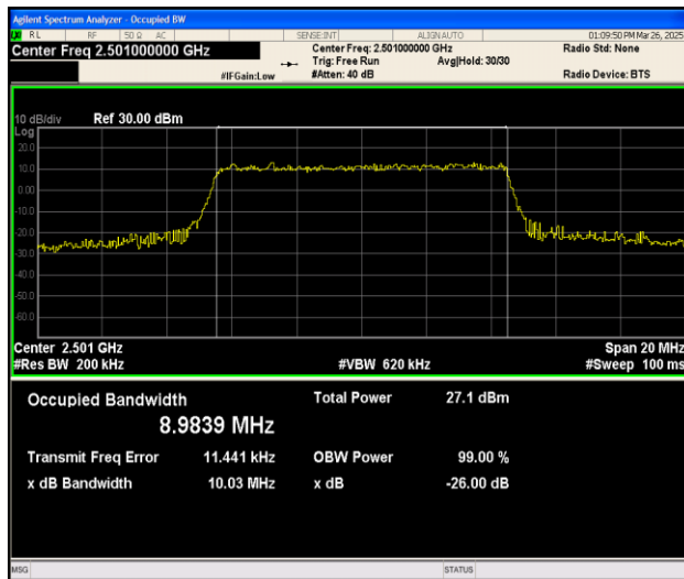
Band41-10MHz-16QAM-39700-50RB#0-PASS
