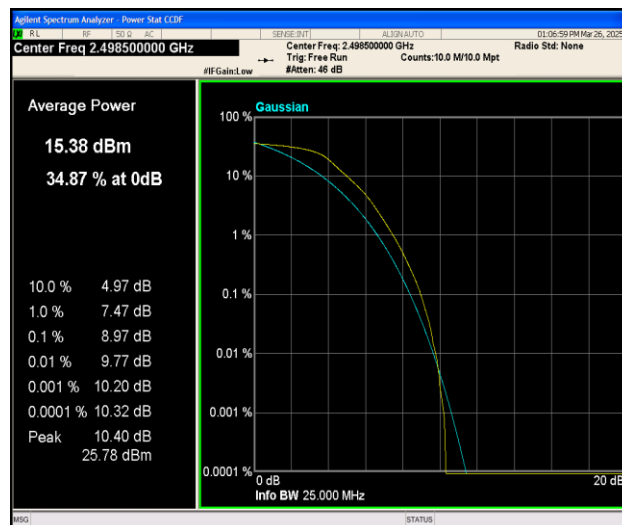
Band41-5MHz-QPSK-39675-25RB#0-PASS
