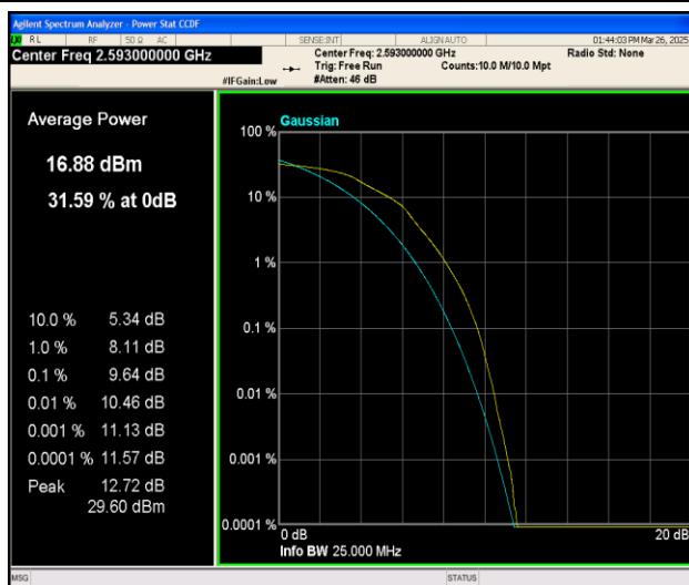
Band41-15MHz-16QAM-40620-75RB#0-PASS
