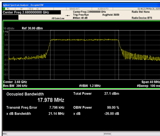
Band41-20MHz-16QAM-41490-100RB#0-PASS
