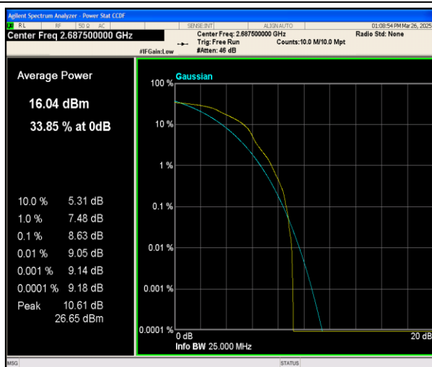
Band41-5MHz-16QAM-41565-1RB#0-PASS
