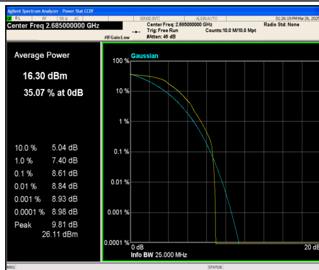
Band41-10MHz-QPSK-41540-1RB#0-PASS
