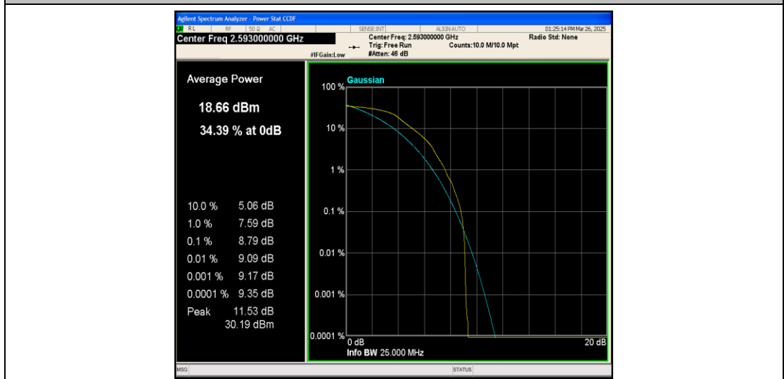
Band41-10MHz-QPSK-40620-1RB#0-PASS
