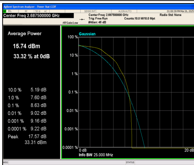
Band41-5MHz-QPSK-41565-1RB#0-PASS
