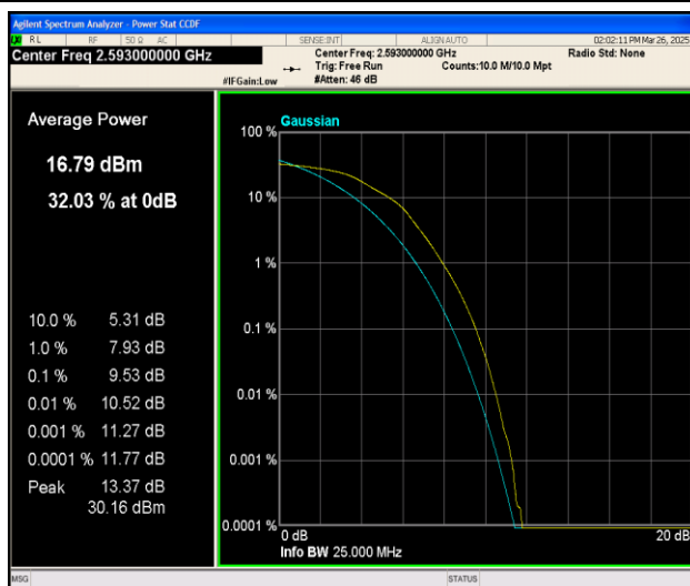
Band41-20MHz-16QAM-40620-100RB#0-PASS
