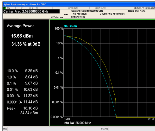
Band41-10MHz-16QAM-40620-50RB#0-PASS
