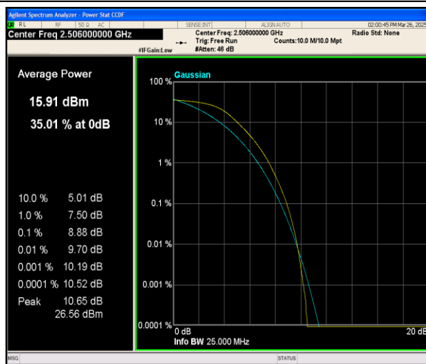
Band41-20MHz-QPSK-39750-100RB#0-PASS
