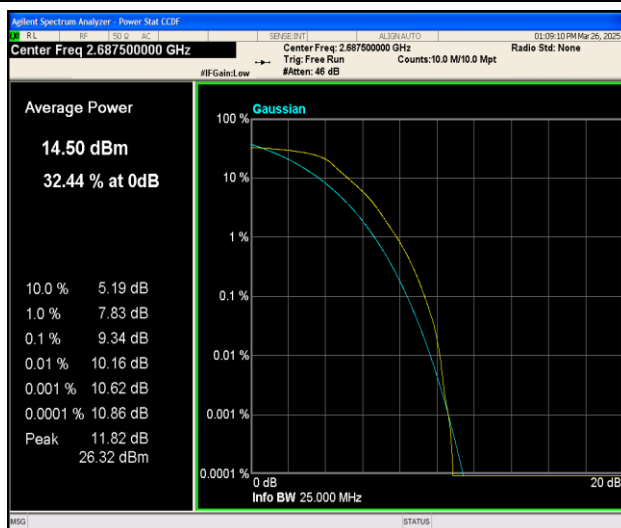
Band41-5MHz-QPSK-41565-25RB#0-PASS
