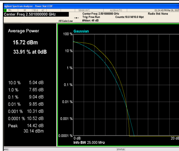
Band41-10MHz-QPSK-39700-50RB#0-PASS
