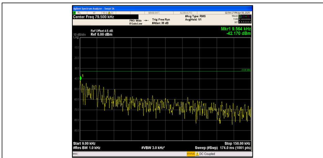
Band26_3MHz_16QAM_26915_1RB#0_0.009~0.15_0.009~0.15
