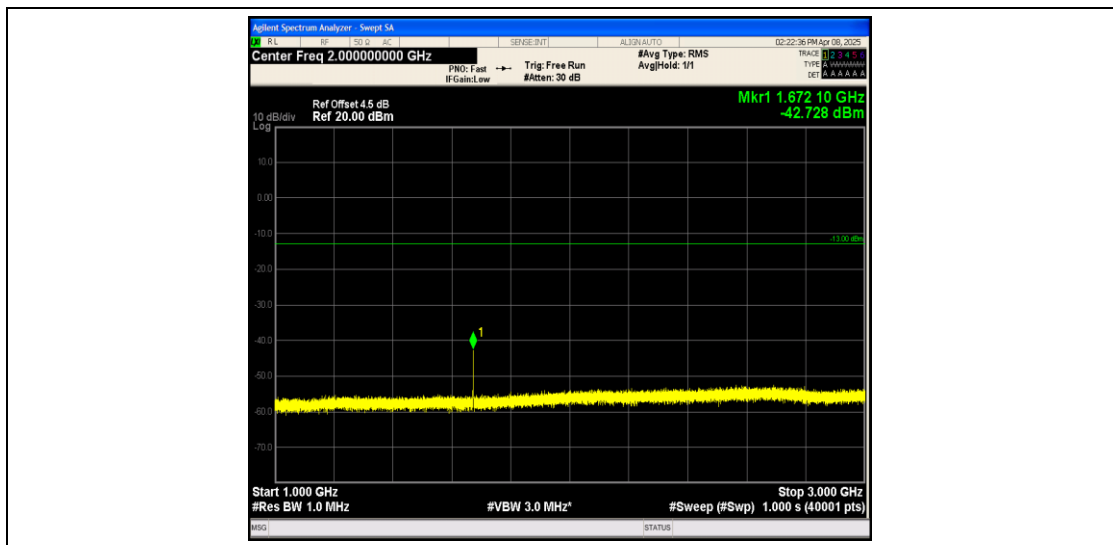
Band26_1.4MHz_16QAM_26915_1RB#0_1000~3000_1000~3000
