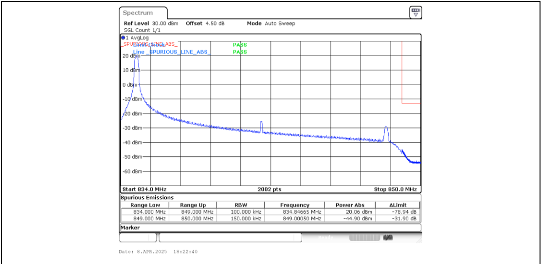
Band26_15MHz_QPSK_26965_1RB#0
