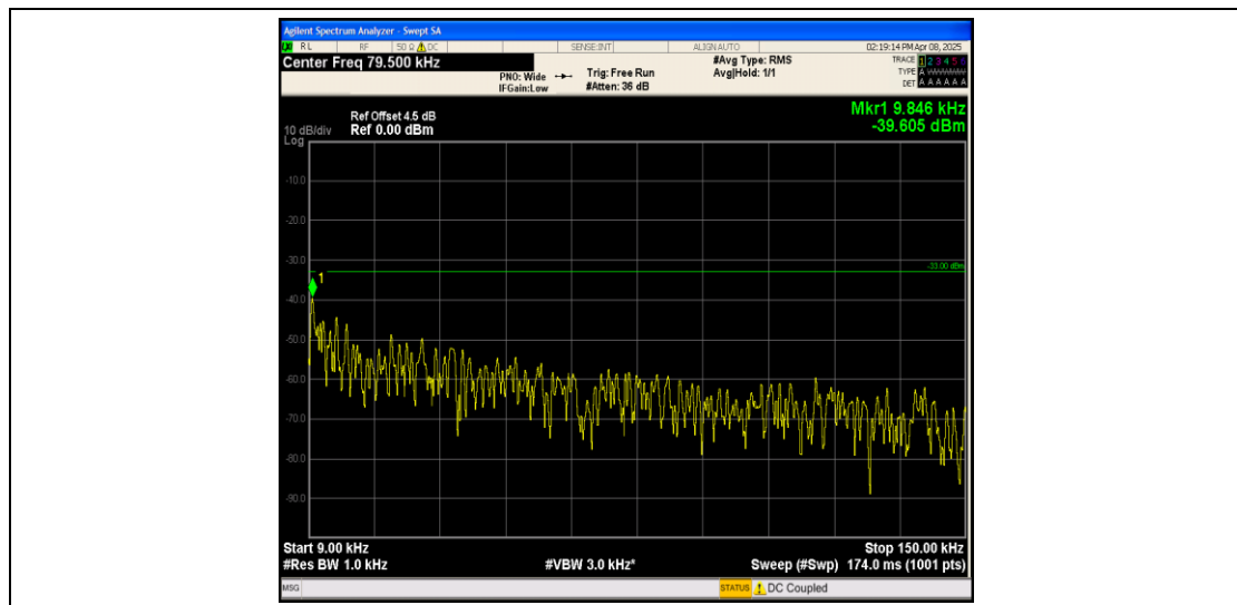
Band26_1.4MHz_QPSK_26797_1RB#0_0.009~0.15_0.009~0.15
