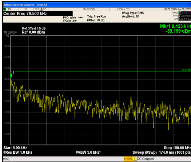
Band26_3MHz_QPSK_26805_1RB#0_0.009~0.15_0.009~0.15
