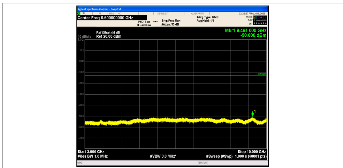
Band26_1.4MHz_QPSK_27033_1RB#0_3000~10000_3000~10000
