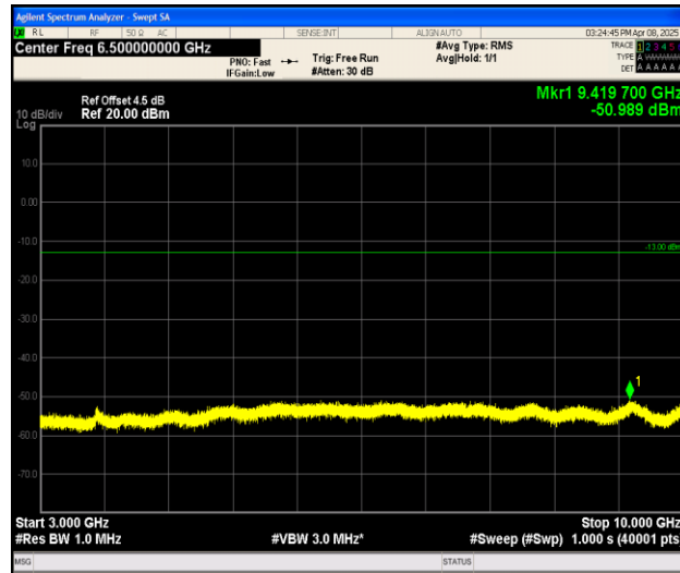
Band26_5MHz_16QAM_26815_1RB#0_3000~10000_3000~10000
