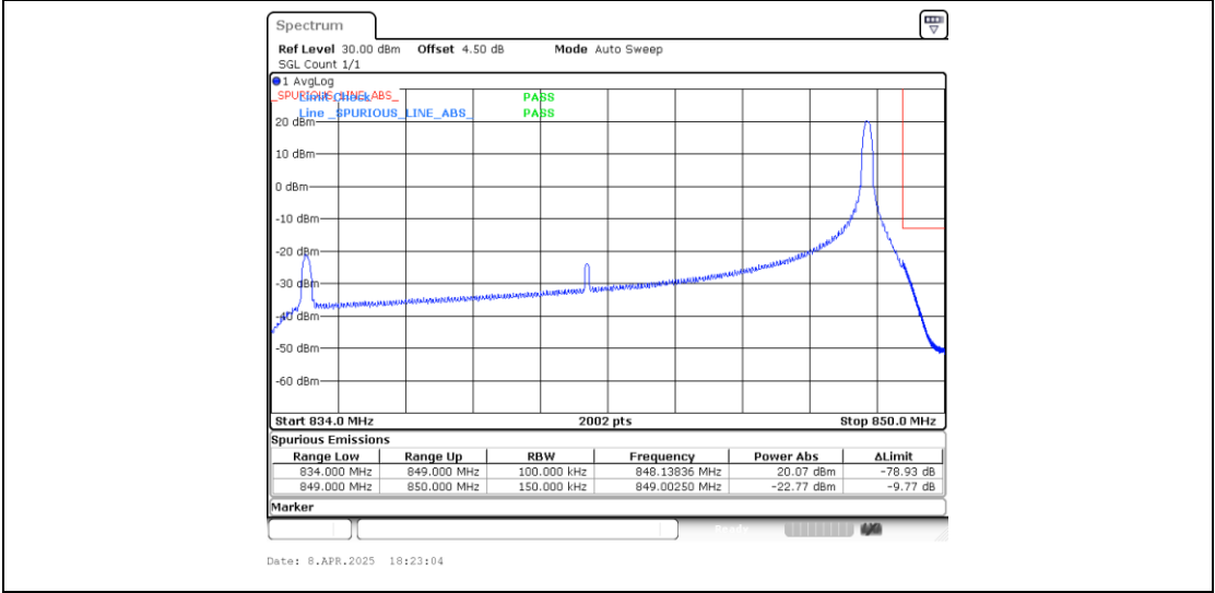
Band26_15MHz_QPSK_26965_1RB#74
