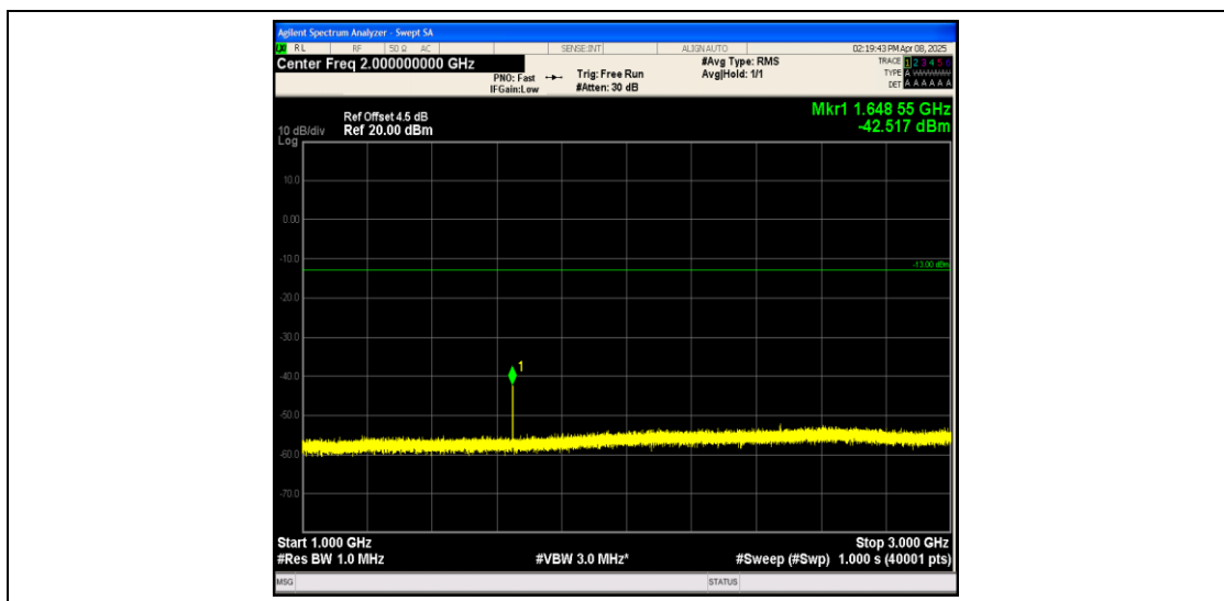
Band26_1.4MHz_QPSK_26797_1RB#0_1000~3000_1000~3000
