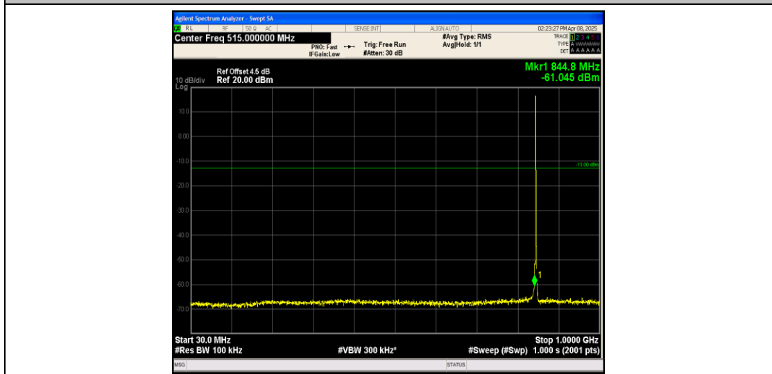
Band26_1.4MHz_QPSK_27033_1RB#0_30~1000_30~1000
