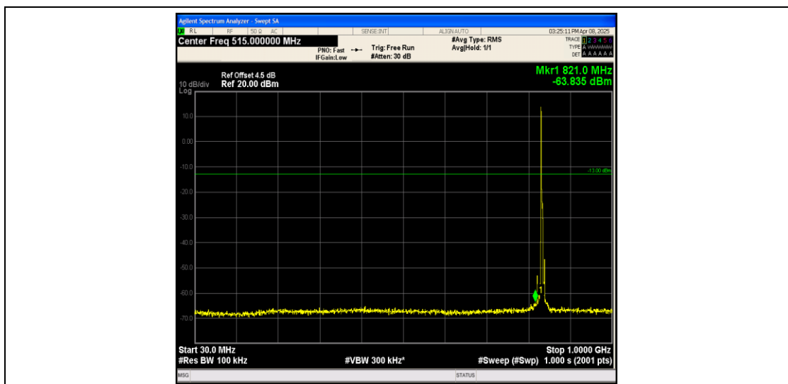
Band26_5MHz_QPSK_26915_1RB#0_30~1000_30~1000
