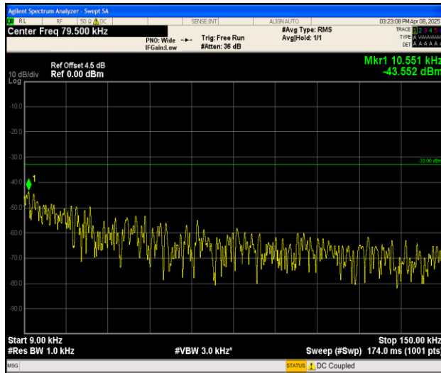
Band26_5MHz_QPSK_26815_1RB#0_0.009~0.15_0.009~0.15
