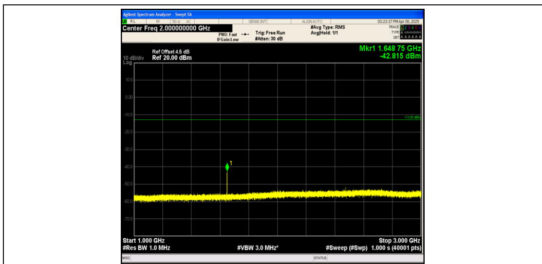
Band26_5MHz_QPSK_26815_1RB#0_1000~3000_1000~3000
