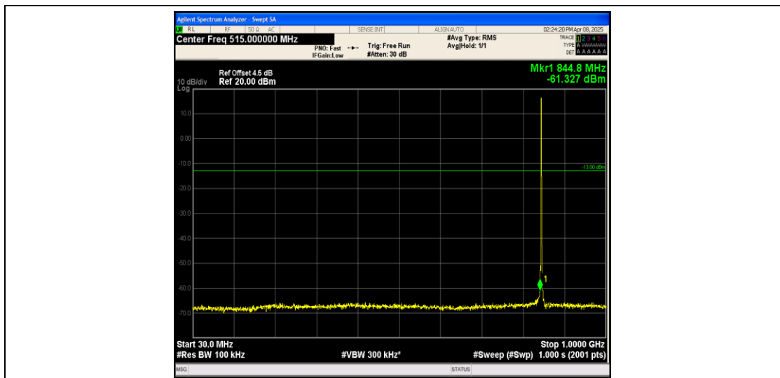
Band26_1.4MHz_16QAM_27033_1RB#0_30~1000_30~1000
