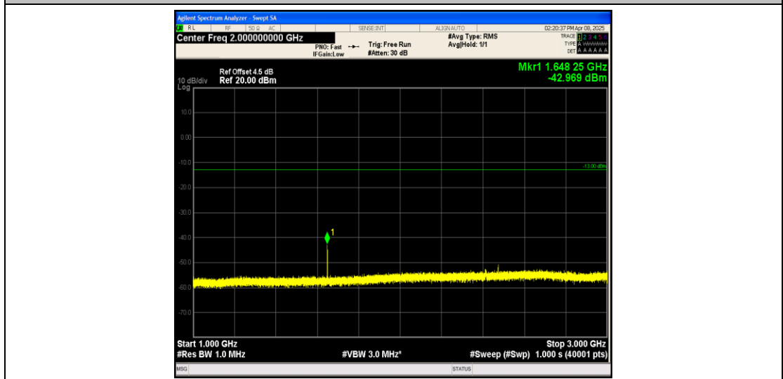
Band26_1.4MHz_16QAM_26797_1RB#0_1000~3000_1000~3000
