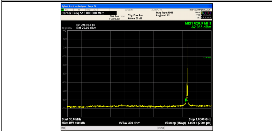
Band26_3MHz_16QAM_26915_1RB#0_30~1000_30~1000
