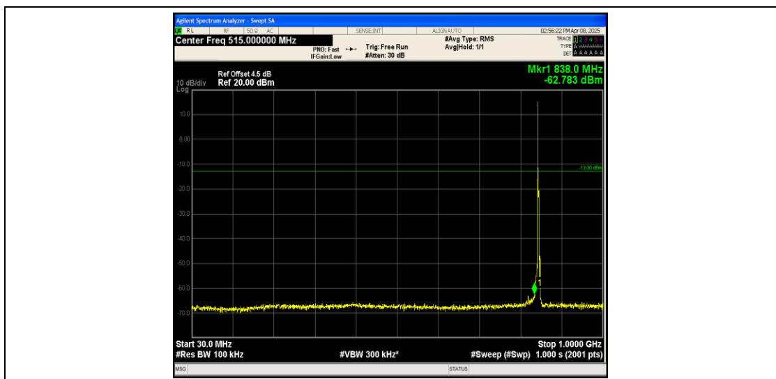
Band26_3MHz_16QAM_27025_1RB#0_30~1000_30~1000
