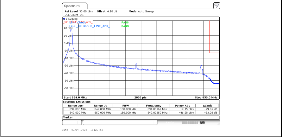
Band26_15MHz_16QAM_26965_1RB#0
