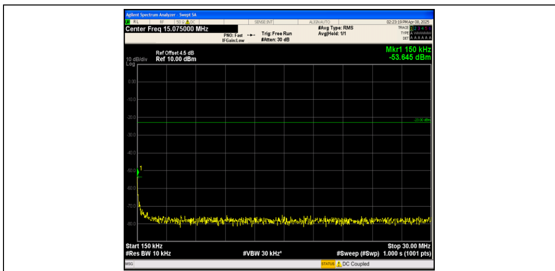
Band26_1.4MHz_QPSK_27033_1RB#0_0.15~30_0.15~30
