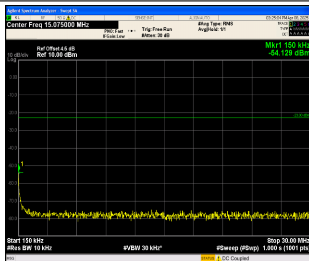
Band26_5MHz_QPSK_26915_1RB#0_0.15~30_0.15~30
