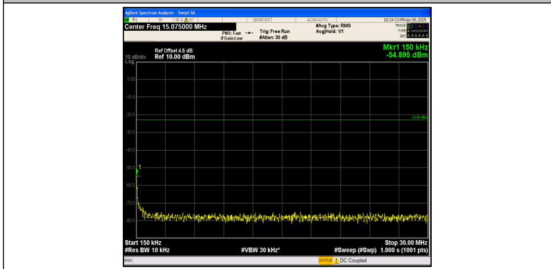
Band26_1.4MHz_16QAM_27033_1RB#0_0.15~30_0.15~30
