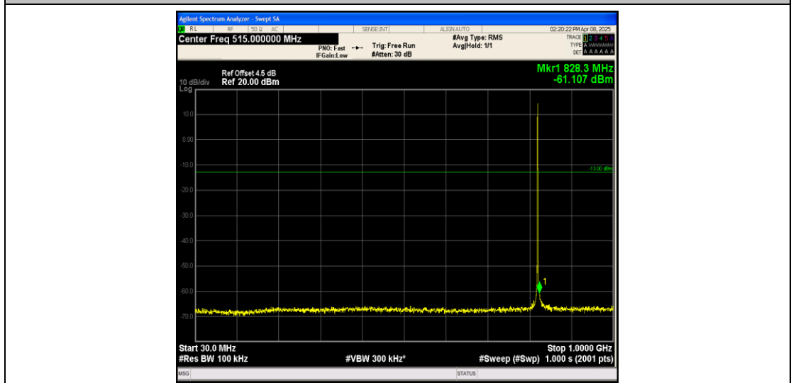
Band26_1.4MHz_16QAM_26797_1RB#0_30~1000_30~1000
