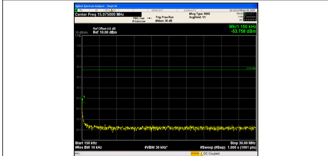
Band26_1.4MHz_QPSK_26797_1RB#0_0.15~30_0.15~30
