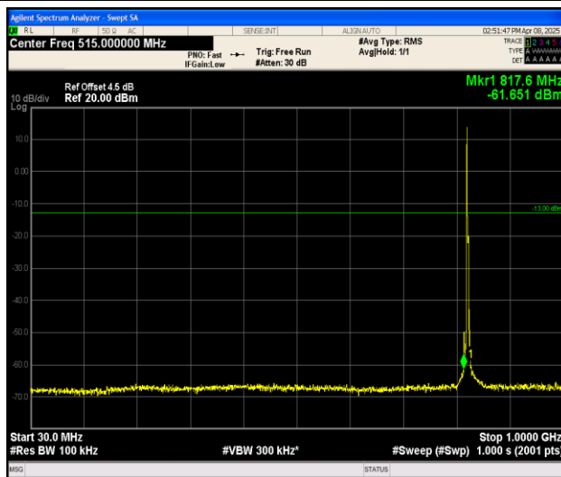
Band26_3MHz_QPSK_26805_1RB#0_30~1000_30~1000
