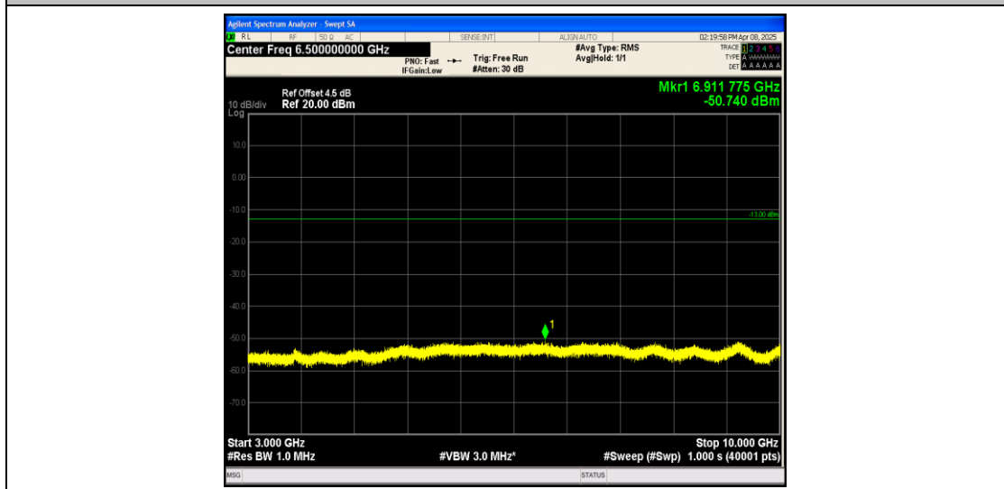
Band26_1.4MHz_QPSK_26797_1RB#0_3000~10000_3000~10000
