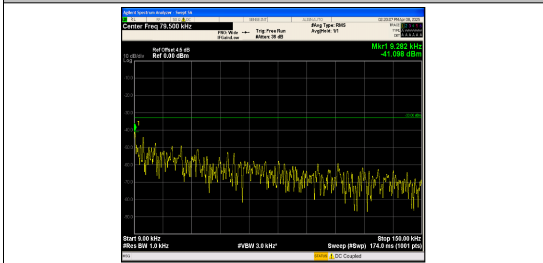
Band26_1.4MHz_16QAM_26797_1RB#0_0.009~0.15_0.009~0.15
