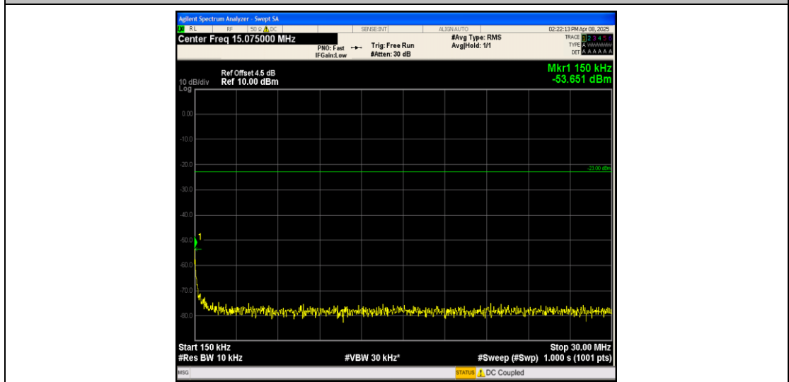
Band26_1.4MHz_16QAM_26915_1RB#0_0.15~30_0.15~30
