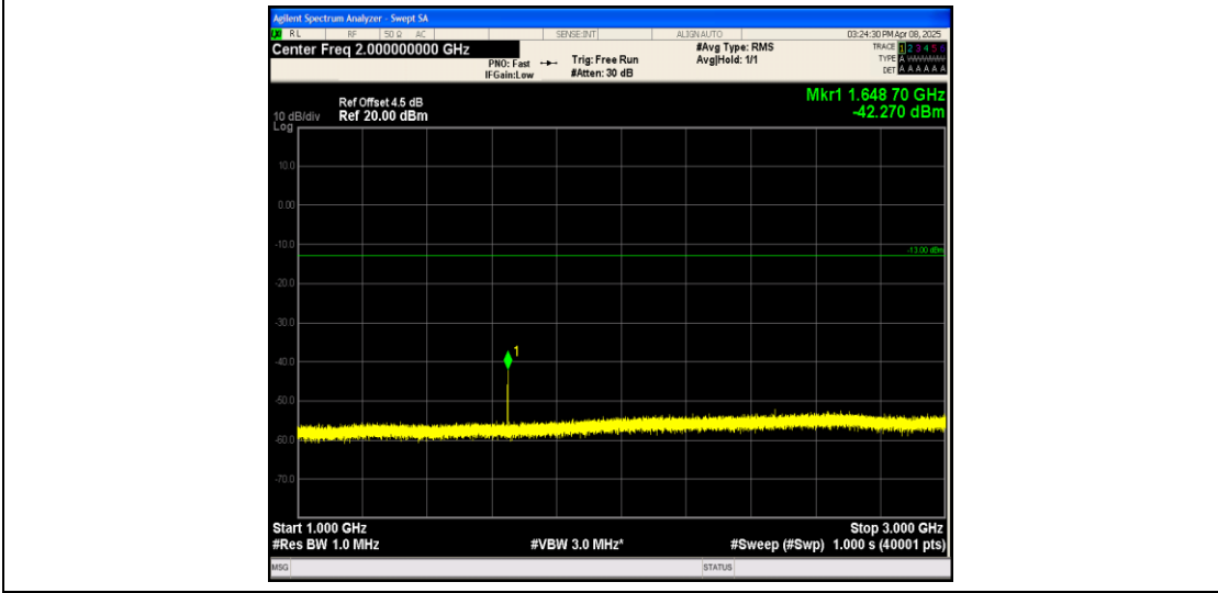
Band26_5MHz_16QAM_26815_1RB#0_1000~3000_1000~3000
