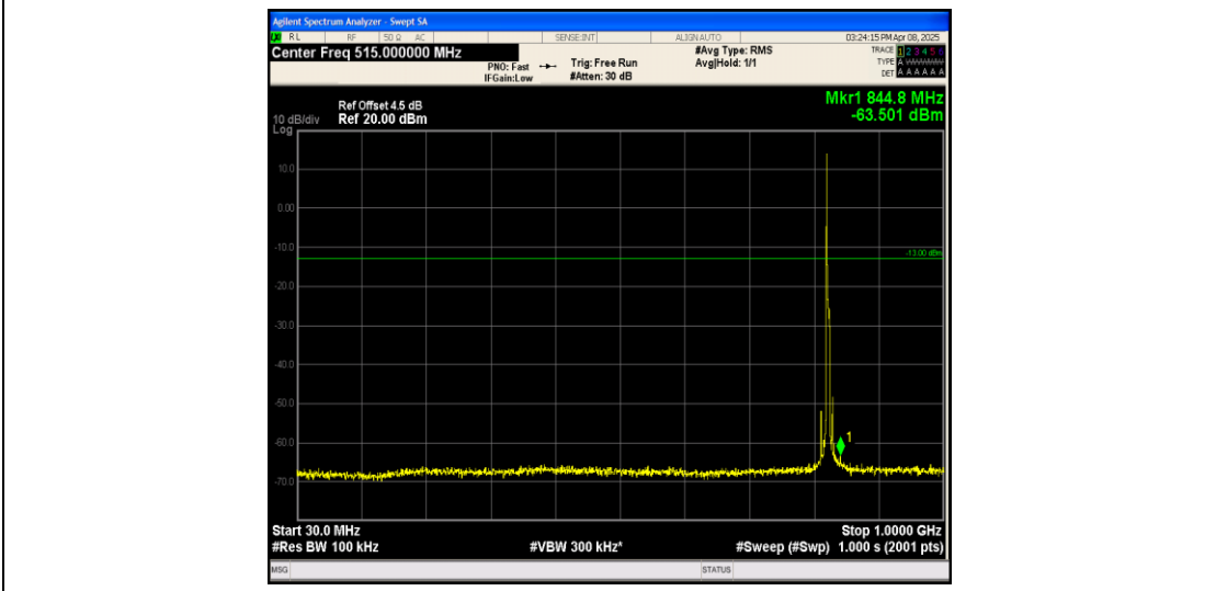
Band26_5MHz_16QAM_26815_1RB#0_30~1000_30~1000
