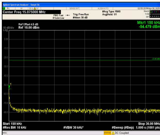
Band26_3MHz_QPSK_27025_1RB#0_0.15~30_0.15~30
