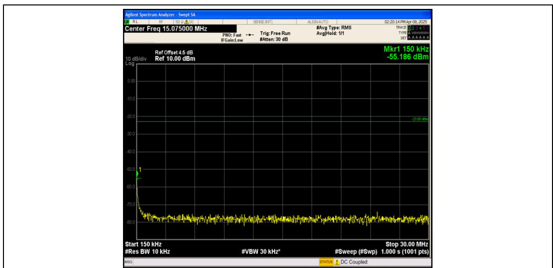
Band26_1.4MHz_16QAM_26797_1RB#0_0.15~30_0.15~30
