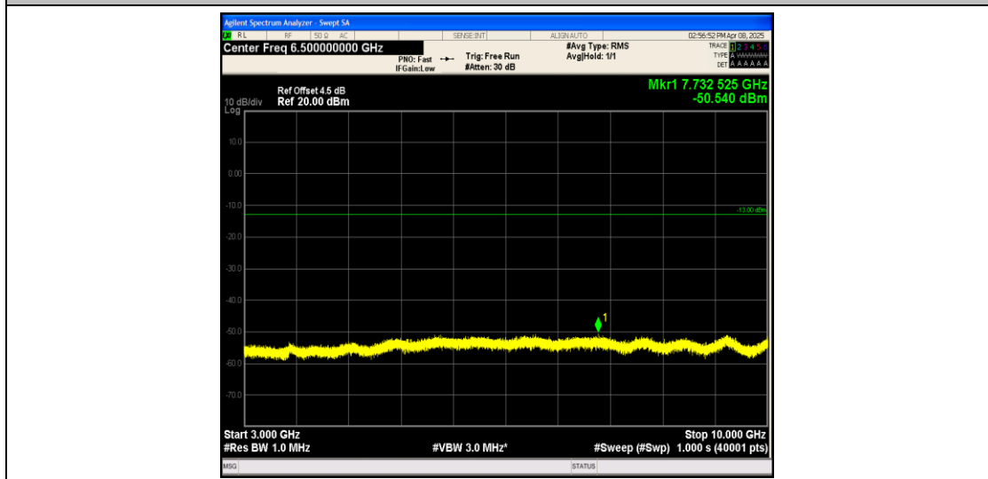
Band26_3MHz_16QAM_27025_1RB#0_3000~10000_3000~10000
