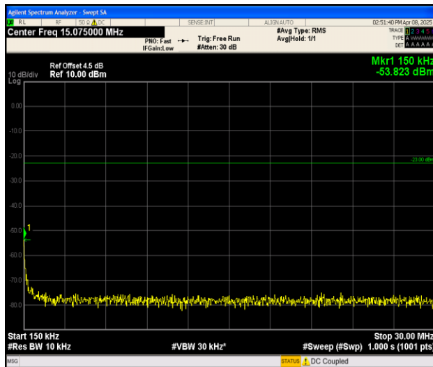
Band26_3MHz_QPSK_26805_1RB#0_0.15~30_0.15~30
