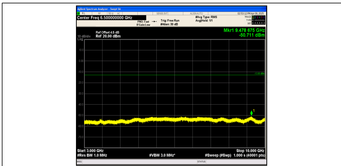
Band26_3MHz_16QAM_26805_1RB#0_3000~10000_3000~10000
