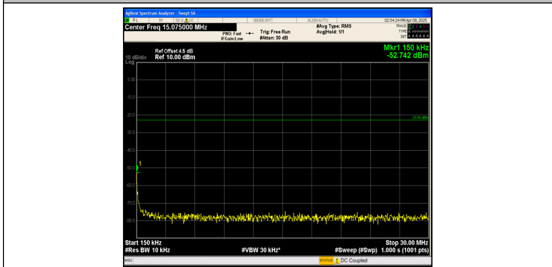
Band26_3MHz_16QAM_26915_1RB#0_0.15~30_0.15~30
