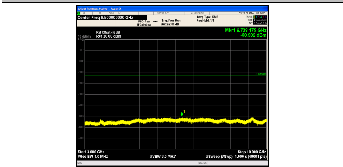
Band26_5MHz_QPSK_26815_1RB#0_3000~10000_3000~10000
