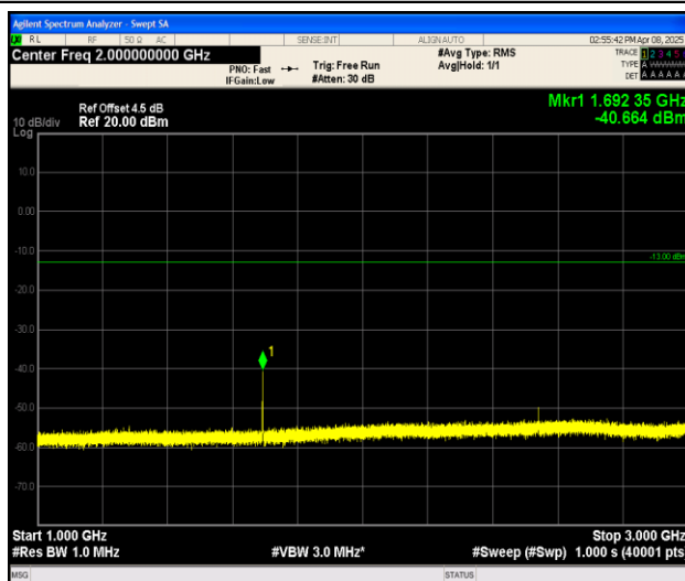
Band26_3MHz_QPSK_27025_1RB#0_1000~3000_1000~3000
