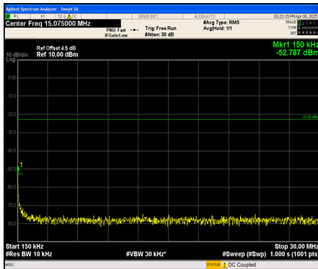
Band26_5MHz_QPSK_26815_1RB#0_0.15~30_0.15~30
