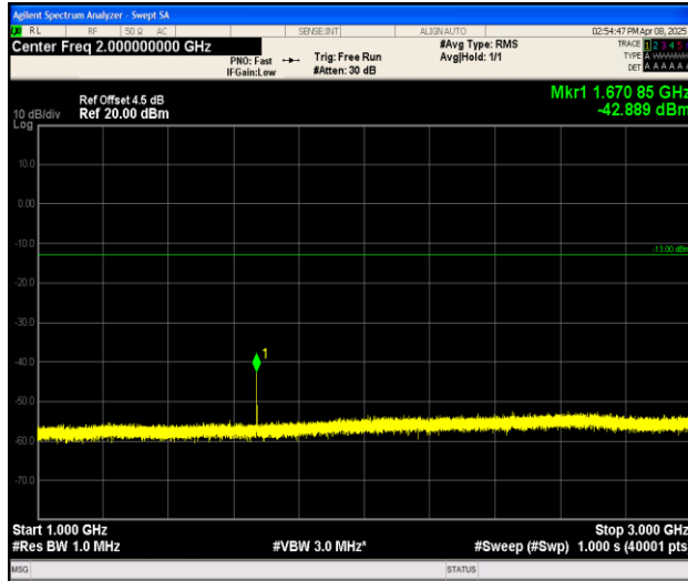
Band26_3MHz_16QAM_26915_1RB#0_1000~3000_1000~3000
