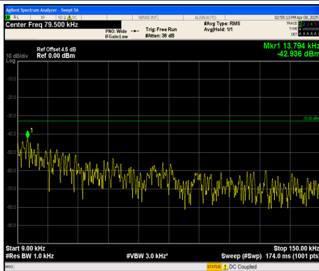
Band26_3MHz_QPSK_27025_1RB#0_0.009~0.15_0.009~0.15
