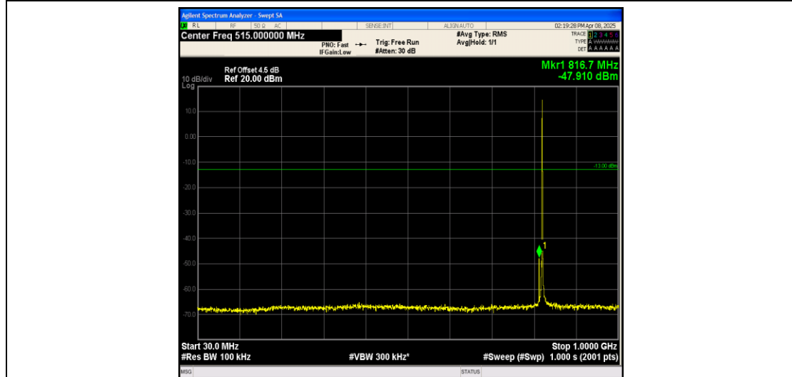
Band26_1.4MHz_QPSK_26797_1RB#0_30~1000_30~1000
