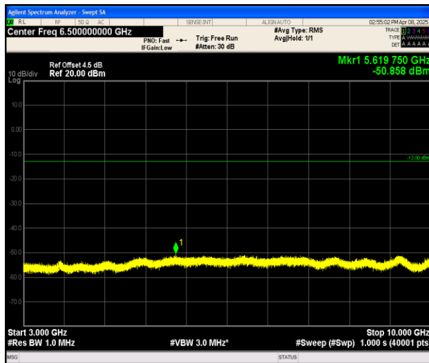
Band26_3MHz_16QAM_26915_1RB#0_3000~10000_3000~10000
