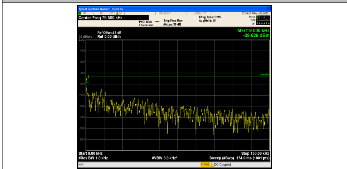
Band26_5MHz_16QAM_26815_1RB#0_0.009~0.15_0.009~0.15
