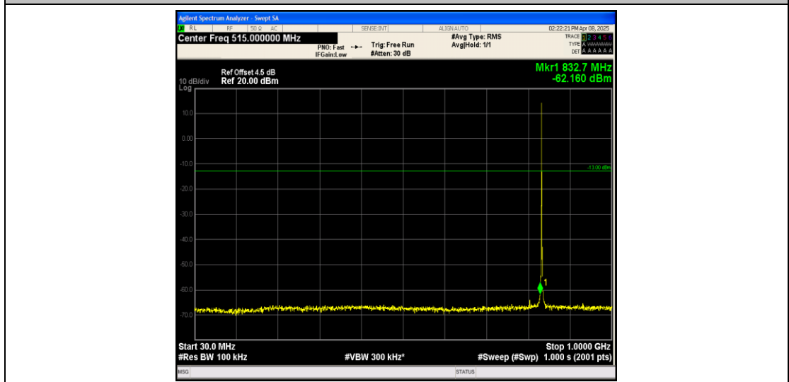
Band26_1.4MHz_16QAM_26915_1RB#0_30~1000_30~1000
