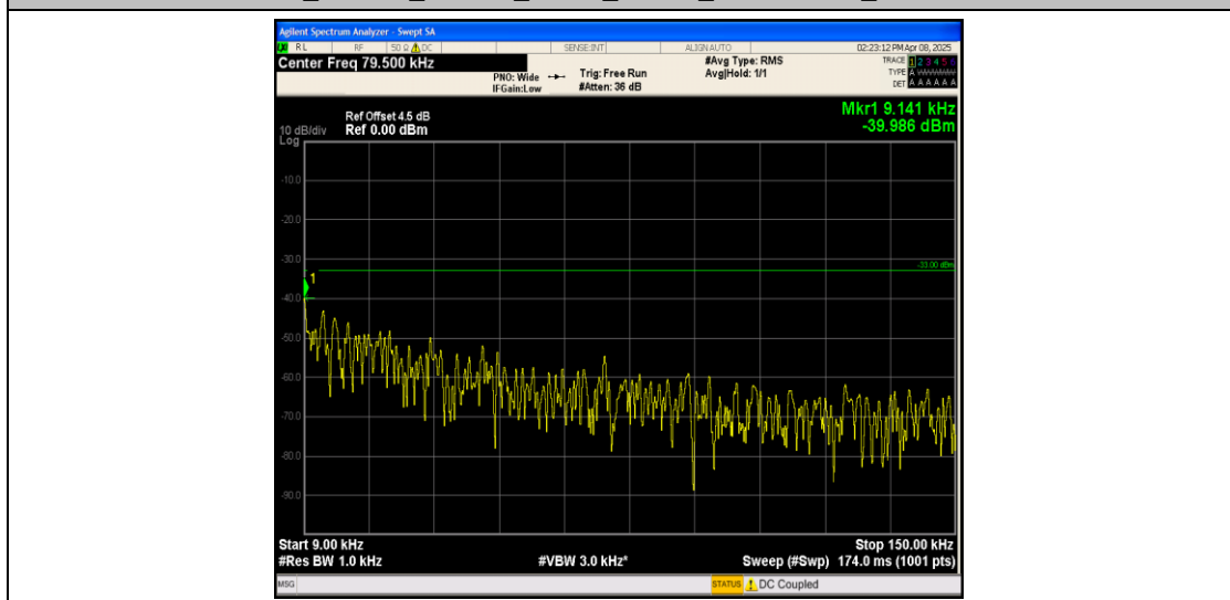
Band26_1.4MHz_QPSK_27033_1RB#0_0.009~0.15_0.009~0.15
