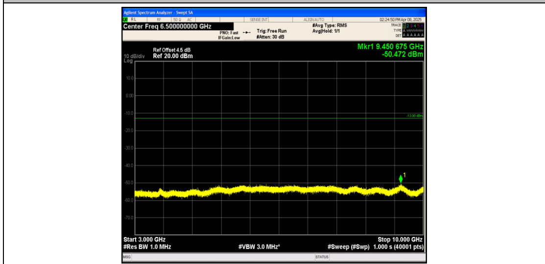
Band26_1.4MHz_16QAM_27033_1RB#0_3000~10000_3000~10000
