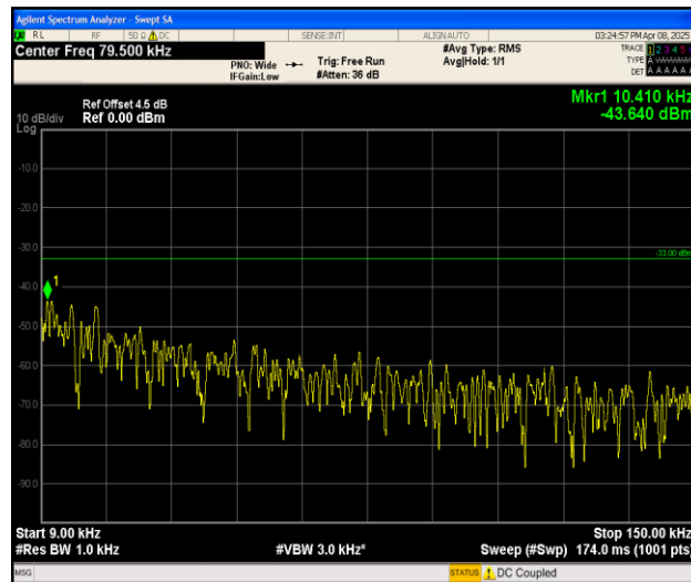
Band26_5MHz_QPSK_26915_1RB#0_0.009~0.15_0.009~0.15
