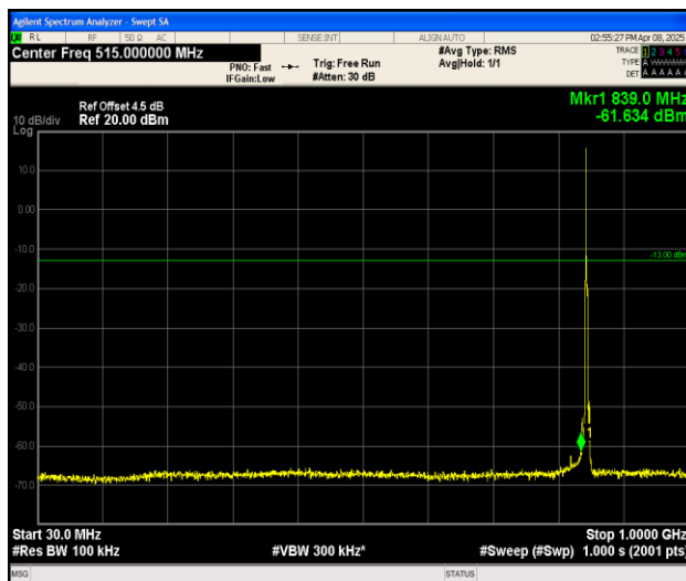
Band26_3MHz_QPSK_27025_1RB#0_30~1000_30~1000
