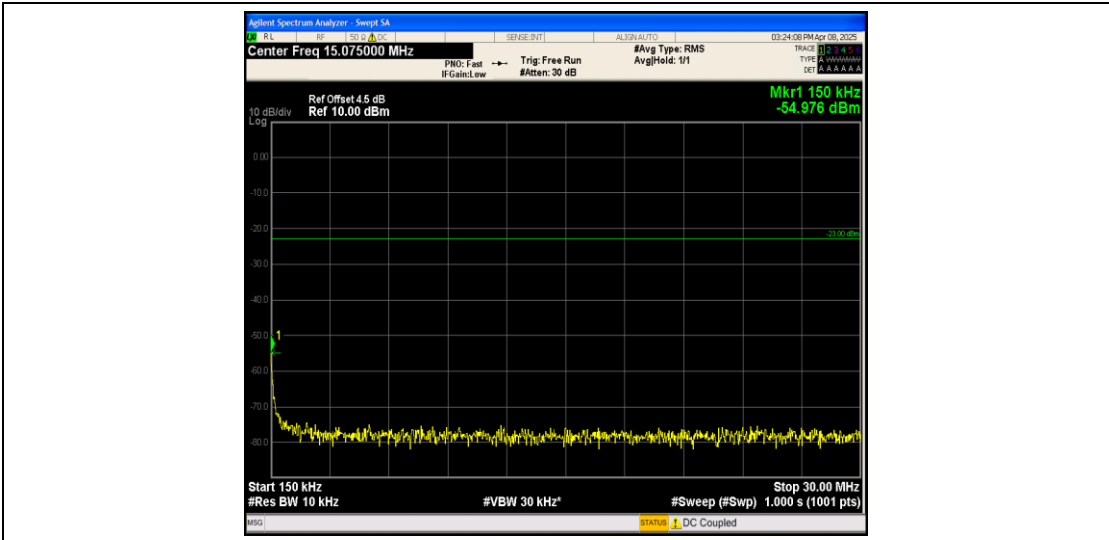
Band26_5MHz_16QAM_26815_1RB#0_0.15~30_0.15~30
