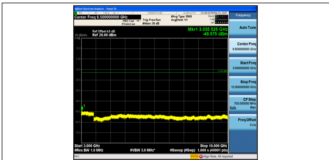
Band26_3MHz_QPSK_26775_1RB#0_3000~10000_3000~10000
