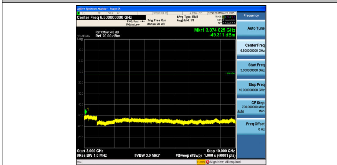
Band26_1.4MHz_16QAM_26783_1RB#0_3000~10000_3000~10000
