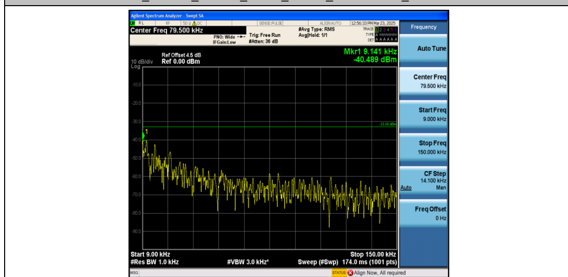
Band26_1.4MHz_QPSK_26783_1RB#0_0.009~0.15_0.009~0.15
