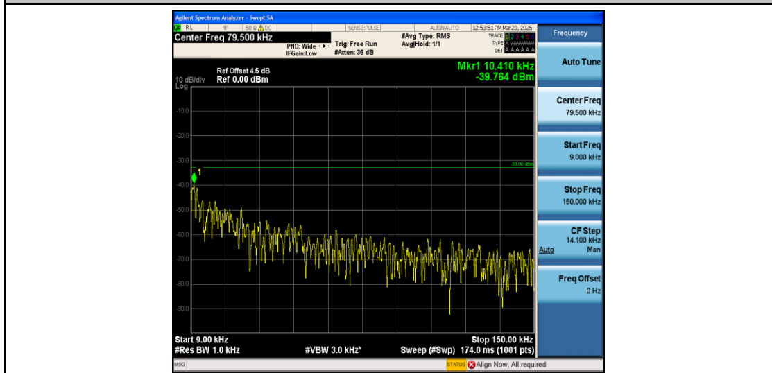
Band26_1.4MHz_16QAM_26697_1RB#0_0.009~0.15_0.009~0.15
