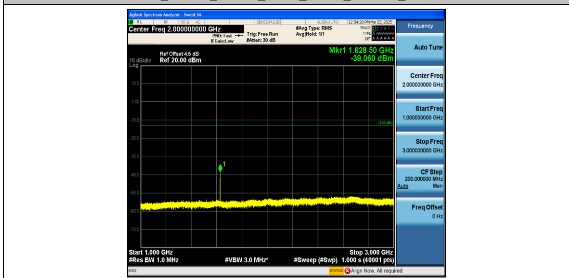
Band26_1.4MHz_16QAM_26697_1RB#0_1000~3000_1000~3000
