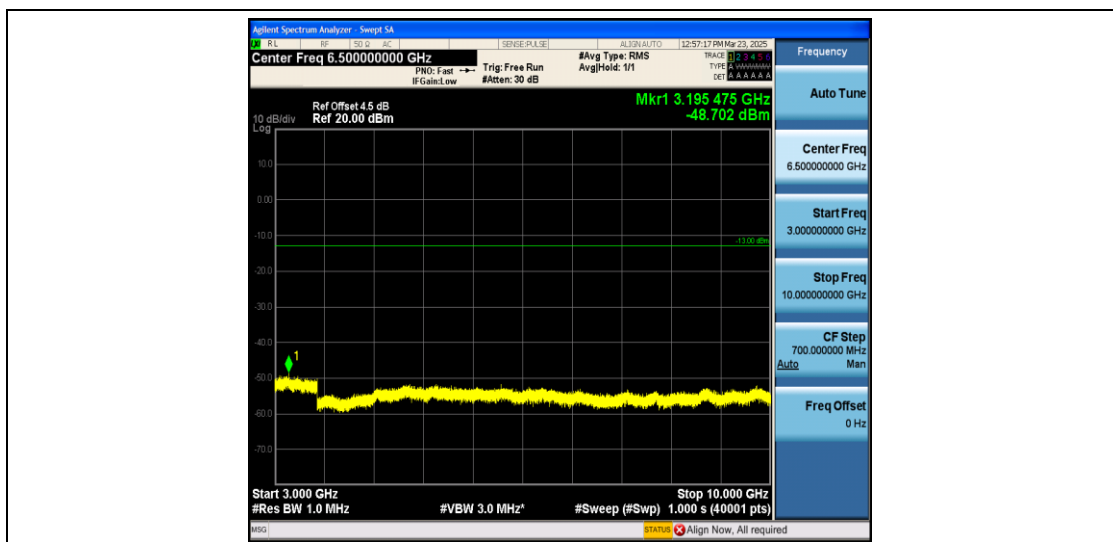
Band26_1.4MHz_QPSK_26783_1RB#0_3000~10000_3000~10000
