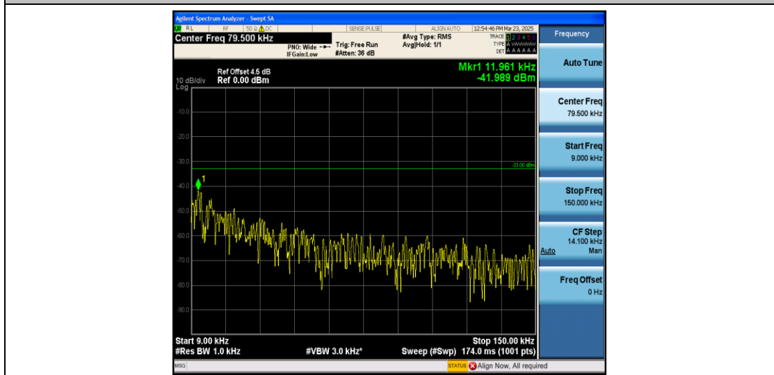
Band26_1.4MHz_QPSK_26740_1RB#0_0.009~0.15_0.009~0.15
