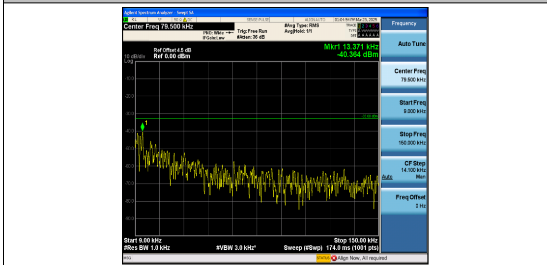
Band26_3MHz_16QAM_26705_1RB#0_0.009~0.15_0.009~0.15
