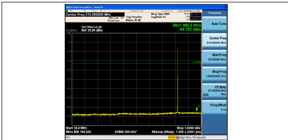
Band26_1.4MHz_16QAM_26783_1RB#0_30~1000_30~1000
