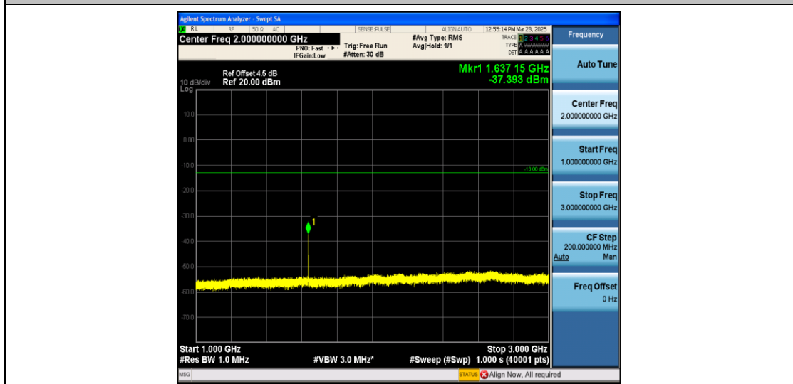
Band26_1.4MHz_QPSK_26740_1RB#0_1000~3000_1000~3000
