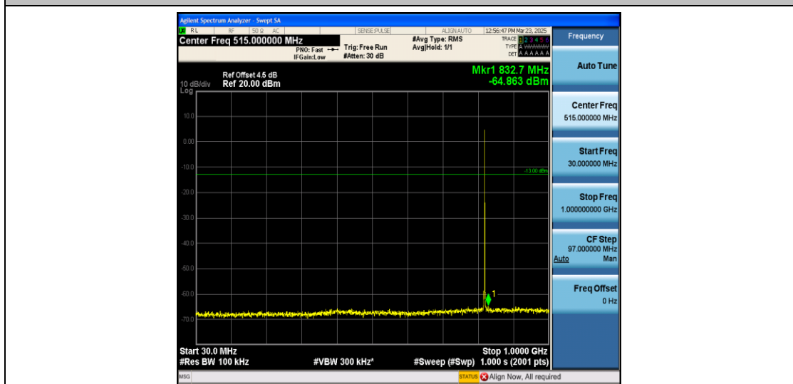
Band26_1.4MHz_QPSK_26783_1RB#0_30~1000_30~1000
