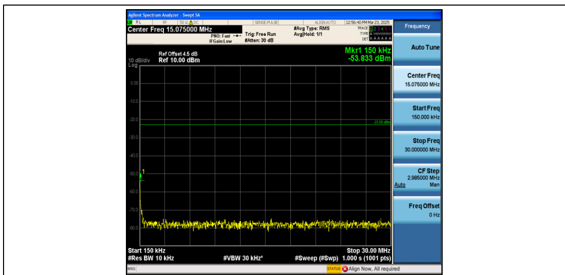
Band26_1.4MHz_QPSK_26783_1RB#0_0.15~30_0.15~30
