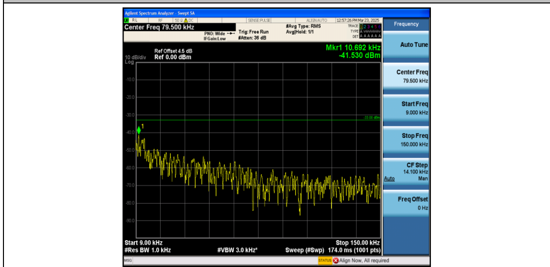
Band26_1.4MHz_16QAM_26783_1RB#0_0.009~0.15_0.009~0.15
