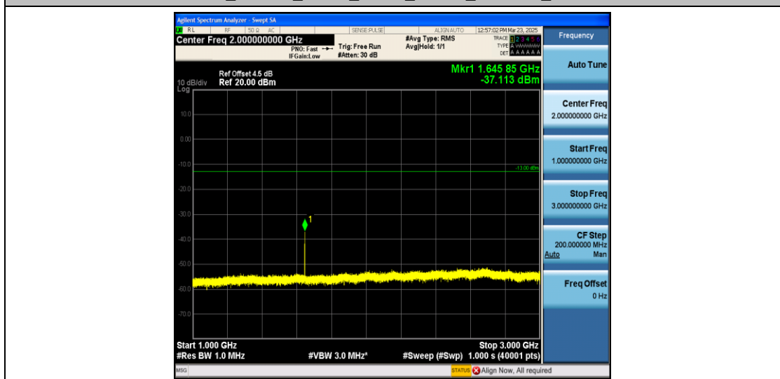
Band26_1.4MHz_QPSK_26783_1RB#0_1000~3000_1000~3000
