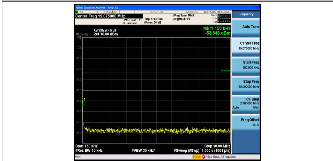
Band26_1.4MHz_QPSK_26740_1RB#0_0.15~30_0.15~30
