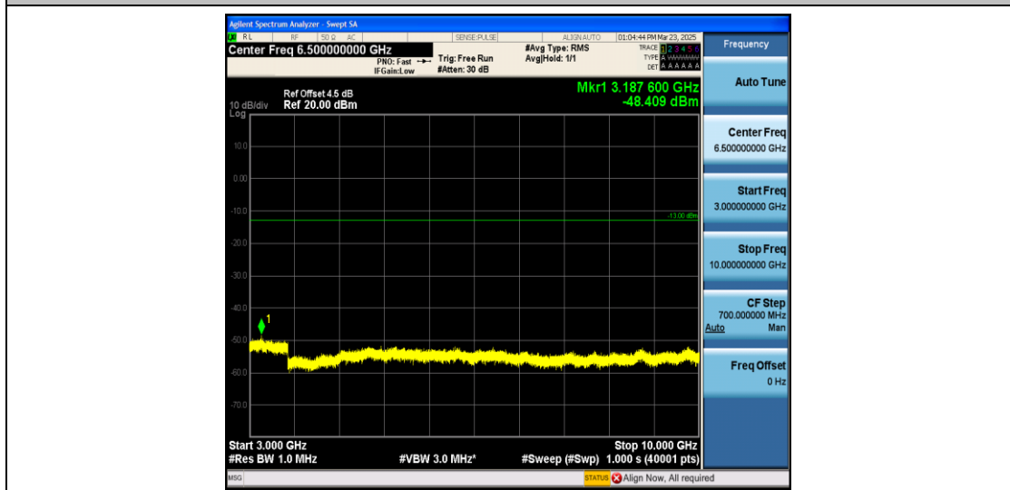
Band26_3MHz_QPSK_26705_1RB#0_3000~10000_3000~10000
