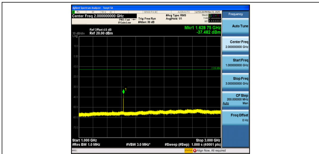
Band26_1.4MHz_QPSK_26697_1RB#0_1000~3000_1000~3000
