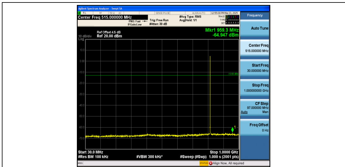
Band26_1.4MHz_QPSK_26740_1RB#0_30~1000_30~1000
