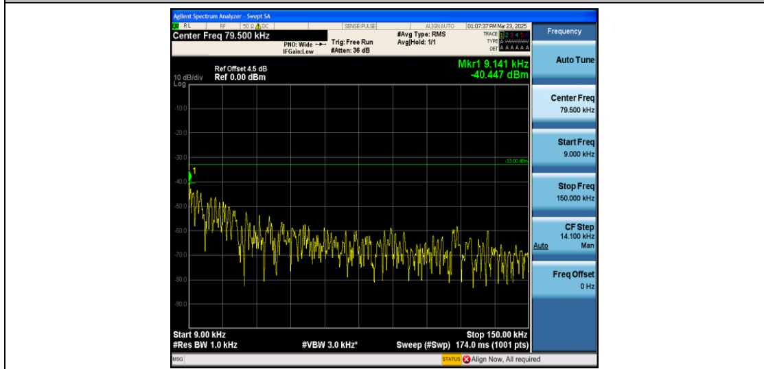
Band26_3MHz_QPSK_26775_1RB#0_0.009~0.15_0.009~0.15
