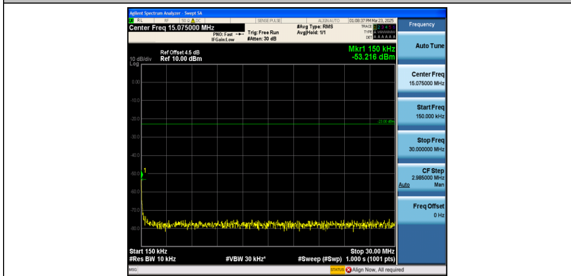
Band26_3MHz_16QAM_26775_1RB#0_0.15~30_0.15~30
