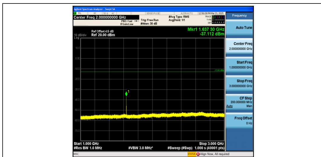
Band26_1.4MHz_16QAM_26740_1RB#0_1000~3000_1000~3000
