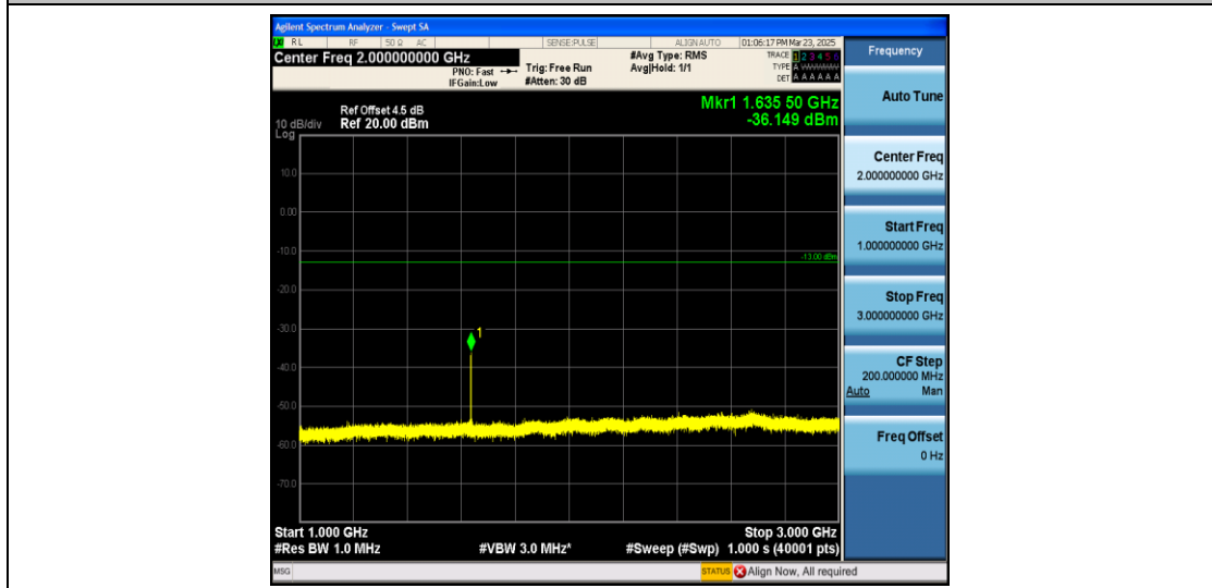
Band26_3MHz_QPSK_26740_1RB#0_1000~3000_1000~3000
