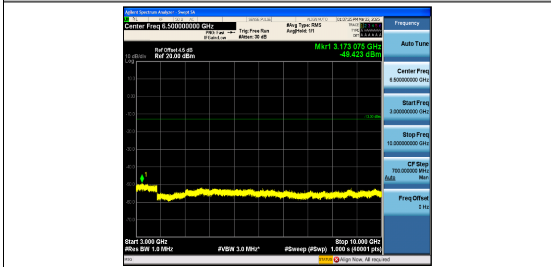
Band26_3MHz_16QAM_26740_1RB#0_3000~10000_3000~10000
