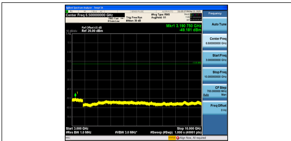
Band26_3MHz_16QAM_26705_1RB#0_3000~10000_3000~10000
