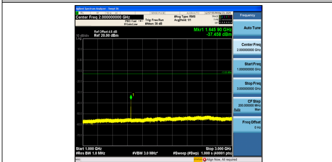
Band26_1.4MHz_16QAM_26783_1RB#0_1000~3000_1000~3000
