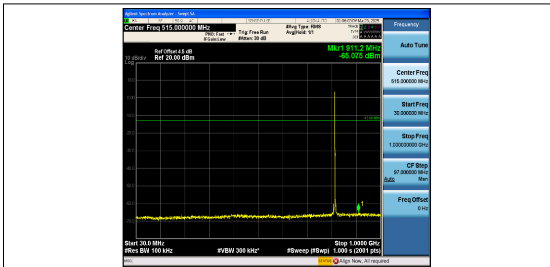
Band26_3MHz_QPSK_26740_1RB#0_30~1000_30~1000
