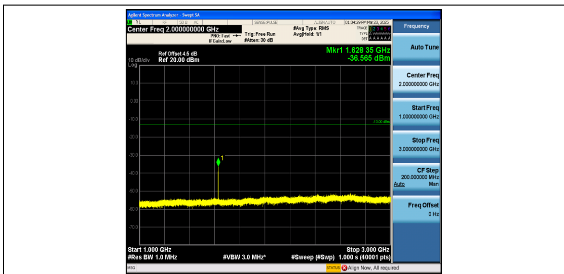
Band26_3MHz_QPSK_26705_1RB#0_1000~3000_1000~3000
