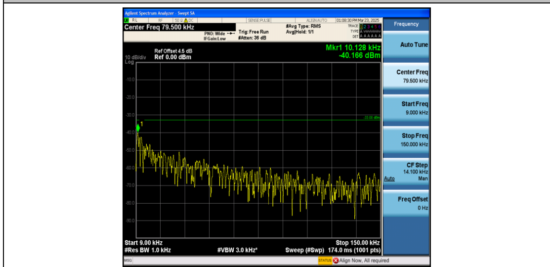
Band26_3MHz_16QAM_26775_1RB#0_0.009~0.15_0.009~0.15
