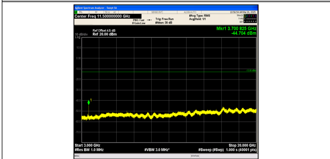
Band25_10MHz_16QAM_26090_1RB#0_3000~20000_3000~20000
