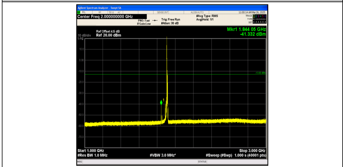
Band25_10MHz_16QAM_26640_1RB#0_1000~3000_1000~3000
