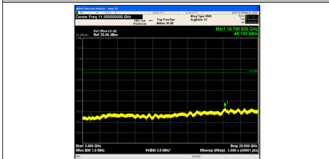
Band25_5MHz_QPSK_26665_1RB#0_3000~20000_3000~20000
