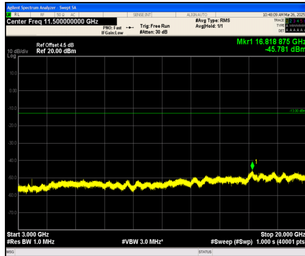
Band25_5MHz_16QAM_26665_1RB#0_3000~20000_3000~20000
