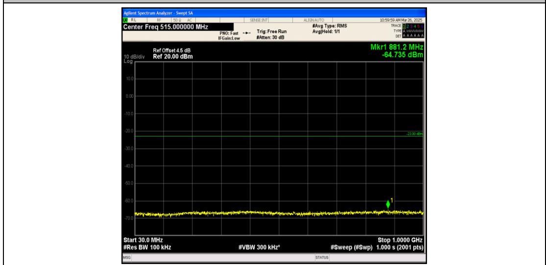
Band25_10MHz_16QAM_26640_1RB#0_30~1000_30~1000
