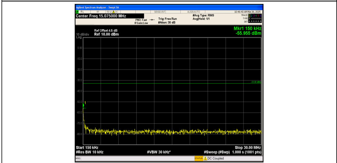
Band25_5MHz_QPSK_26665_1RB#0_0.15~30_0.15~30
