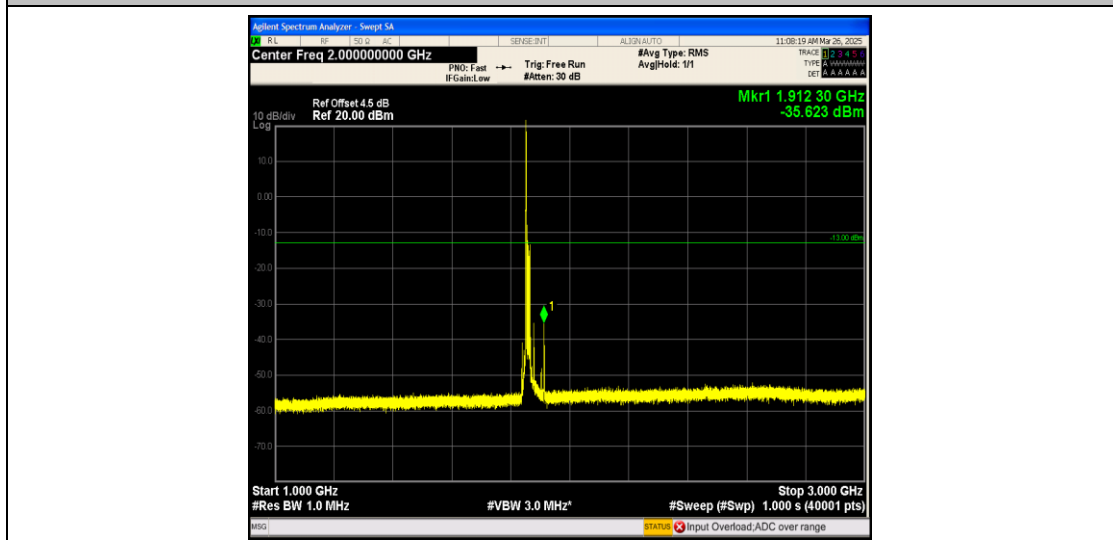
Band25_15MHz_QPSK_26115_1RB#0_1000~3000_1000~3000
