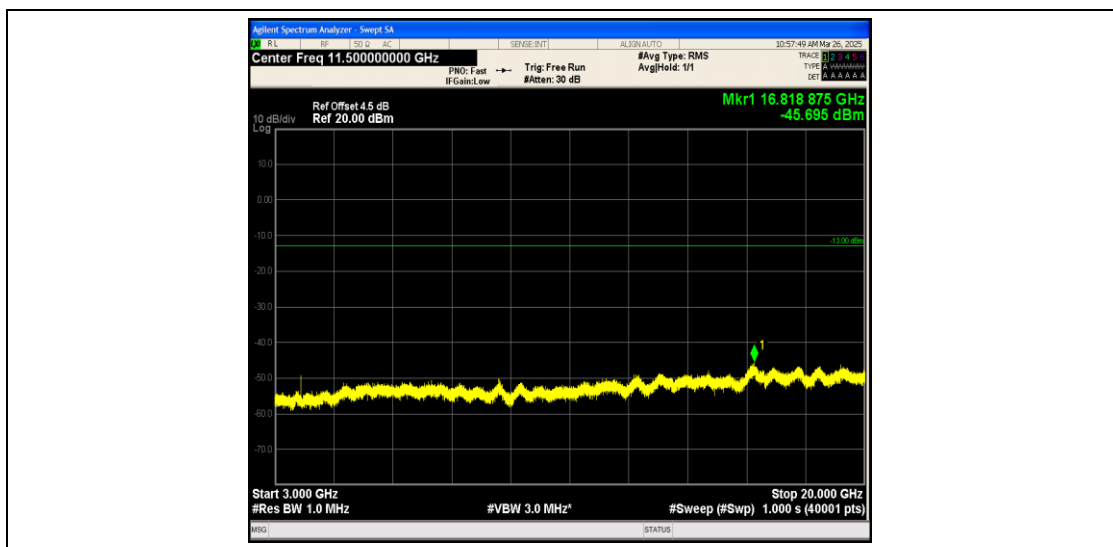
Band25_10MHz_QPSK_26365_1RB#0_3000~20000_3000~20000
