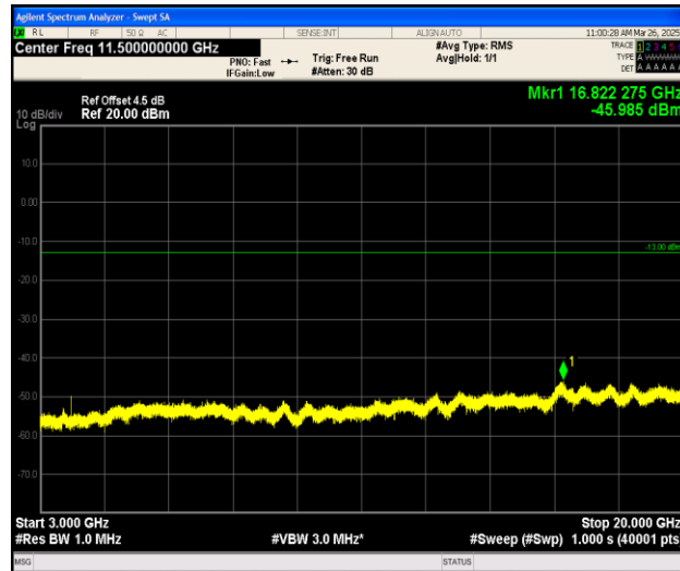
Band25_10MHz_16QAM_26640_1RB#0_3000~20000_3000~20000
