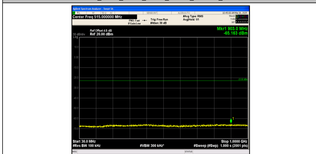
Band25_5MHz_QPSK_26365_1RB#0_30~1000_30~1000
