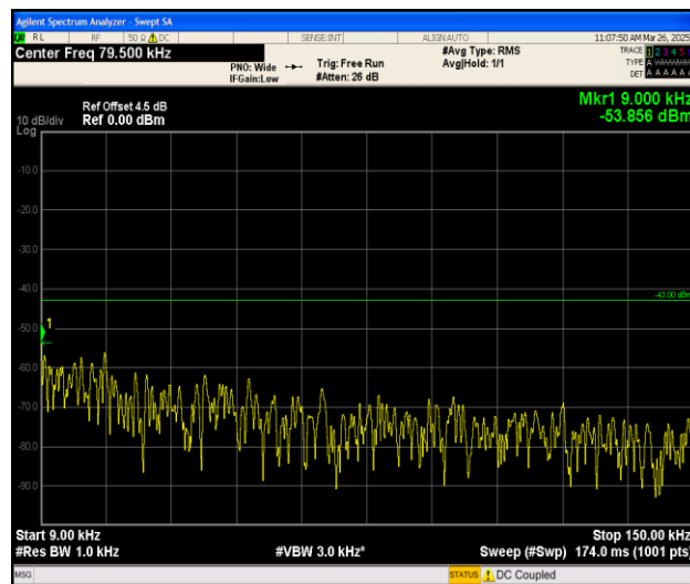
Band25_15MHz_QPSK_26115_1RB#0_0.009~0.15_0.009~0.15
