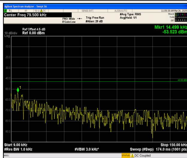
Band25_15MHz_QPSK_26365_1RB#0_0.009~0.15_0.009~0.15
