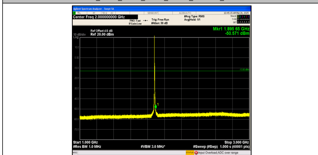
Band25_5MHz_QPSK_26365_1RB#0_1000~3000_1000~3000
