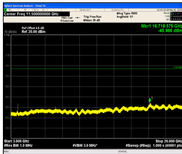
Band25_5MHz_16QAM_26065_1RB#0_3000~20000_3000~20000
