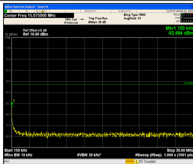
Band25_15MHz_QPSK_26115_1RB#0_0.15~30_0.15~30
