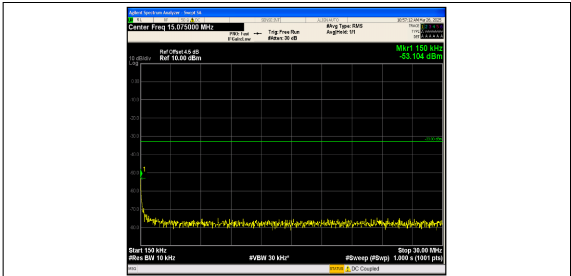
Band25_10MHz_QPSK_26365_1RB#0_0.15~30_0.15~30
