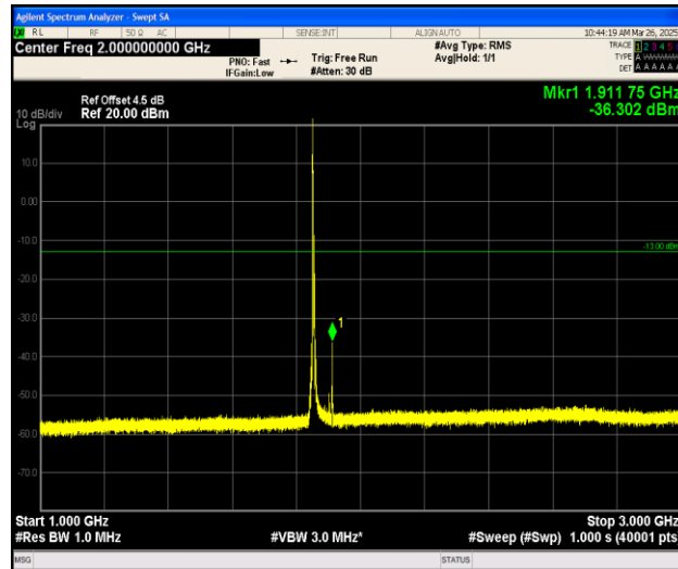
Band25_5MHz_16QAM_26065_1RB#0_1000~3000_1000~3000
