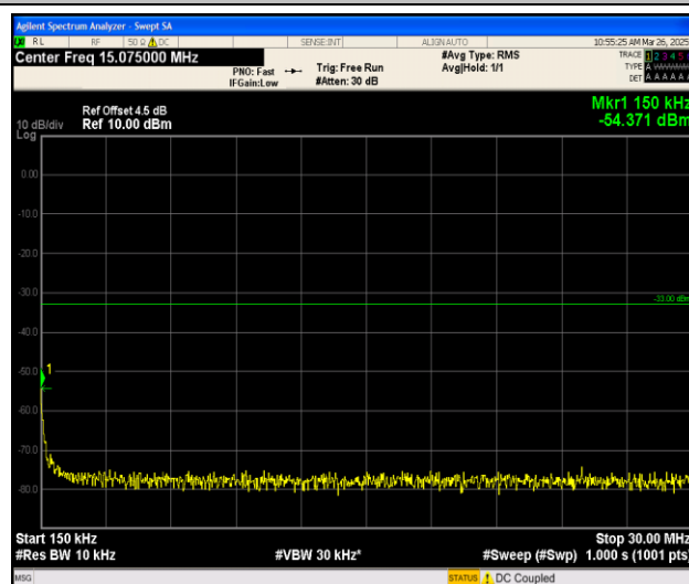
Band25_10MHz_QPSK_26090_1RB#0_0.15~30_0.15~30
