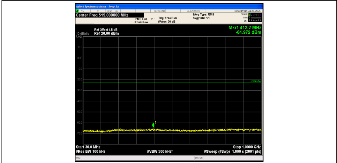
Band25_10MHz_QPSK_26365_1RB#0_30~1000_30~1000
