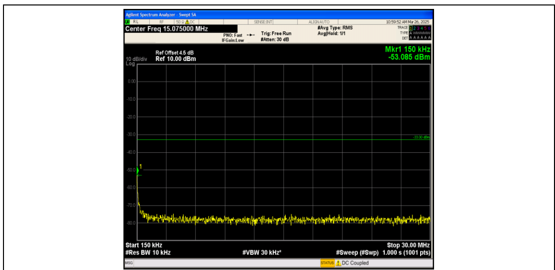
Band25_10MHz_16QAM_26640_1RB#0_0.15~30_0.15~30
