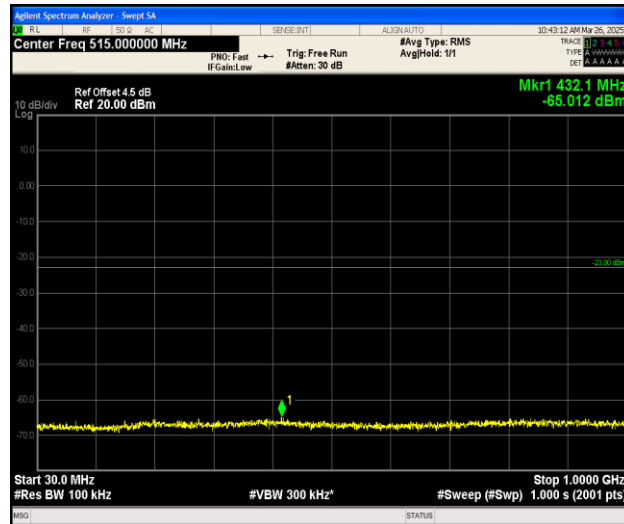
Band25_5MHz_QPSK_26065_1RB#0_30~1000_30~1000
