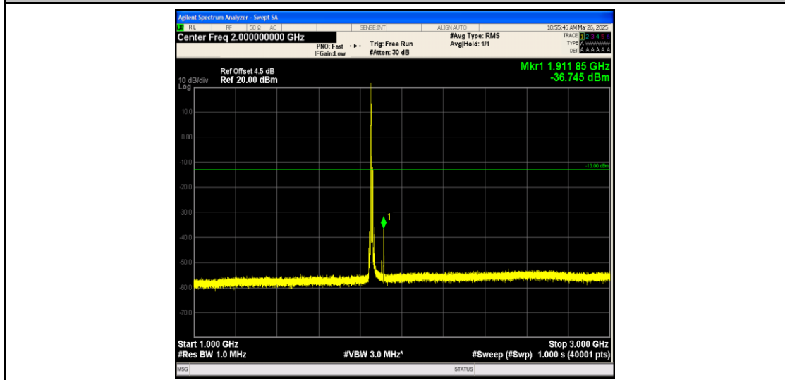
Band25_10MHz_QPSK_26090_1RB#0_1000~3000_1000~3000
