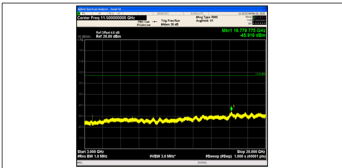
Band25_15MHz_QPSK_26365_1RB#0_3000~20000_3000~20000
