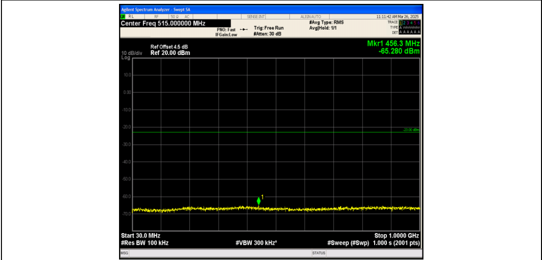
Band25_15MHz_QPSK_26615_1RB#0_30~1000_30~1000
