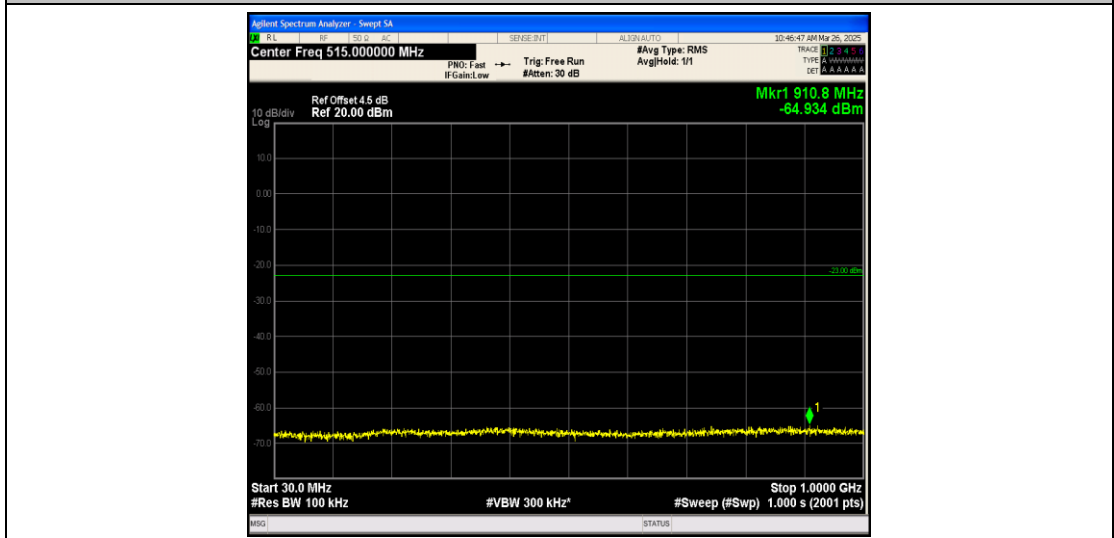
Band25_5MHz_QPSK_26665_1RB#0_30~1000_30~1000
