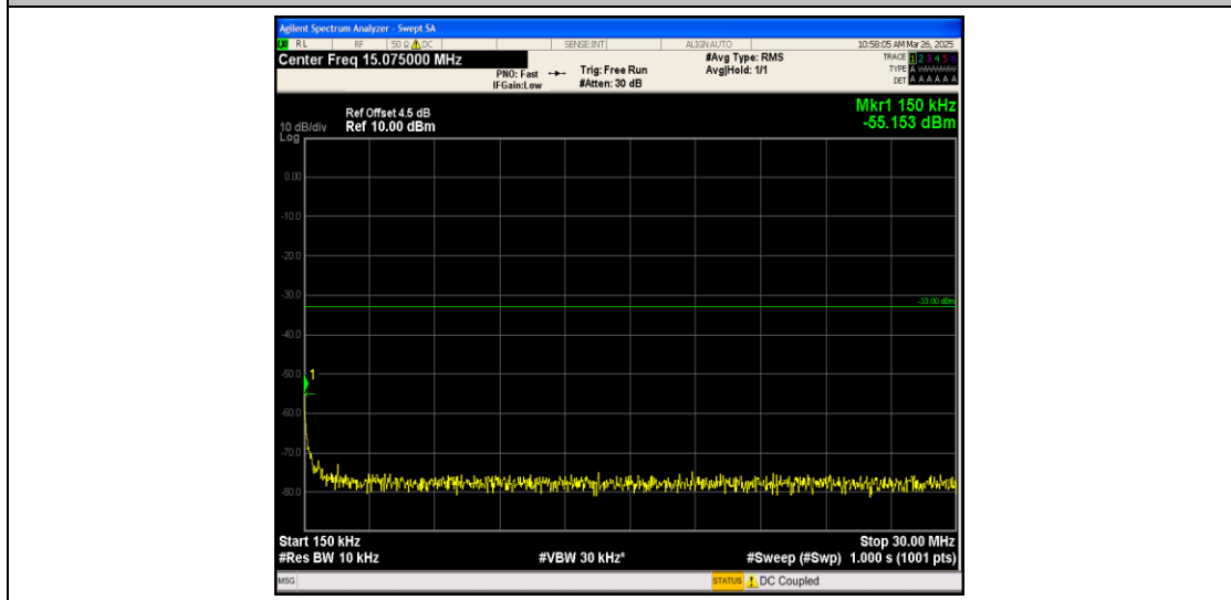
Band25_10MHz_16QAM_26365_1RB#0_0.15~30_0.15~30
