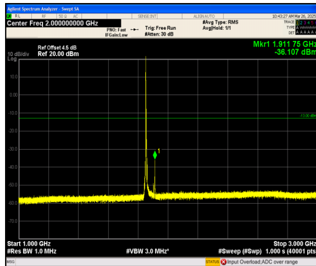
Band25_5MHz_QPSK_26065_1RB#0_1000~3000_1000~3000
