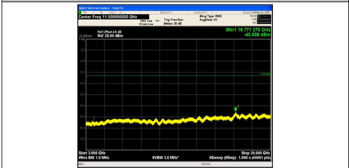
Band25_15MHz_16QAM_26365_1RB#0_3000~20000_3000~20000
