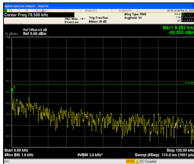
Band25_10MHz_QPSK_26090_1RB#0_0.009~0.15_0.009~0.15
