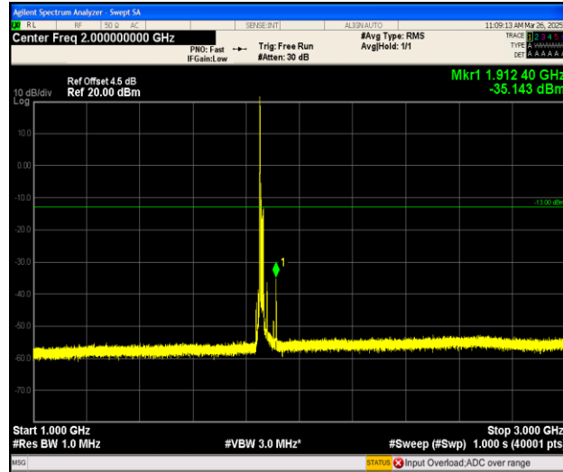
Band25_15MHz_16QAM_26115_1RB#0_1000~3000_1000~3000
