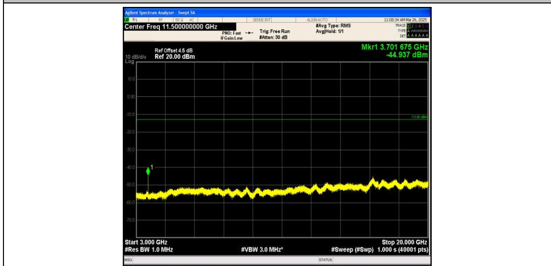
Band25_15MHz_QPSK_26115_1RB#0_3000~20000_3000~20000
