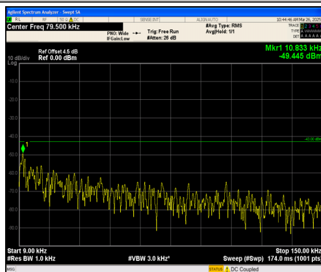
Band25_5MHz_QPSK_26365_1RB#0_0.009~0.15_0.009~0.15
