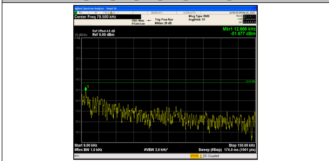
Band25_10MHz_16QAM_26640_1RB#0_0.009~0.15_0.009~0.15
