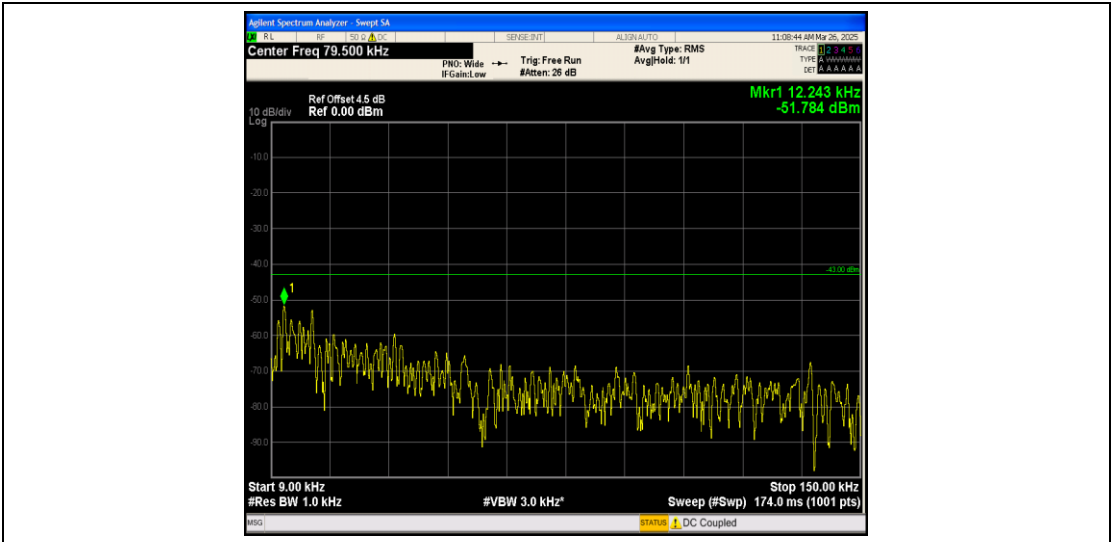
Band25_15MHz_16QAM_26115_1RB#0_0.009~0.15_0.009~0.15
