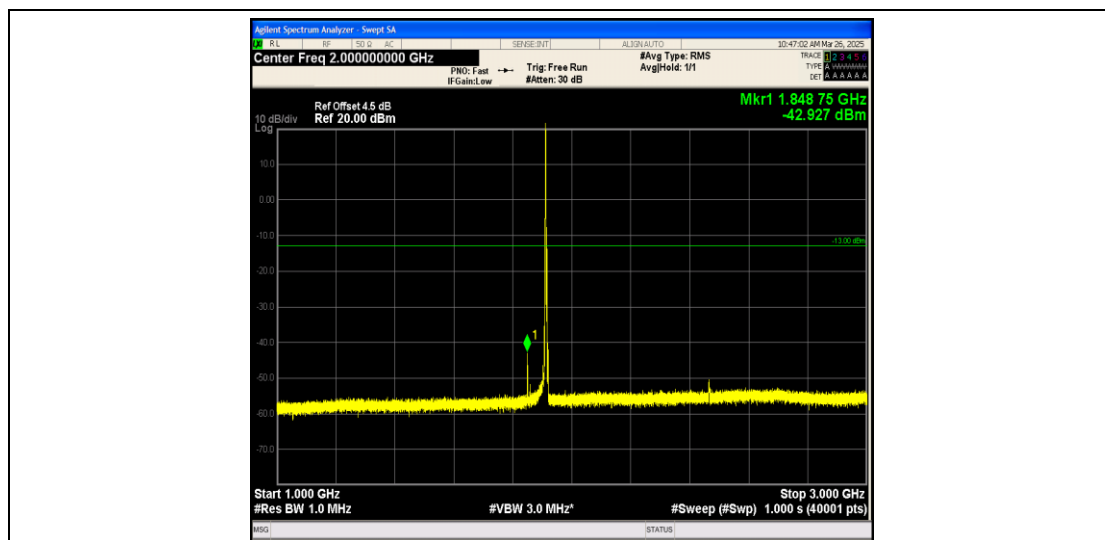
Band25_5MHz_QPSK_26665_1RB#0_1000~3000_1000~3000
