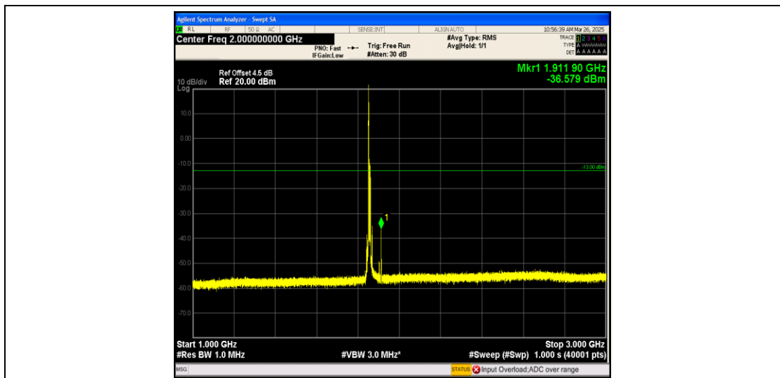
Band25_10MHz_16QAM_26090_1RB#0_1000~3000_1000~3000
