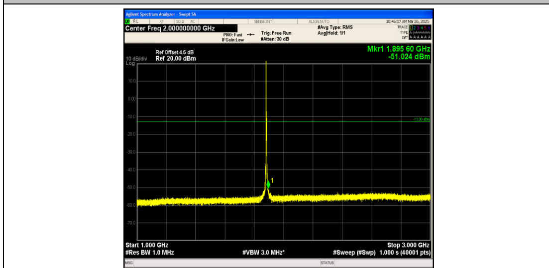
Band25_5MHz_16QAM_26365_1RB#0_1000~3000_1000~3000
