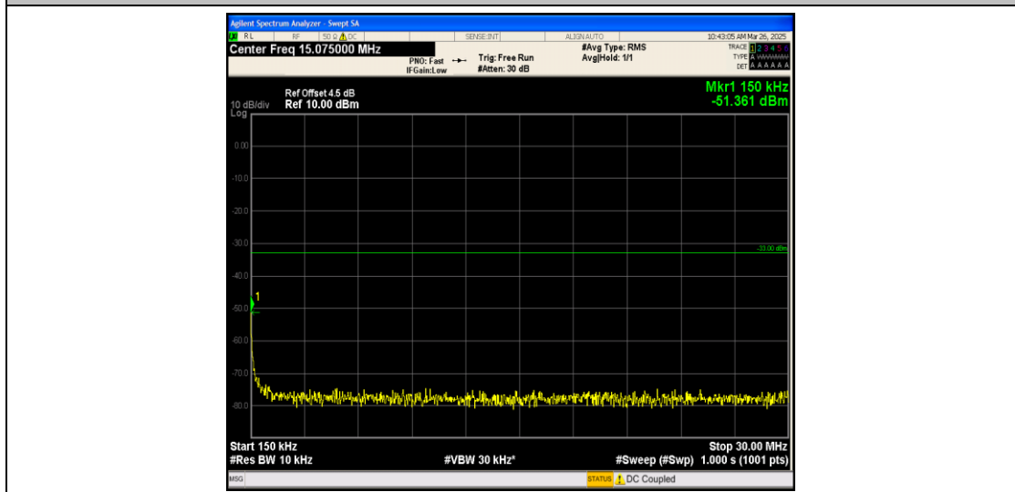
Band25_5MHz_QPSK_26065_1RB#0_0.15~30_0.15~30
