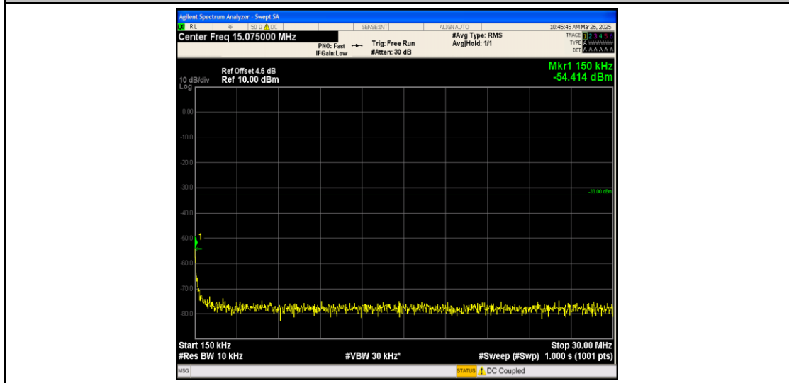
Band25_5MHz_16QAM_26365_1RB#0_0.15~30_0.15~30
