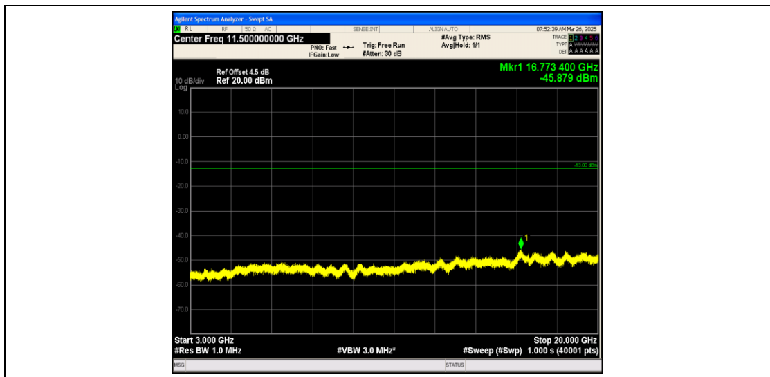
Band25_3MHz_16QAM_26675_1RB#0_3000~20000_3000~20000
