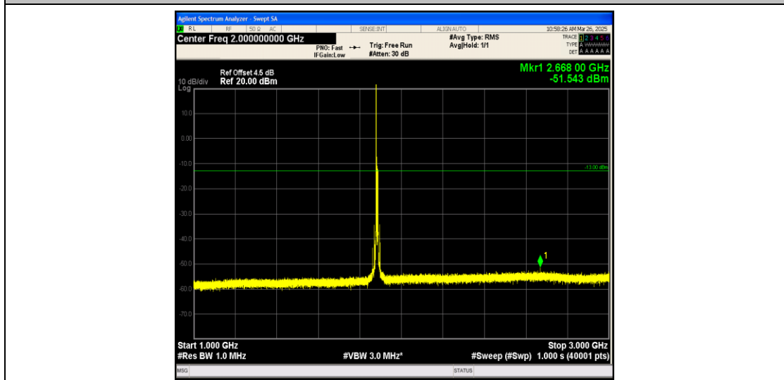
Band25_10MHz_16QAM_26365_1RB#0_1000~3000_1000~3000
