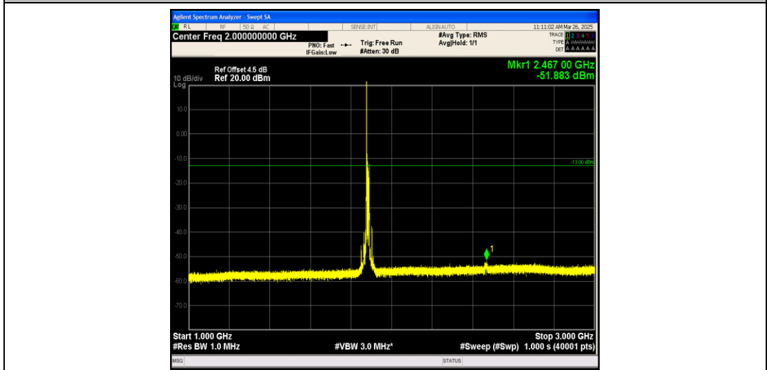
Band25_15MHz_16QAM_26365_1RB#0_1000~3000_1000~3000
