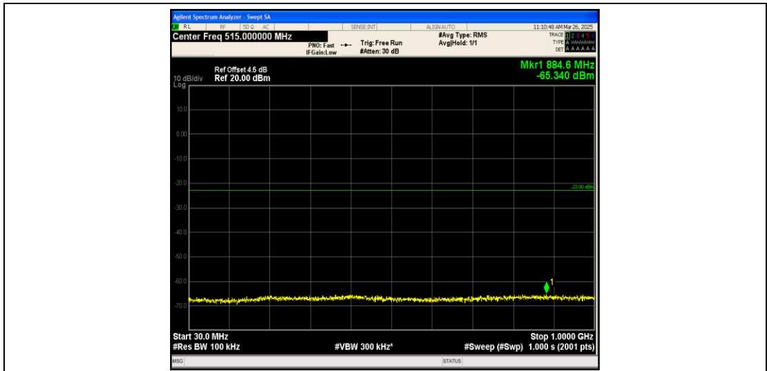
Band25_15MHz_16QAM_26365_1RB#0_30~1000_30~1000
