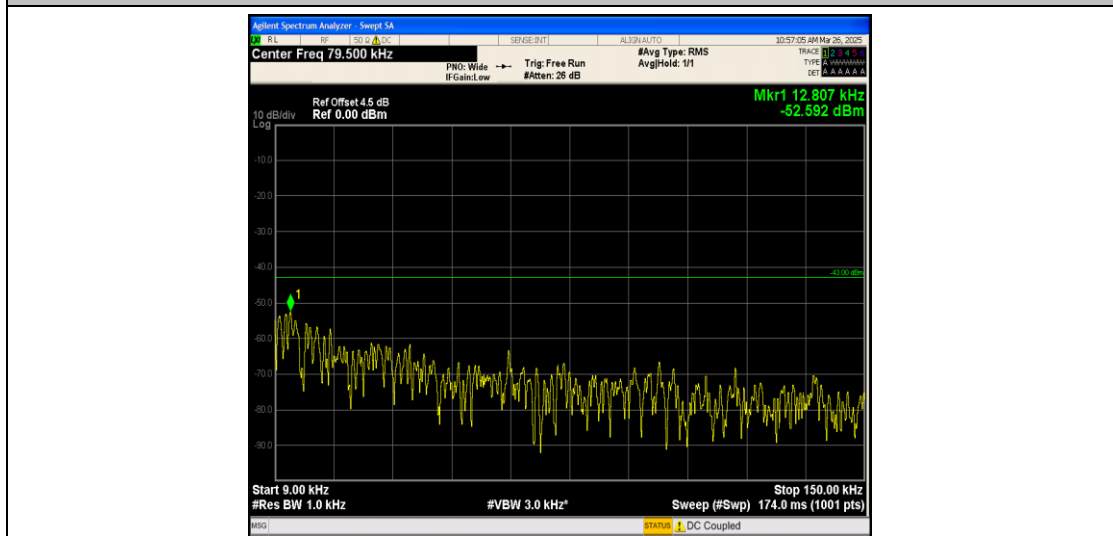
Band25_10MHz_QPSK_26365_1RB#0_0.009~0.15_0.009~0.15
