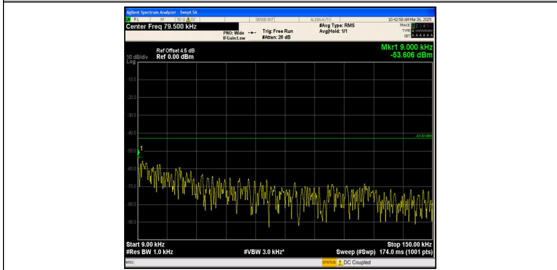
Band25_5MHz_QPSK_26065_1RB#0_0.009~0.15_0.009~0.15
