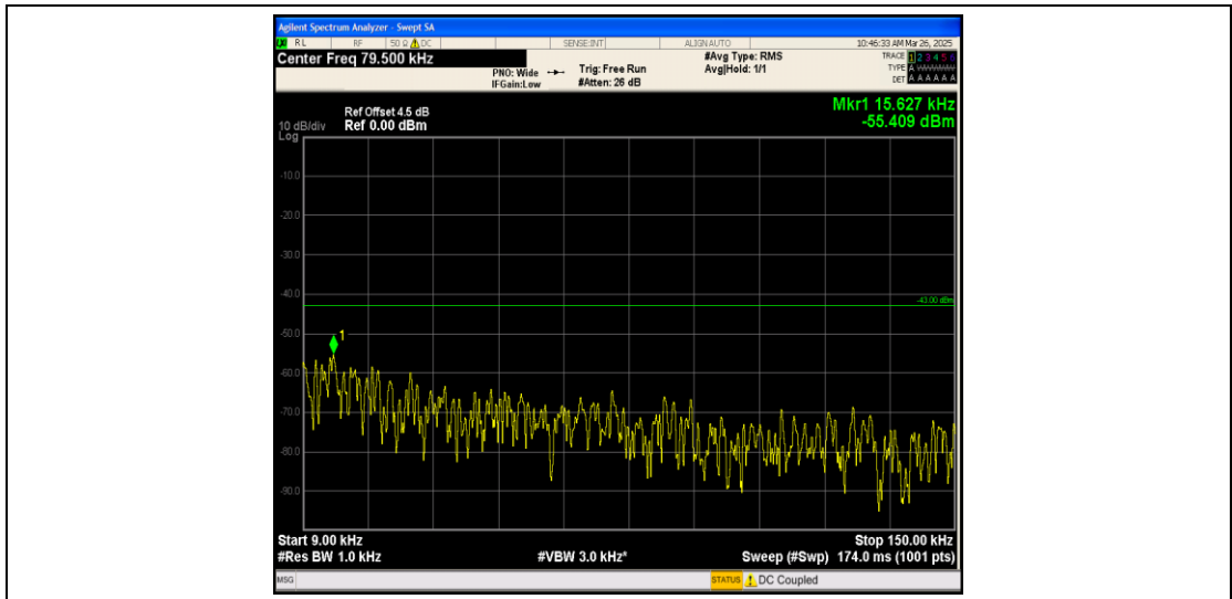
Band25_5MHz_QPSK_26665_1RB#0_0.009~0.15_0.009~0.15
