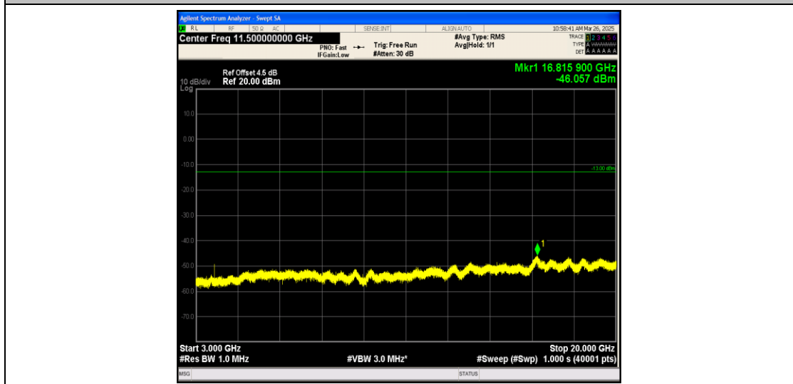
Band25_10MHz_16QAM_26365_1RB#0_3000~20000_3000~20000
