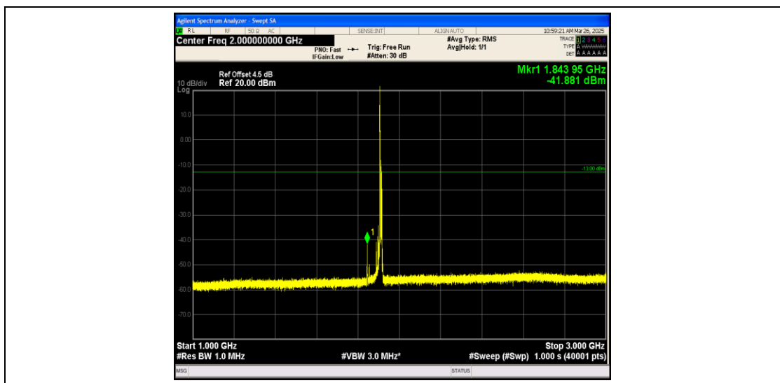
Band25_10MHz_QPSK_26640_1RB#0_1000~3000_1000~3000
