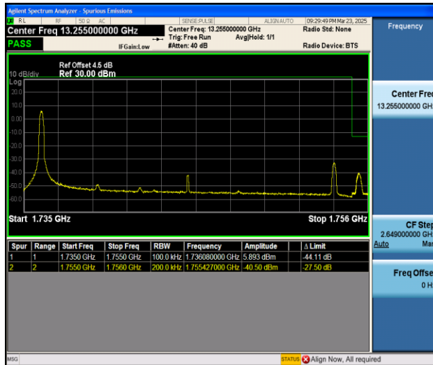
Band4_20MHz_QPSK_20300_1RB#0
