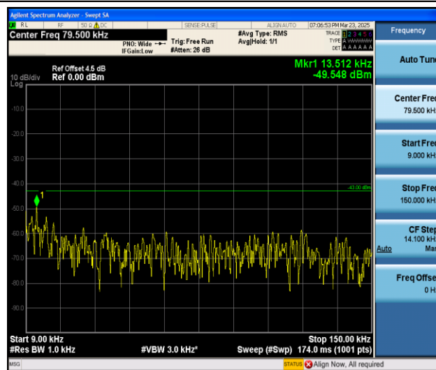
Band4_1.4MHz_QPSK_20175_1RB#0_0.009~0.15_0.009~0.15
