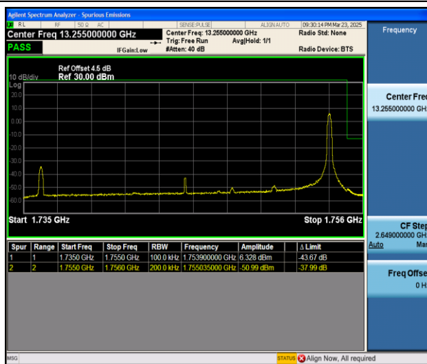
Band4_20MHz_QPSK_20300_1RB#99
