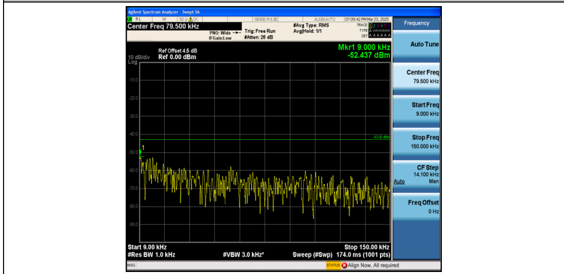
Band4_1.4MHz_16QAM_20393_1RB#0_0.009~0.15_0.009~0.15
