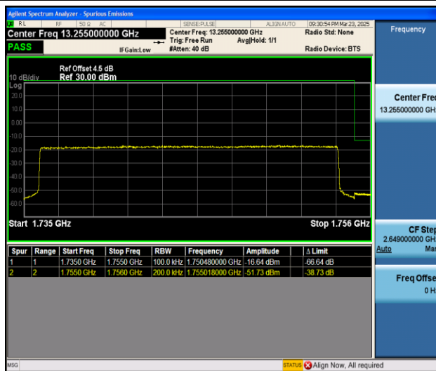
Band4_20MHz_16QAM_20300_100RB#0
