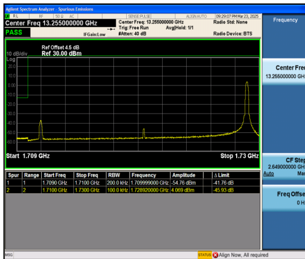
Band4_20MHz_16QAM_20050_1RB#99
