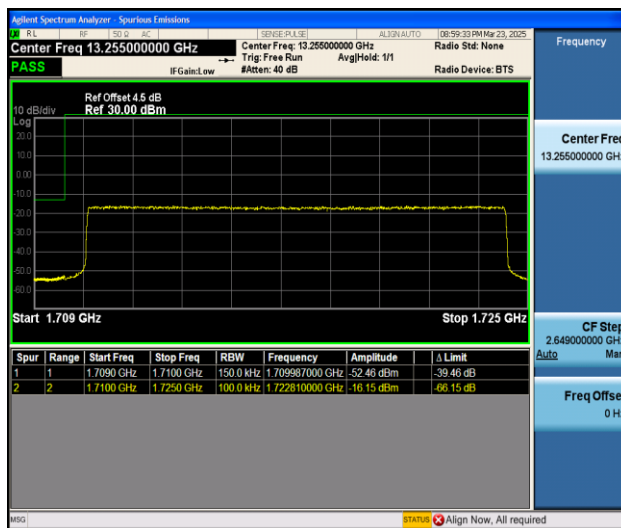
Band4_15MHz_QPSK_20025_75RB#0
