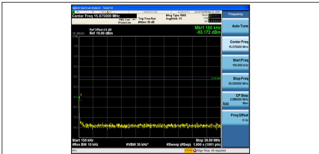
Band4_1.4MHz_QPSK_20175_1RB#0_0.15~30_0.15~30
