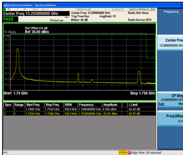
Band4_15MHz_16QAM_20325_1RB#0
