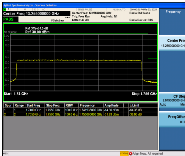
Band4_15MHz_QPSK_20325_75RB#0
