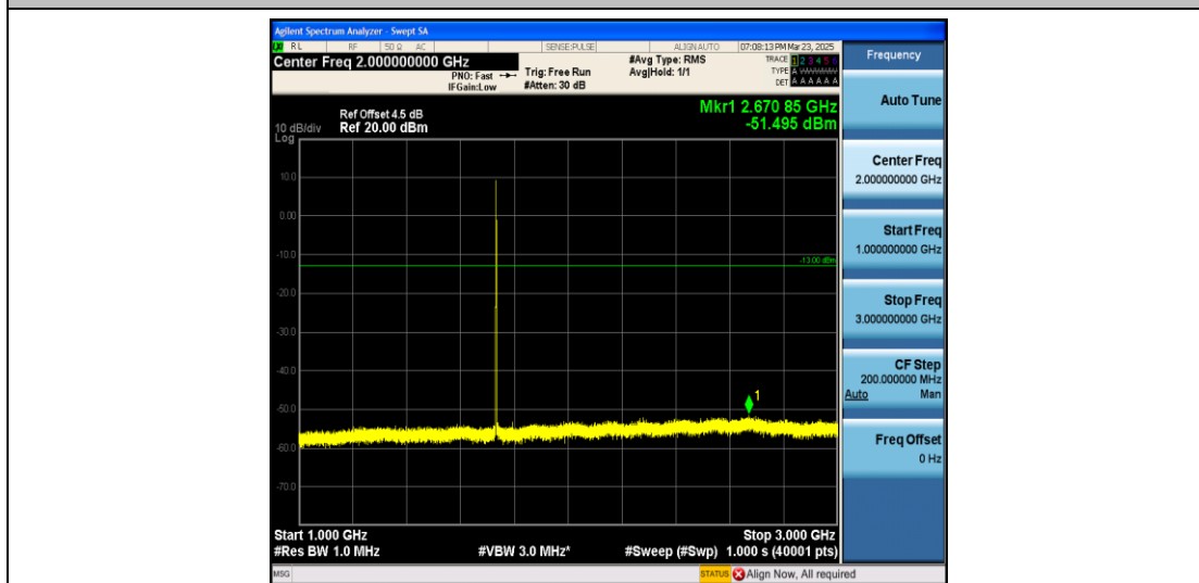
Band4_1.4MHz_16QAM_20175_1RB#0_1000~3000_1000~3000
