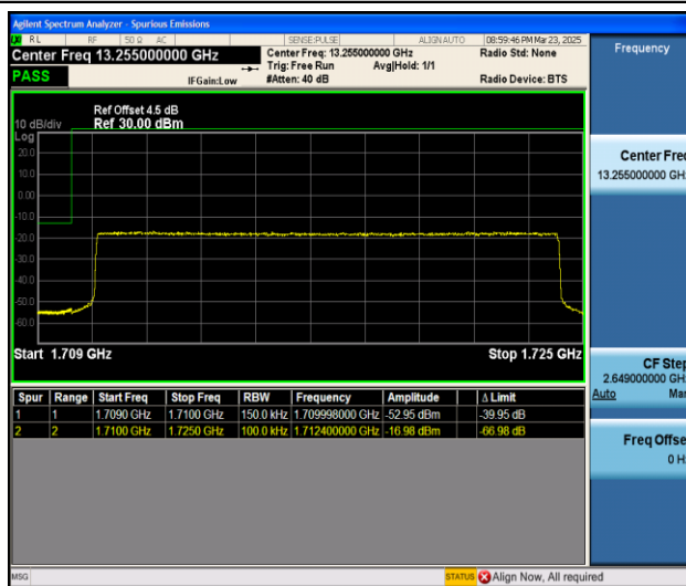
Band4_15MHz_16QAM_20025_75RB#0
