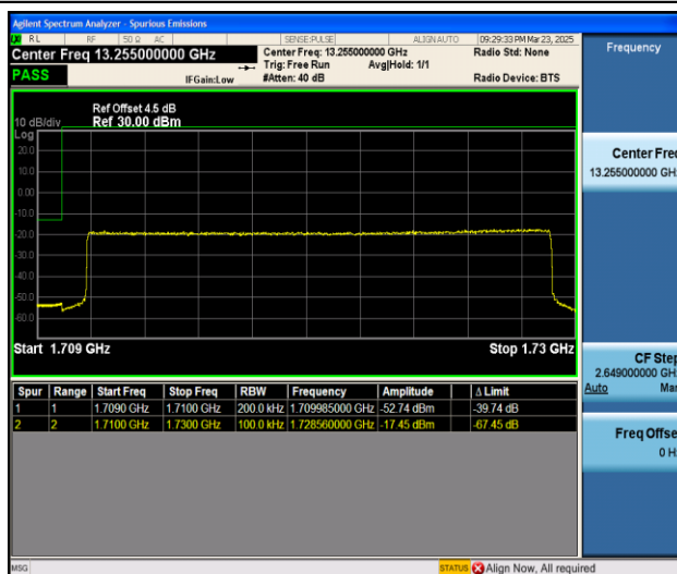
Band4_20MHz_16QAM_20050_100RB#0
