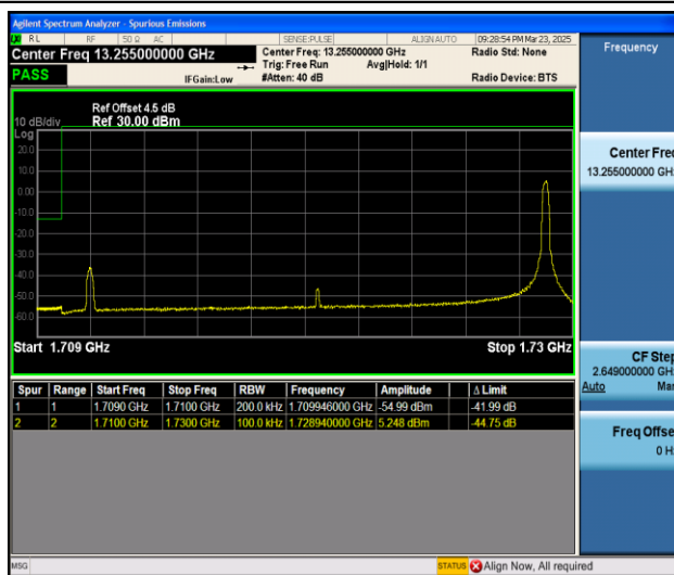
Band4_20MHz_QPSK_20050_1RB#99
