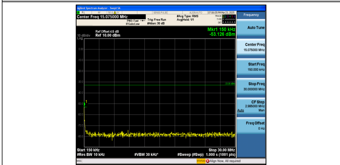
Band4_1.4MHz_16QAM_19957_1RB#0_0.15~30_0.15~30
