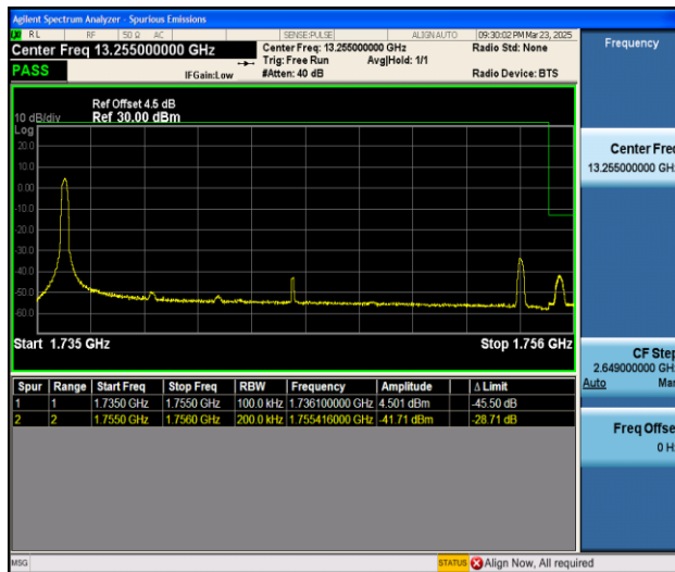
Band4_20MHz_16QAM_20300_1RB#0
