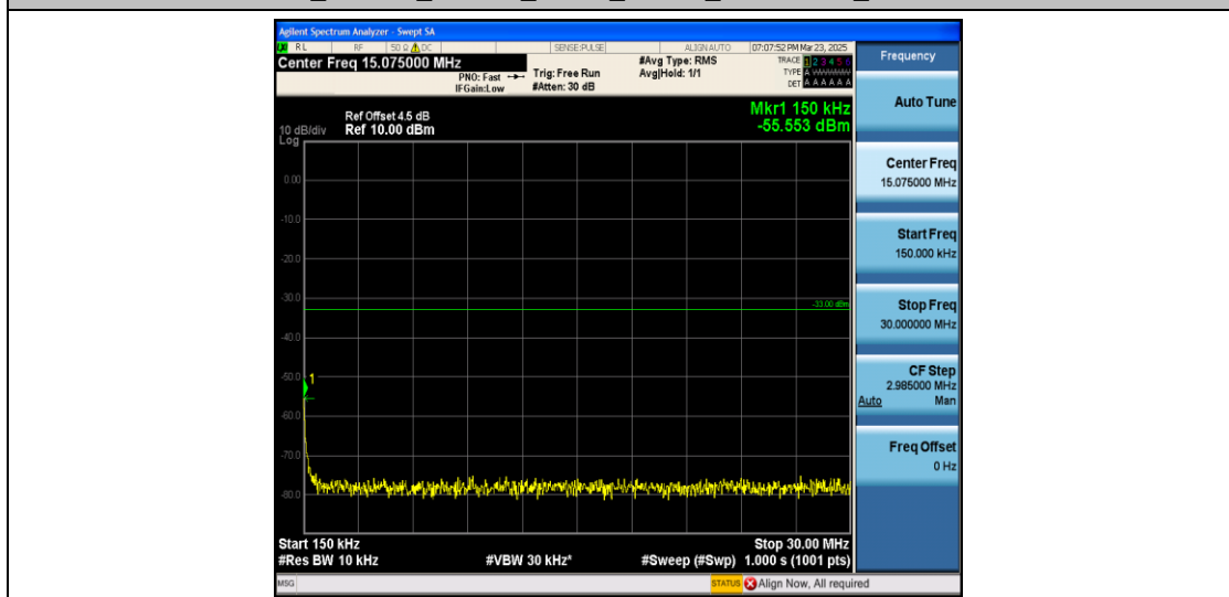
Band4_1.4MHz_16QAM_20175_1RB#0_0.15~30_0.15~30
