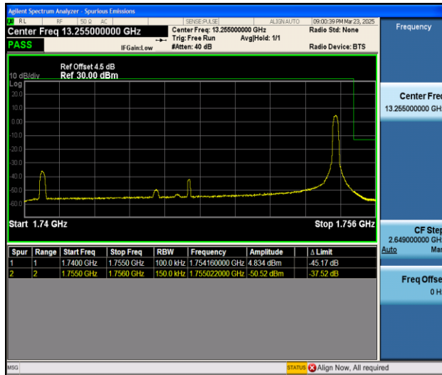
Band4_15MHz_16QAM_20325_1RB#74
