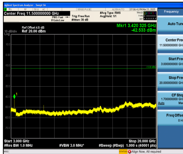
Band4_1.4MHz_16QAM_19957_1RB#0_3000~20000_3000~20000
