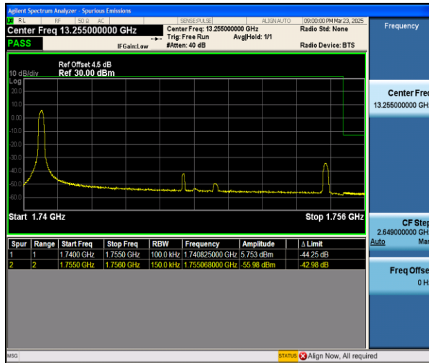
Band4_15MHz_QPSK_20325_1RB#0
