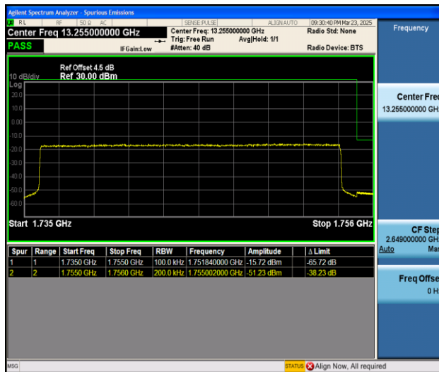
Band4_20MHz_QPSK_20300_100RB#0
