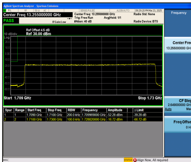
Band4_20MHz_QPSK_20050_100RB#0
