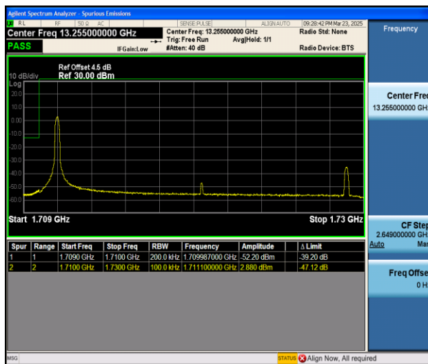
Band4_20MHz_16QAM_20050_1RB#0
