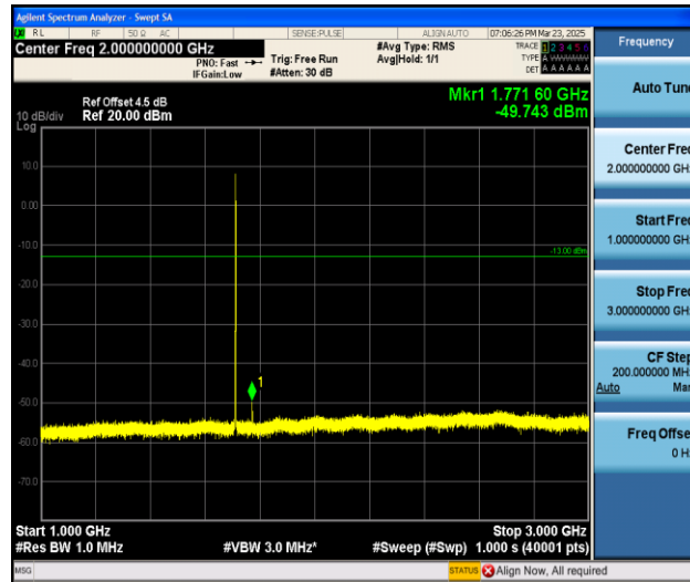
Band4_1.4MHz_16QAM_19957_1RB#0_1000~3000_1000~3000
