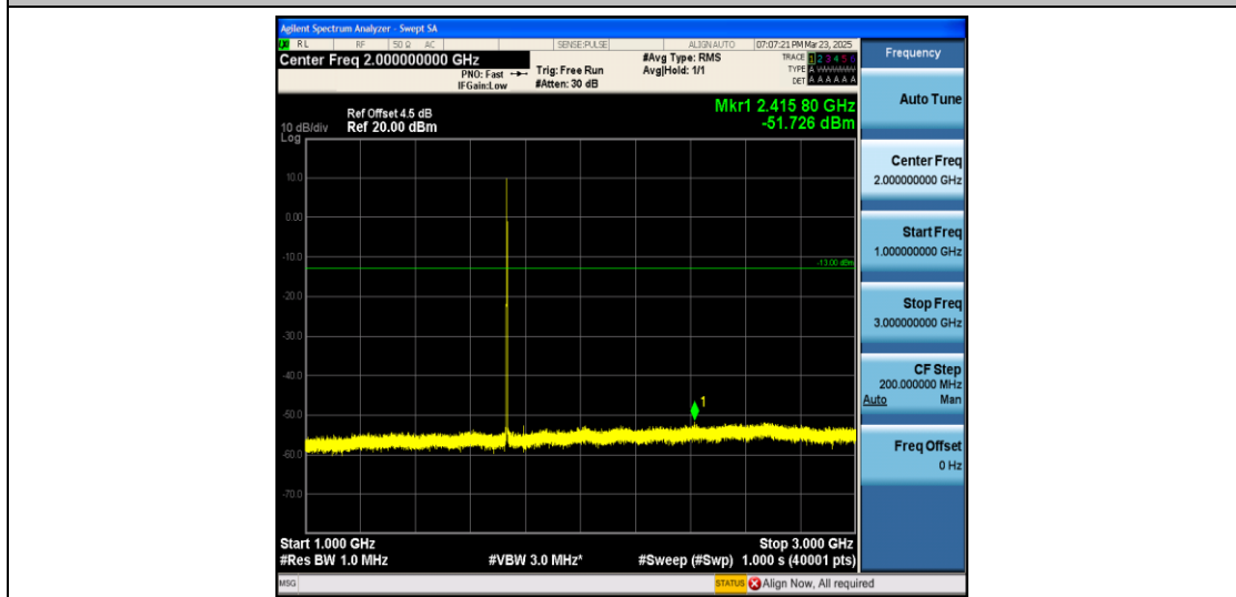
Band4_1.4MHz_QPSK_20175_1RB#0_1000~3000_1000~3000
