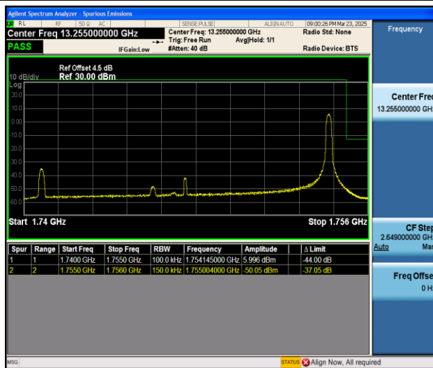
Band4_15MHz_QPSK_20325_1RB#74
