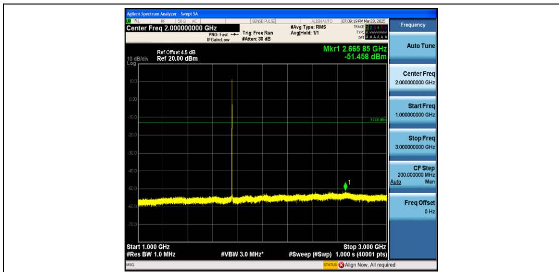
Band4_1.4MHz_QPSK_20393_1RB#0_1000~3000_1000~3000
