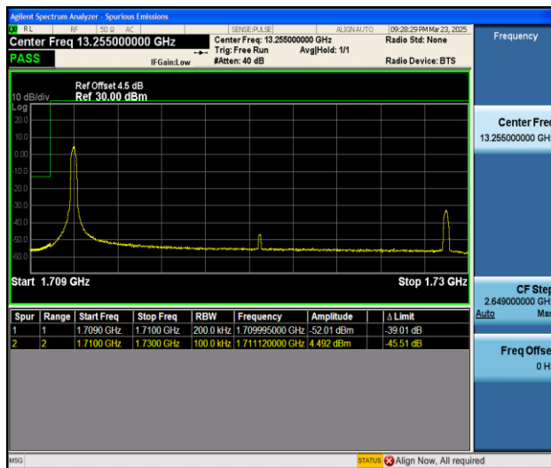
Band4_20MHz_QPSK_20050_1RB#0
