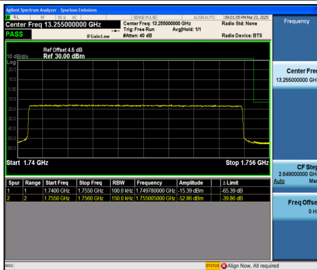
Band4_15MHz_16QAM_20325_75RB#0
