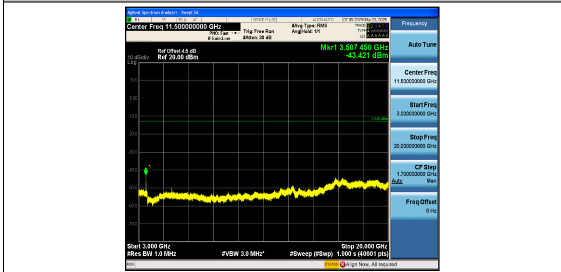
Band4_1.4MHz_QPSK_20393_1RB#0_3000~20000_3000~20000
