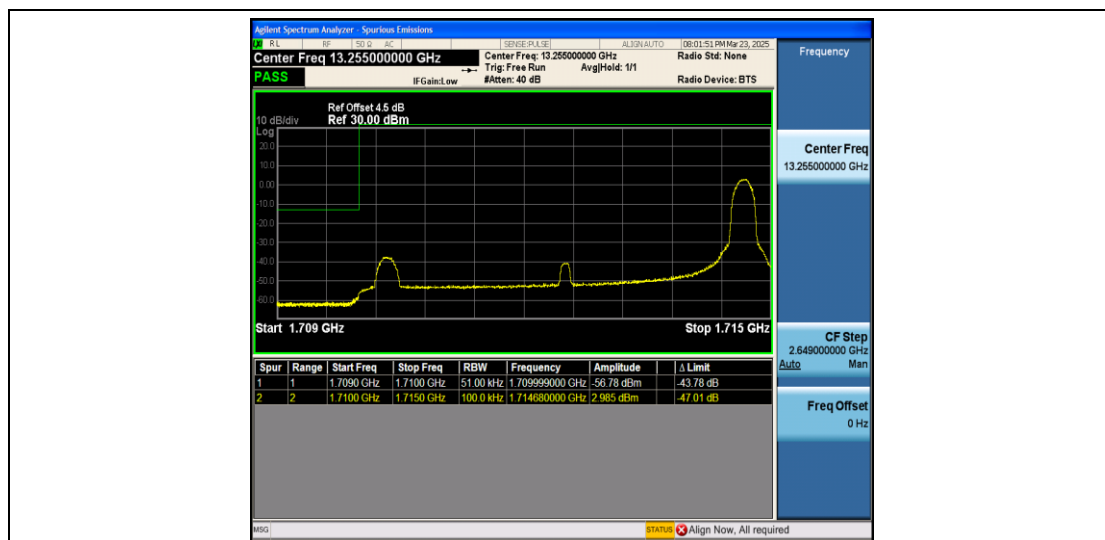
Band4_5MHz_16QAM_19975_1RB#24
