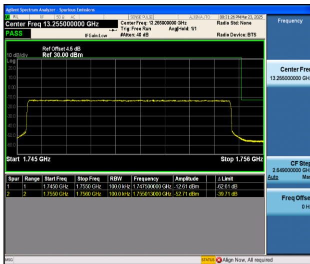
Band4_10MHz_QPSK_20350_50RB#0
