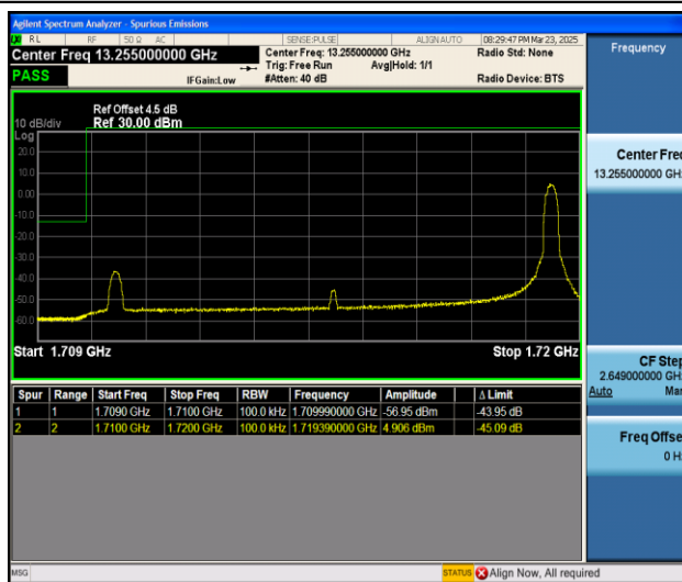
Band4_10MHz_QPSK_20000_1RB#49
