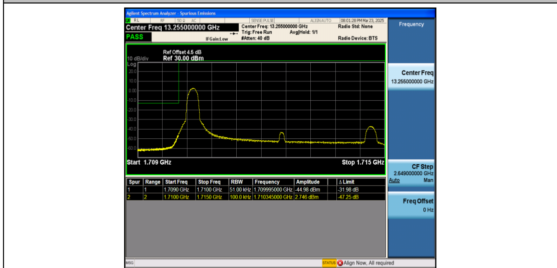
Band4_5MHz_16QAM_19975_1RB#0
