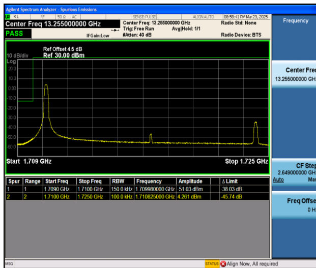
Band4_15MHz_QPSK_20025_1RB#0
