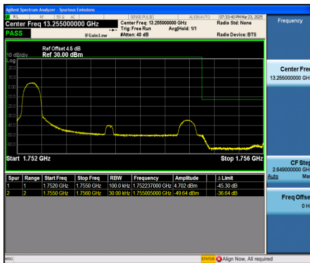
Band4_3MHz_16QAM_20385_1RB#0
