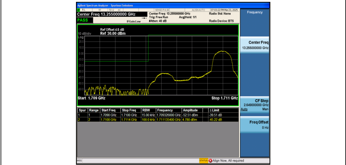
Band4_1.4MHz_QPSK_19957_1RB#5
