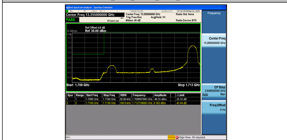
Band4_3MHz_QPSK_19965_1RB#14
