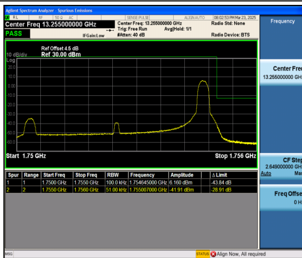
Band4_5MHz_QPSK_20375_1RB#24
