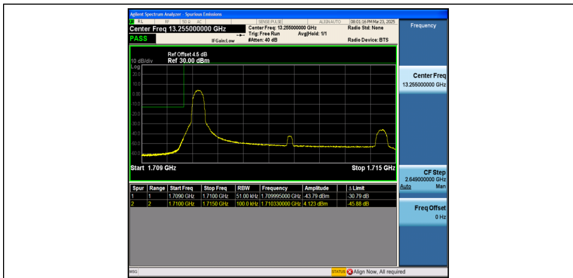
Band4_5MHz_QPSK_19975_1RB#0
