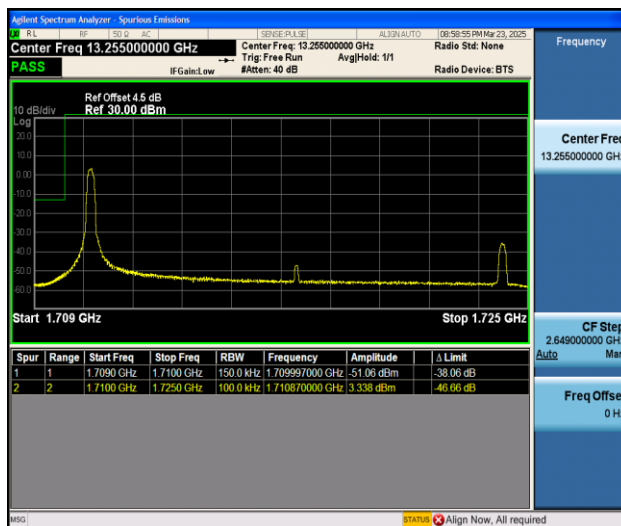
Band4_15MHz_16QAM_20025_1RB#0
