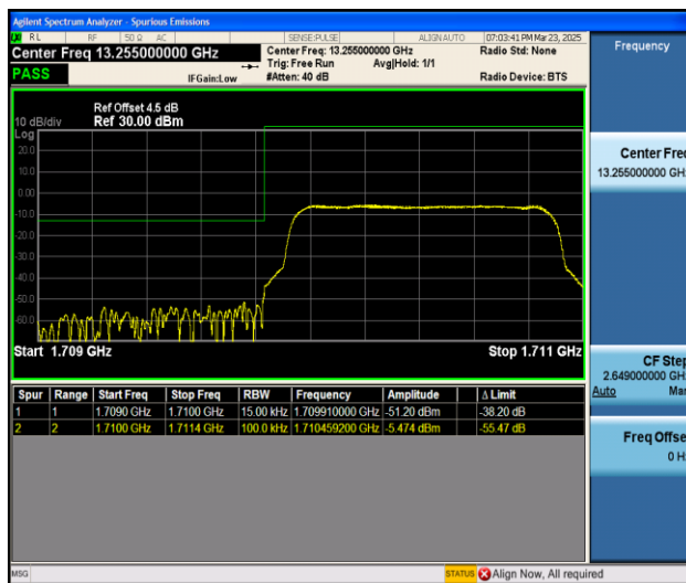
Band4_1.4MHz_QPSK_19957_6RB#0
