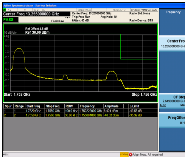
Band4_3MHz_QPSK_20385_1RB#0
