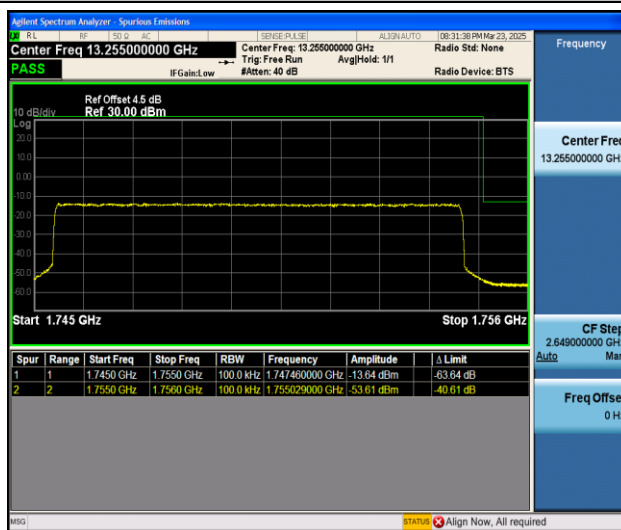
Band4_10MHz_16QAM_20350_50RB#0
