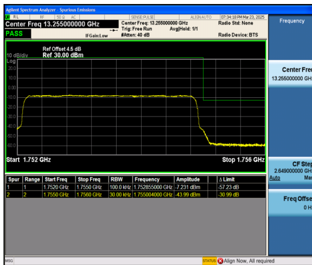
Band4_3MHz_QPSK_20385_15RB#0
