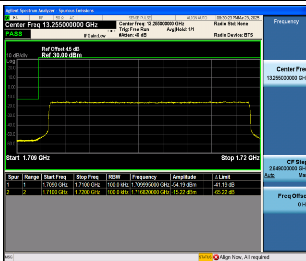
Band4_10MHz_16QAM_20000_50RB#0
