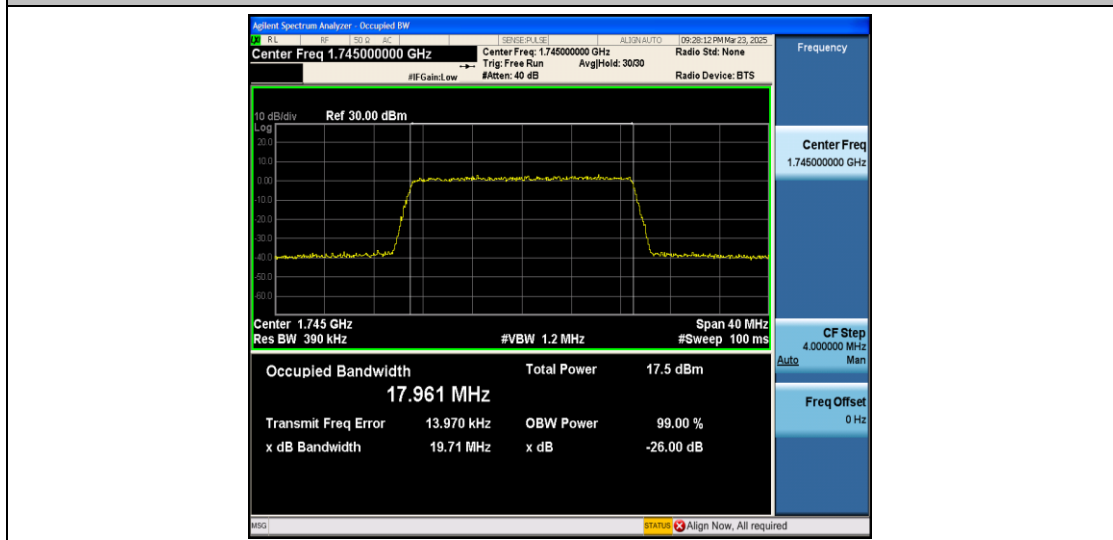
Band4-20MHz-16QAM-20300-100RB#0-PASS
