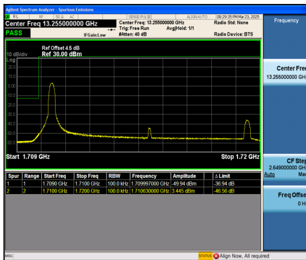
Band4_10MHz_16QAM_20000_1RB#0
