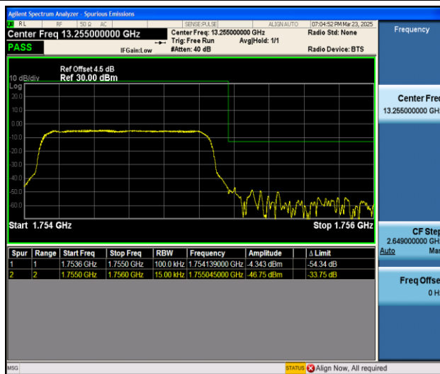
Band4_1.4MHz_16QAM_20393_6RB#0
