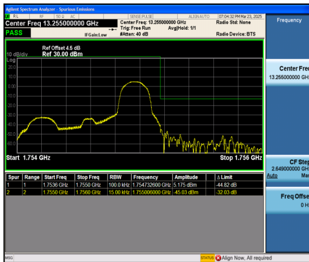
Band4_1.4MHz_16QAM_20393_1RB#5
