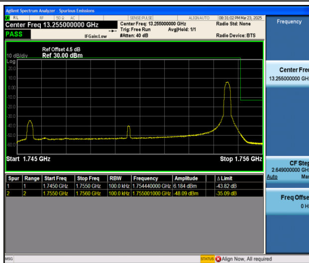
Band4_10MHz_QPSK_20350_1RB#49
