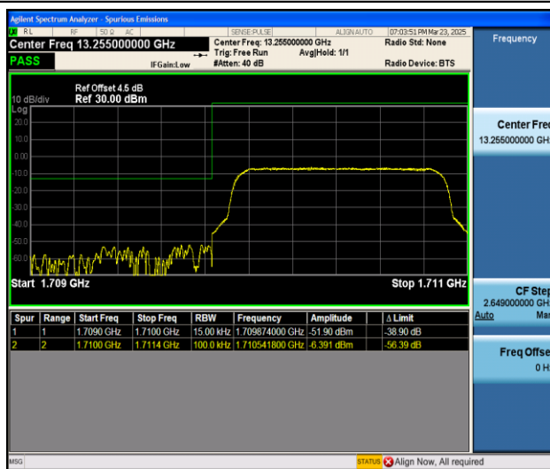
Band4_1.4MHz_16QAM_19957_6RB#0
