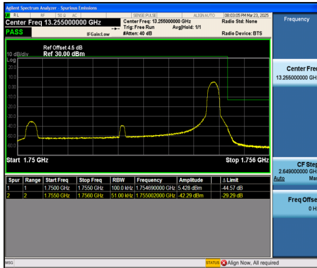
Band4_5MHz_16QAM_20375_1RB#24
