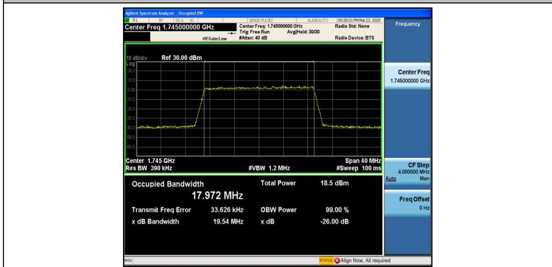
Band4-20MHz-QPSK-20300-100RB#0-PASS
