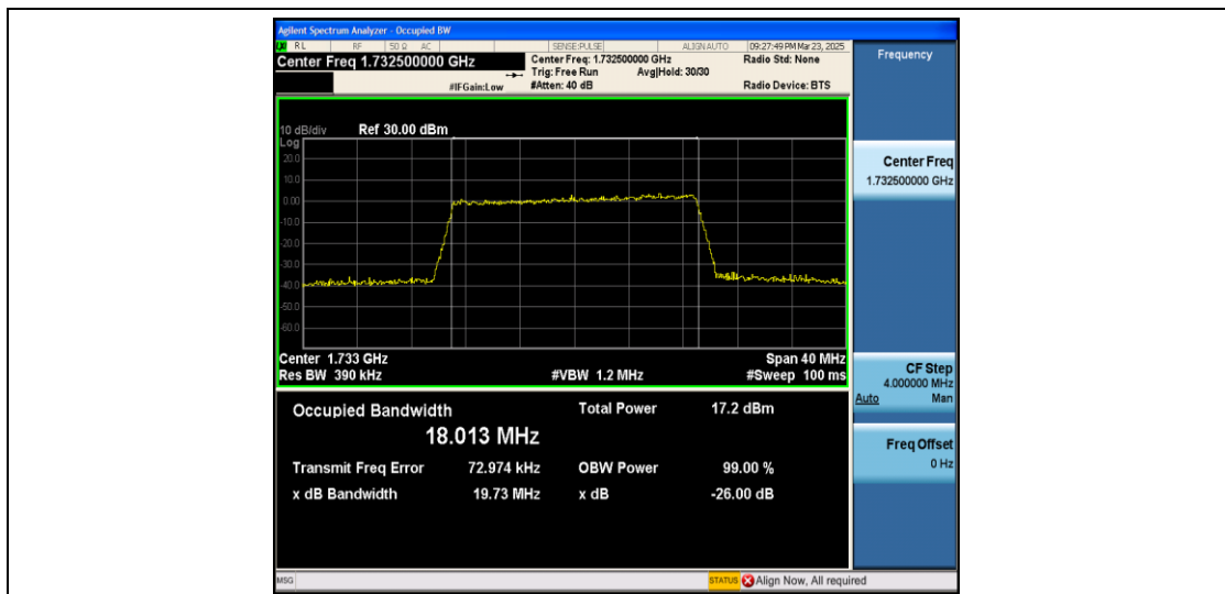
Band4-20MHz-16QAM-20175-100RB#0-PASS
