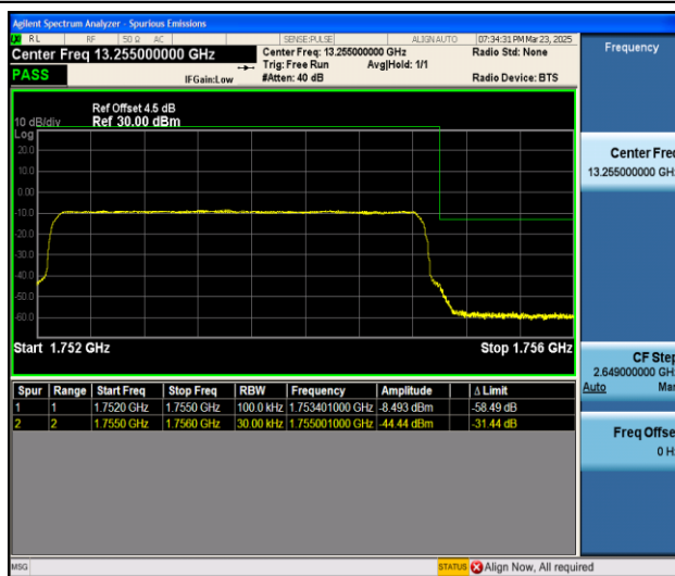
Band4_3MHz_16QAM_20385_15RB#0
