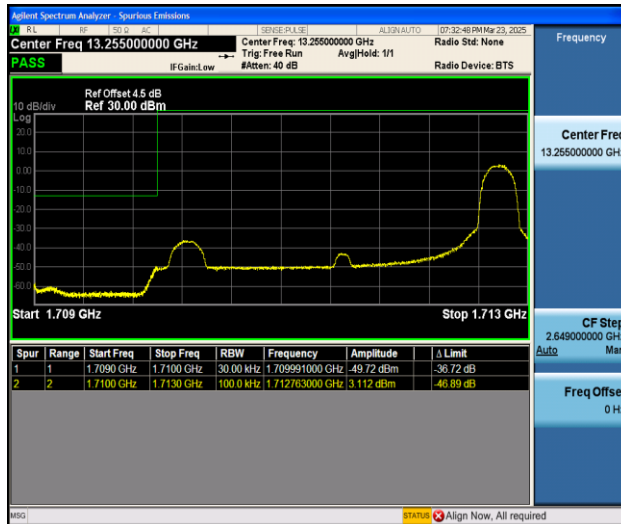
Band4_3MHz_16QAM_19965_1RB#14
