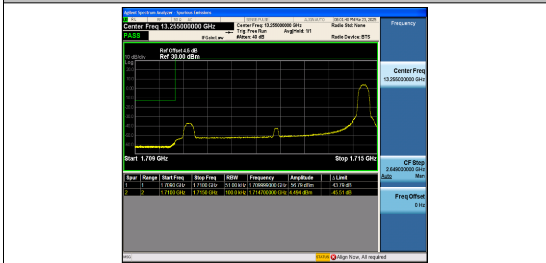
Band4_5MHz_QPSK_19975_1RB#24
