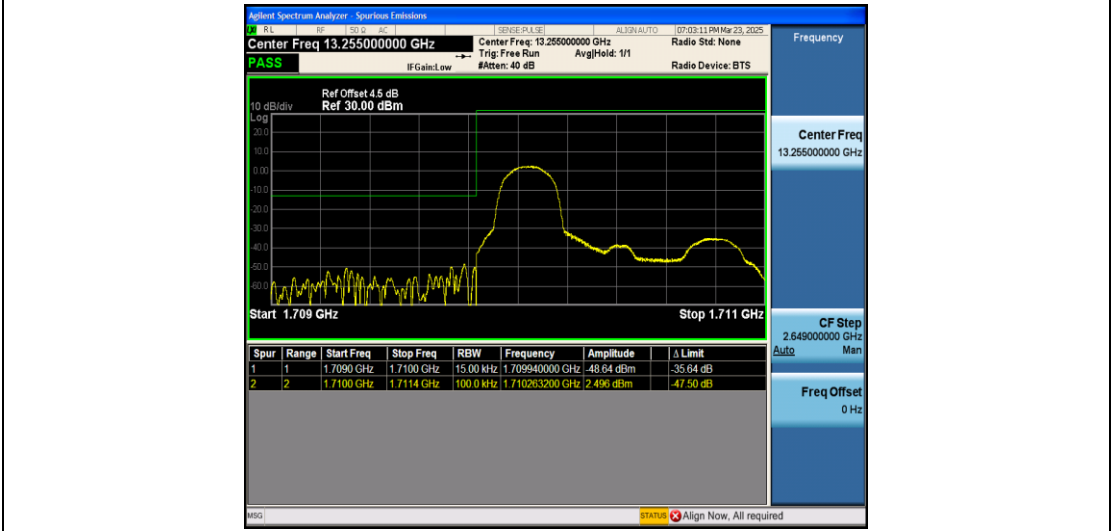
Band4_1.4MHz_16QAM_19957_1RB#0
