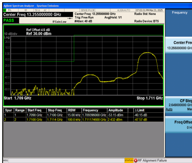
Band4_1.4MHz_16QAM_19957_1RB#5
