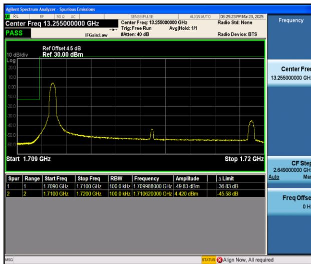
Band4_10MHz_QPSK_20000_1RB#0
