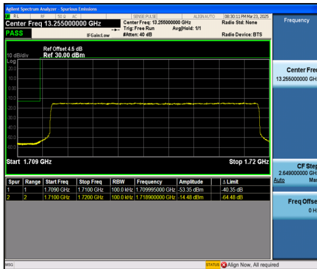
Band4_10MHz_QPSK_20000_50RB#0
