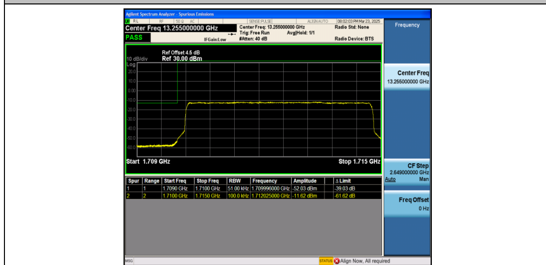
Band4_5MHz_QPSK_19975_25RB#0
