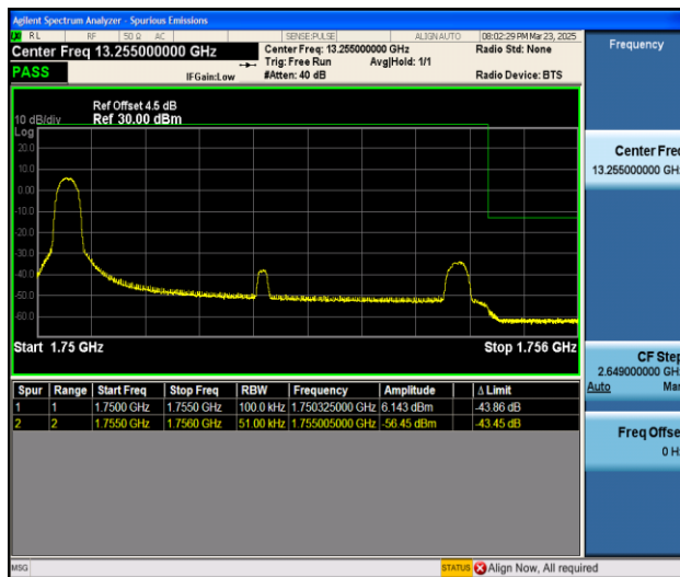
Band4_5MHz_QPSK_20375_1RB#0
