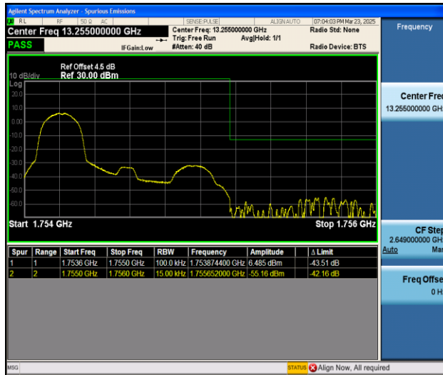
Band4_1.4MHz_QPSK_20393_1RB#0
