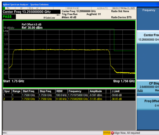
Band4_5MHz_QPSK_20375_25RB#0
