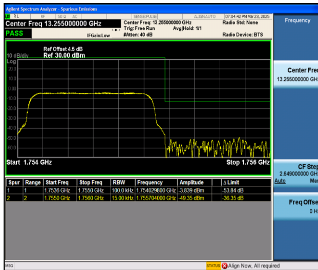
Band4_1.4MHz_QPSK_20393_6RB#0
