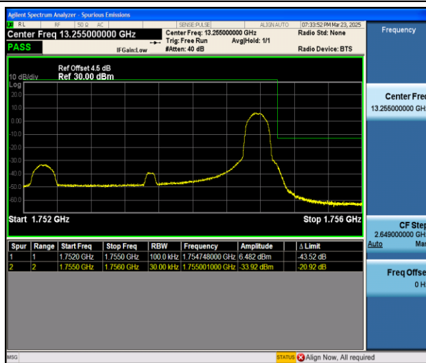
Band4_3MHz_QPSK_20385_1RB#14
