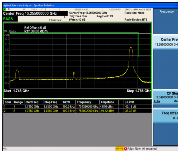
Band4_10MHz_16QAM_20350_1RB#49
