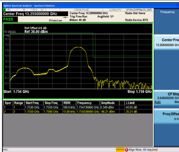
Band4_1.4MHz_QPSK_20393_1RB#5
