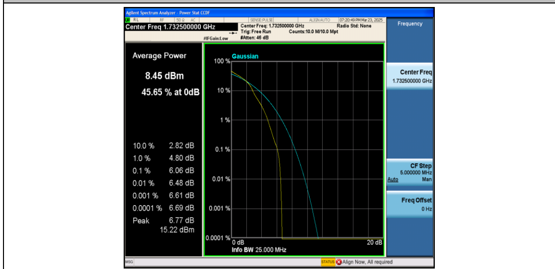
Band4-1.4MHz-16QAM-20175-1RB#0-PASS
