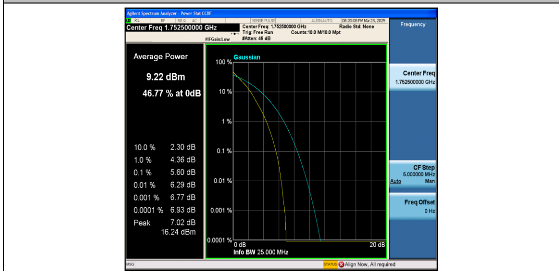
Band4-5MHz-QPSK-20375-25RB#0-PASS
