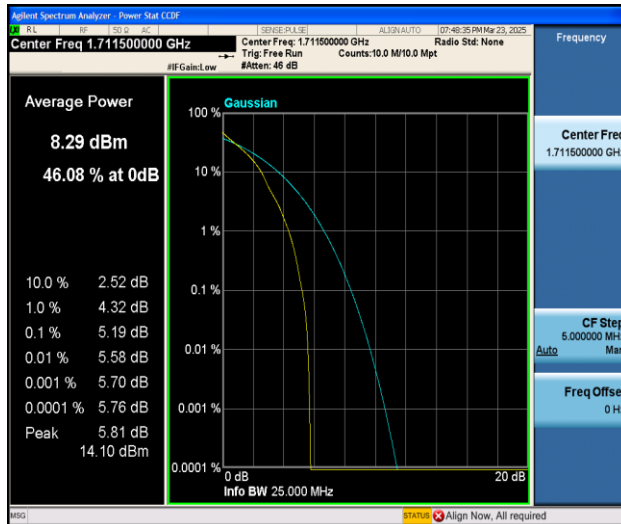
Band4-3MHz-QPSK-19965-1RB#0-PASS
