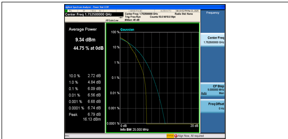
Band4-5MHz-16QAM-20375-1RB#0-PASS
