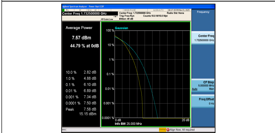
Band4-10MHz-16QAM-20175-50RB#0-PASS
