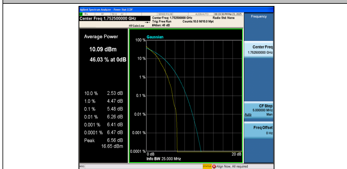
Band4-5MHz-QPSK-20375-1RB#0-PASS
