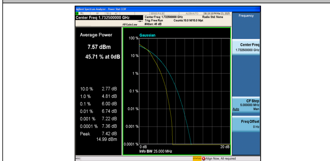
Band4-5MHz-16QAM-20175-25RB#0-PASS
