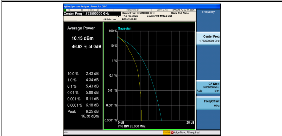
Band4-3MHz-QPSK-20385-1RB#0-PASS
