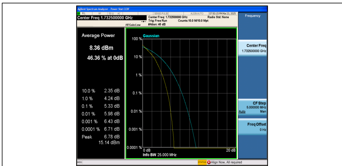
Band4-3MHz-QPSK-20175-15RB#0-PASS
