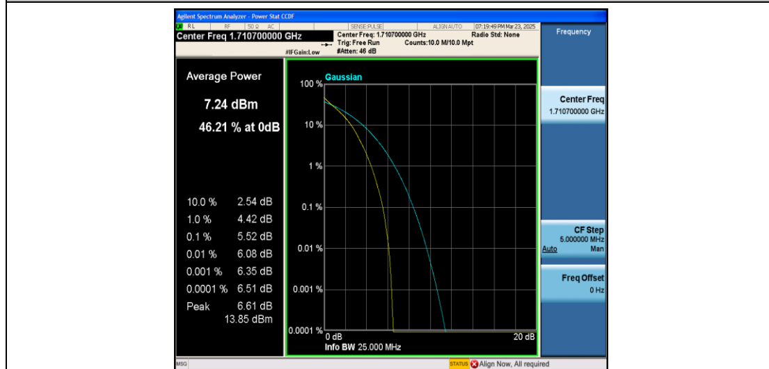
Band4-1.4MHz-QPSK-19957-6RB#0-PASS
