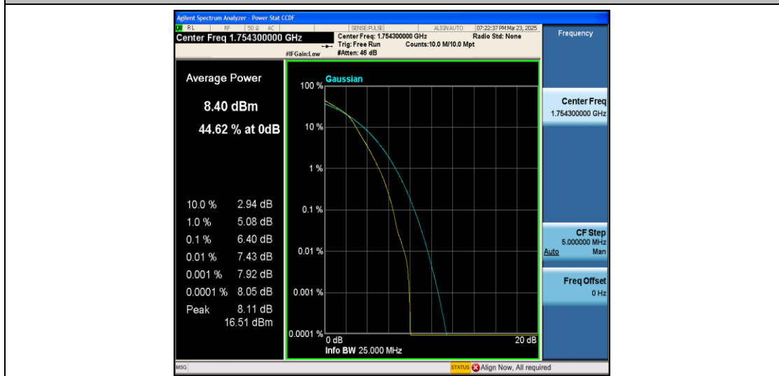
Band4-1.4MHz-16QAM-20393-6RB#0-PASS
