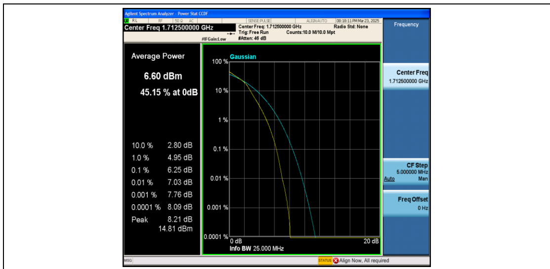
Band4-5MHz-16QAM-19975-25RB#0-PASS
