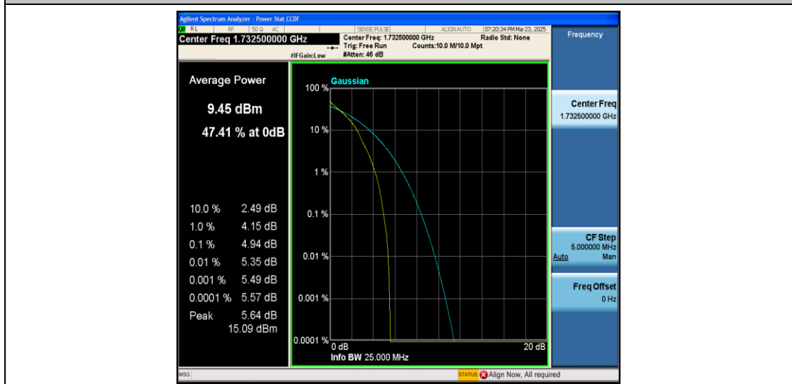
Band4-1.4MHz-QPSK-20175-1RB#0-PASS
