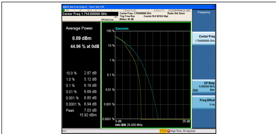
Band4-1.4MHz-16QAM-20393-1RB#0-PASS
