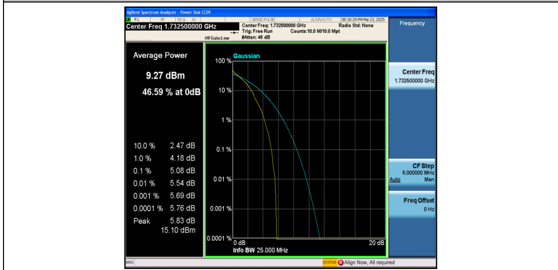
Band4-5MHz-QPSK-20175-1RB#0-PASS
