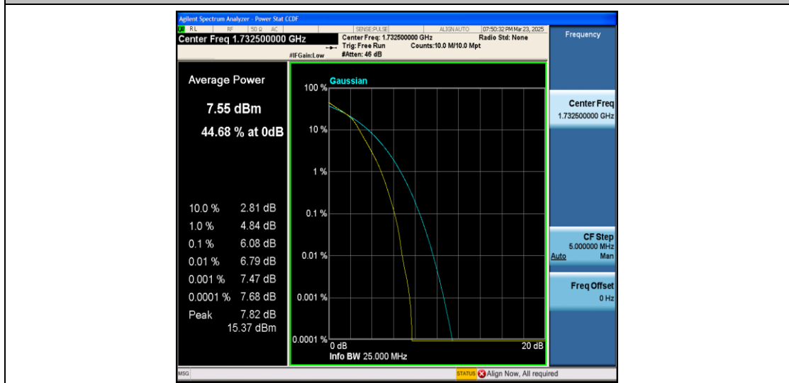
Band4-3MHz-16QAM-20175-15RB#0-PASS
