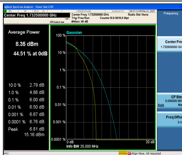
Band4-10MHz-16QAM-20175-1RB#0-PASS
