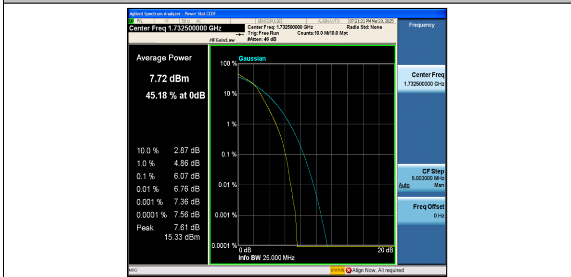
Band4-1.4MHz-16QAM-20175-6RB#0-PASS
