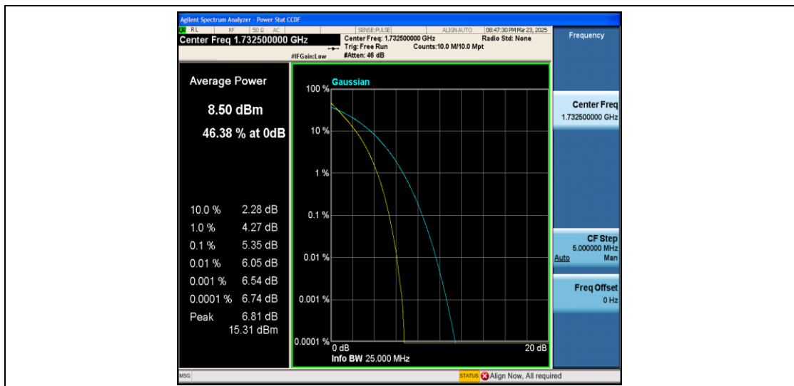
Band4-10MHz-QPSK-20175-50RB#0-PASS
