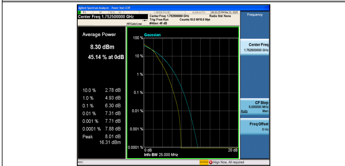
Band4-5MHz-16QAM-20375-25RB#0-PASS
