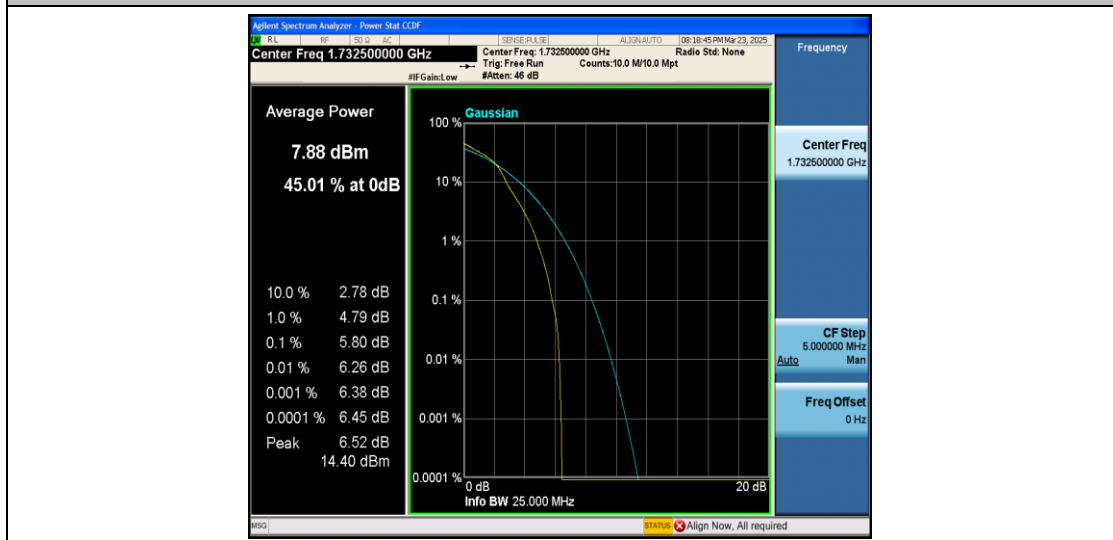
Band4-5MHz-16QAM-20175-1RB#0-PASS
