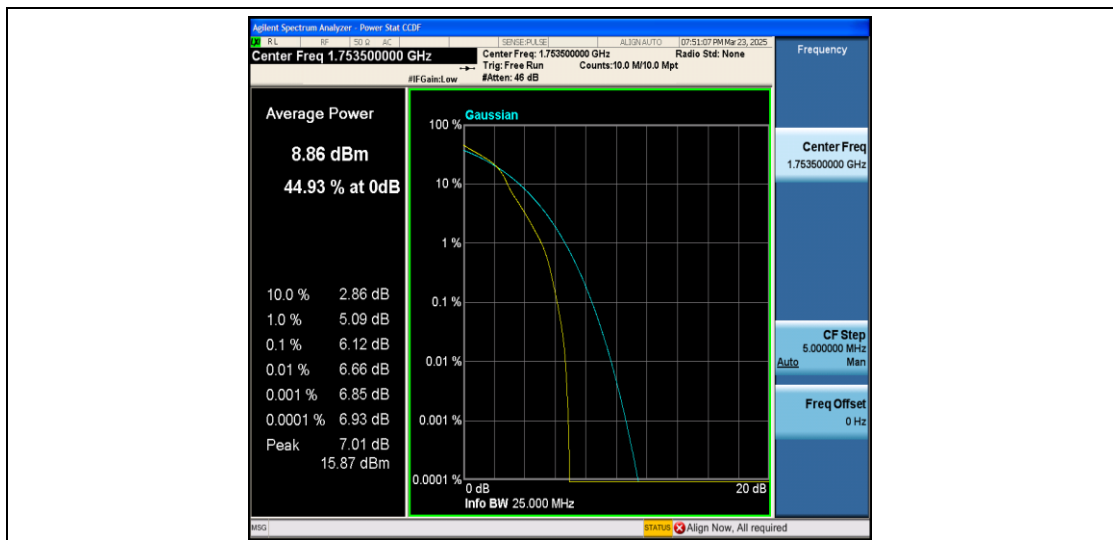
Band4-3MHz-16QAM-20385-1RB#0-PASS
