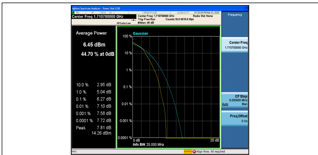
Band4-1.4MHz-16QAM-19957-6RB#0-PASS
