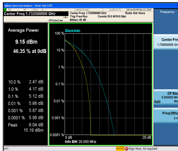
Band4-10MHz-QPSK-20175-1RB#0-PASS
