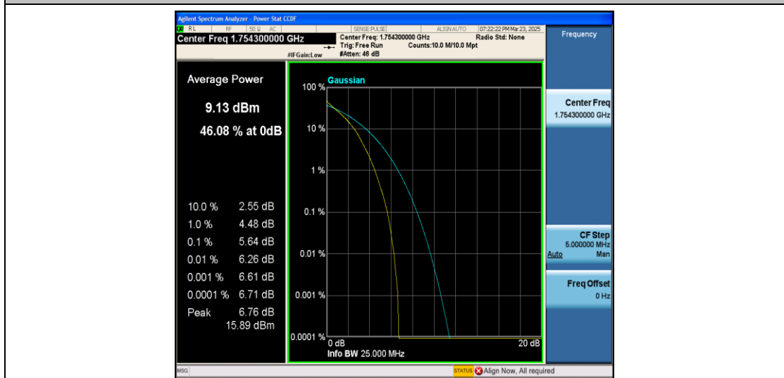
Band4-1.4MHz-QPSK-20393-6RB#0-PASS
