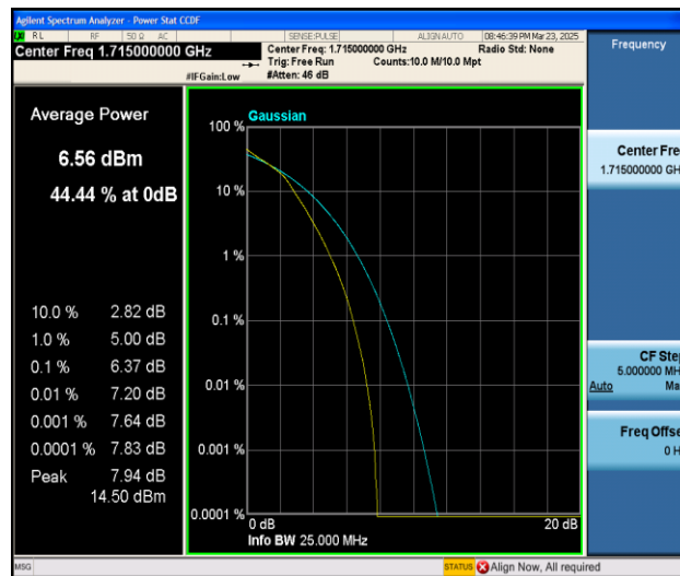
Band4-10MHz-16QAM-20000-50RB#0-PASS
