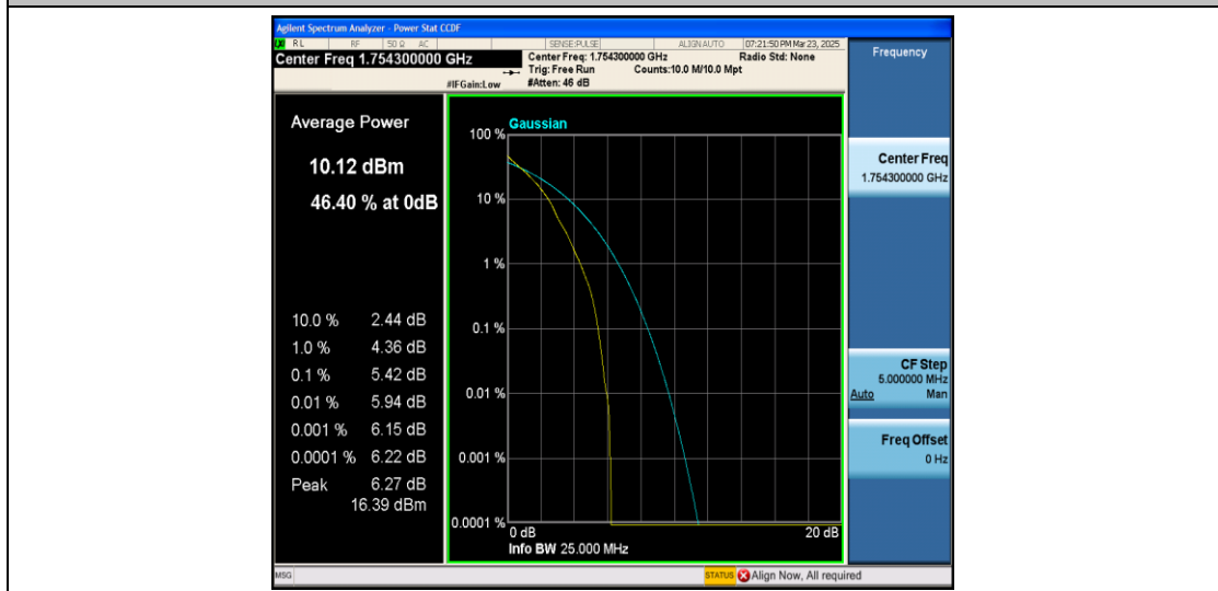
Band4-1.4MHz-QPSK-20393-1RB#0-PASS
