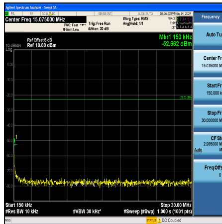
Band12_3MHz_QPSK_23165_1RB#0_0.15~30_0.15~30
