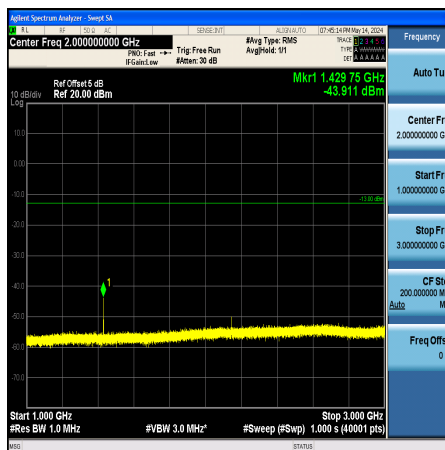
Band12_1.4MHz_QPSK_23173_1RB#0_1000~3000_1000~3000
