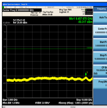
Band12_10MHz_QPSK_23095_1RB#0_3000~10000_3000~10000
