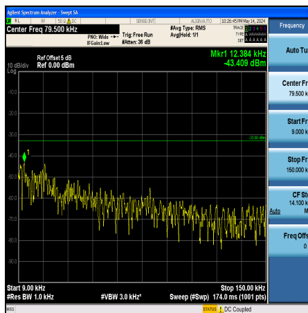
Band12_3MHz_QPSK_23165_1RB#0_0.009~0.15_0.009~0.15
