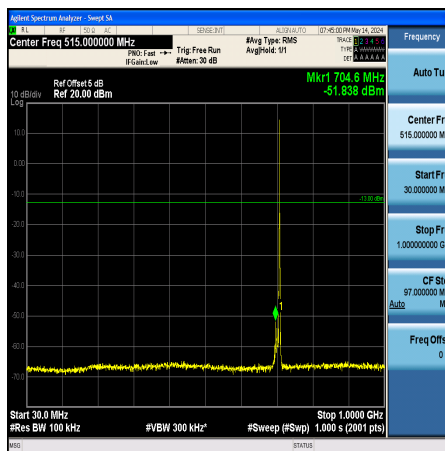
Band12_1.4MHz_QPSK_23173_1RB#0_30~1000_30~1000
