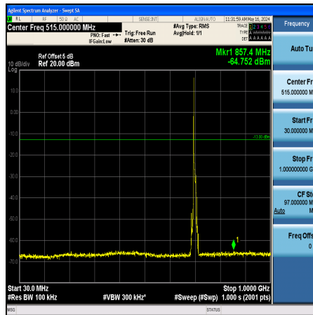
Band12_10MHz_QPSK_23095_1RB#0_30~1000_30~1000
