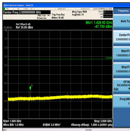
Band12_3MHz_QPSK_23165_1RB#0_1000~3000_1000~3000
