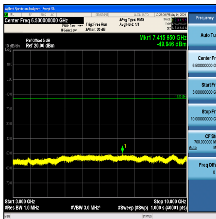
Band12_3MHz_16QAM_23095_1RB#0_3000~10000_3000~10000
