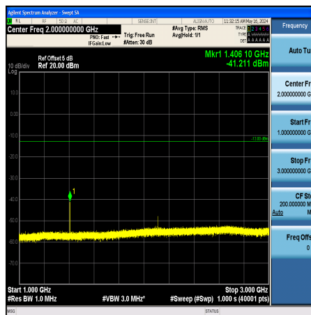
Band12_10MHz_QPSK_23095_1RB#0_1000~3000_1000~3000
