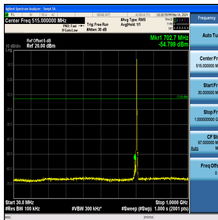
Band12_3MHz_QPSK_23165_1RB#0_30~1000_30~1000
