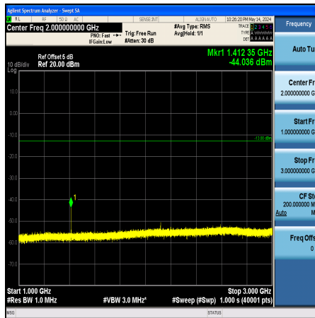
Band12_3MHz_16QAM_23095_1RB#0_1000~3000_1000~3000
