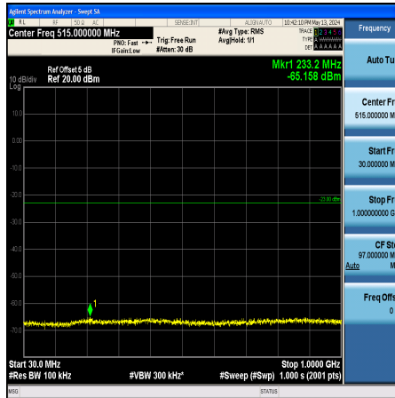
Band2_5MHz_QPSK_18900_1RB#0_30~1000_30~1000
