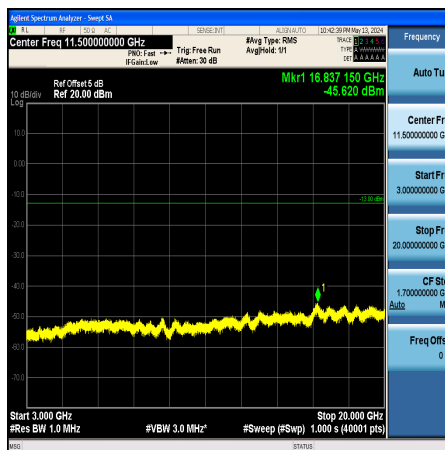
Band2_5MHz_QPSK_18900_1RB#0_3000~20000_3000~20000
