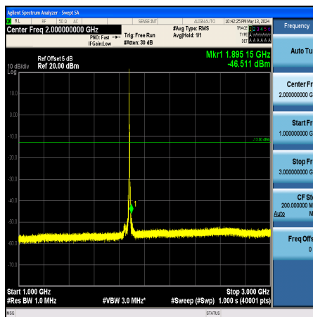
Band2_5MHz_QPSK_18900_1RB#0_1000~3000_1000~3000
