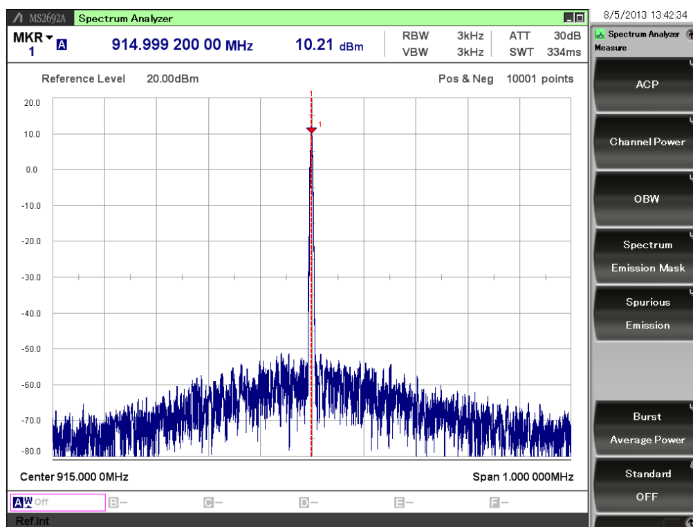
Figure 112. Conducted Measurement Result, 4463-PCE20C915 in a Reduced ( \sim 10 dBm) Power State
